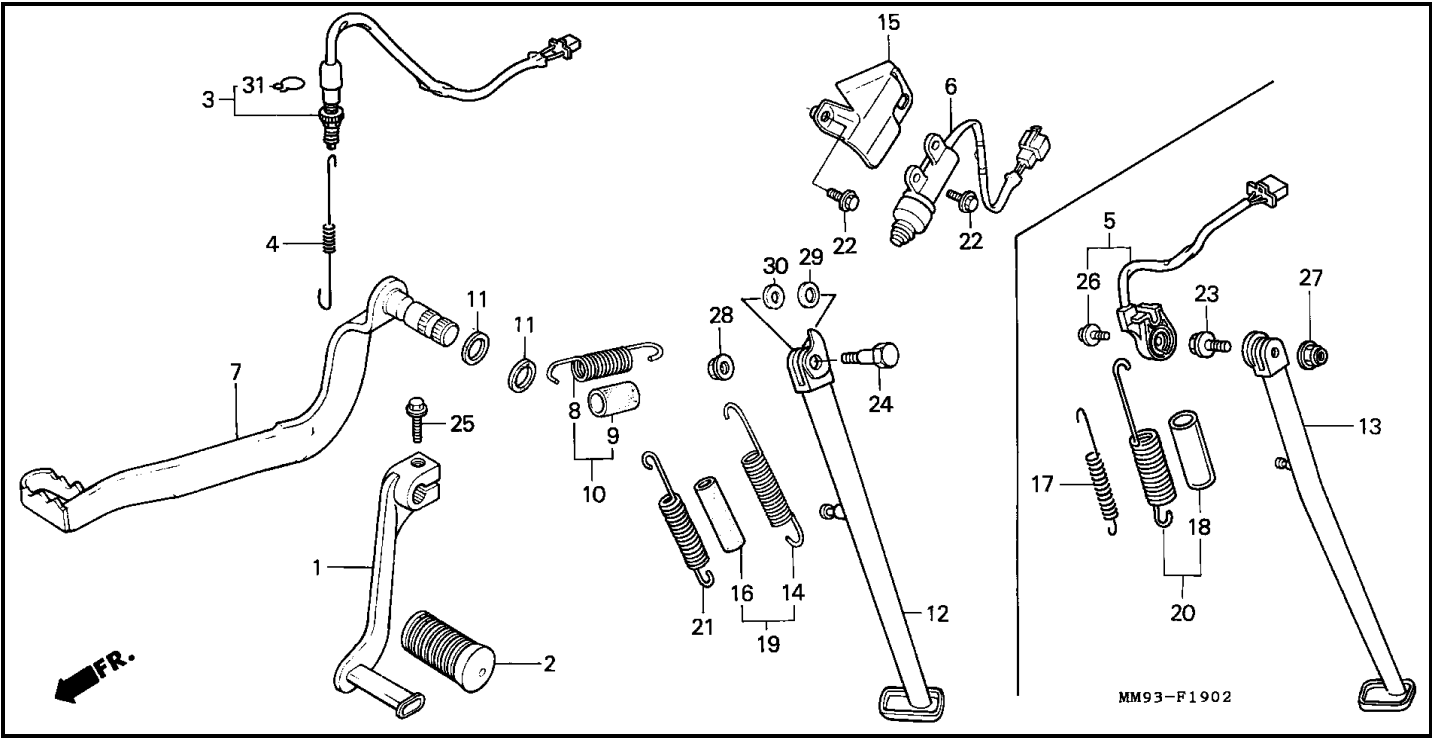
Bloque F-19-2 PEDAL/ESTANTE (XL600VM/VN/VP/VR)
