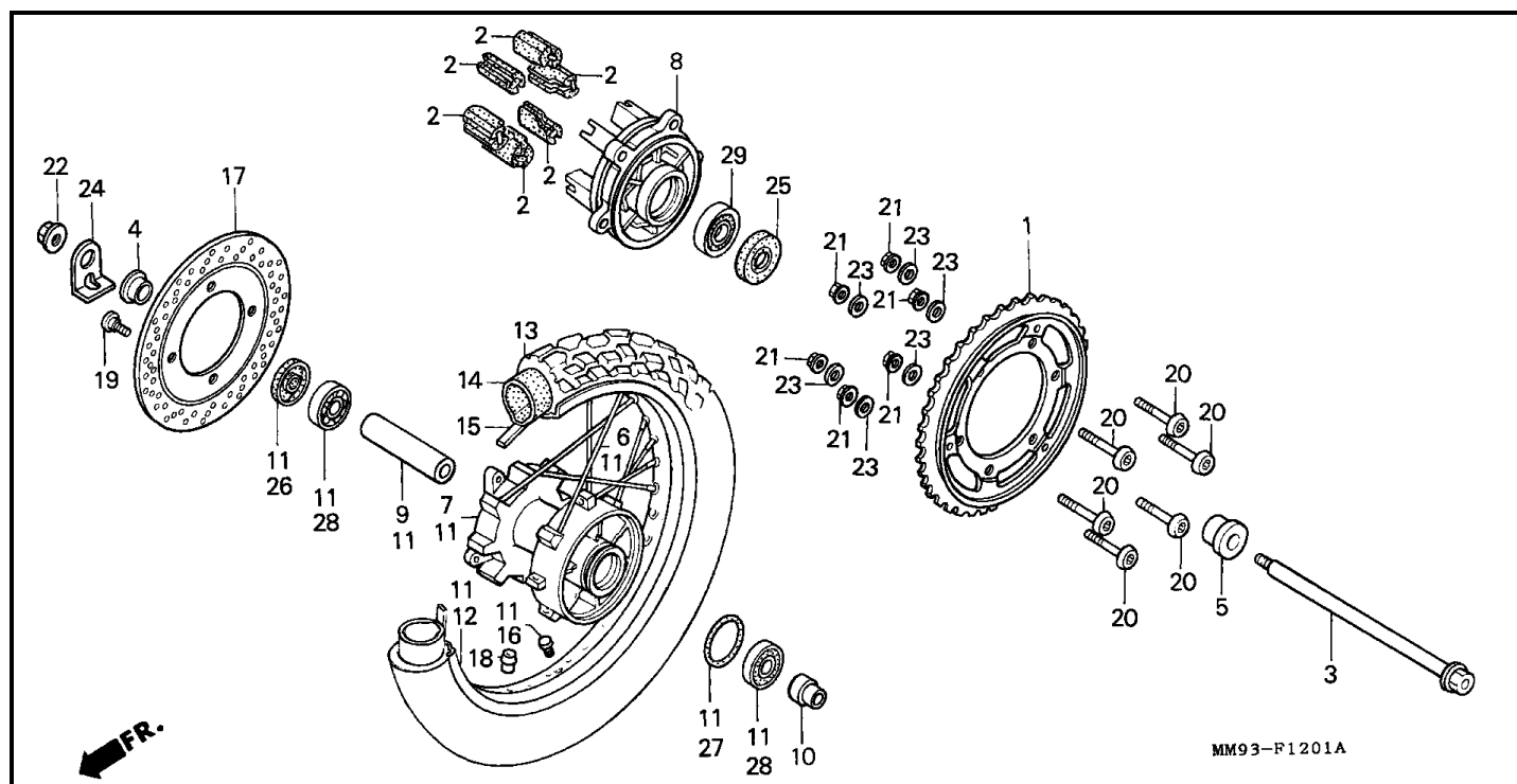
Bloque F-12-1 RUEDA TRASERA (XL600VM/VN/VP/VR)
