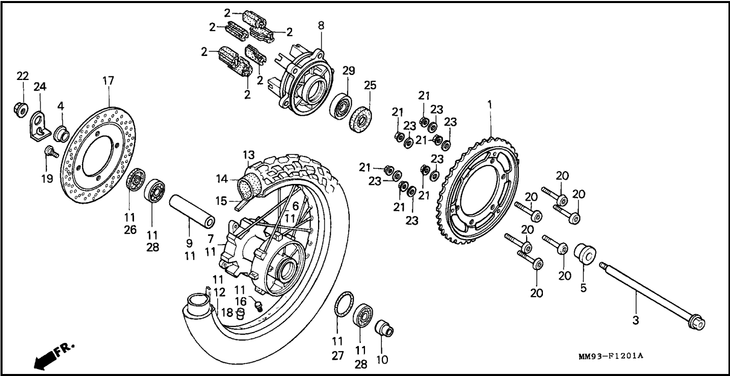
Bloque F-12-1 RUEDA TRASERA (XL600VM/VN/VP/VR)
