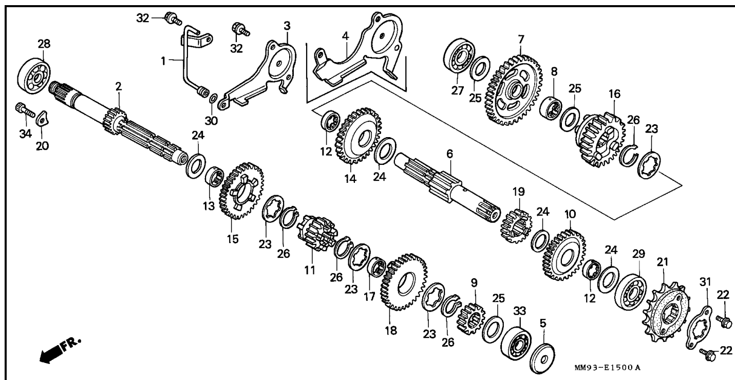
Bloque E-15 TRANSMISION
