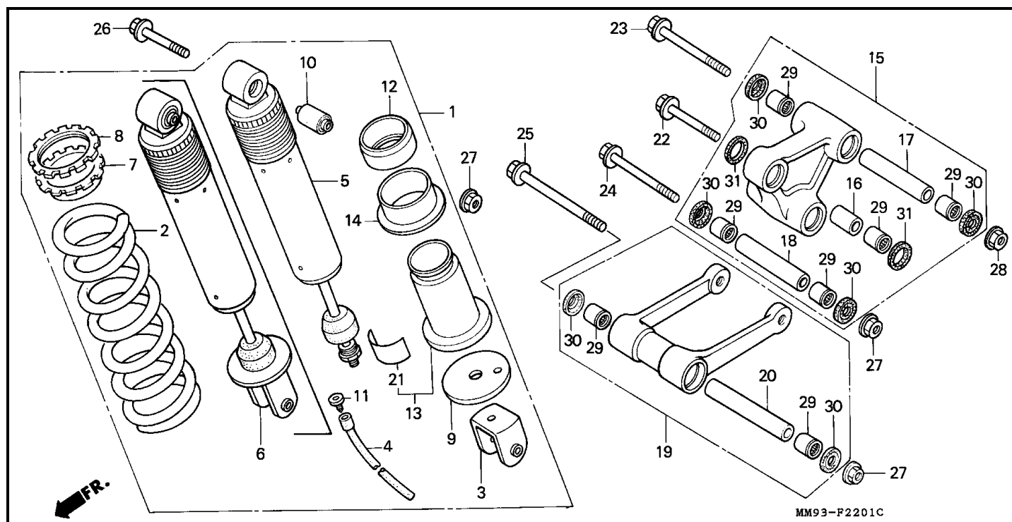
Bloque F-22-1 ALMOHADILLA TRASERA (XL600VK/VL/VM/VN/VP/VR)
