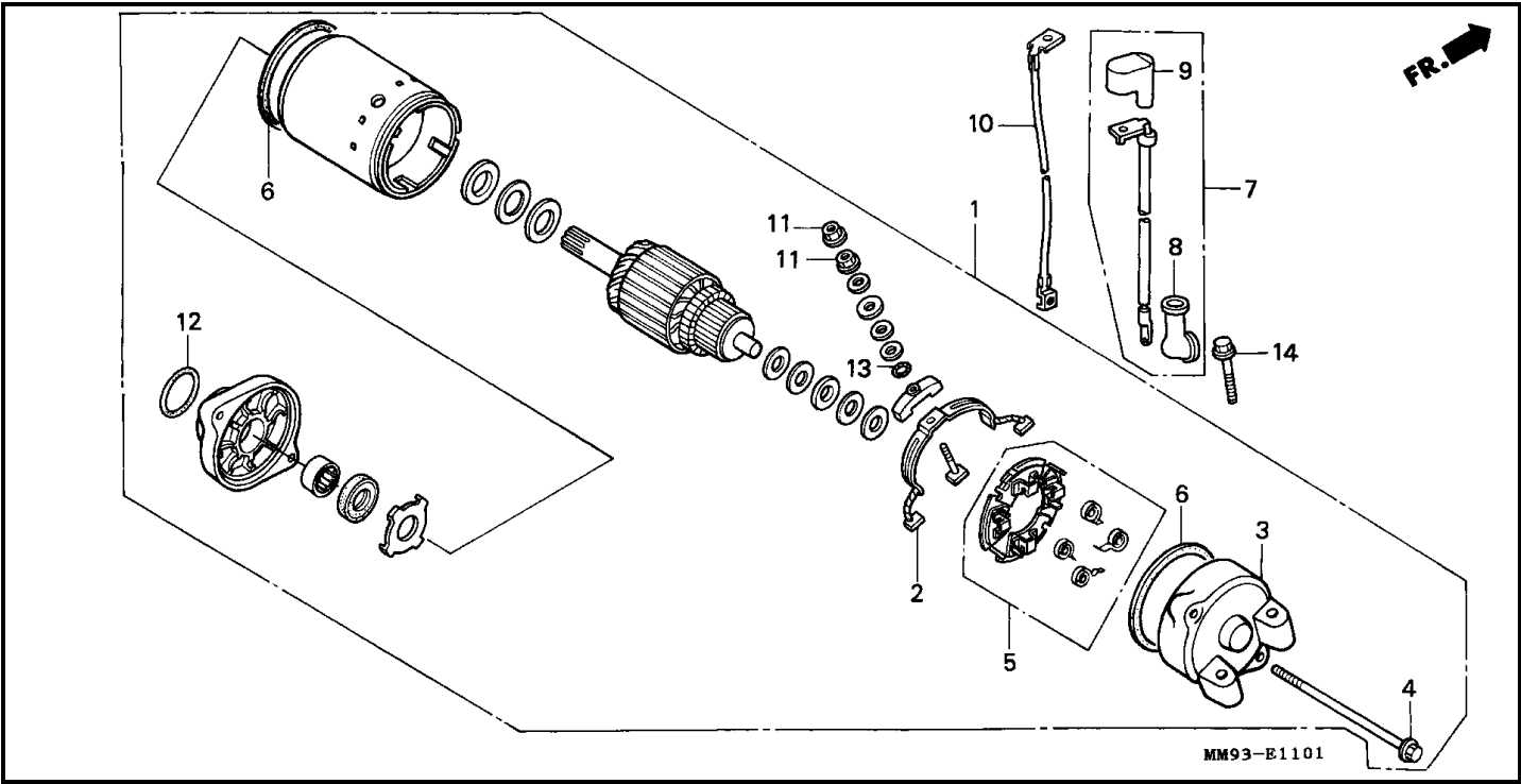
Bloque E-11-1 MOTOR DE ARRANQUE (XL600VK/VL/VM/VN/VP/VR)
