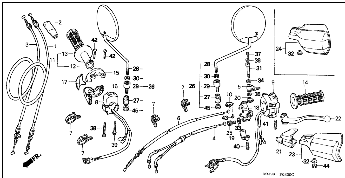
Bloque F-3 INTERRUPTOR/CABLE
