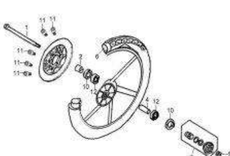
Front Wheel
