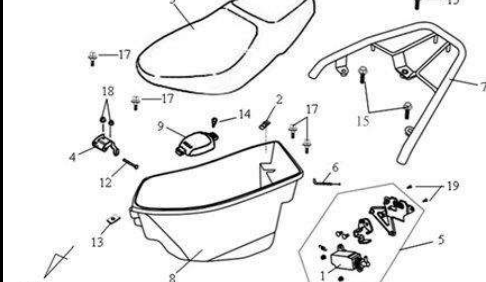
Seat o Rear Grip
