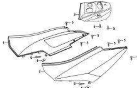
Body Cover
