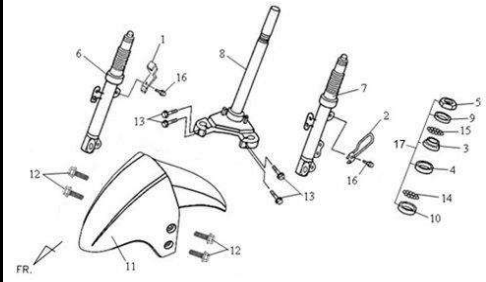
Steering Stem o Front Cushion
