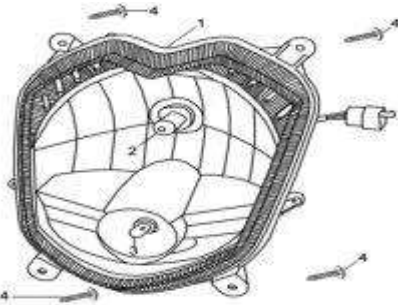
Head Light
