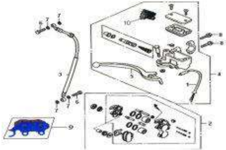
Front Brake Master Cylinder
