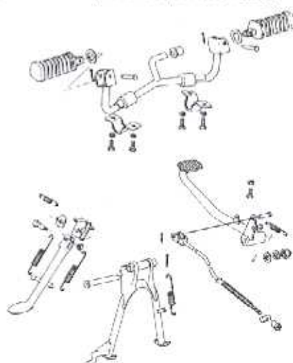
20-1. Footrests, Stands, Brake Pedal ... Page 43
