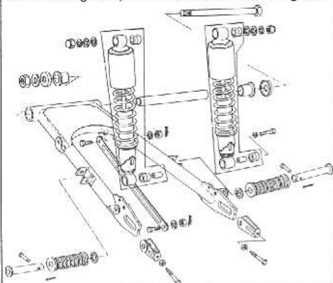
19-1. Swing Arm, Rear Shock Absorber. . Page 39
