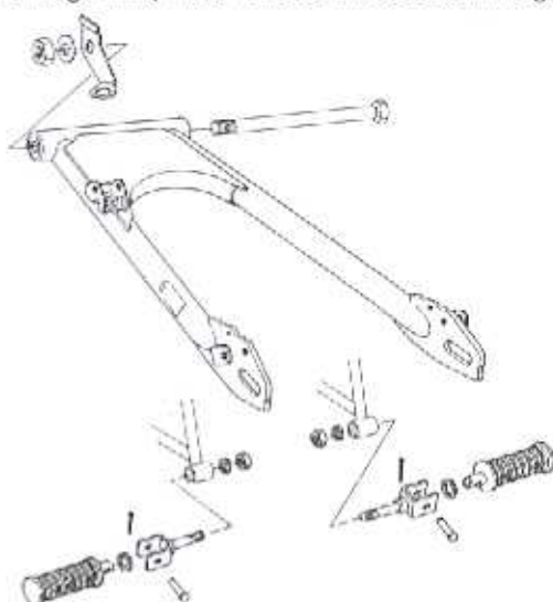
20-1. Footrests, Stands, Brake Pedal ... Page 43
