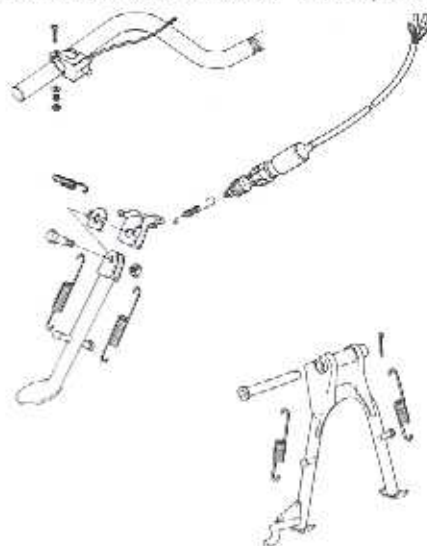
20-2. Stands (W. GERMANY TYPE).... Page 47
