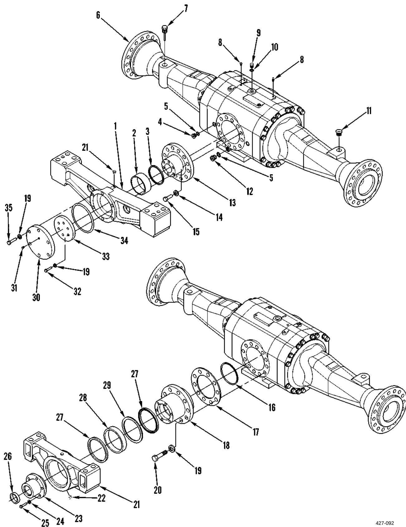
Figure 78. Rear Axle Assembly
