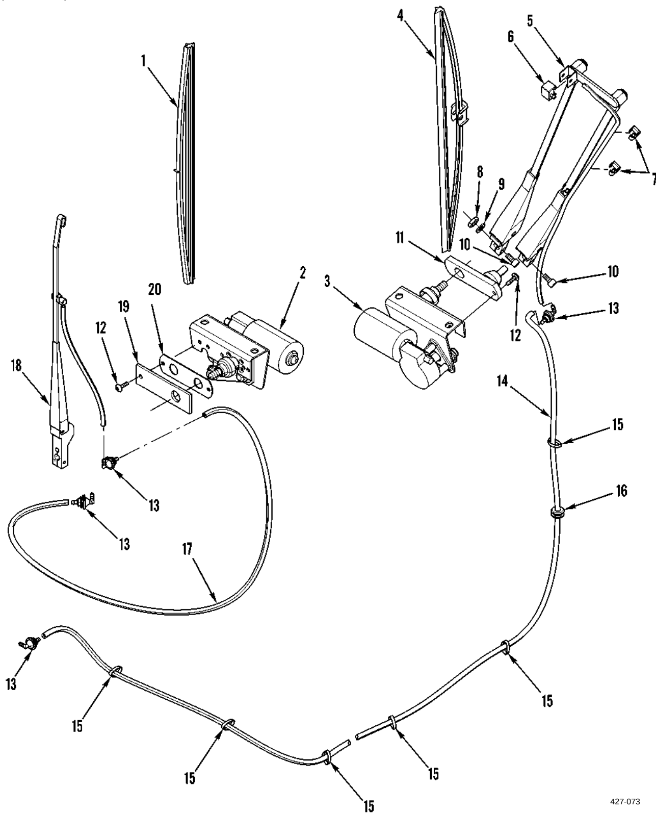
Figure 116. Windshield Wiper and Related Parts
