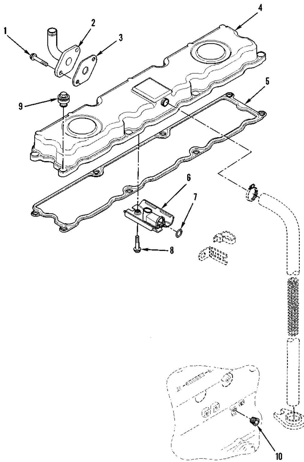
Figure 7. Valve Cover
