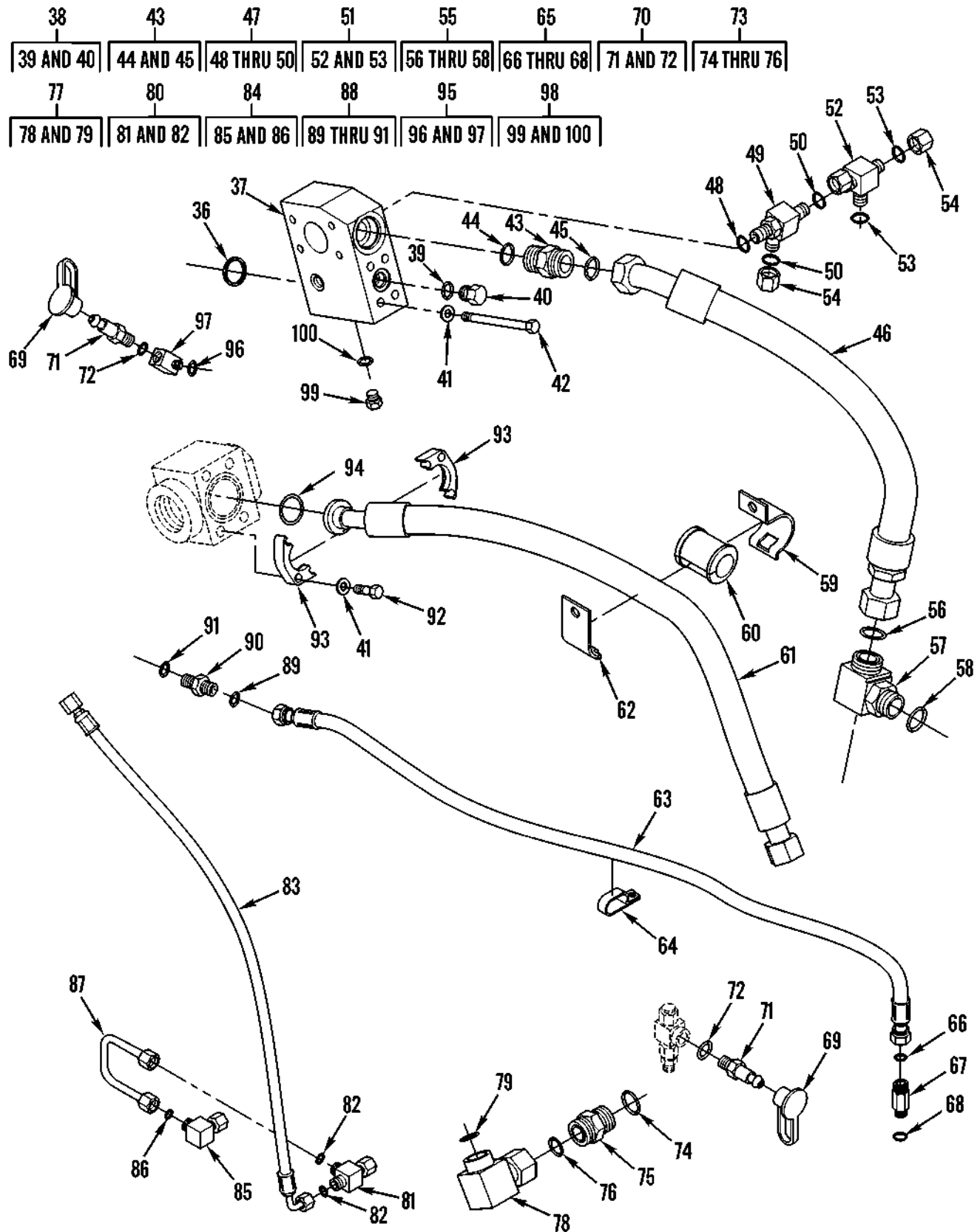
Figure 146. Hydraulic Oil Lines (Sheet 2 of 2)
