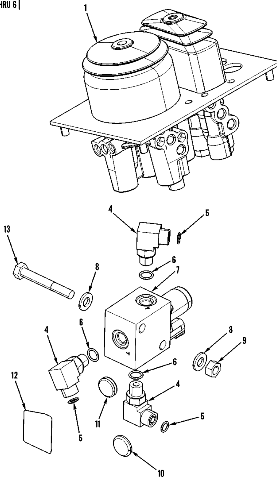
Figure 128. Pilot Operated Hydraulic Control Valve and Lockout Valve
