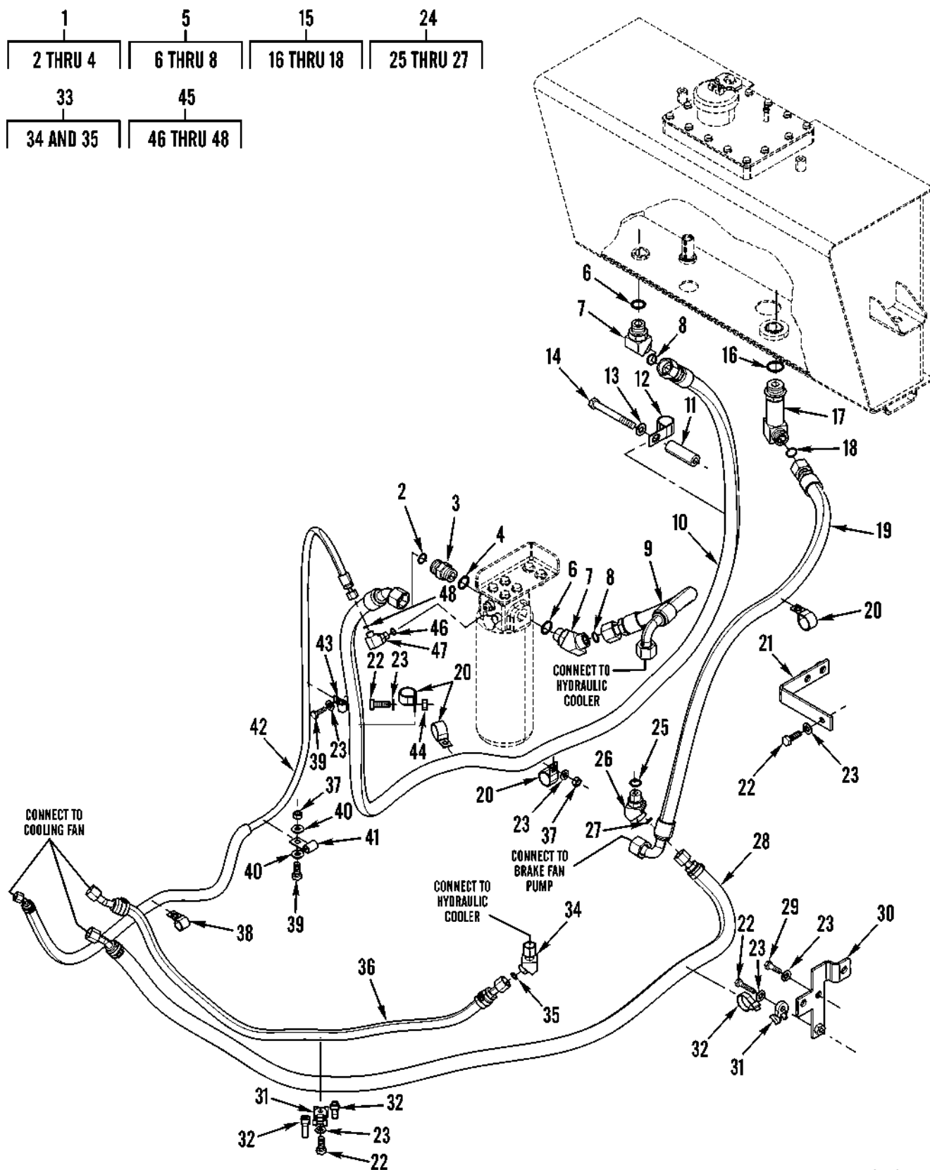
Figure 149. Fan Supply Lines (Standard)
