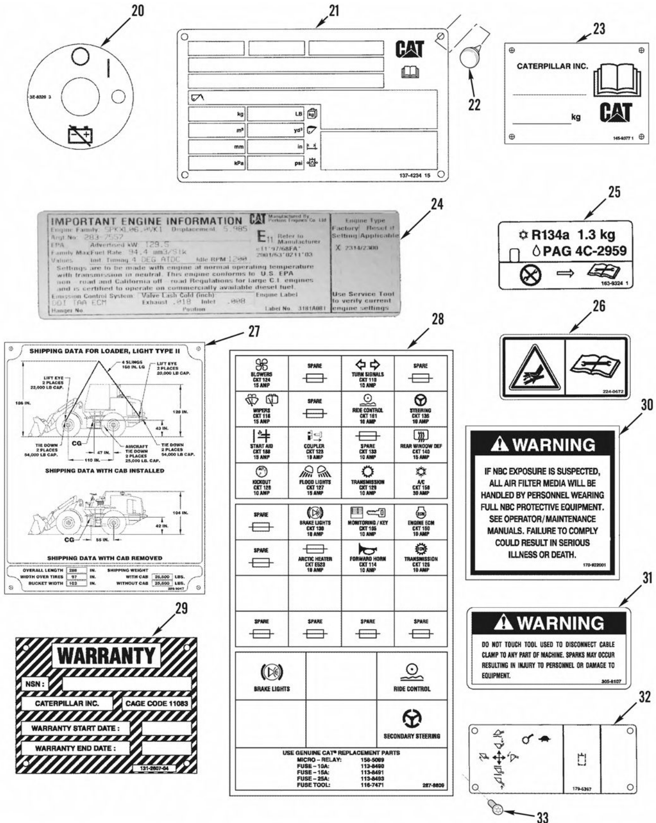
Figure 123. Data Plates and Instruction Holders (Sheet 2 of 2)
