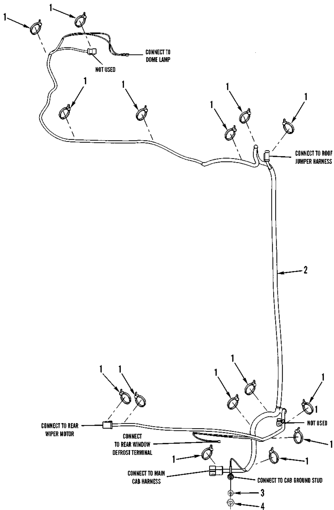
Figure 61. Cab Wiring
