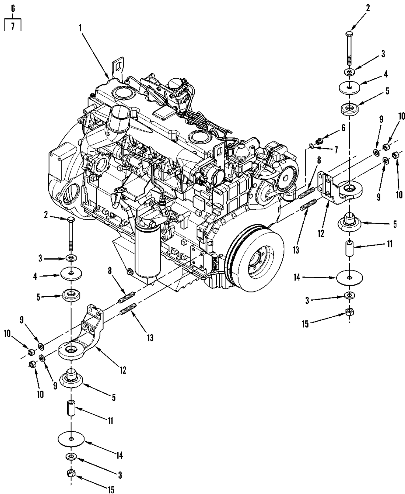
Figure 1. Engine and Engine Mounting
