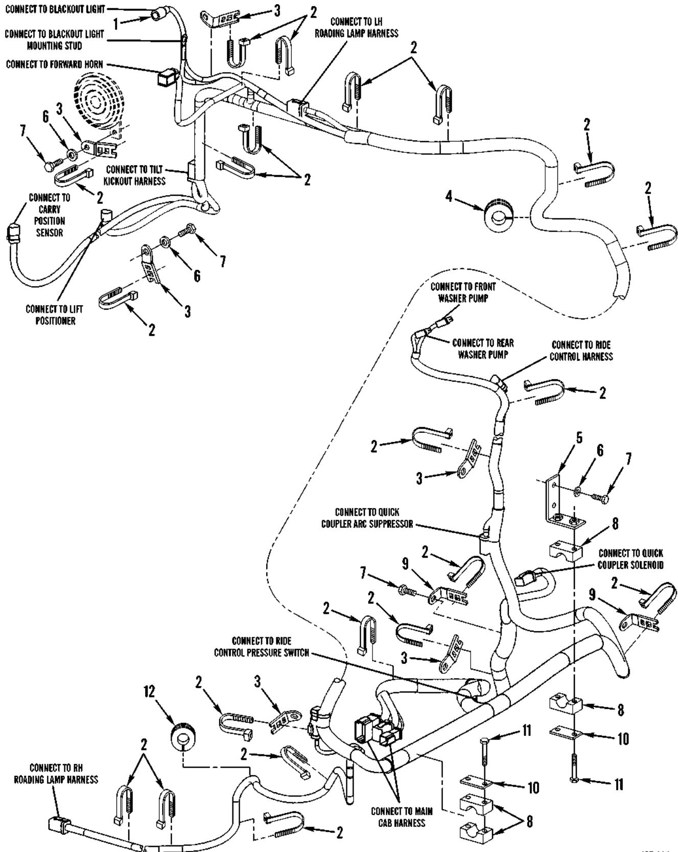
Figure 64. Front Wiring Harness
