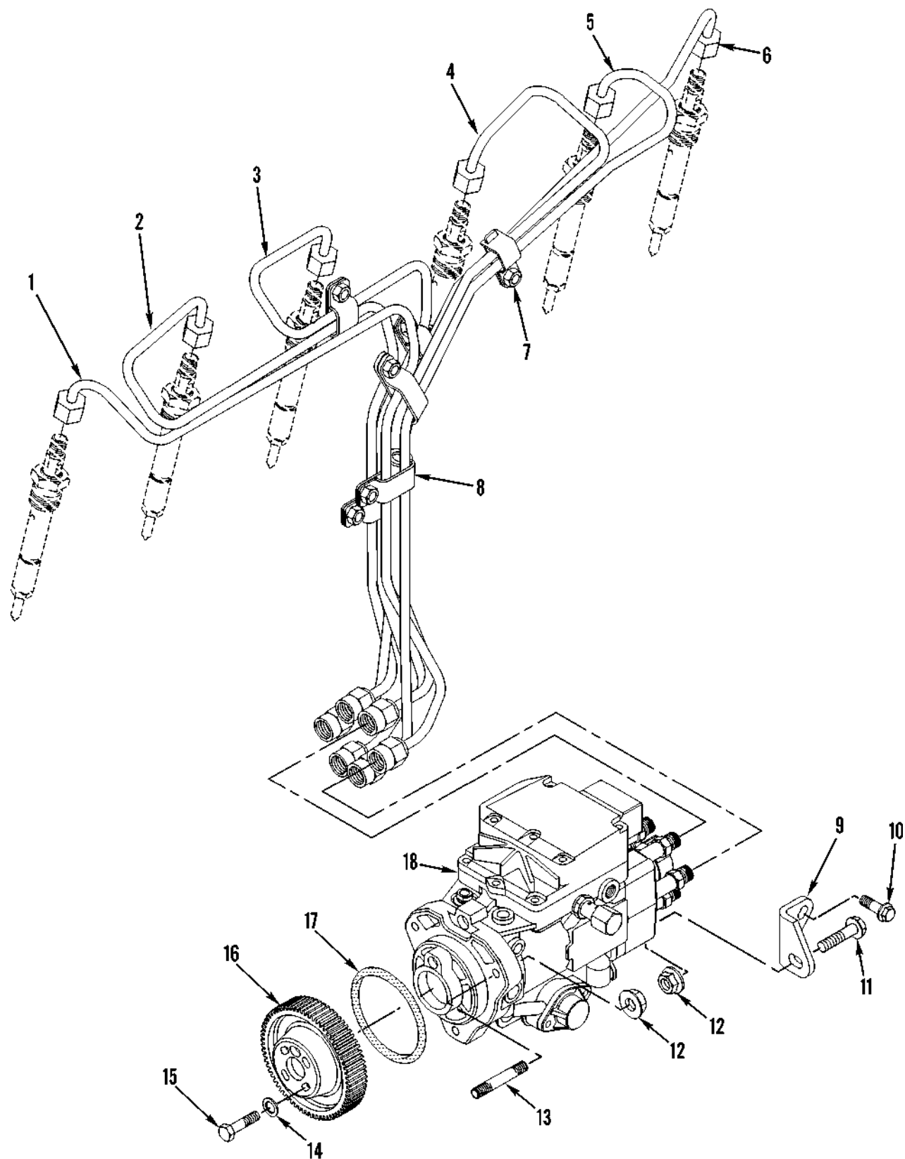
Figure 19. Fuel Injection Pump, Lines, and Related Parts
