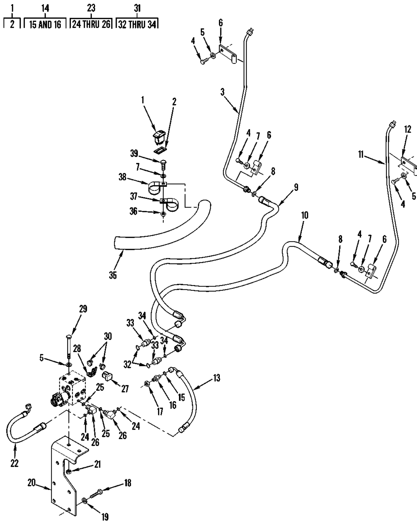
Figure 147. Coupler Lines (Sheet 1 of 2)
