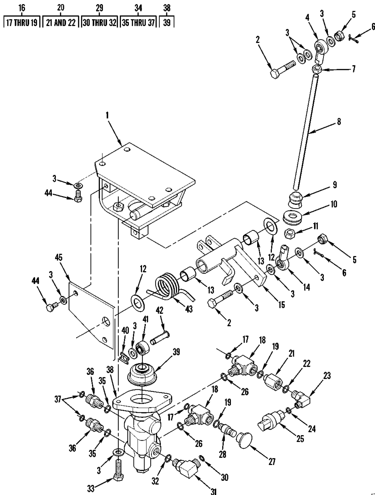
Figure 81. Service Brake Control and Related Parts
