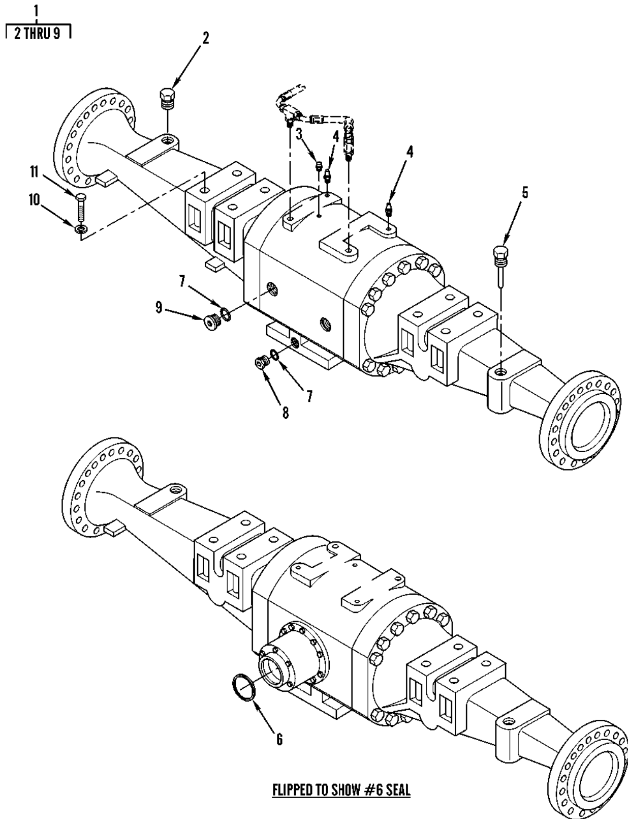
Figure 77. Front Axle Assembly
