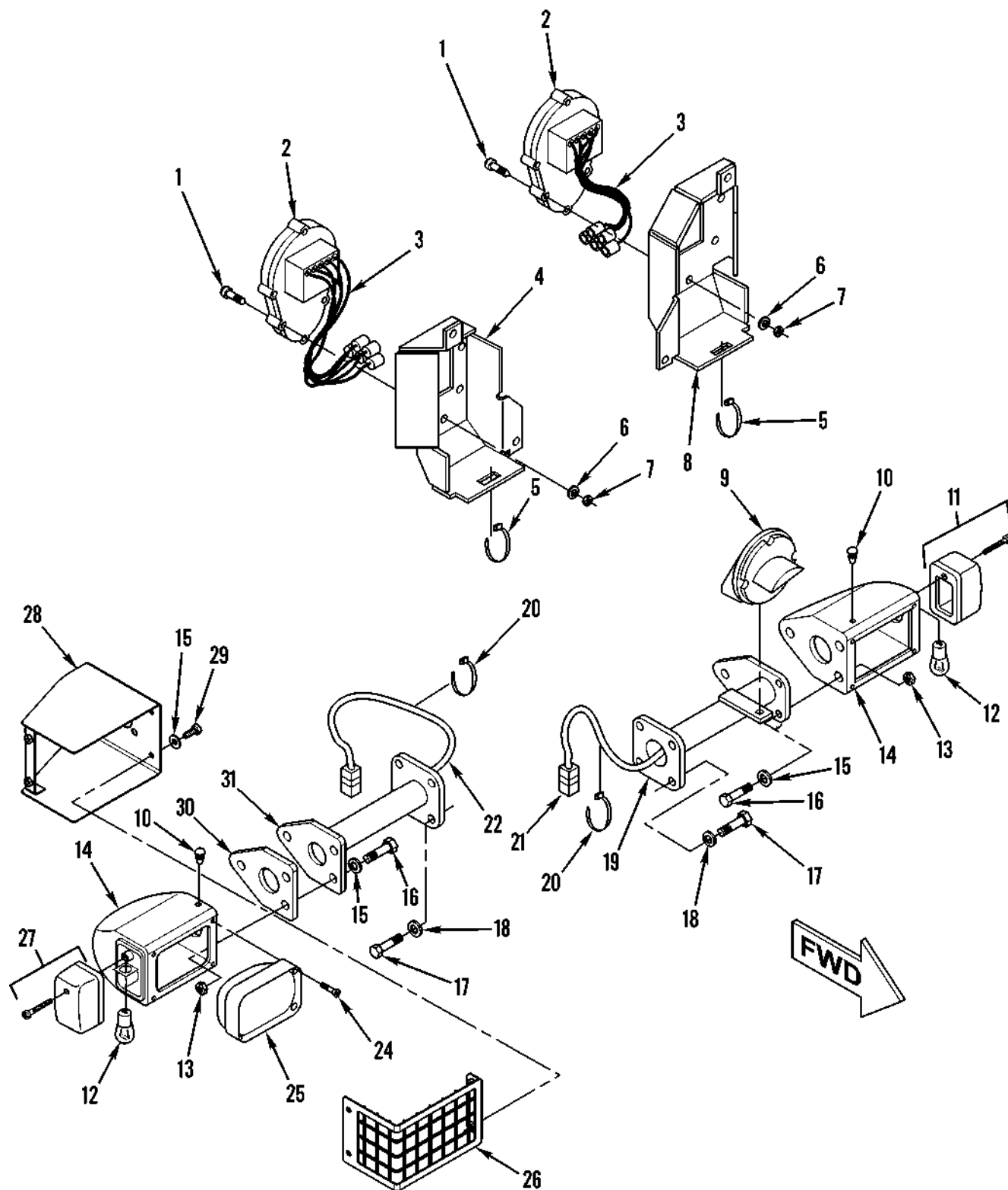
Figure 48. Lights (Service, Rear, Blackout Drive, and Turn Signal)
