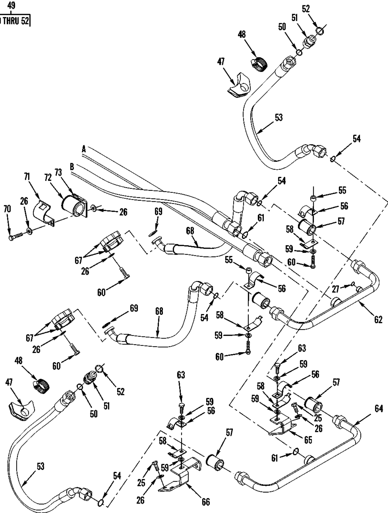
Figure 140. Lift Cylinder Lines (Sheet 2 of 2)
