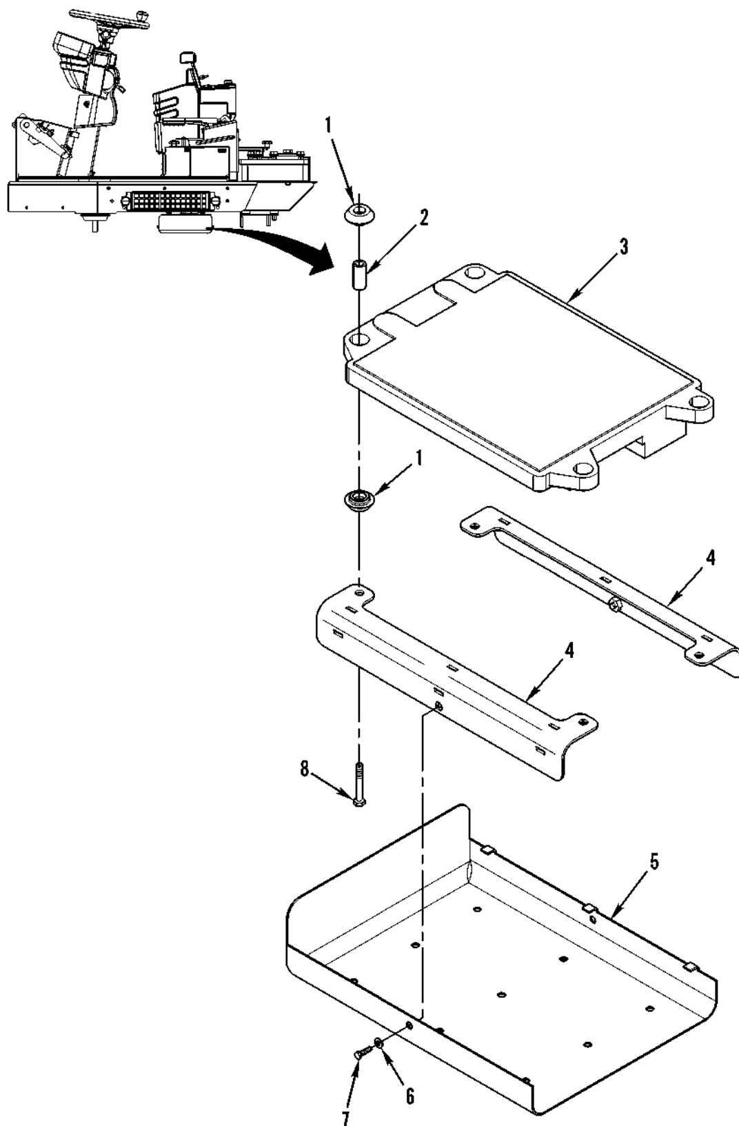
Figure 44. Machine (Transmission) ECM
