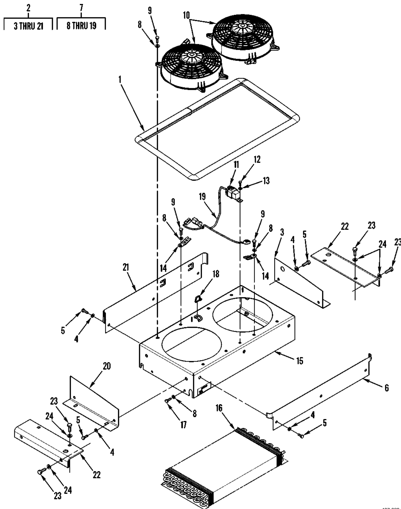
Figure 166. A/C Condenser and Mounting
