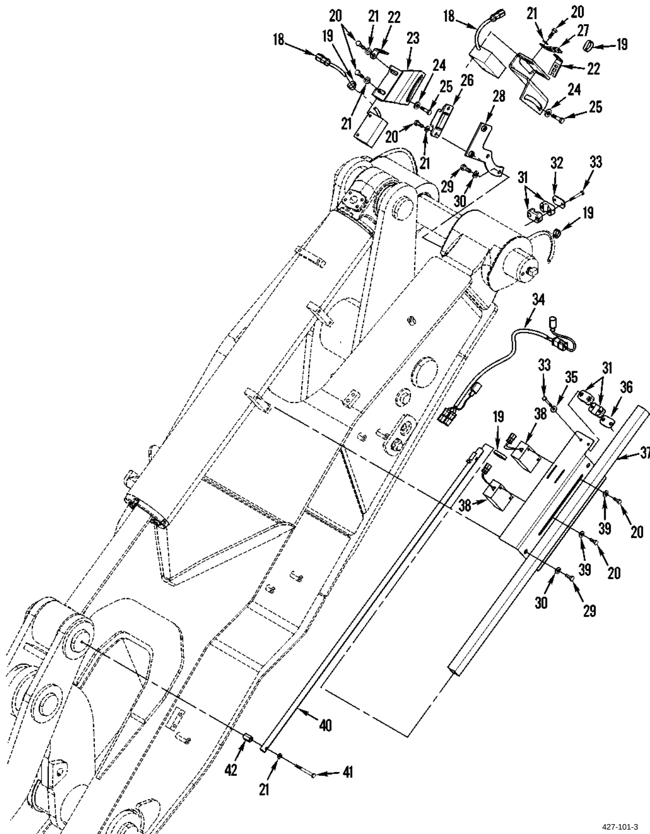
Figure 51. Electrical Sensors, Switches, and Related Parts (Sheet 3 of 4)
