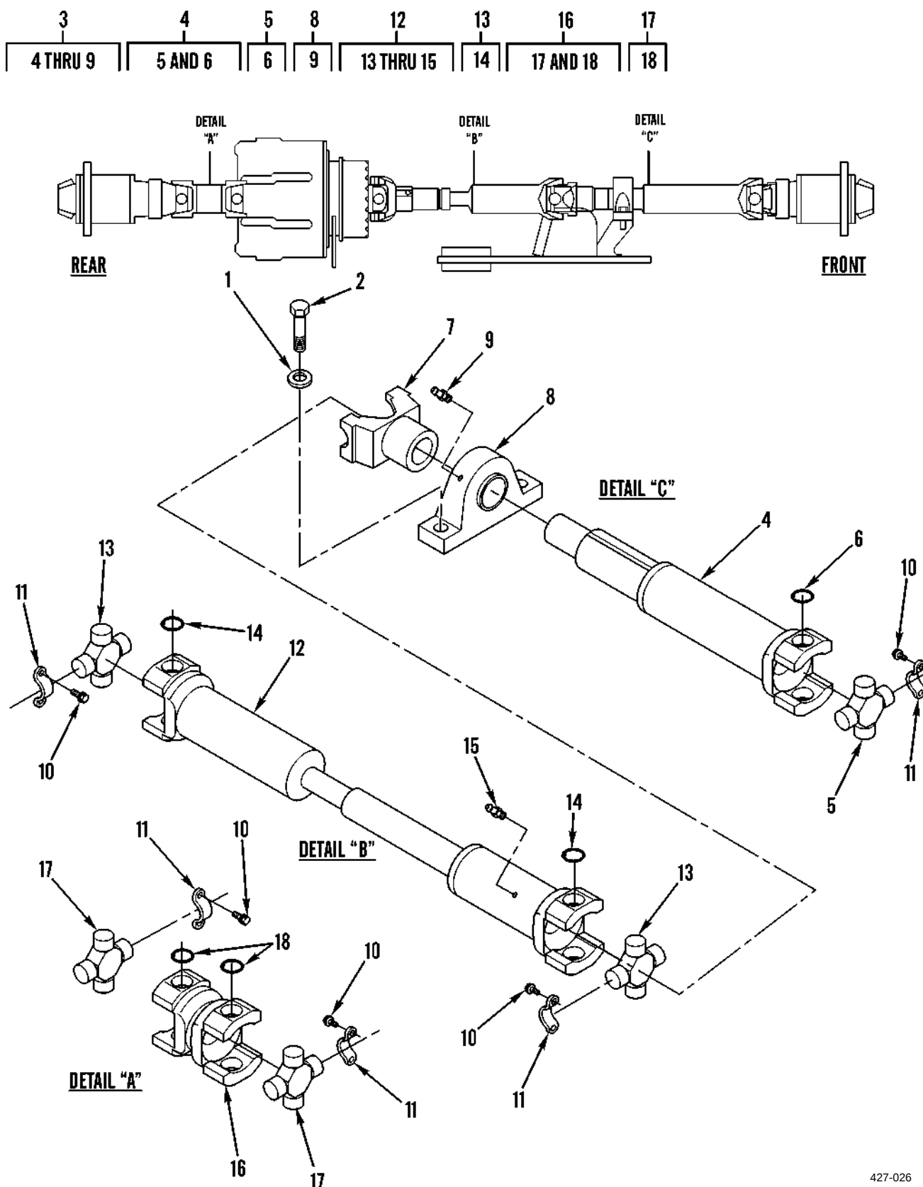
Figure 76. Drive Shafts and Related Parts
