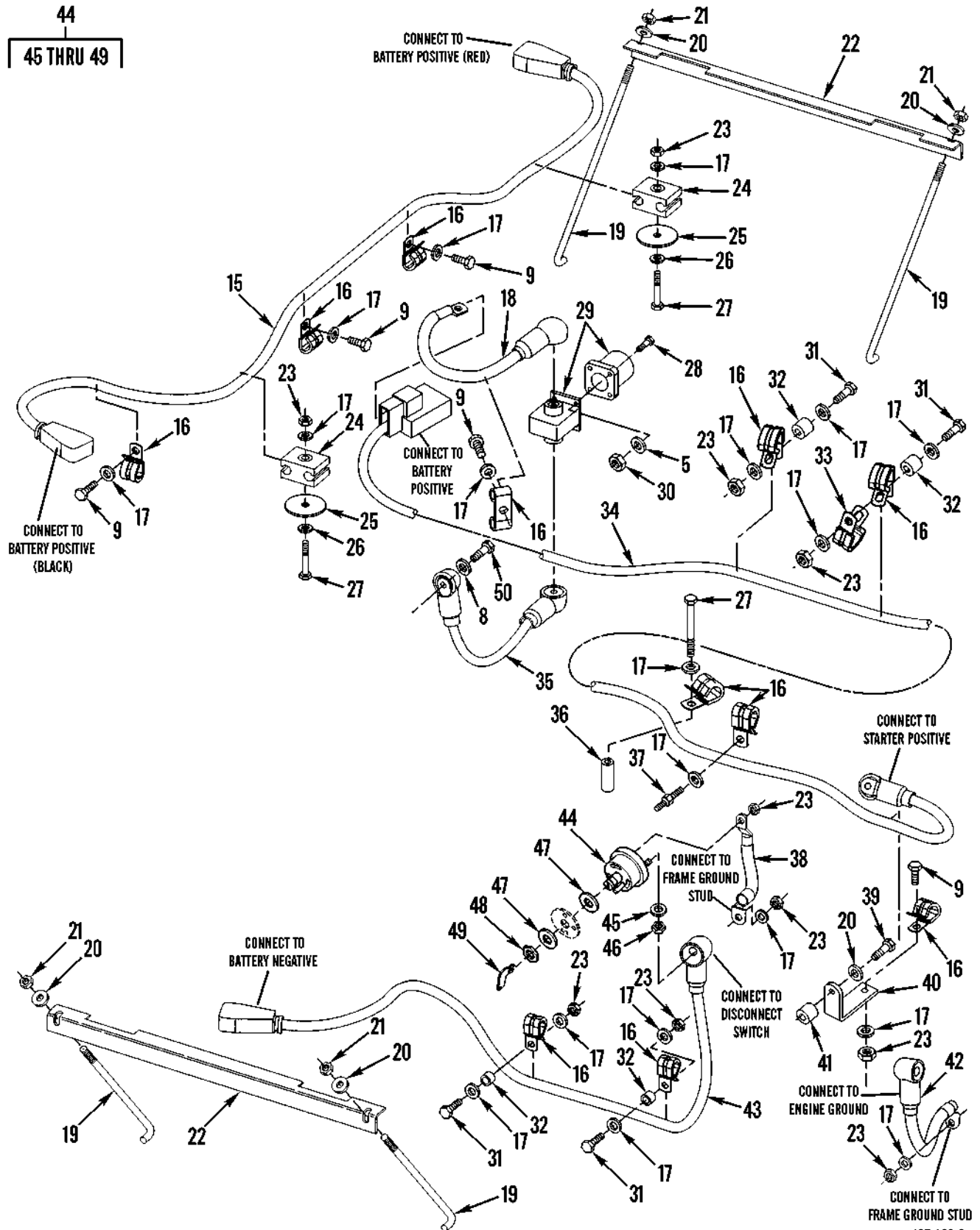
Figure 56. Battery Box and Wiring (Standard) (Sheet 2 of 2)
