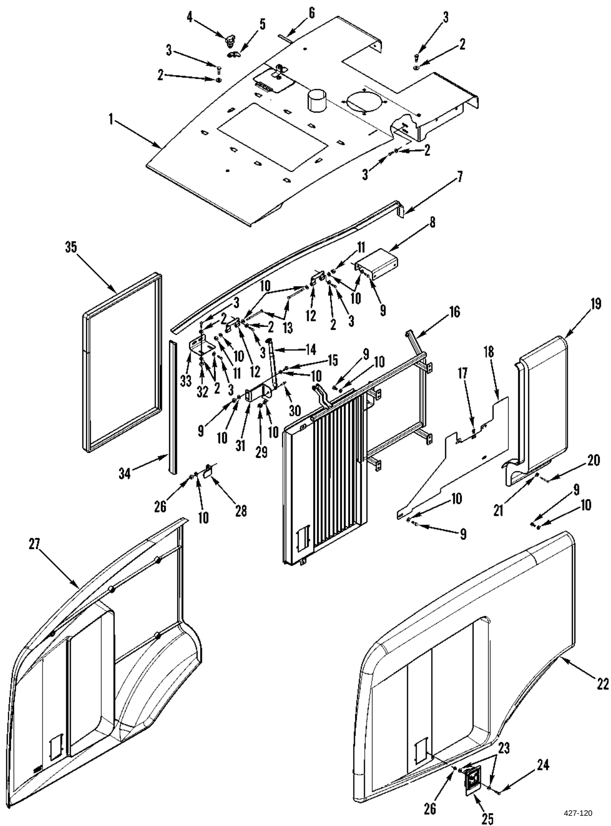
Figure 108. Hood, Side Covers, and Related Parts
