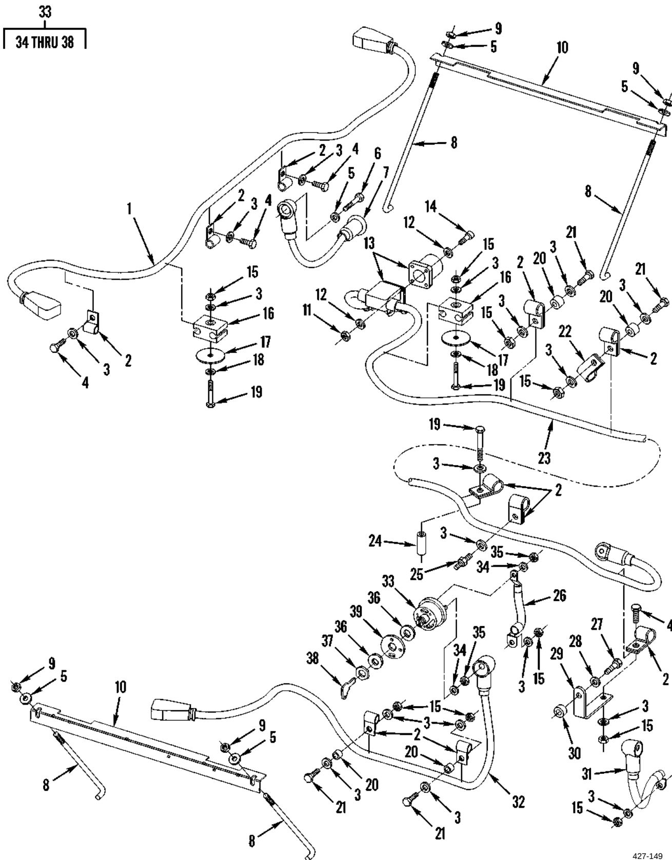
Figure 159. Battery Wiring (Arctic)
