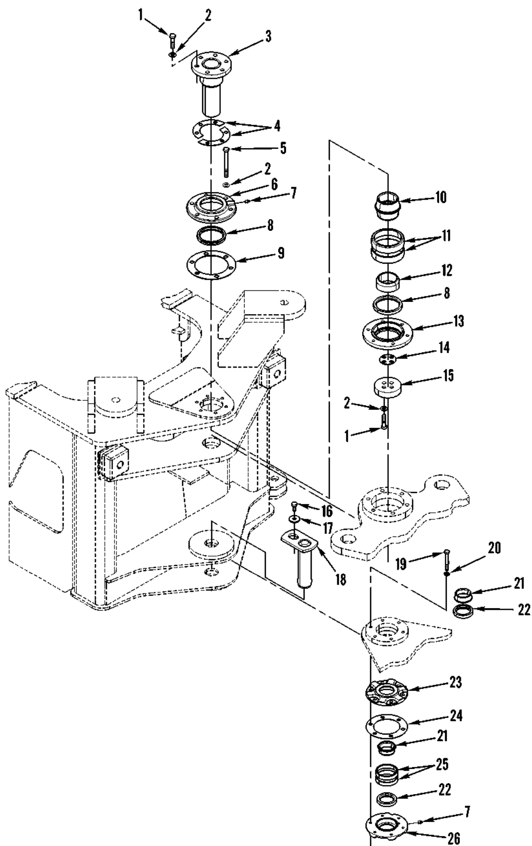
Figure 99. Articulating Hitch and Related Parts
