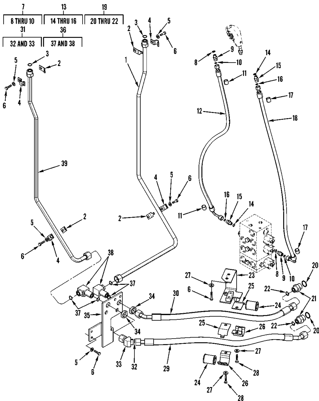
Figure 137. Hydraulic Lines
