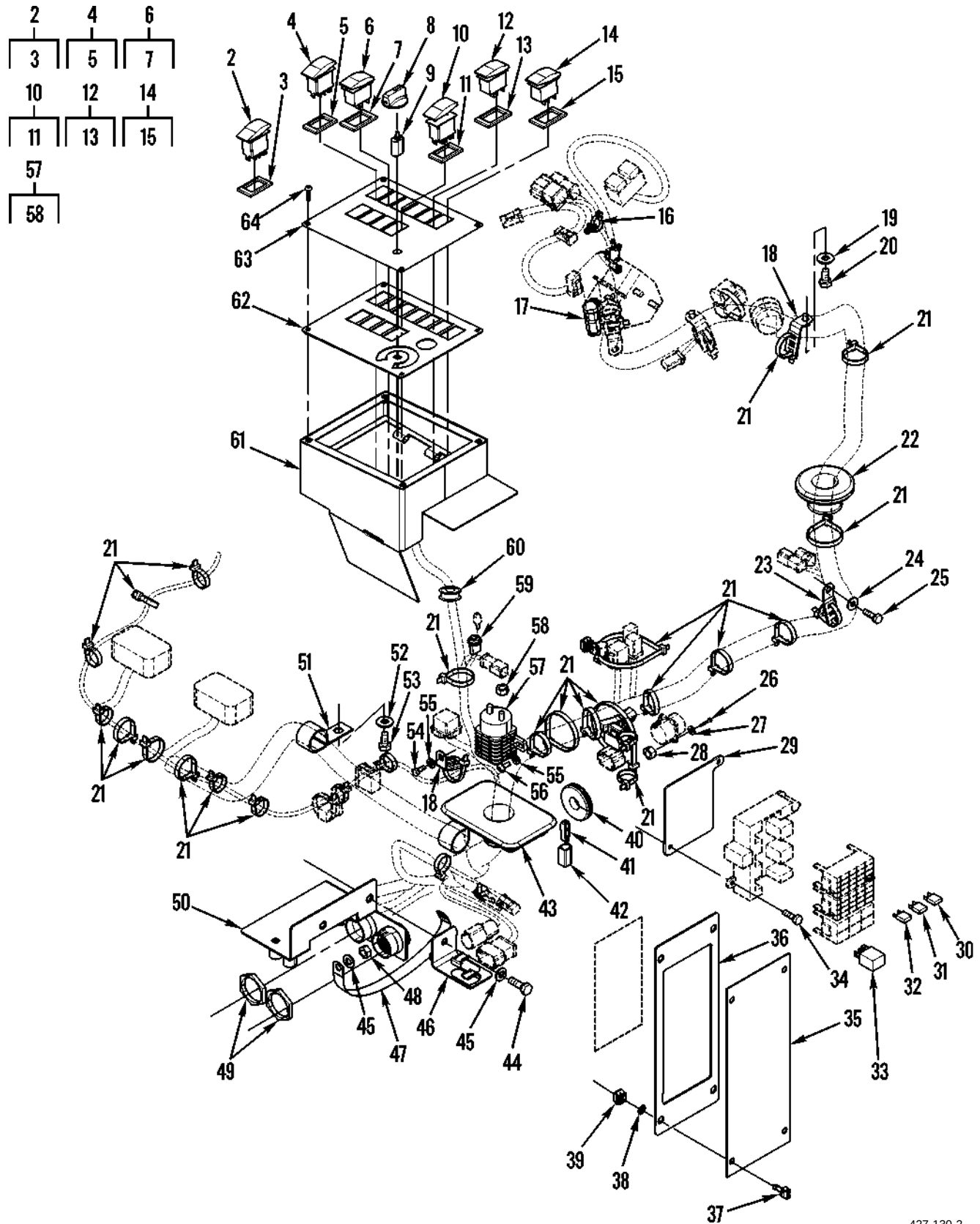
Figure 43. Cab Wiring Harness and Control Switches (Right Side) (Sheet 2 of 2)
