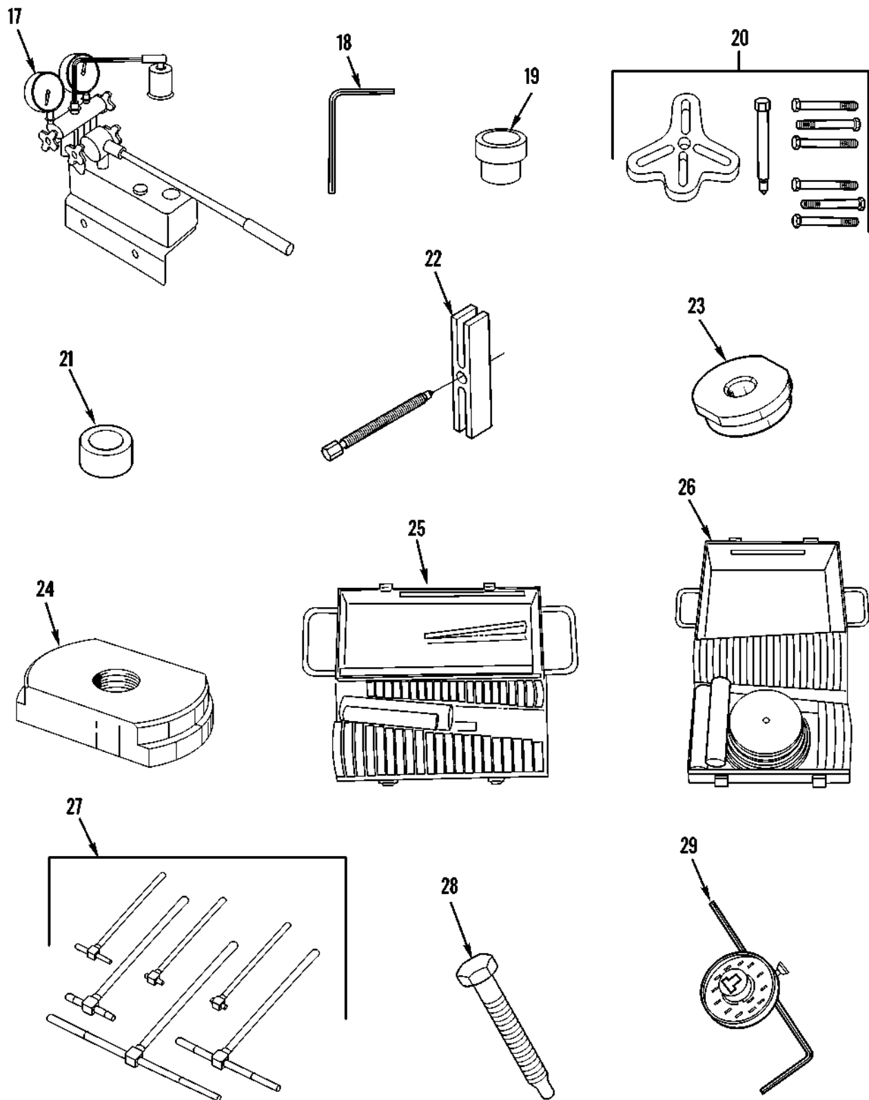
Figure 175. Direct Support Special Tools (Sheet 2 of 3)
