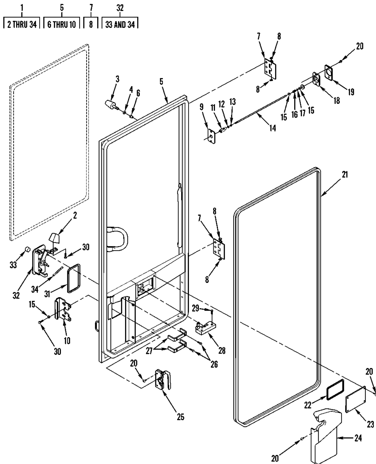
Figure 105. Door Assembly (Right Side)
