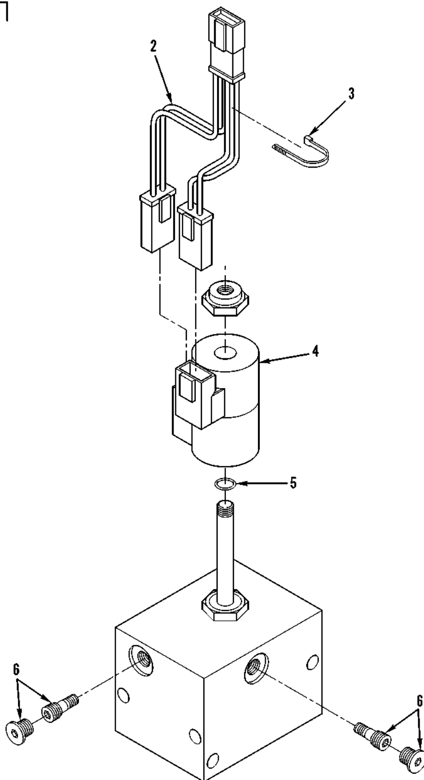
Figure 130. Coupler Valve
