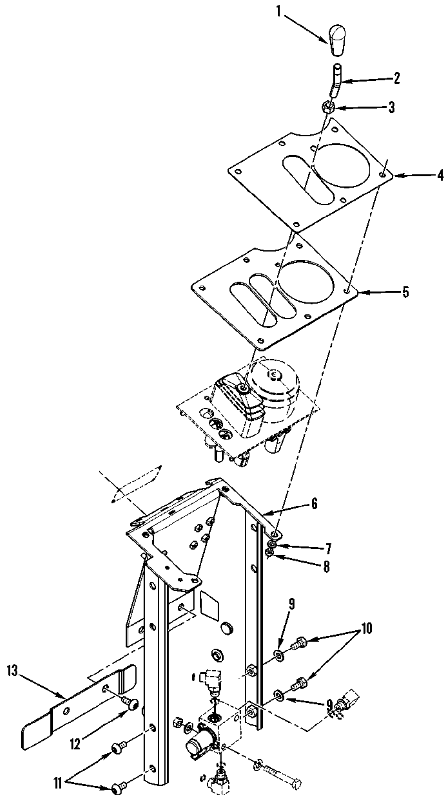
Figure 131. Pilot Operated Hydraulic Controls and Related Parts
