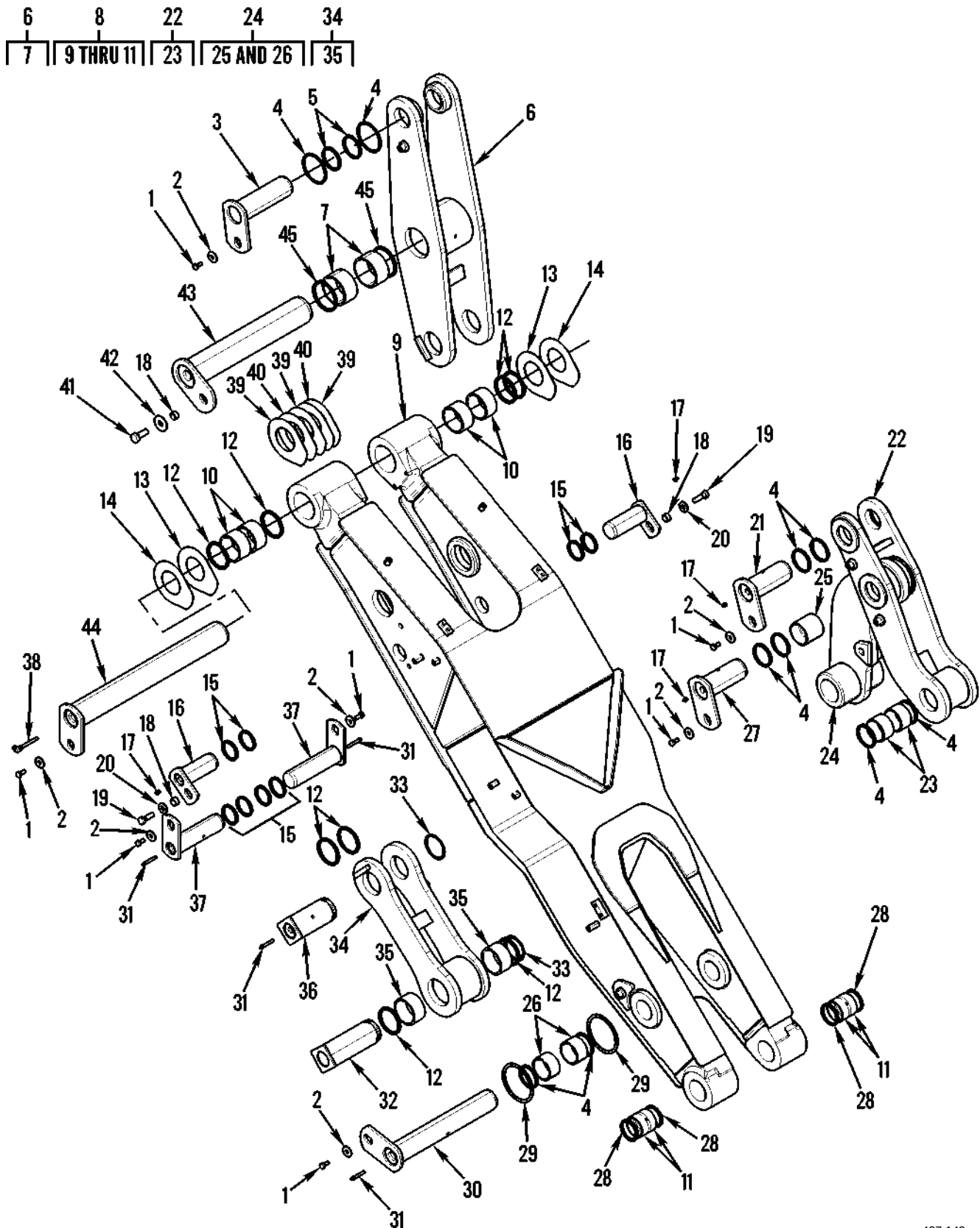
Figure 172. Implement Control
