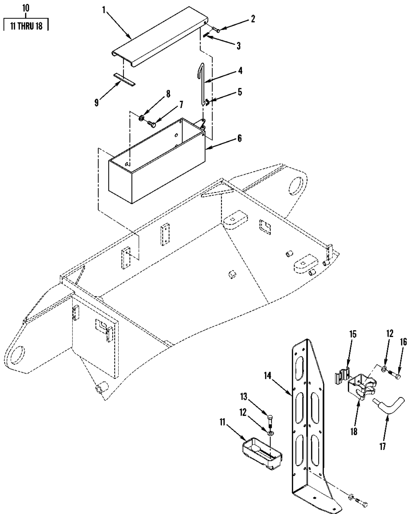
Figure 114. Toolbox and Rifle Rack
