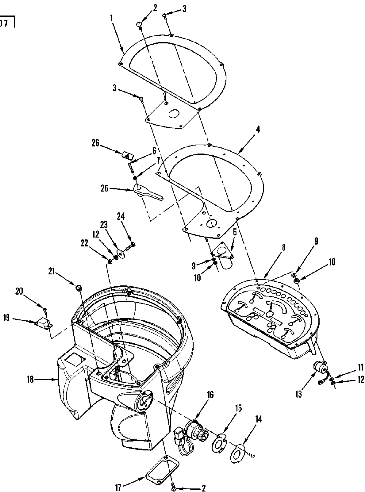
Figure 41. Control Switches and Panel
