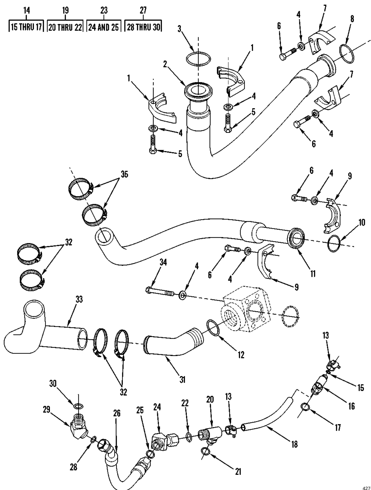
Figure 146. Hydraulic Oil Lines (Sheet 1 of 2)
