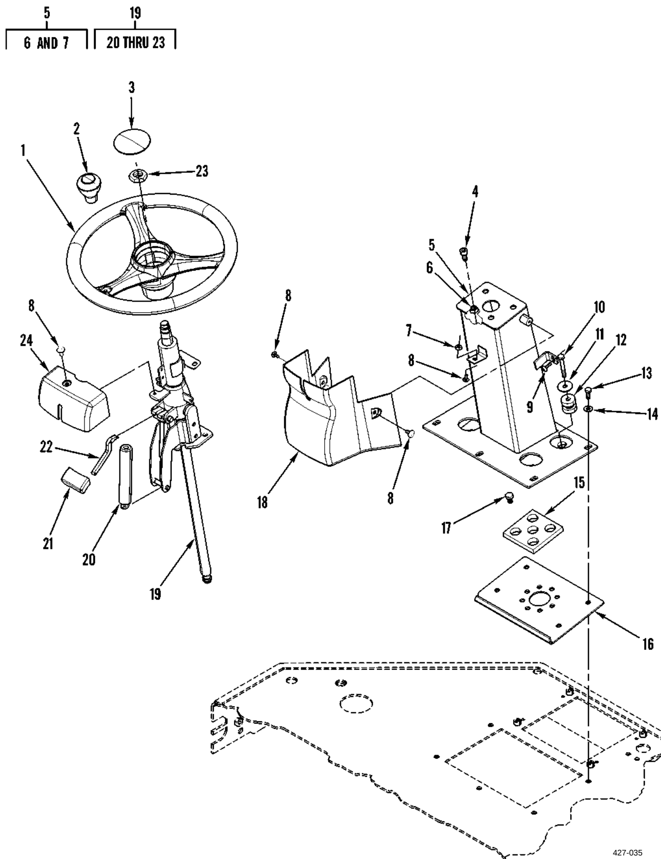
Figure 86. Steering Wheel and Related Parts
