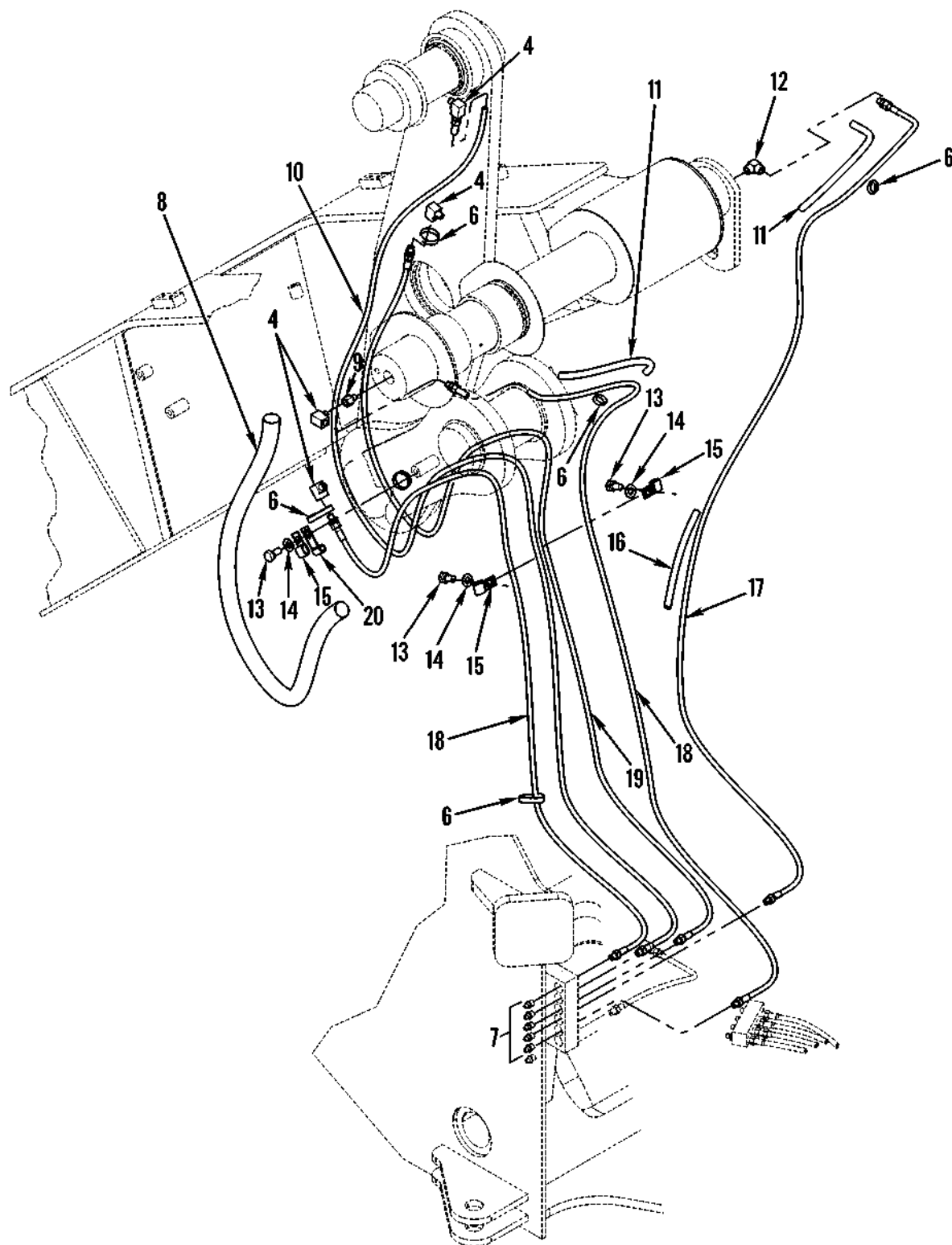
Figure 95. Remote Lubrication Lines (Sheet 2 of 2)
