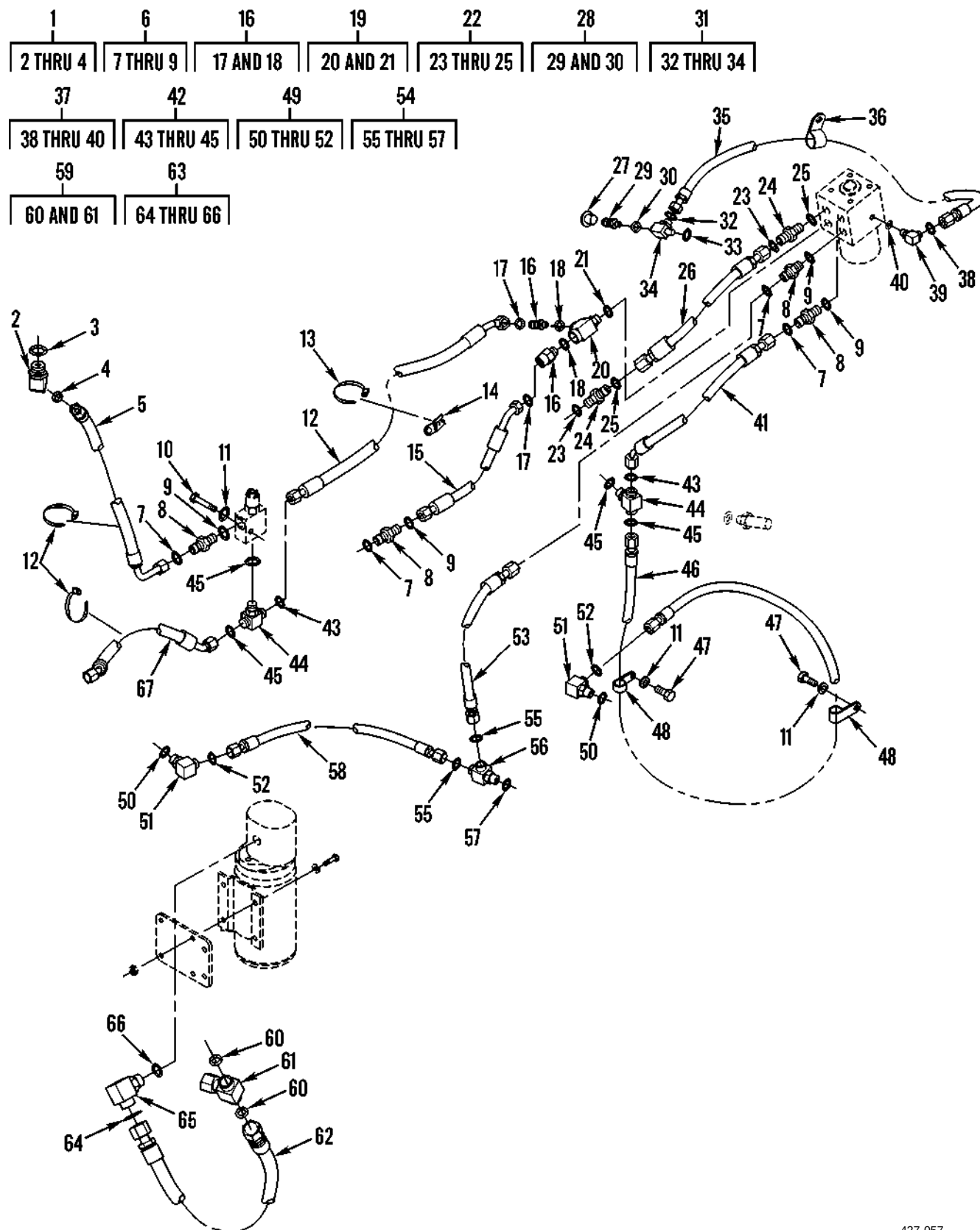
Figure 89. Steering Lines
