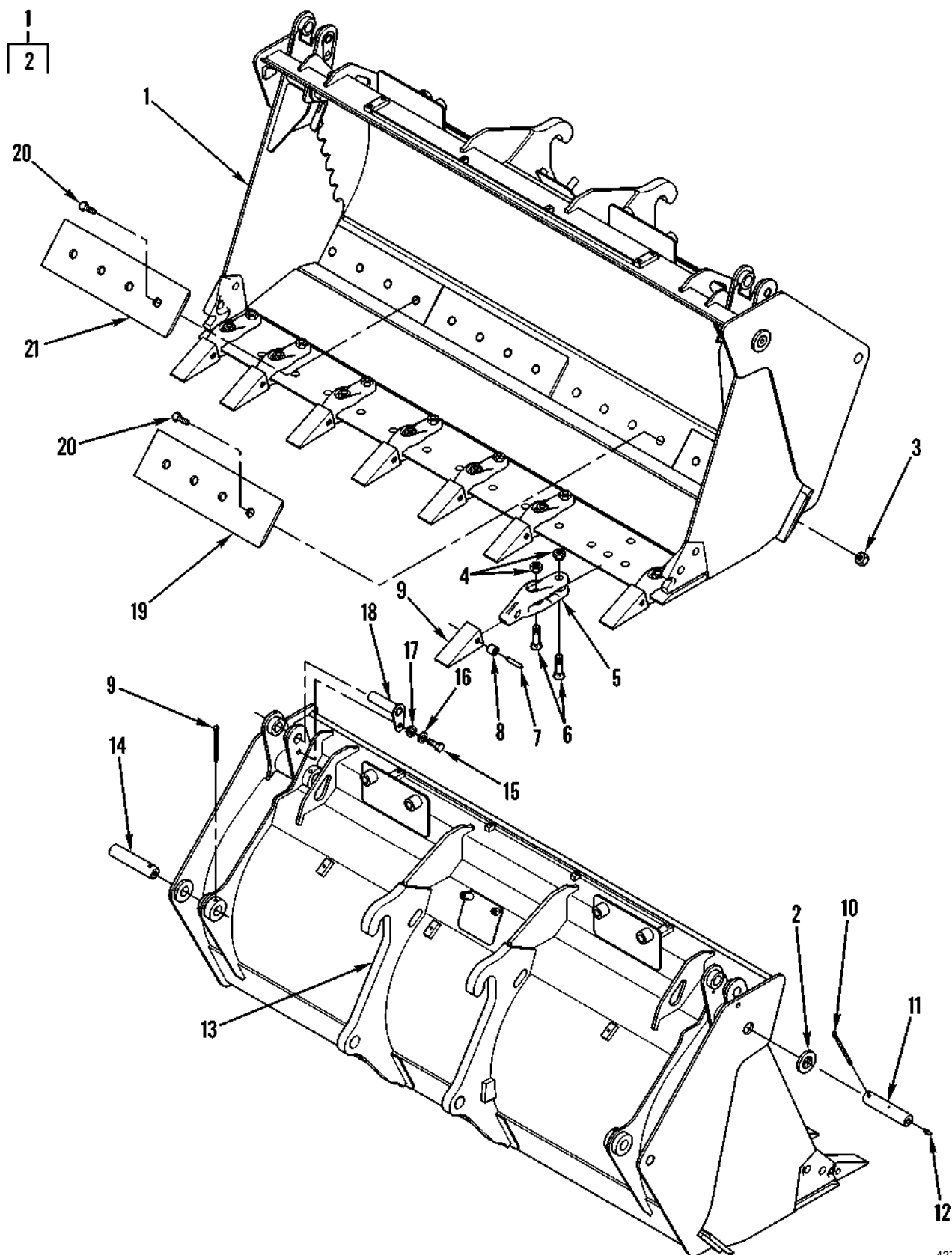
Figure 173. Bucket and Related Parts
