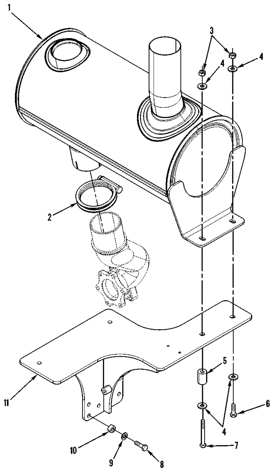
Figure 31. Muffler
