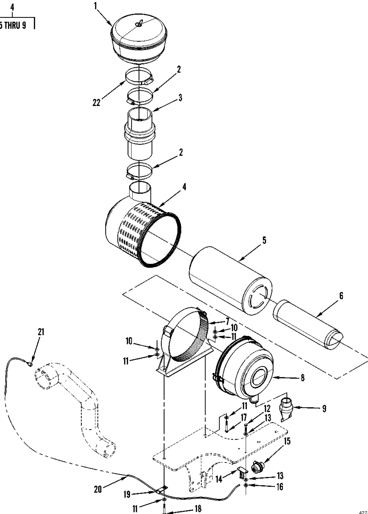
Figure 20. Air Cleaner, Housing, Precleaner, and Restriction Indicator
