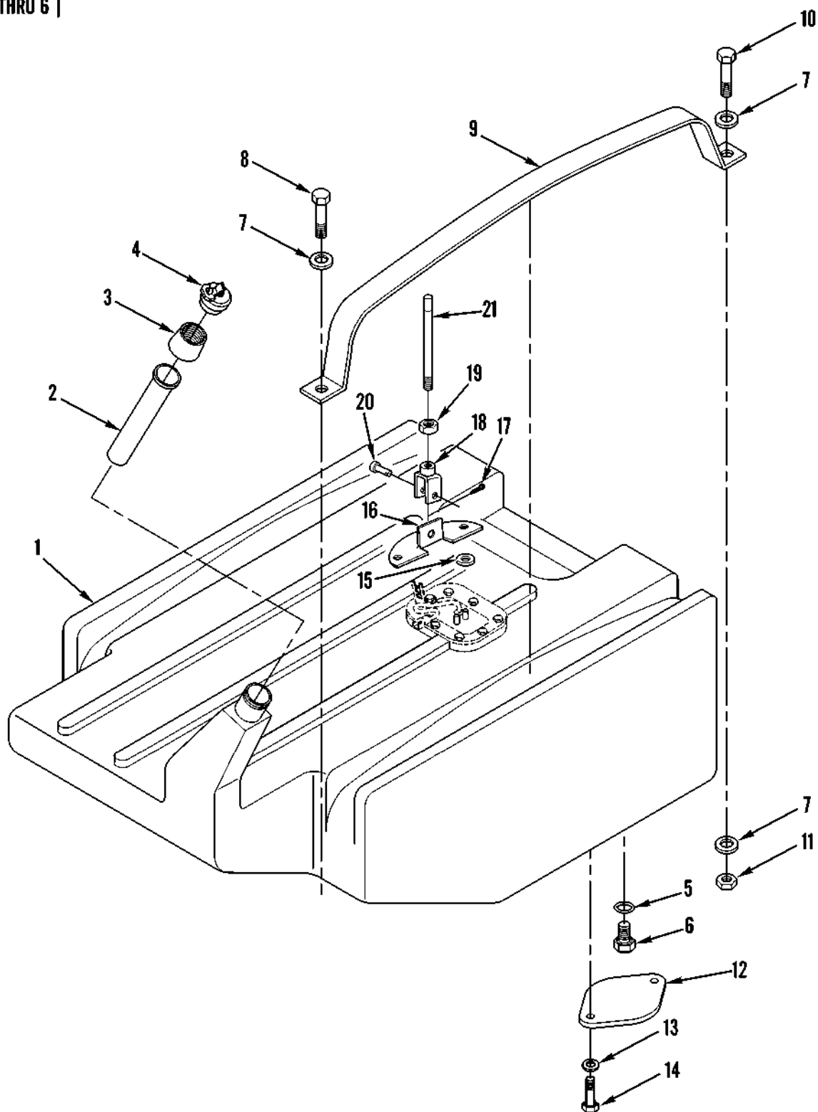
Figure 25. Fuel Tank, Standard
