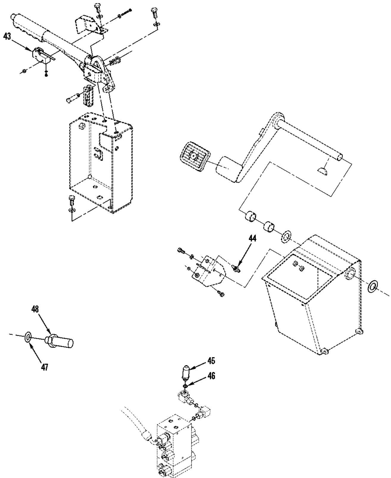
Figure 51. Electrical Sensors, Switches, and Related Parts (Sheet 4 of 4)
