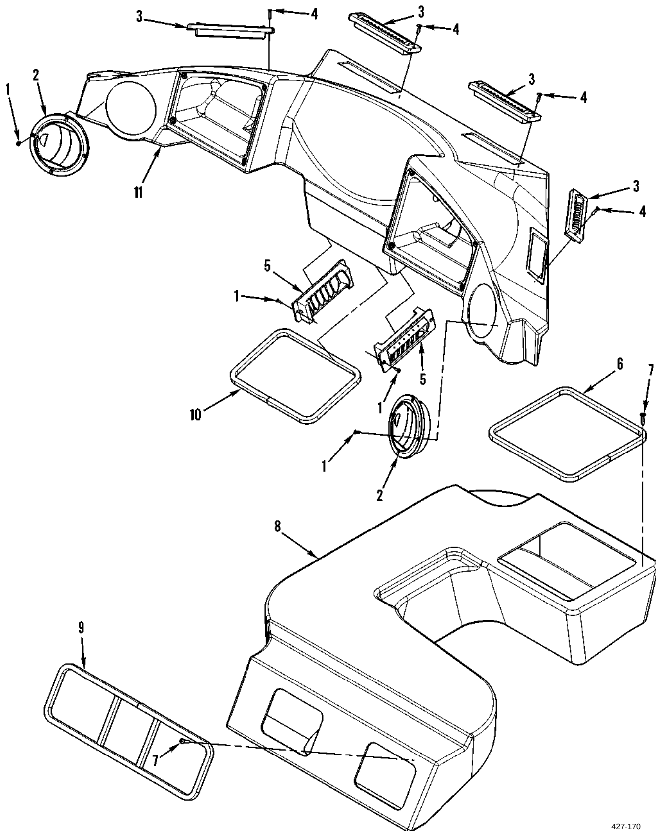
Figure 121. Air Duct
