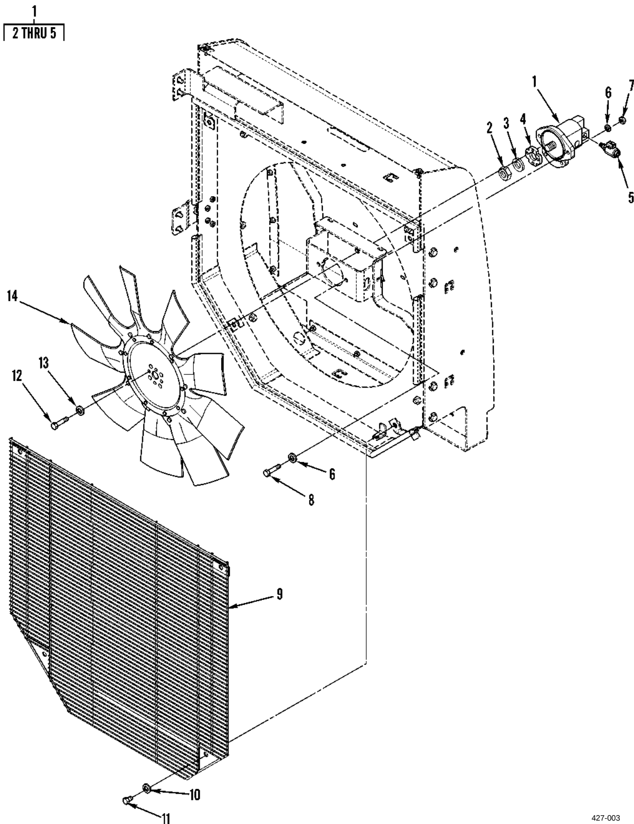
Figure 37. Hydraulic Fan, Motor, and Related Parts
