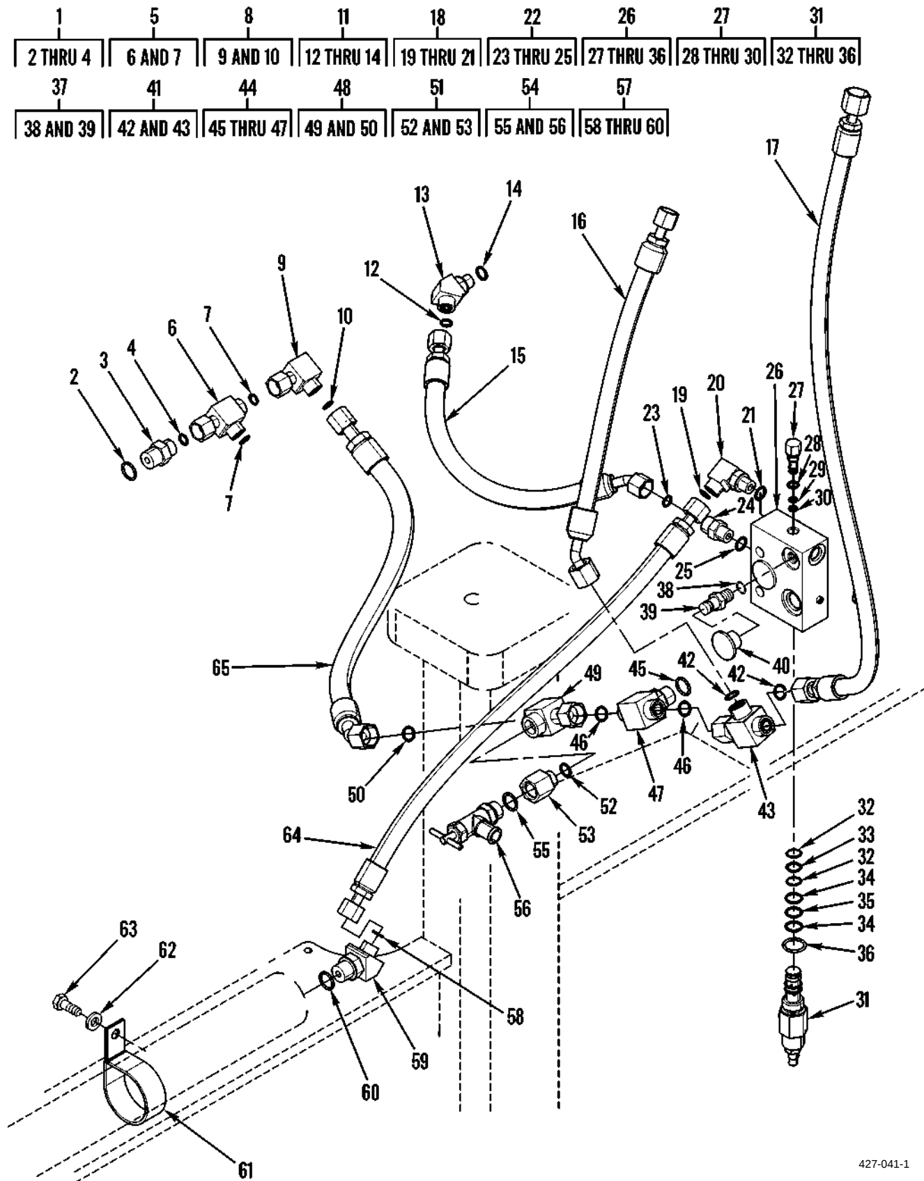
Figure 138. Pilot Lines (Hydraulic) (Sheet 1 of 2)
