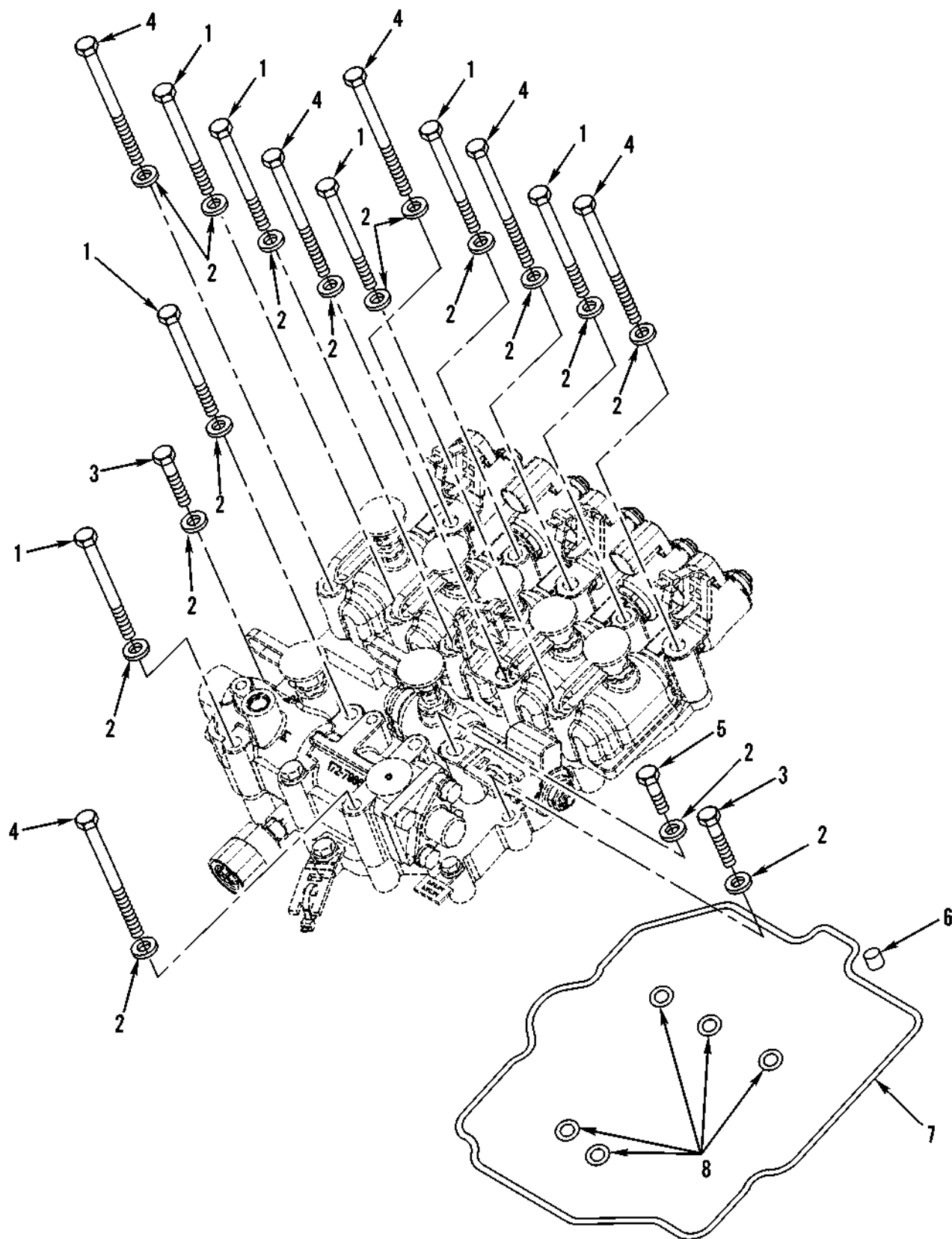
Figure 69. Transmission Control Valve and Related Parts (Sheet 1 of 2)
