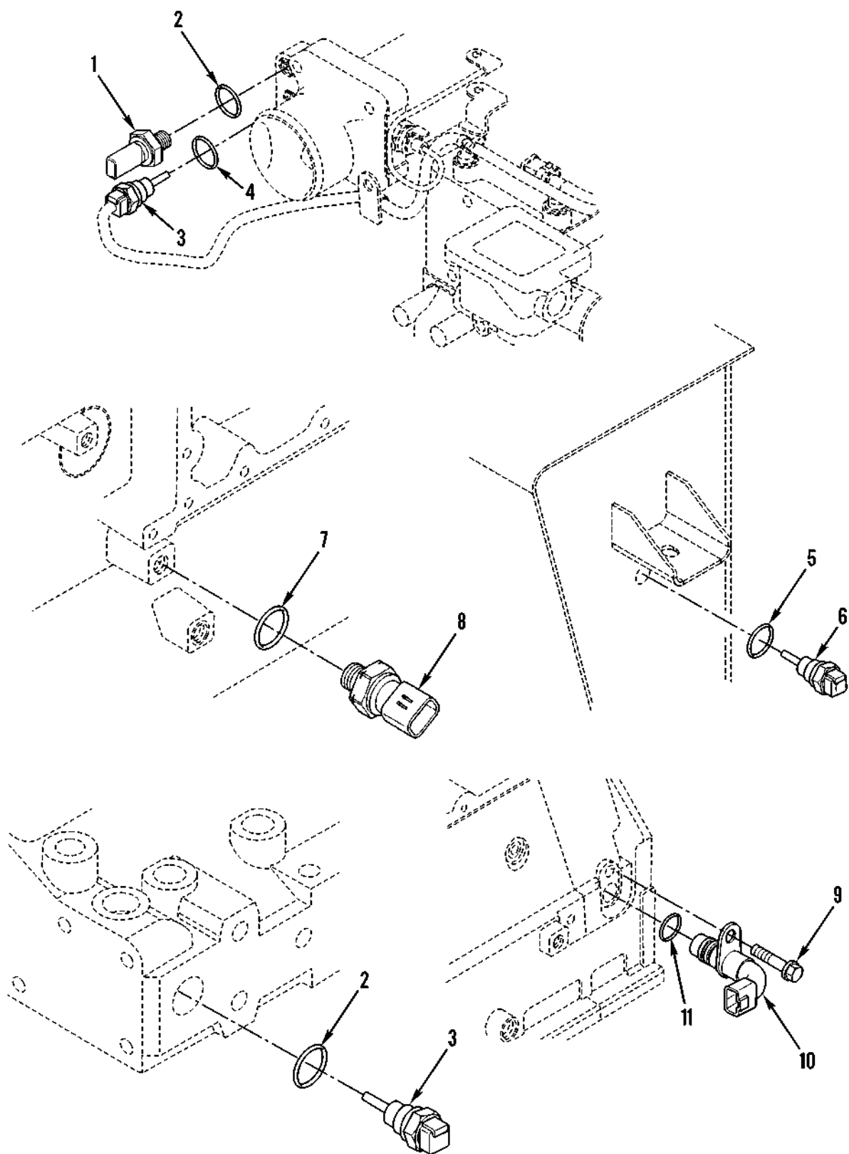
Figure 51. Electrical Sensors, Switches, and Related Parts (Sheet 1 of 4)
