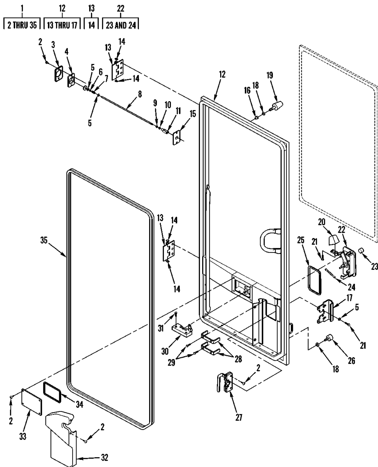
Figure 104. Door Assembly (Left Side)
