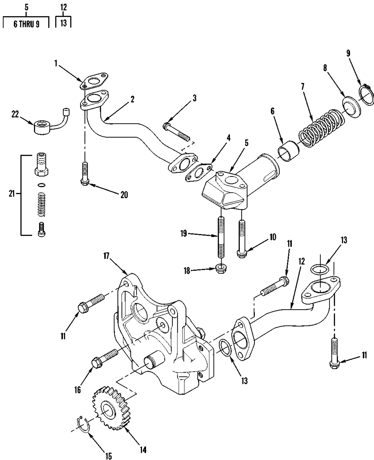
Figure 11. Engine Oil Pump, Bypass Valve, and Piston Cooling Jets
