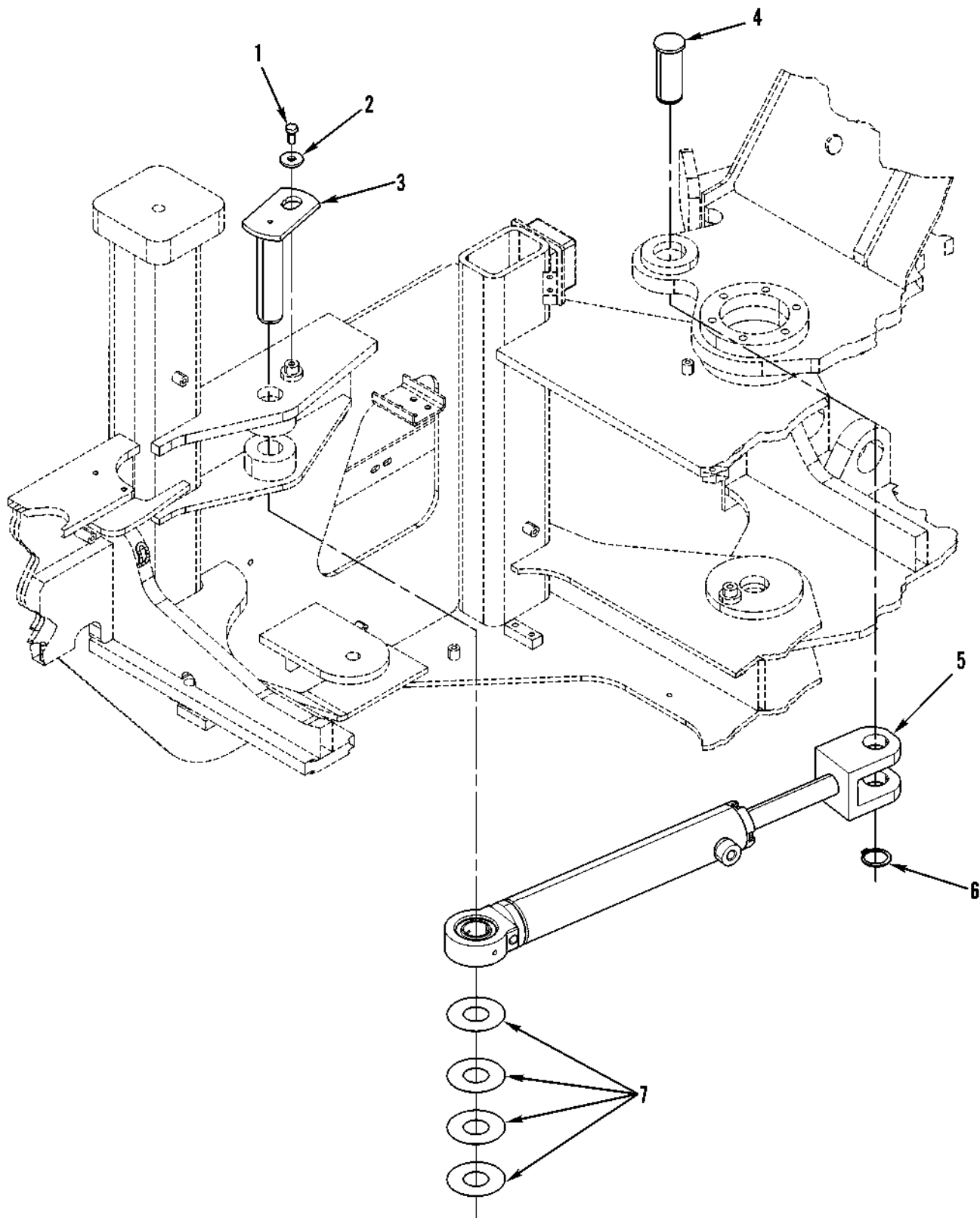
Figure 90. Steering Cylinder and Mounting
