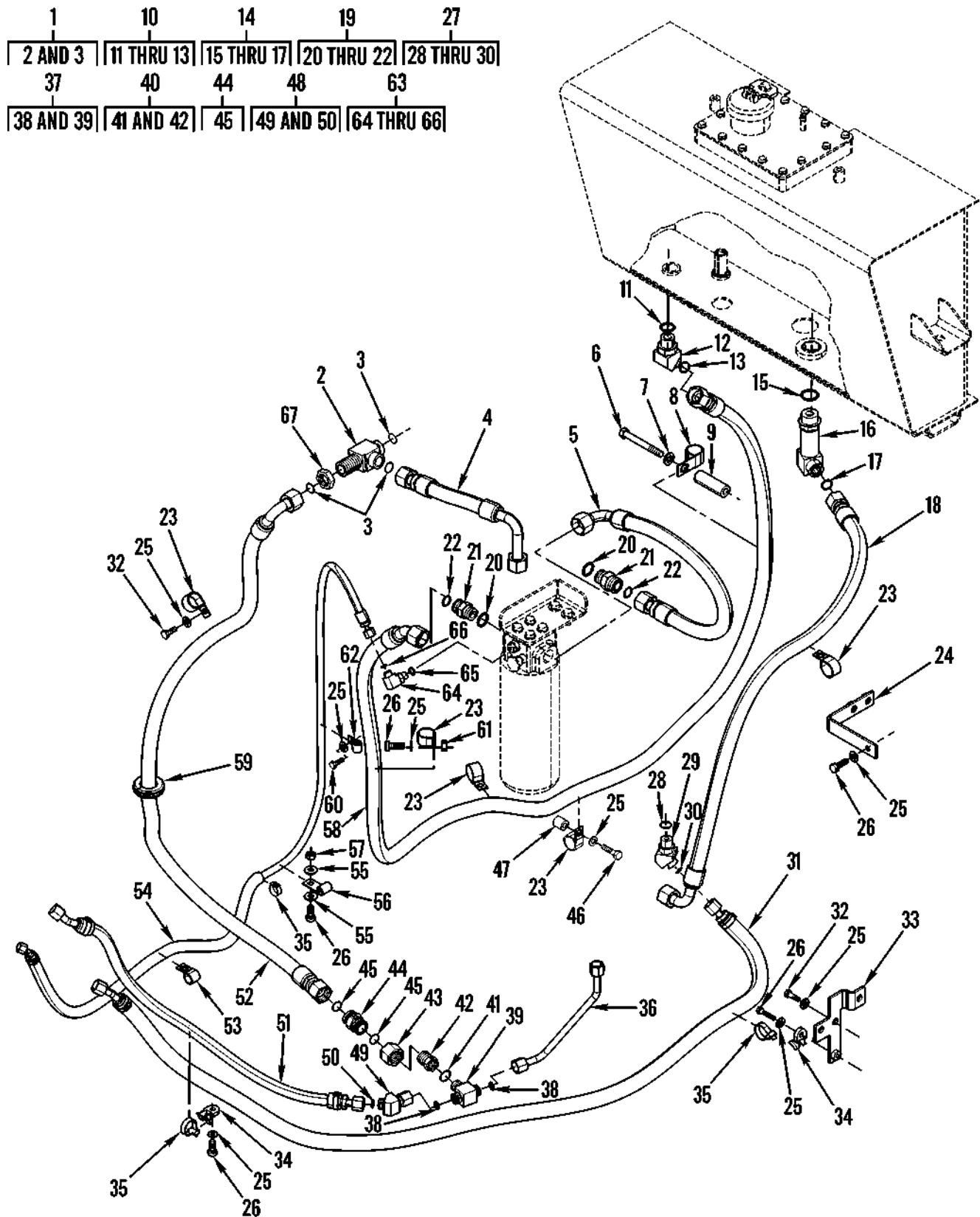
Figure 154. Fan Supply Lines (Arctic)
