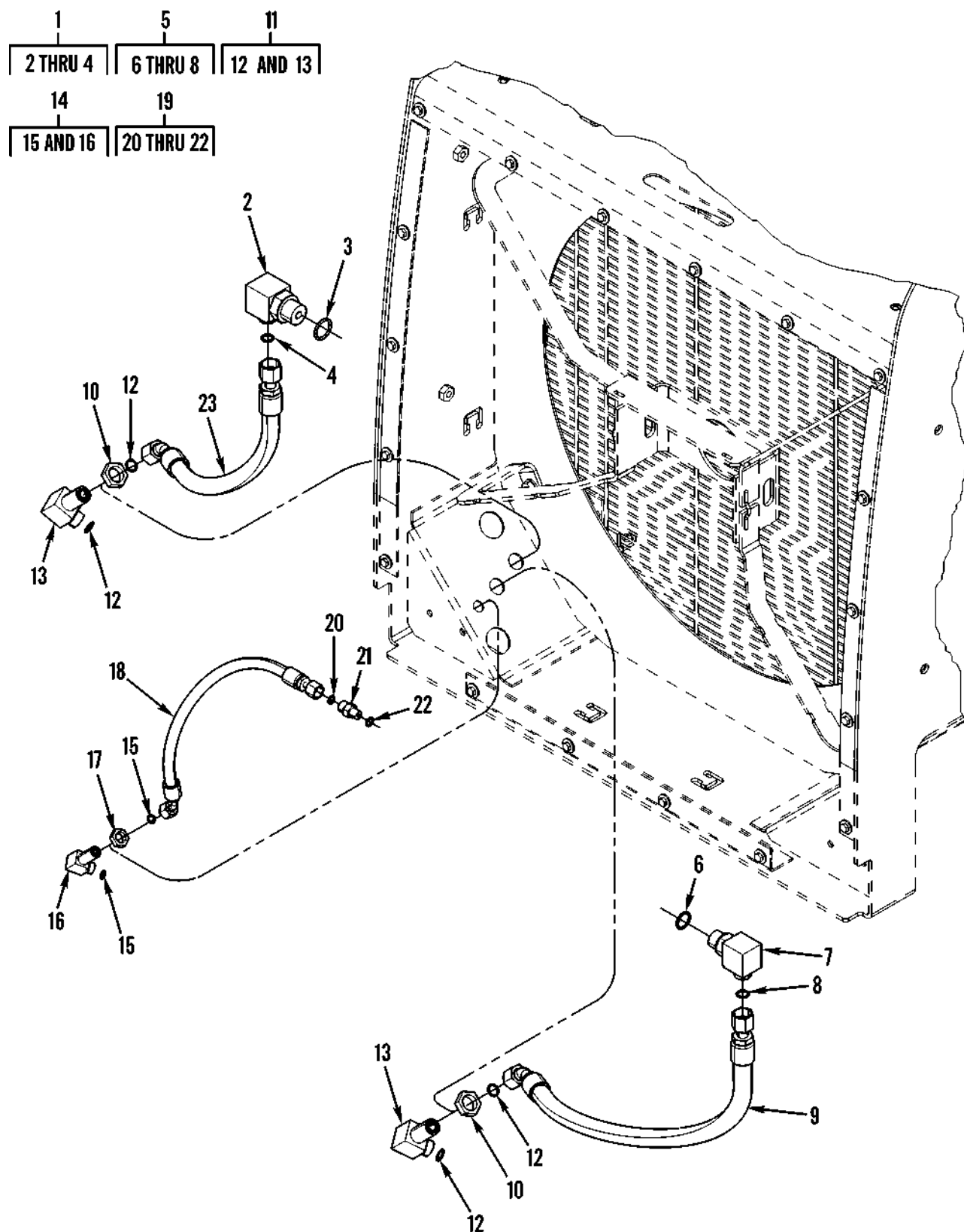
Figure 144. Hydraulic Fan Motor Lines
