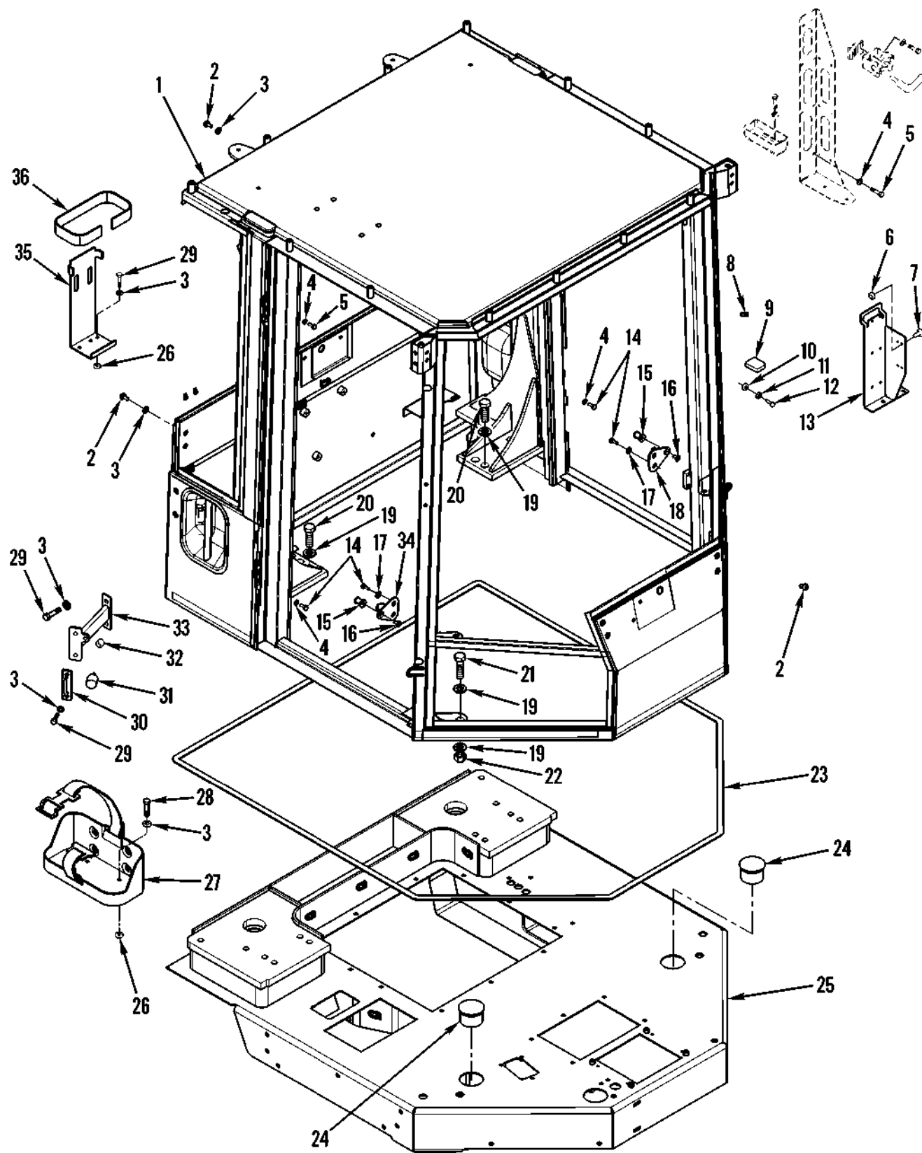
Figure 103. Cab
