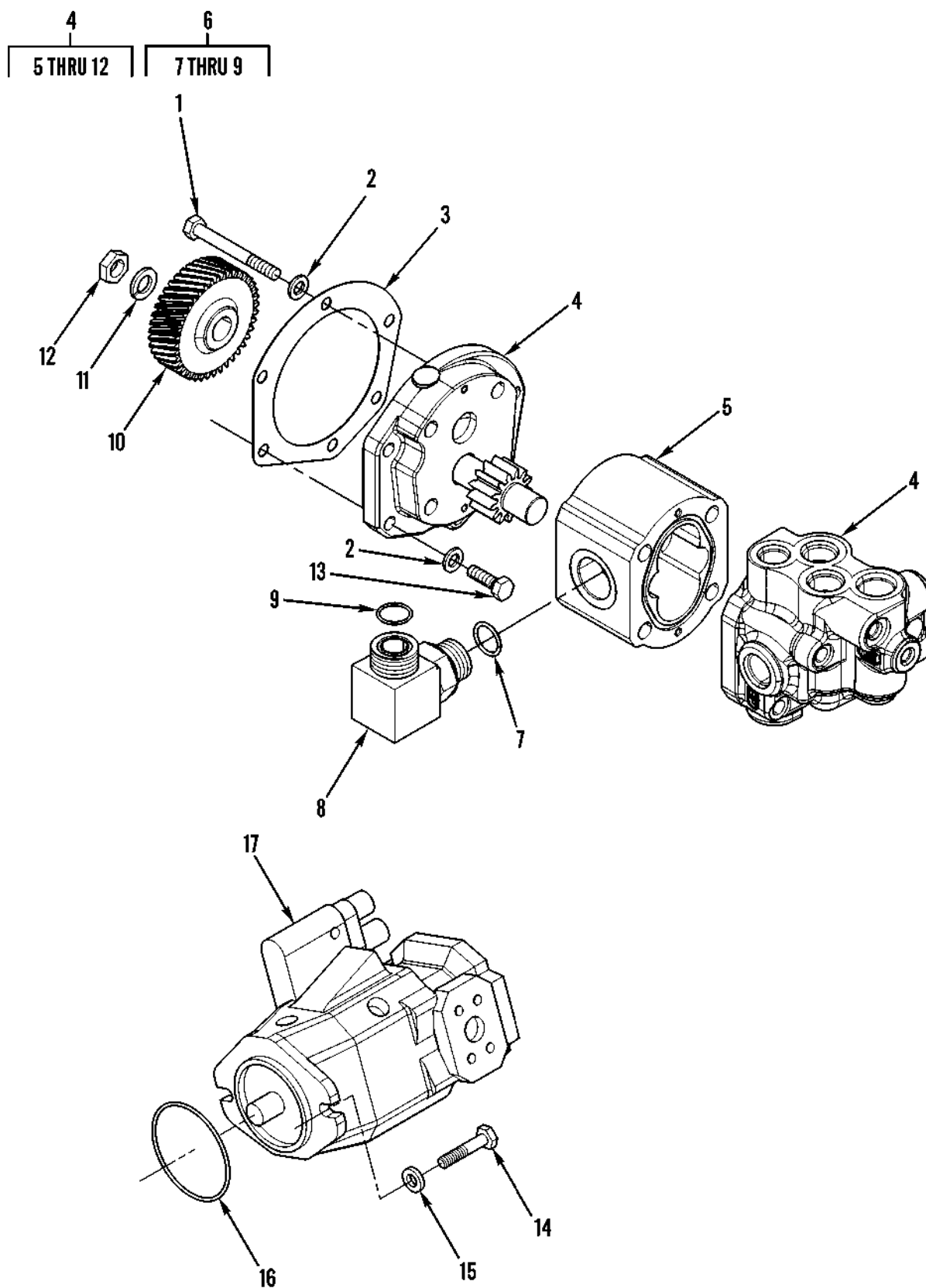
Figure 124. Braking and Hydraulic Fan Pump
