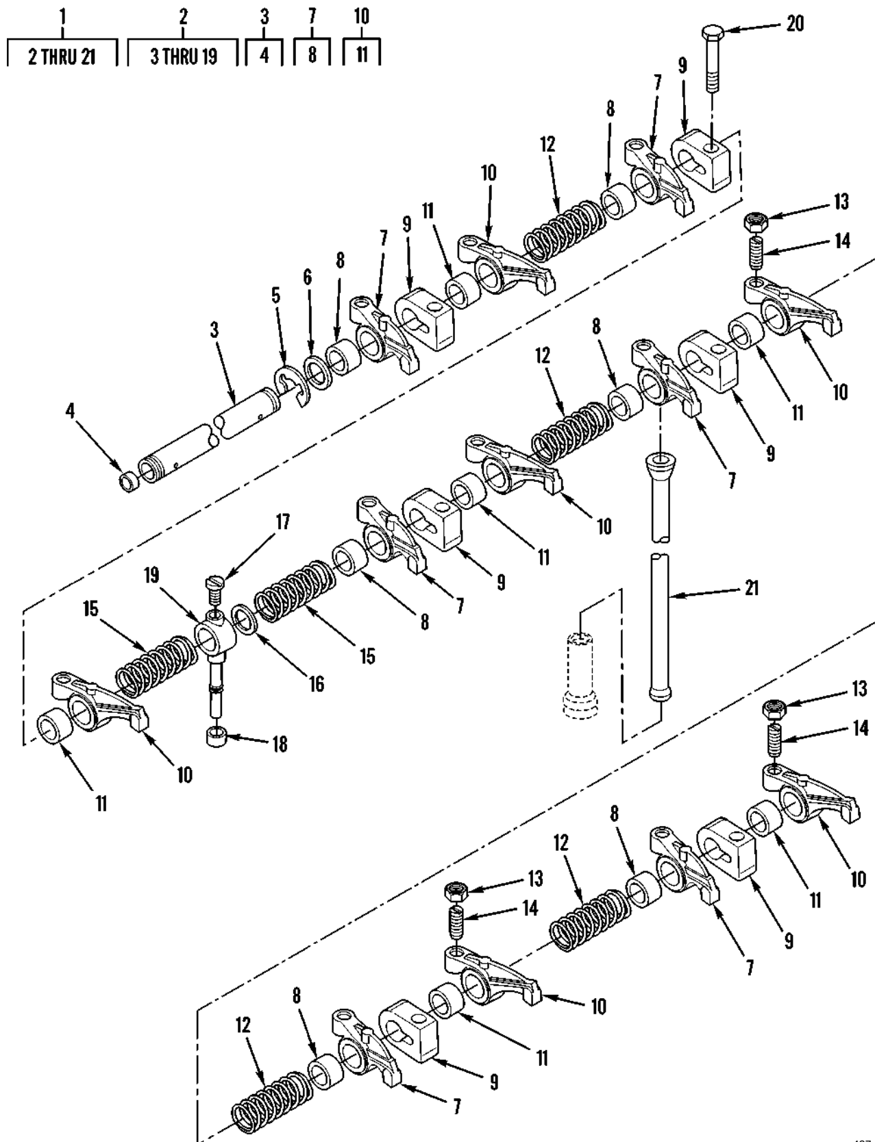
Figure 6. Rocker Arm
