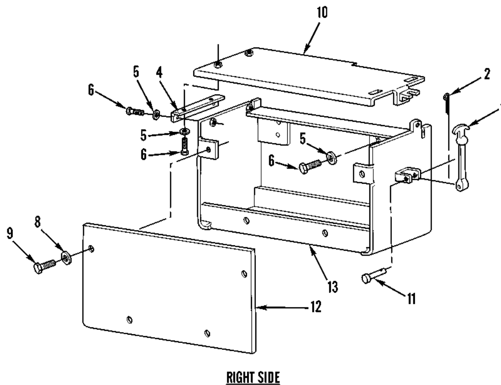
Figure 56. Battery Box and Wiring (Standard) (Sheet 1 of 2)
