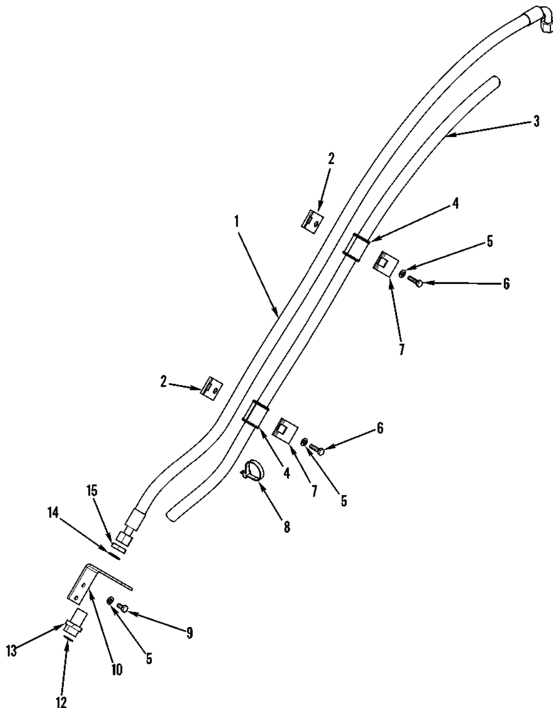
Figure 142. Quick Coupler Lines
