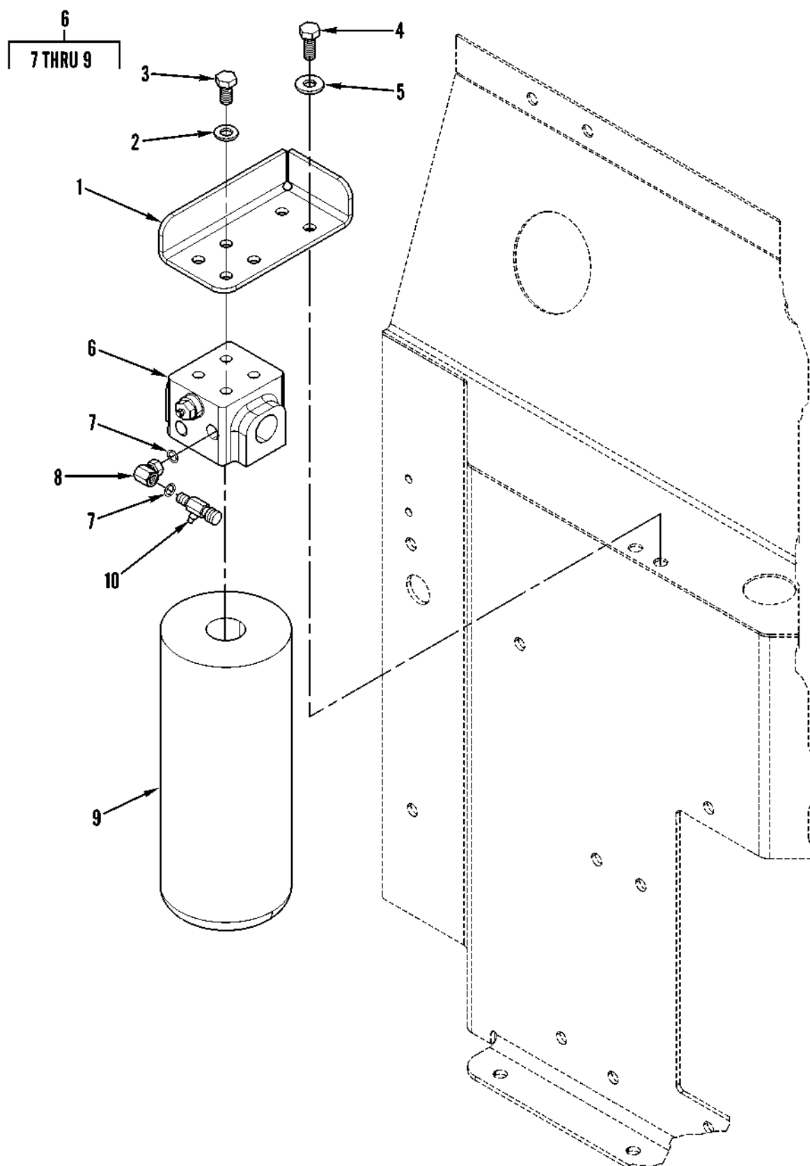
Figure 139. Hydraulic Oil Filter and Sampling Valve
