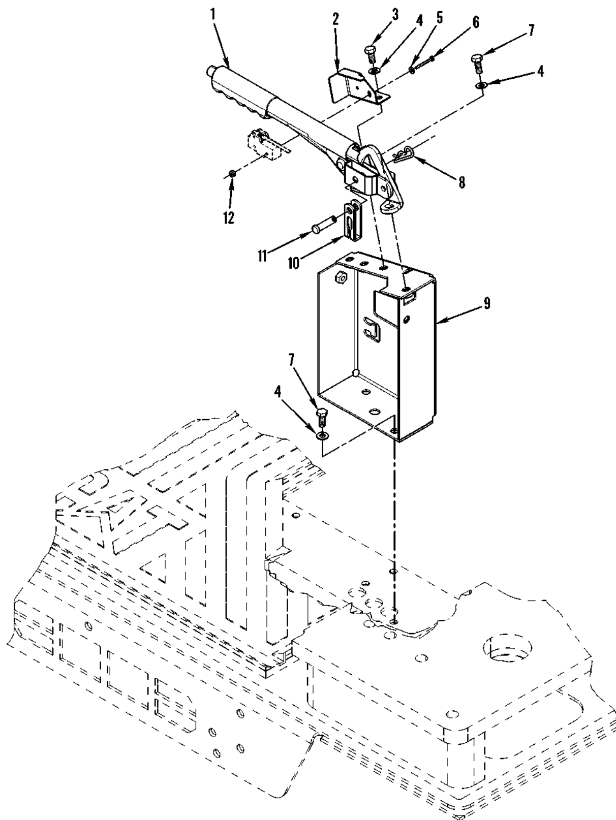
Figure 80. Parking Brake Handle and Related Parts
