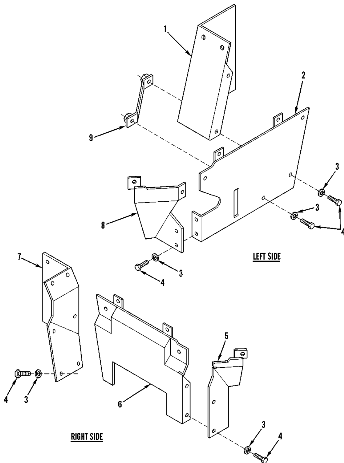
Figure 160. Chassis Guards and Covers (Arctic)
