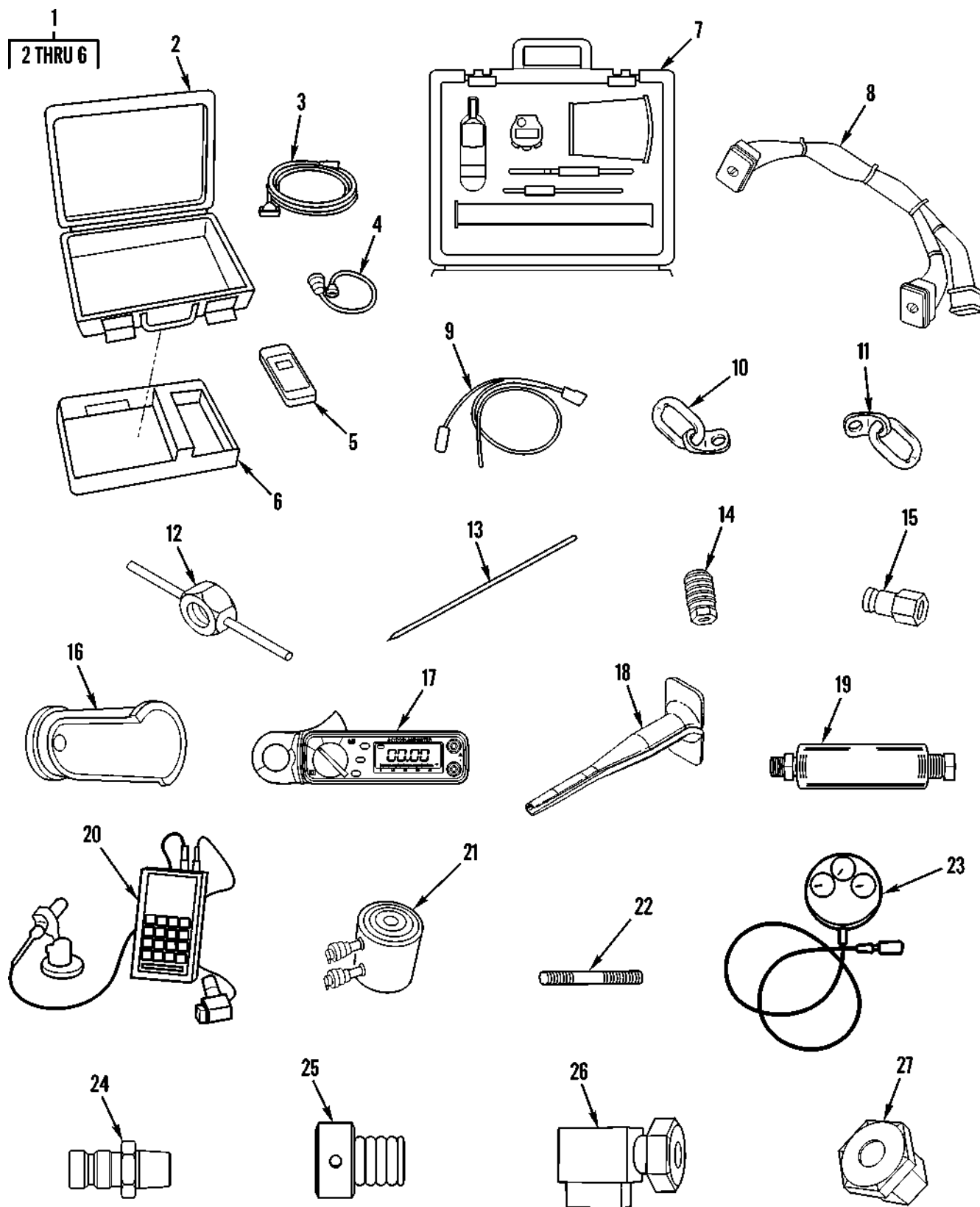
Figure 174. Unit Support Special Tools (Sheet 1 of 3)
