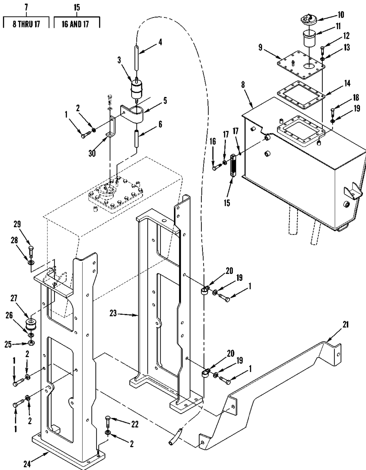
Figure 152. Hydraulic Tank and Mounting
