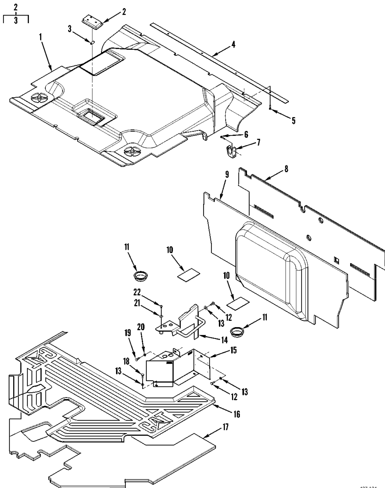
Figure 113. Cab Liners
