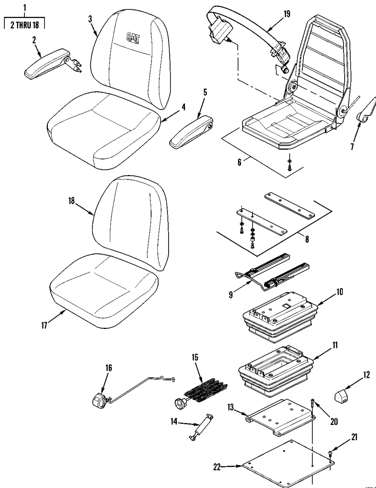
Figure 112. Seat
