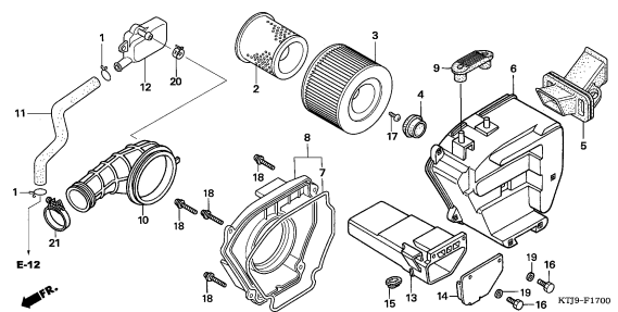
AIR CLEANER
