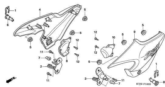
SIDE COVER
