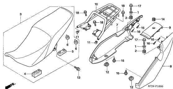
SEAT/REAR COWL
