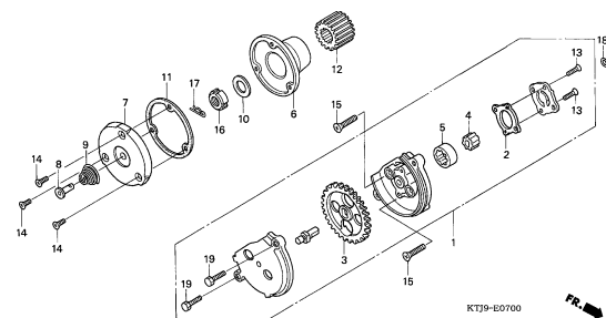
OIL PUMP
