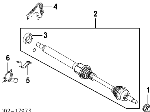
R&I Axle Shaft Assy
