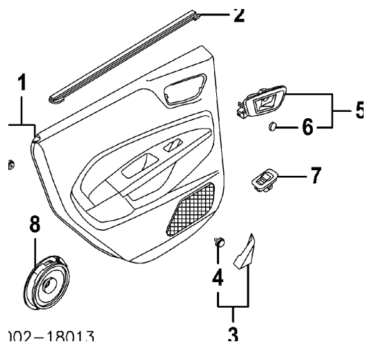
R&I Trim Panel
