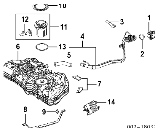
R&I Fuel Tank
