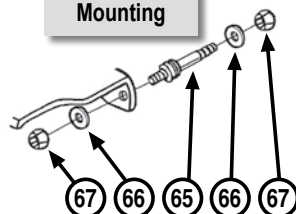
68-79 Multi Leaf Lower Shock Mounting
