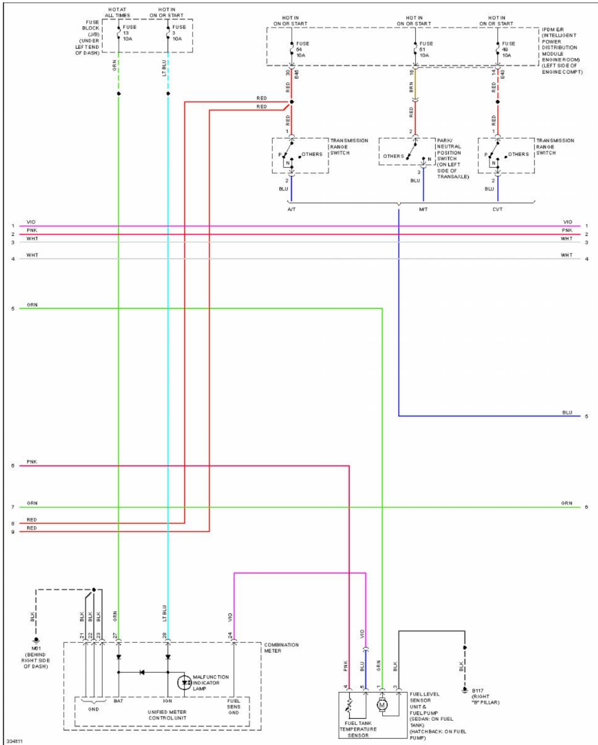
Fig. 17: 1.6L, Engine Performance Circuit (4 of 5)
