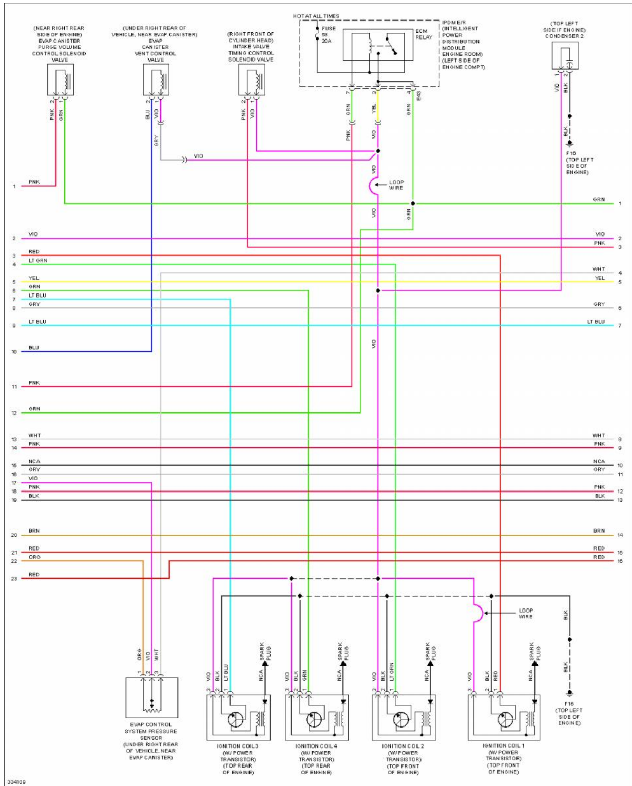
Fig. 15: 1.6L, Engine Performance Circuit (2 of 5)
