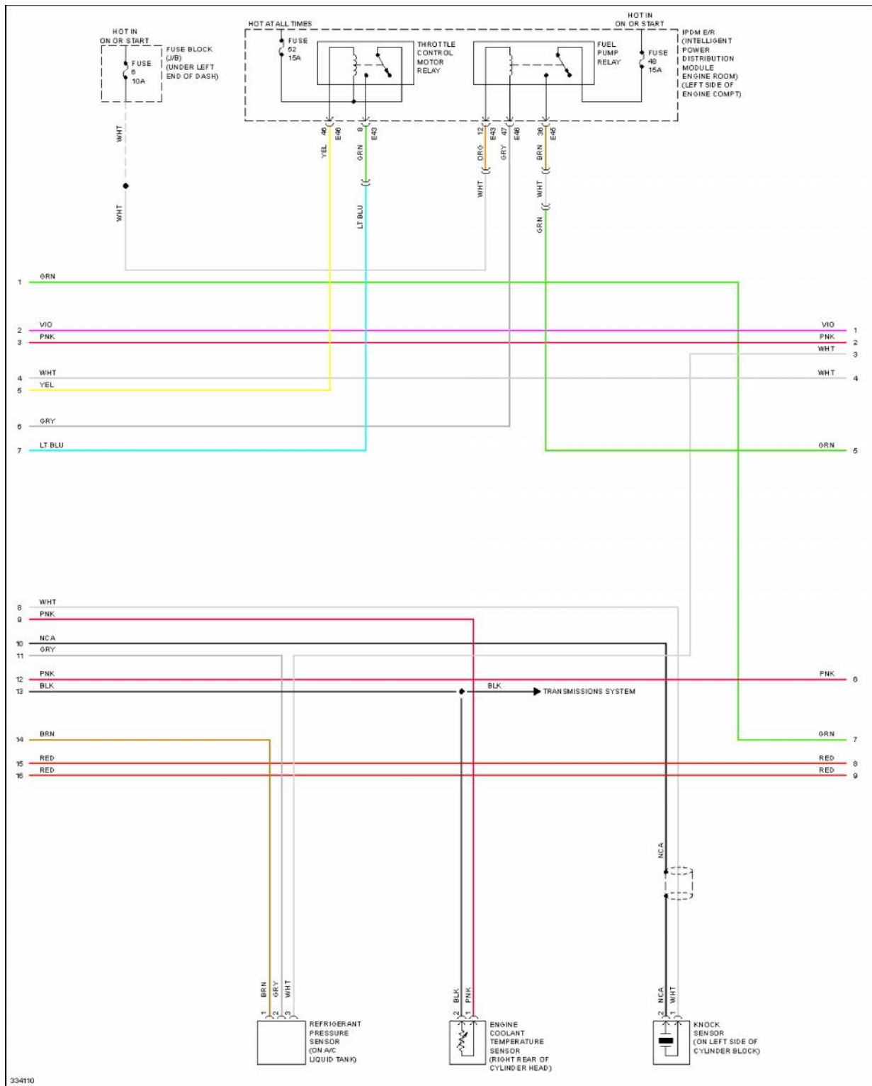
Fig. 16: 1.6L, Engine Performance Circuit (3 of 5)
