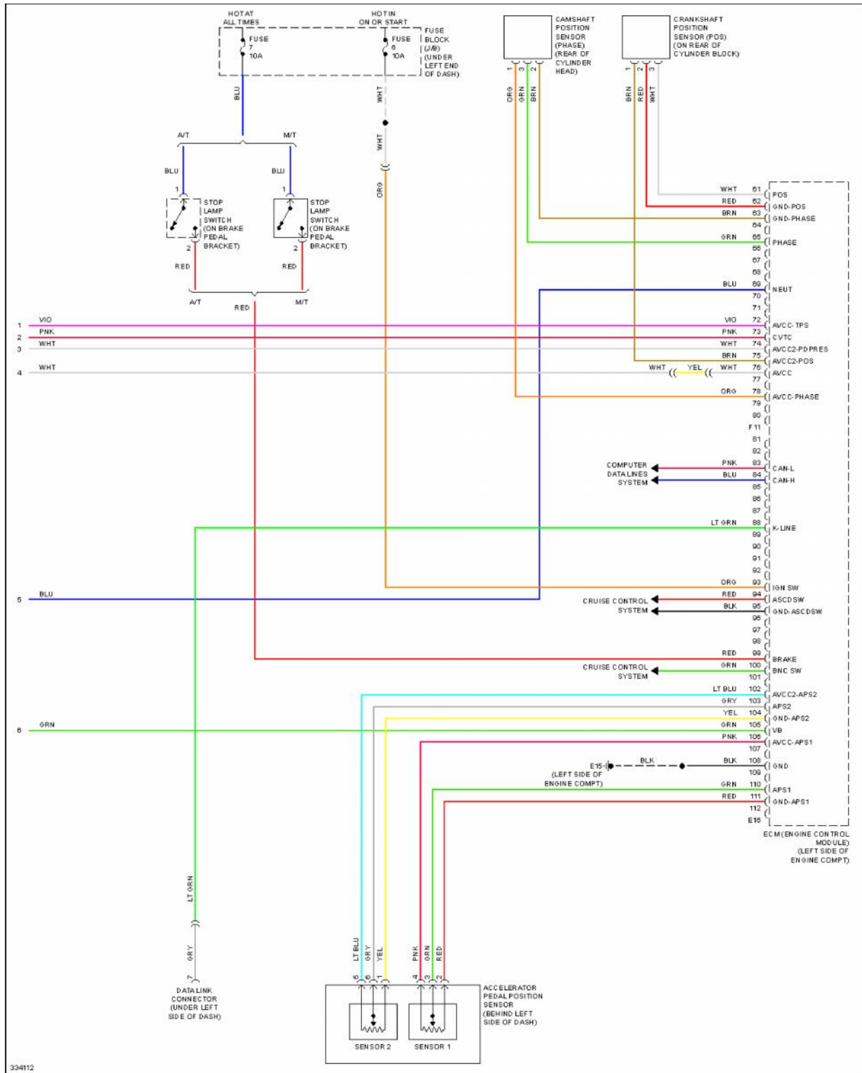
Fig. 18: 1.6L, Engine Performance Circuit (5 of 5)
