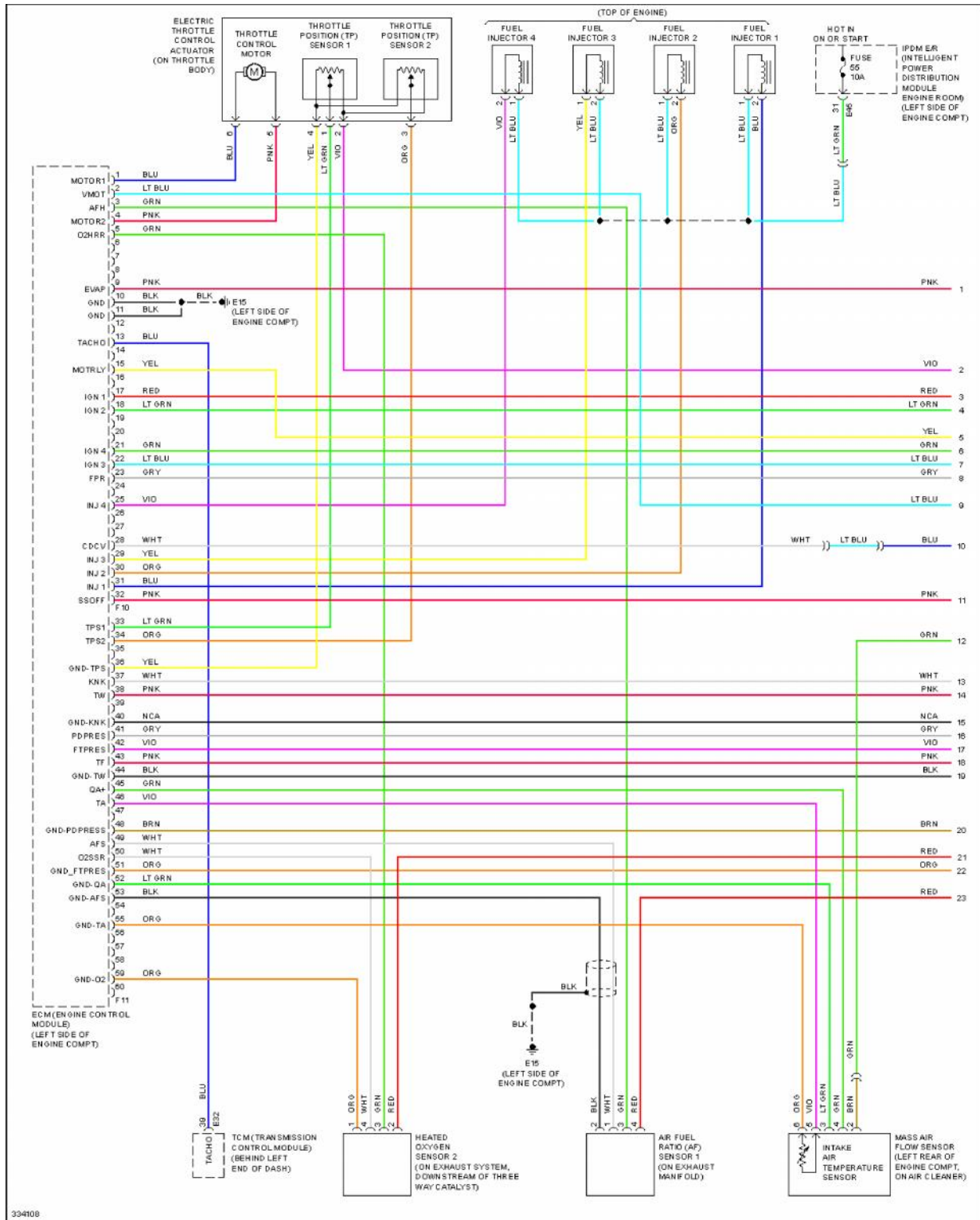
Fig. 14: 1.6L, Engine Performance Circuit (1 of 5)
