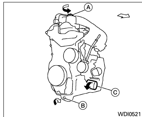
Motor MR18DE
