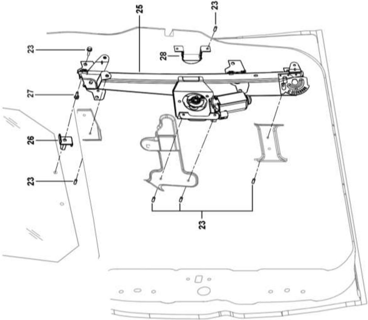
GROUP 2608A - DOOR MECHANISM - FRONT
