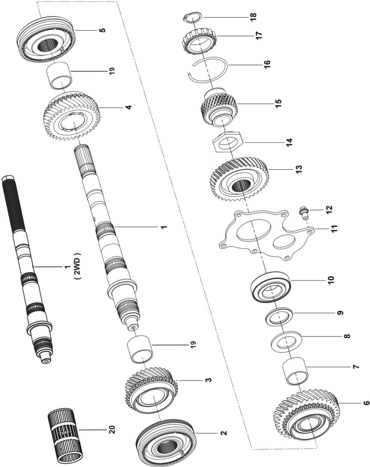
GROUP 1705 - MAIN SHAFT DRIVE GEAR & SYNCHRONIZER - 2WD/4WD
