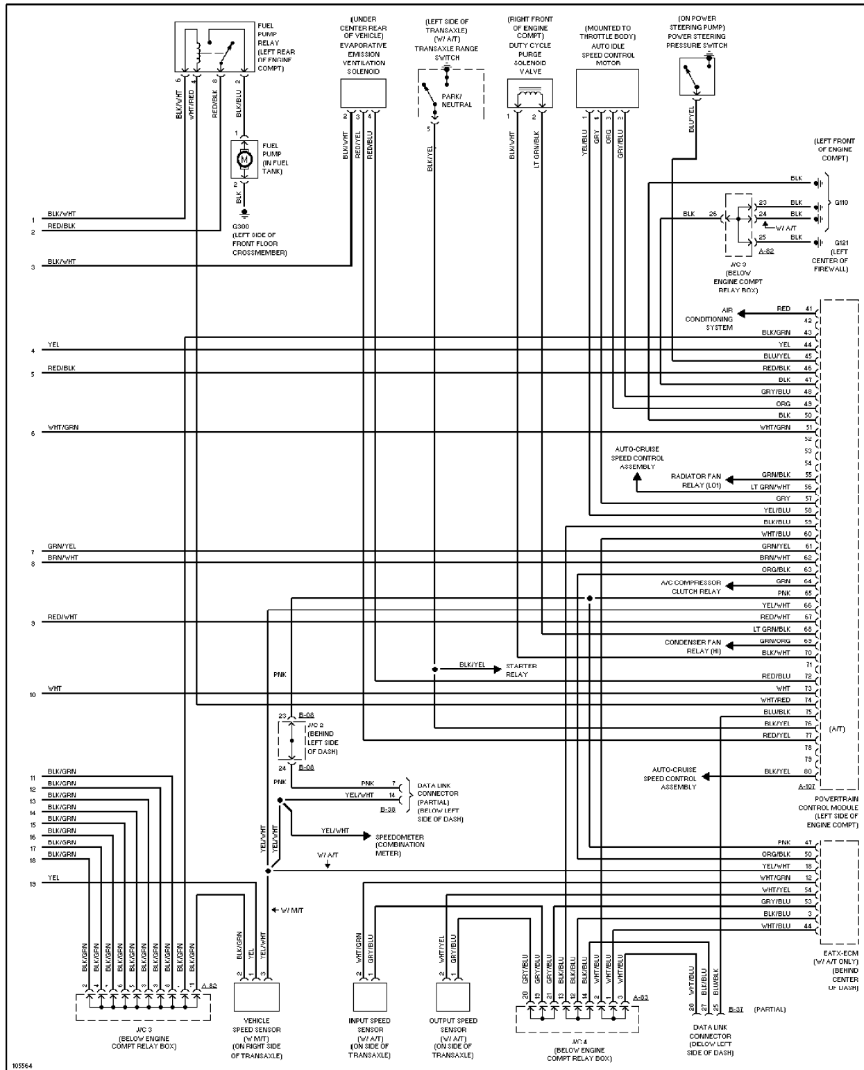
Fig. 6: Wiring Diagram (Eclipse 2.0L Non-Turbo - 3 Of 3)
