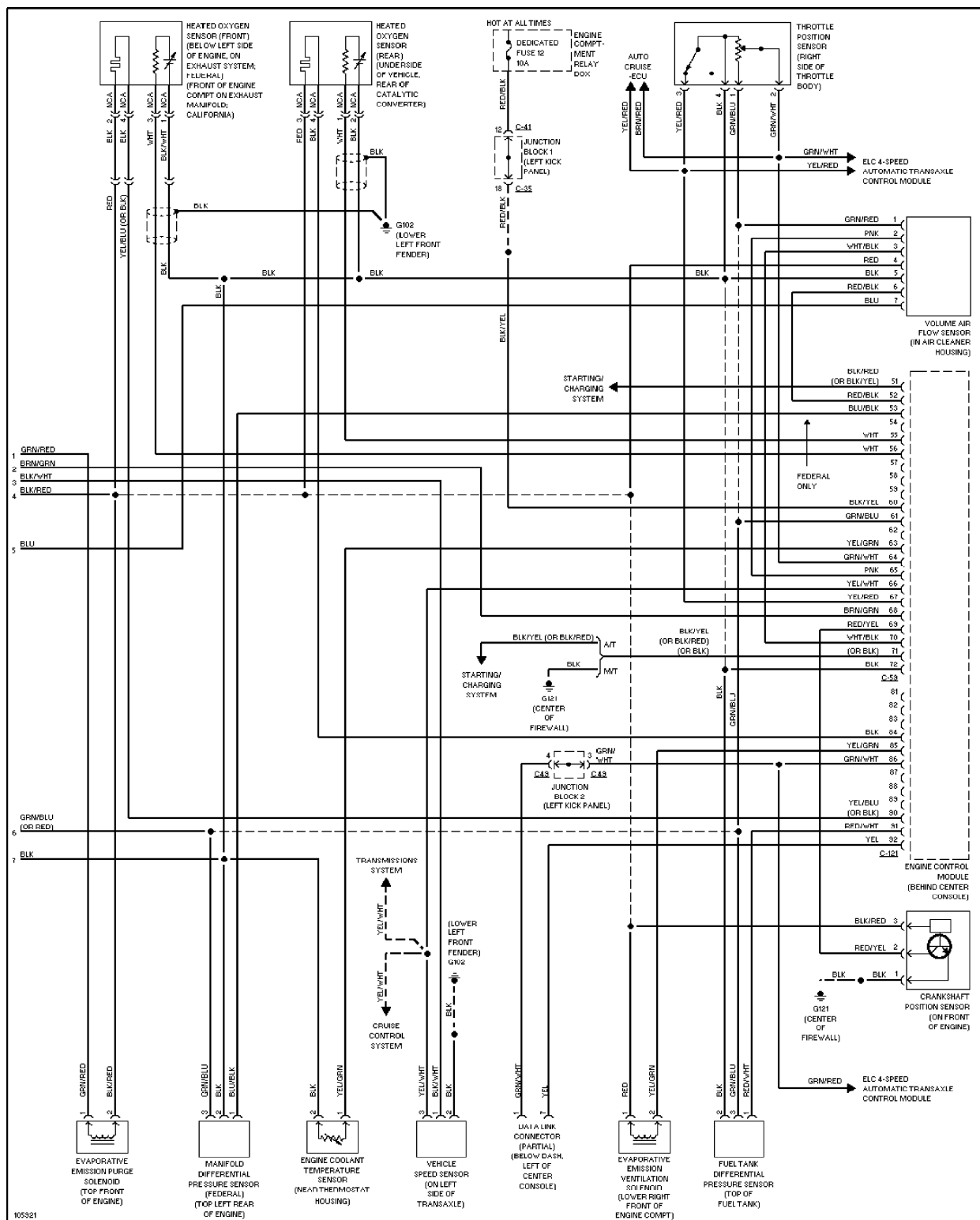
Fig. 12: Wiring Diagram (Galant 2.4L - 2 Of 2)
