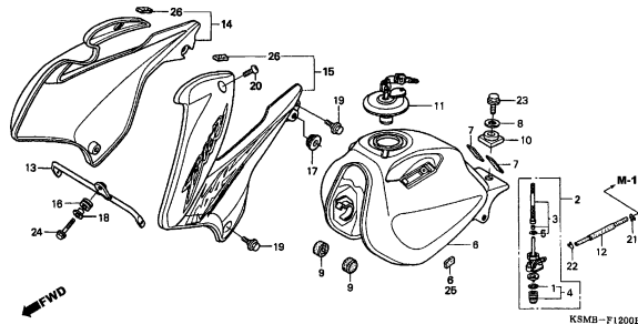
C-14.1 Tampa Lateral / Side Cover / Cubierta Lateral
