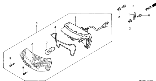
C-27 Chassi / Frame / Chasis
