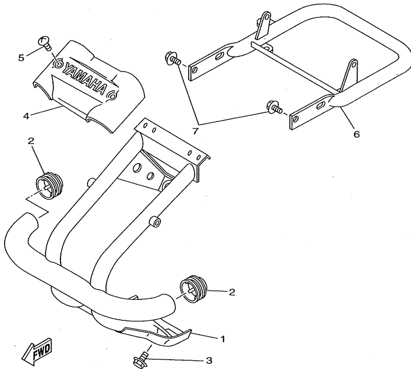
REF. NO. PART NO. DESCRIPTION U49 CAN EUR JPN REMARKS 1 3JM-2845N-00 BAR, CARRY FRONT 1 1 3JM-2845N-10 BAR, CARRY FRONT 1 1 2 2HR-28415-00 DAMPER 1 2 2 2 2 3 95817-08016 BOLT, FLANGE 3 3 3 3 4 2XJ-2842M-00 COVER 1 1 1 1 1 5 90154-05059 SCREW, BINDING 2 2 2 2 6 3JM-2845R-00 BAR, CARRY REAR 1 1 3JM-2845R-10 BAR, CARRY REAR 1 3JM-2845R-30 BAR, CARRY REAR 1 7 95817-08016 BOLT, FLANGE 3 3 3 3
