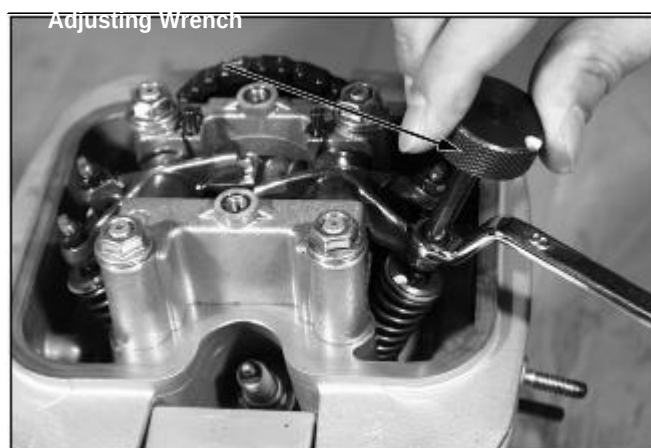
Adjusting Wrench
