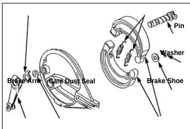
Brake Cam
