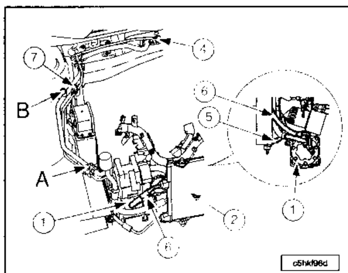
Motores DW10TD y DW10ATED.
