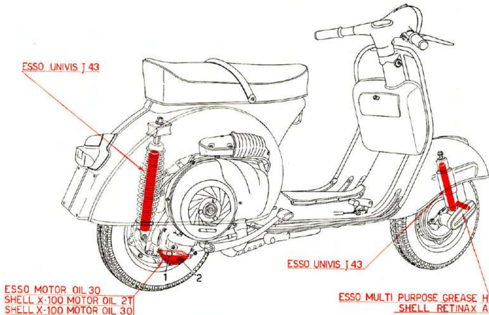
Fig. 23 - Lubrication scheme
