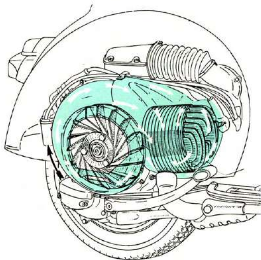
Fig. 9 - Cooling circuit
