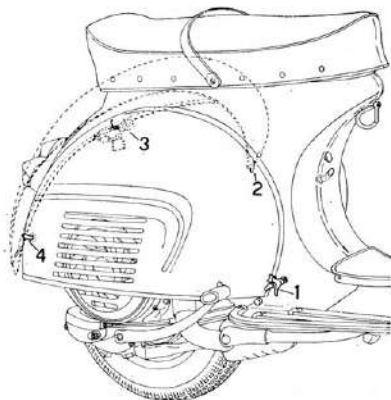
Fig. 17 - Detaching engine cowl
