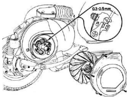
Fig. 22 - Registration of contact breaker points
