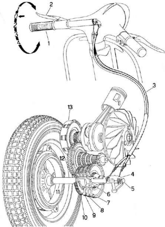
Fig. 16 - Layout of gear box and transmission
