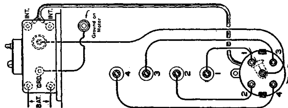
Fig. 4. Diagram of wiring Type 14 Ford System.
