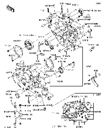
C-5 Crankcase
