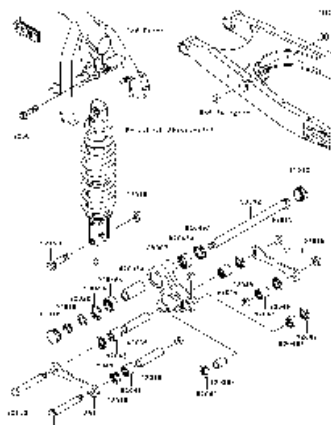
E-7 Rear Suspension
