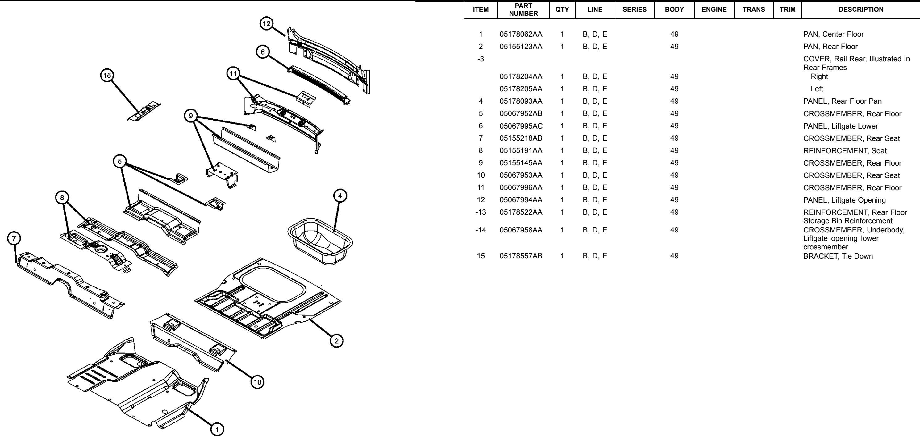
Center and Rear Floor Pan Figure 60-130
