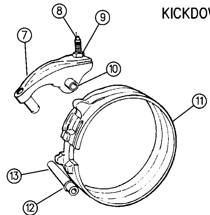
DOUBLE WRAP REVERSE BAND
