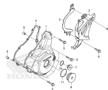
LEFT CRANKCASE COVER
