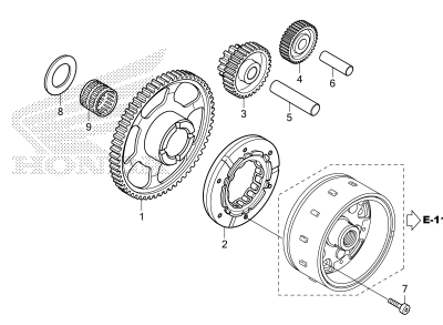
STARTING CLUTCH
