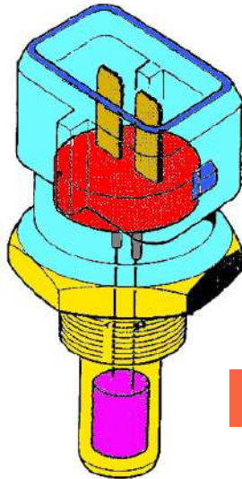
Sensor NTC
