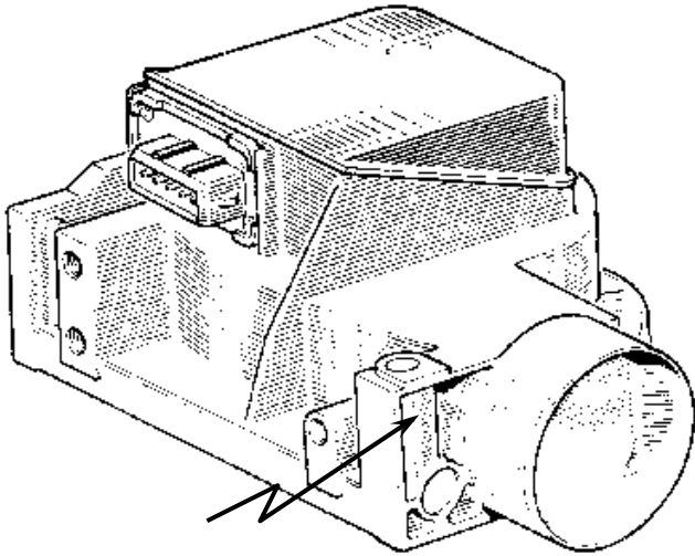
Canal by-pass
