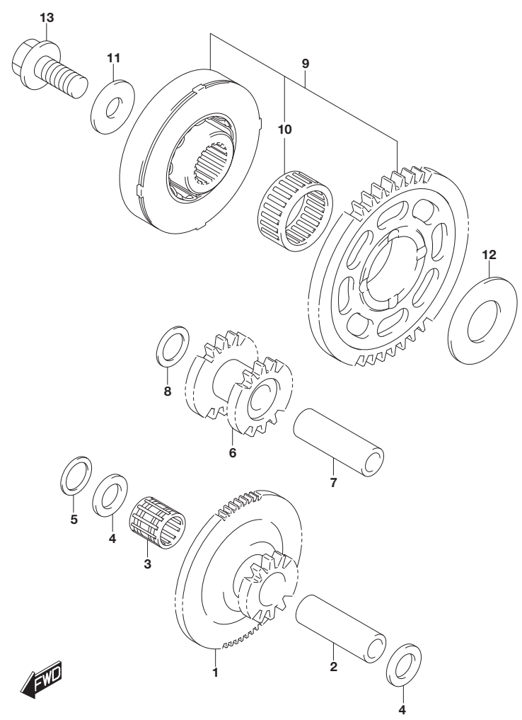
GSX-S750L8_E03_E28_122A STARTER CLUTCH
