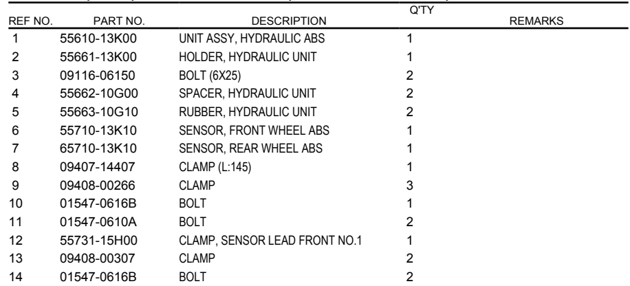
FIG.533C (2-D-2) HYDRAULIC UNIT (GSX-S750AZL8 E28)
