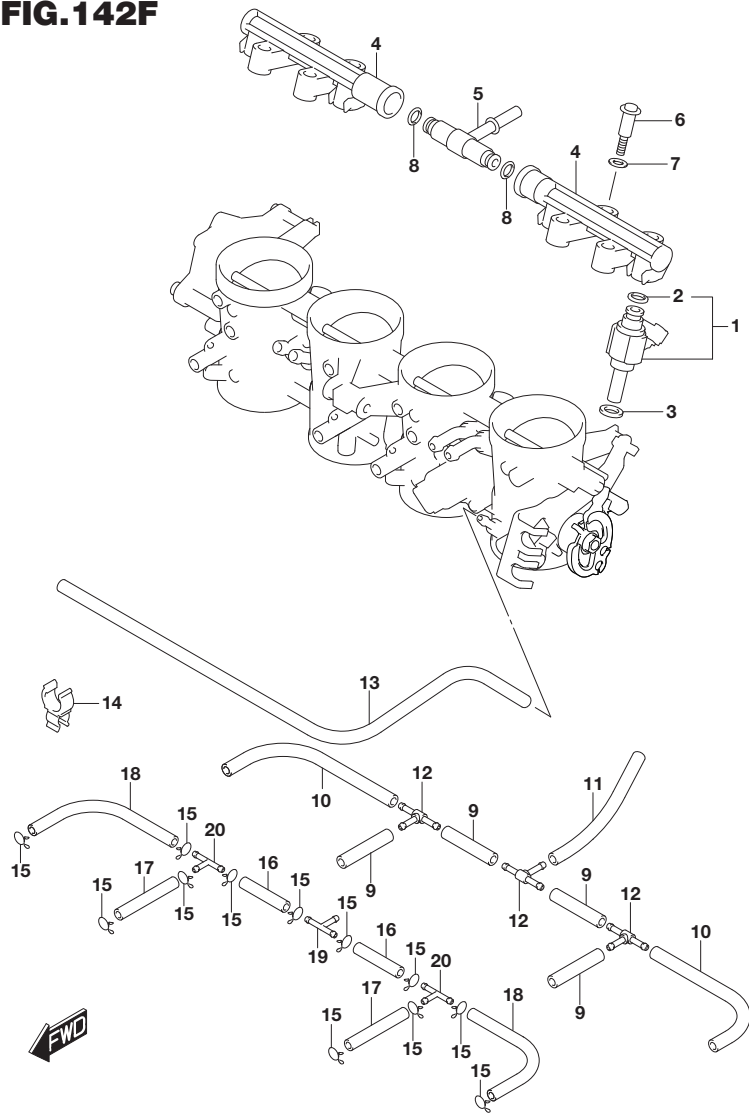
FIG.142F (1-C-14) THROTTLE BODY HOSE/JOINT (GSX-S750AL8 E33)
