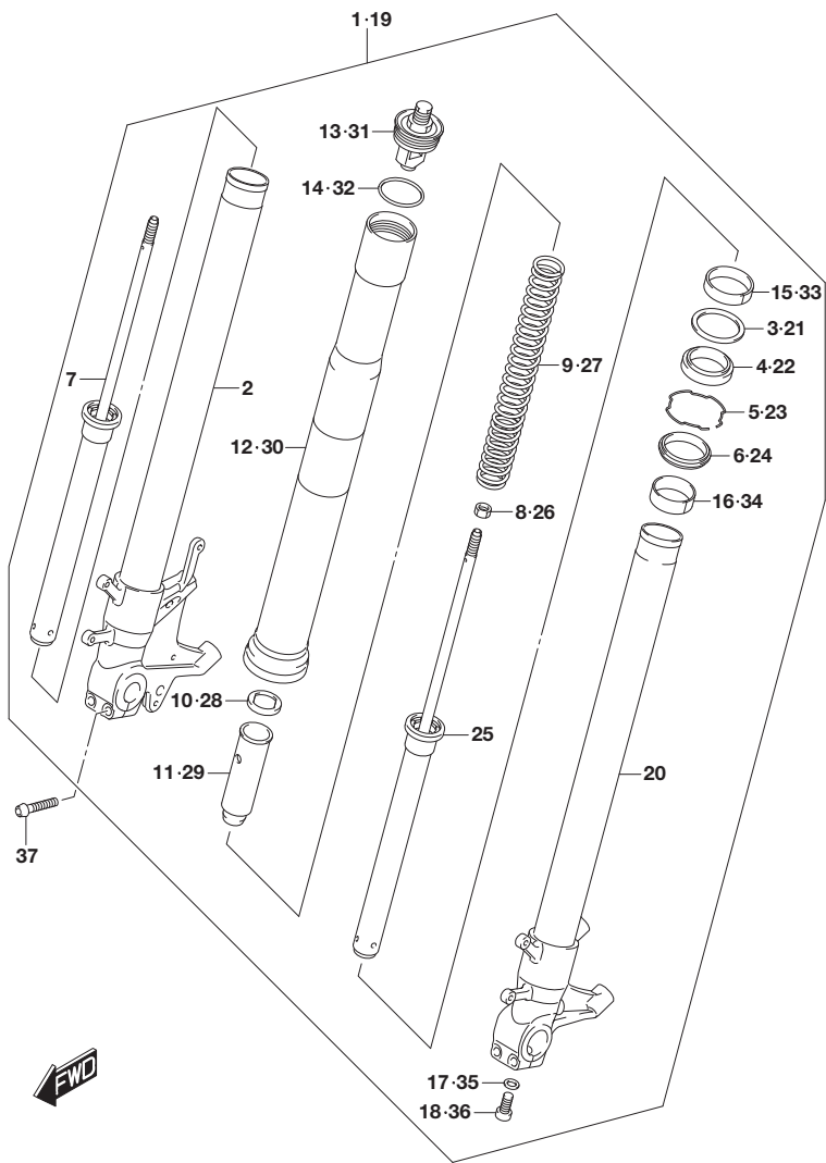
GSX-S750L8_E03_E28_521H FRONT FORK DAMPER
