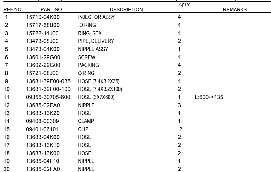
FIG.142B (1-C-10) THROTTLE BODY HOSE/JOINT (GSX-S750L8 E33)
