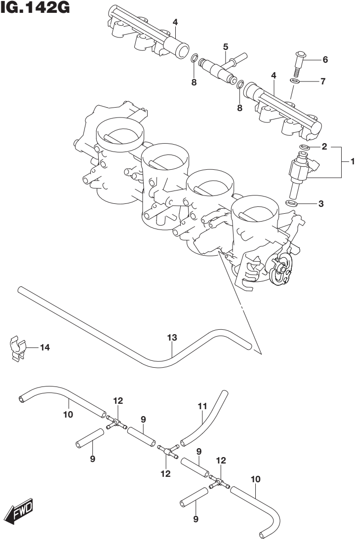
FIG.142G (1-C-15) THROTTLE BODY HOSE/JOINT (GSX-S750AZL8 E28)
