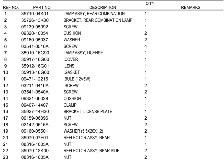
FIG.339A (1-H-3) REAR COMBINATION LAMP
