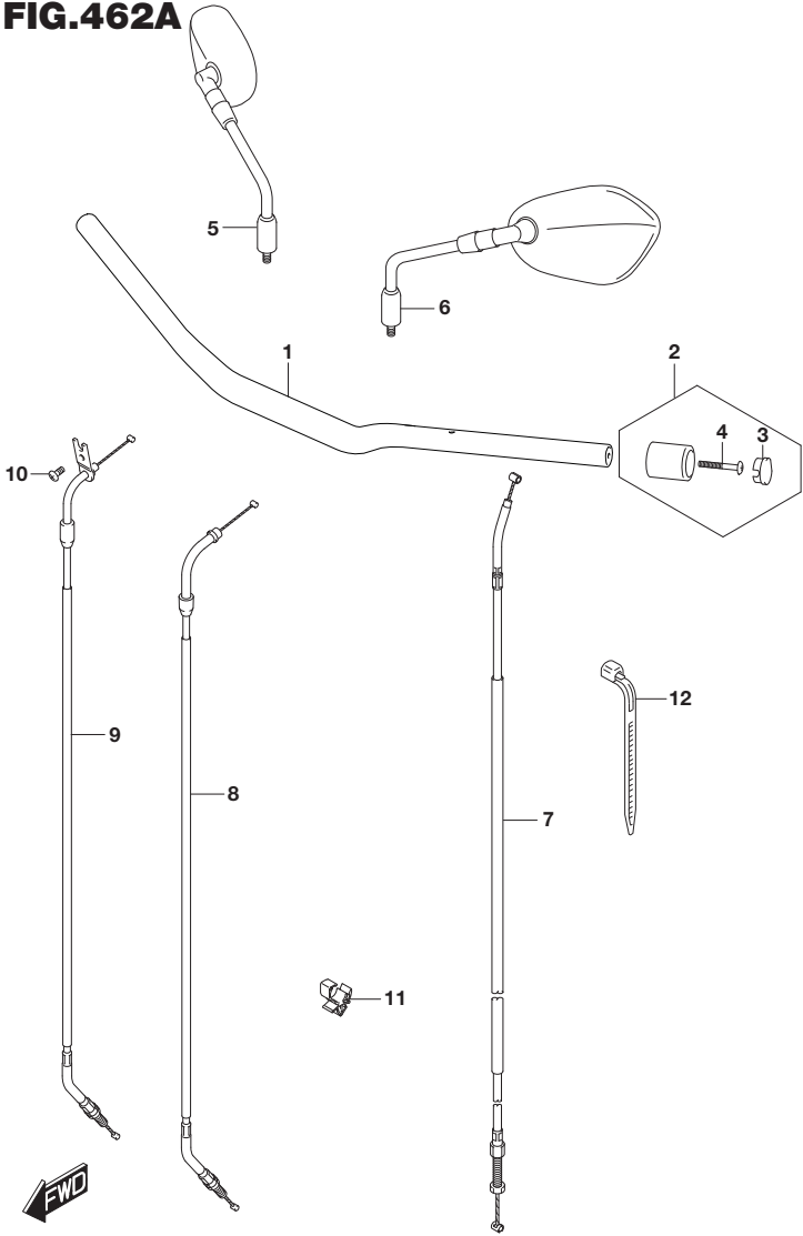
GSX-S750L8_E03_E28_462A HANDLEBAR
