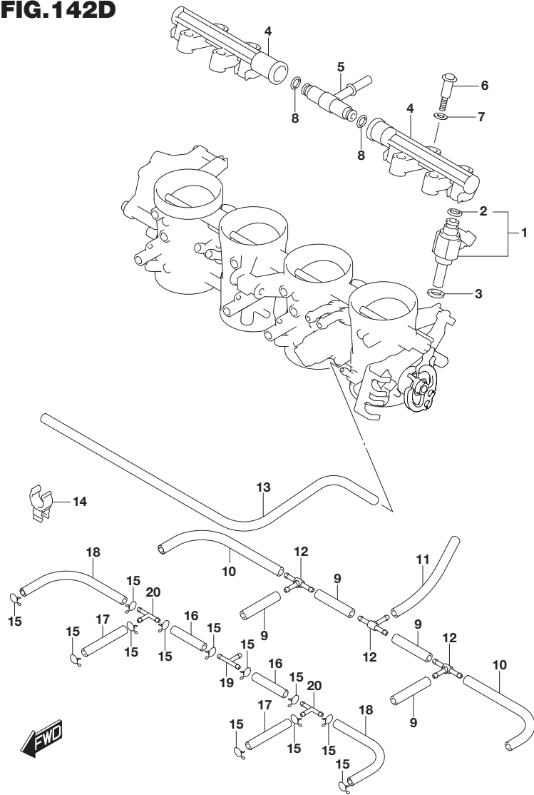
FIG.142D (1-C-12) THROTTLE BODY HOSE/JOINT (GSX-S750ZL8 E33)
