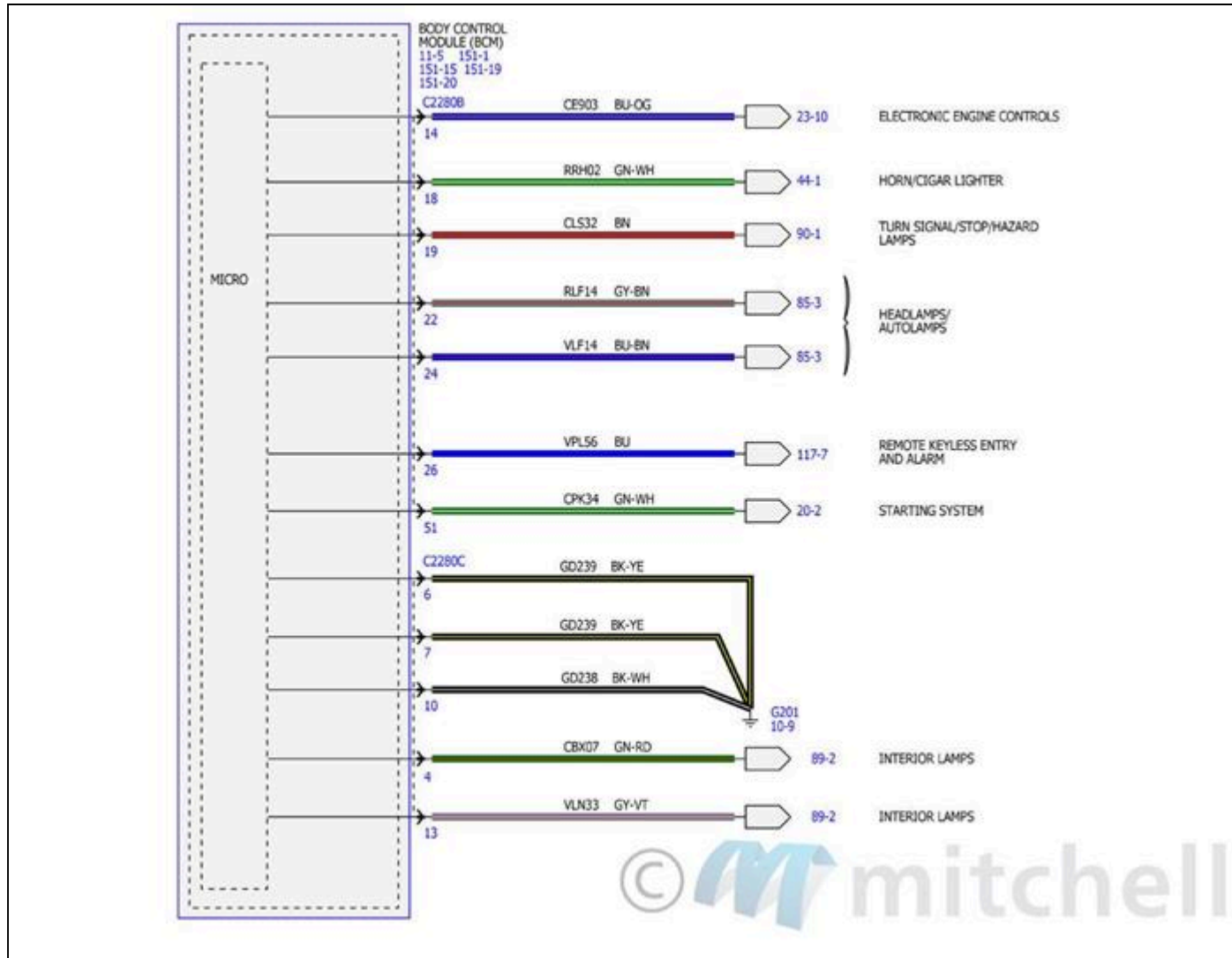
Fig. 161: Power Distribution/BCM Wiring Diagrams (32 Of 34)
