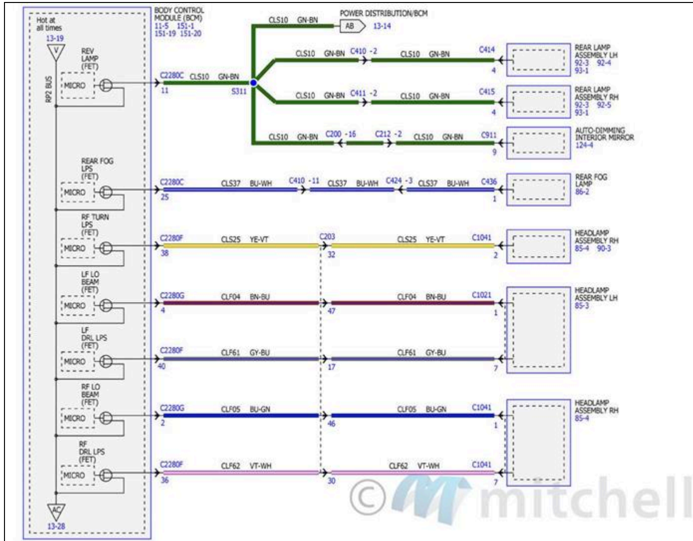
Fig. 156: Power Distribution/BCM Wiring Diagrams (27 Of 34)
