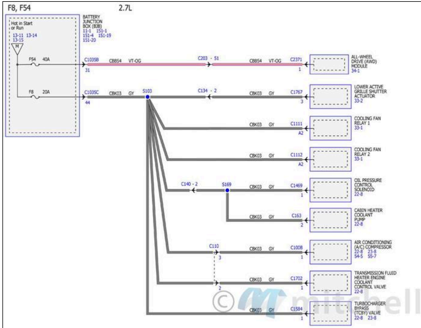
Fig. 142: Power Distribution/BCM Wiring Diagrams (13 Of 34)
