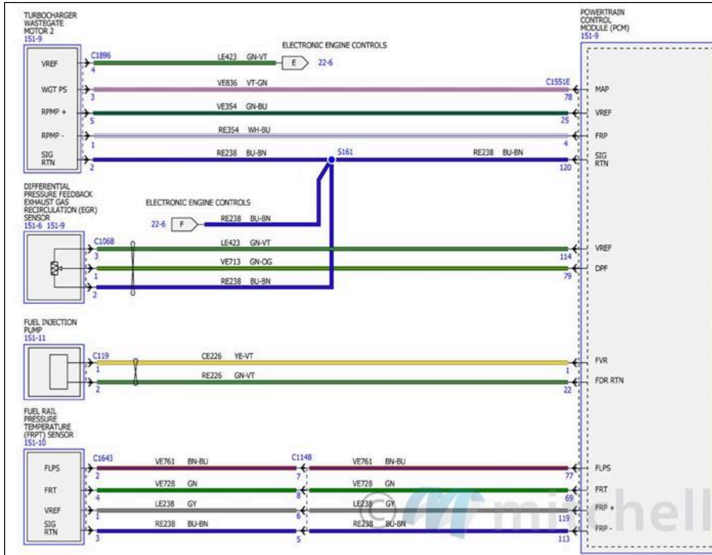
Fig. 66: Electronic Engine Controls Wiring Diagrams - 2.7L (7 Of 18)
