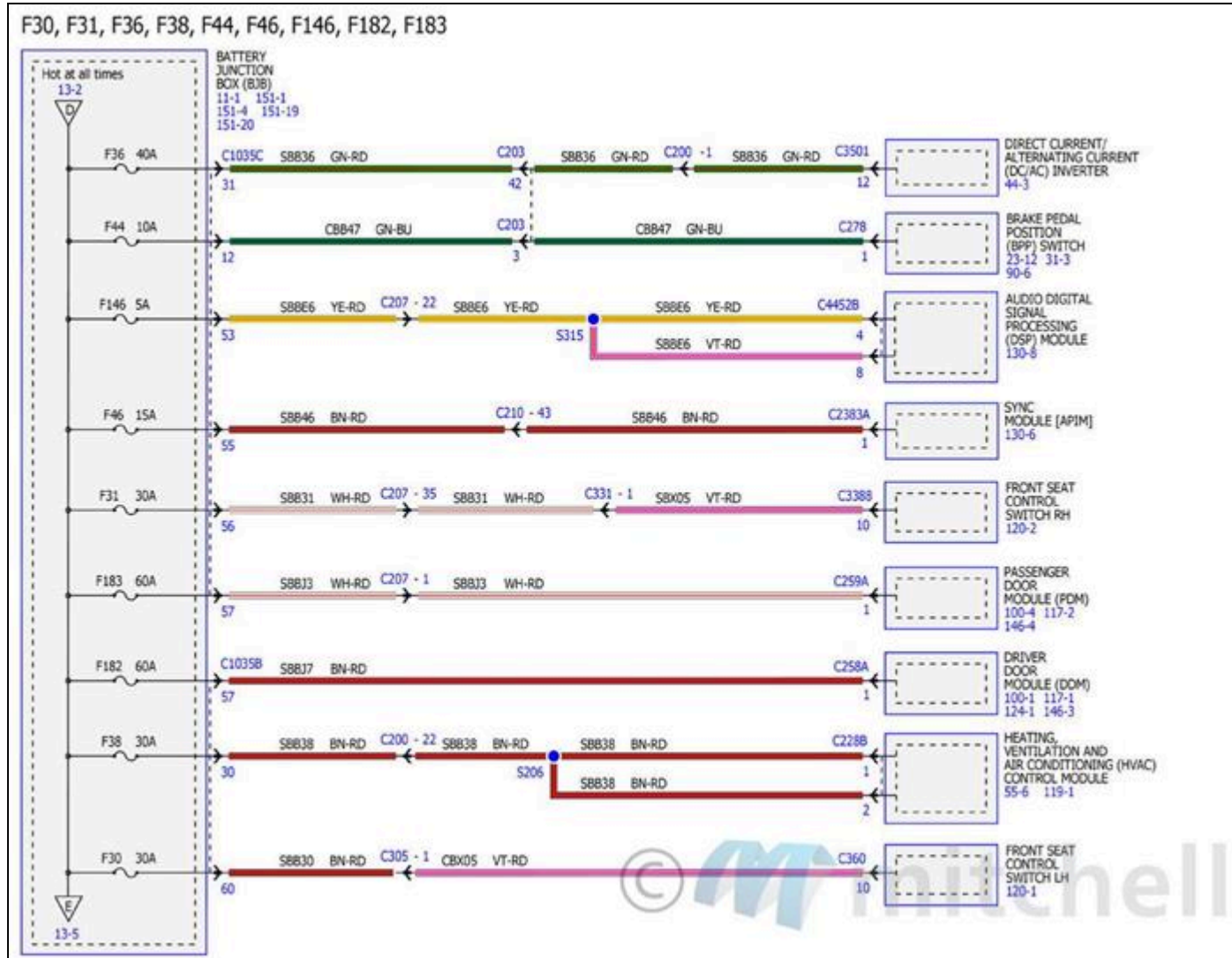
Fig. 133: Power Distribution/BCM Wiring Diagrams (4 Of 34)
