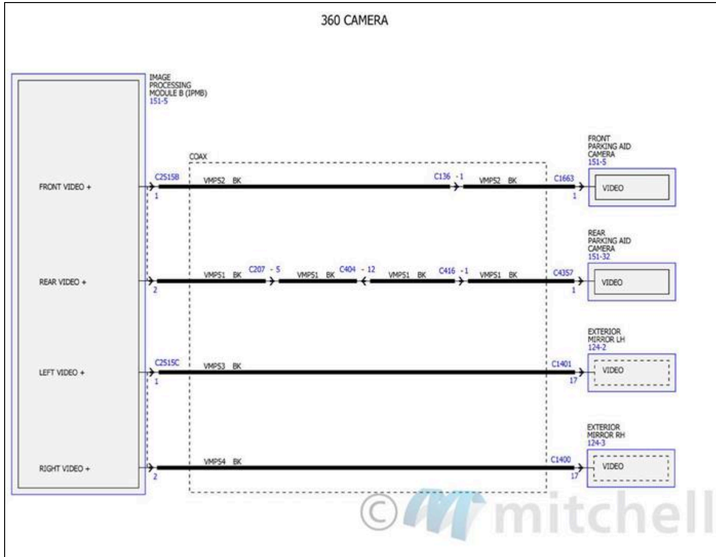
Fig. 120: Parking Aid Wiring Diagrams (6 Of 6)
