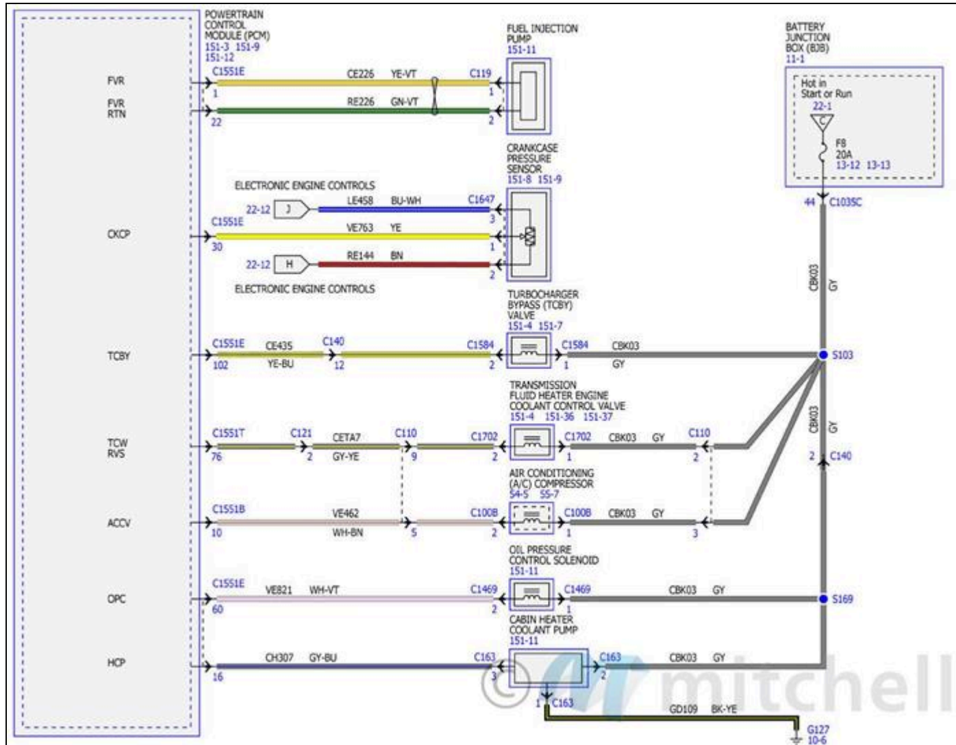
Fig. 67: Electronic Engine Controls Wiring Diagrams - 2.7L (8 Of 18)
