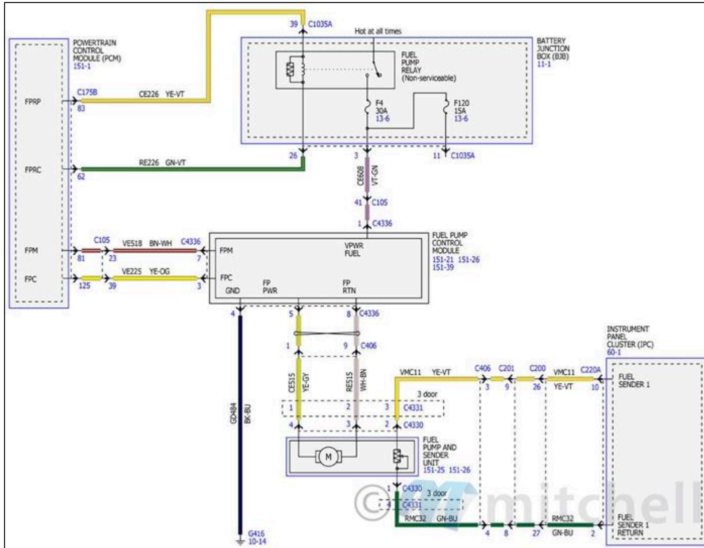
Fig. 56: Electronic Engine Controls Wiring Diagrams - 2.3L (14 Of 17)
