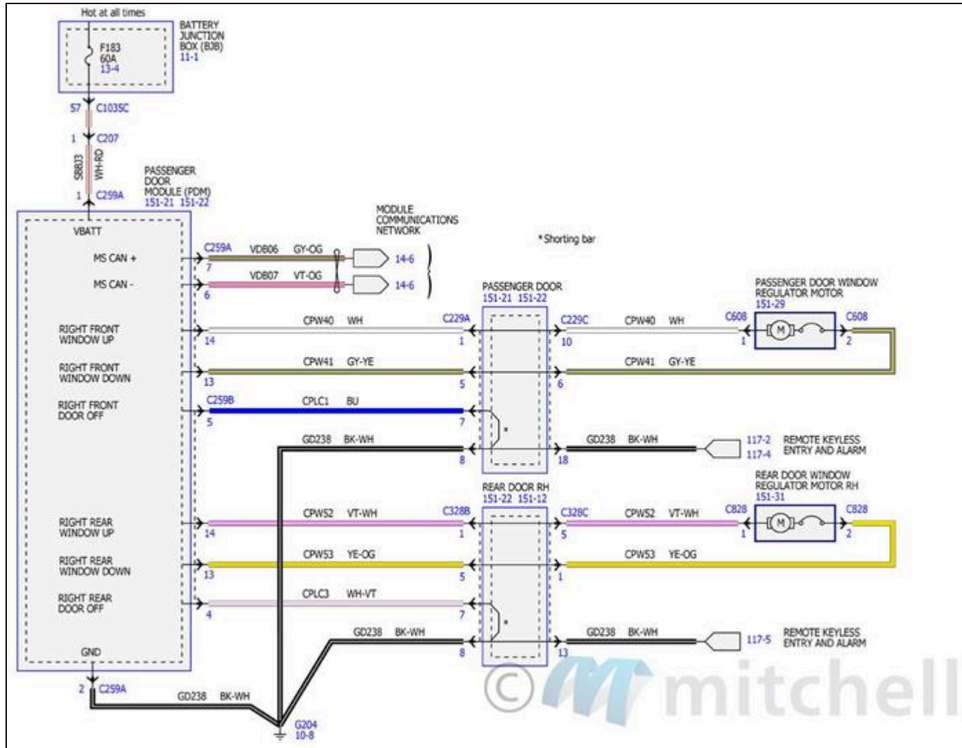
Fig. 174: Power Windows Wiring Diagrams (4 Of 6)
