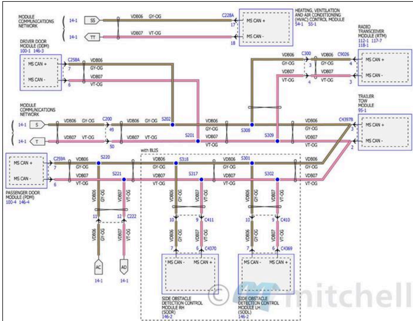
Fig. 113: Module Communications Network Wiring Diagrams (7 Of 8)
