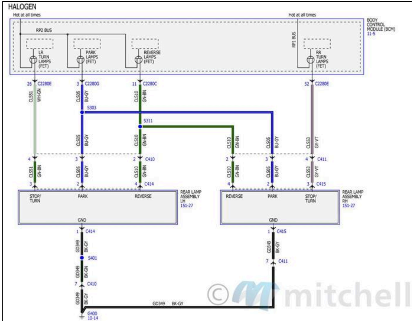
Fig. 123: Parking, Rear and License Lamps Wiring Diagrams (3 Of 6)
