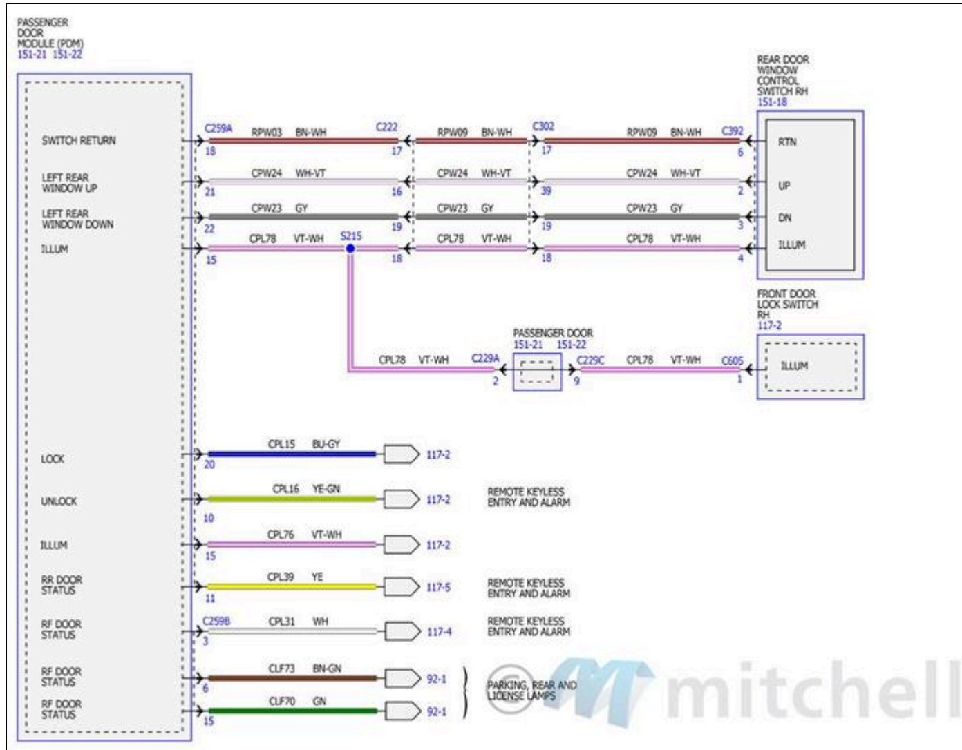
Fig. 175: Power Windows Wiring Diagrams (5 Of 6)
