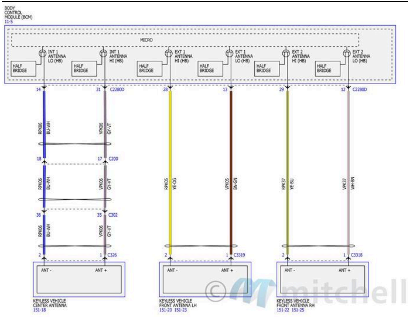
Fig. 182: Remote Keyless Entry and Alarm Wiring Diagrams (6 Of 8)
