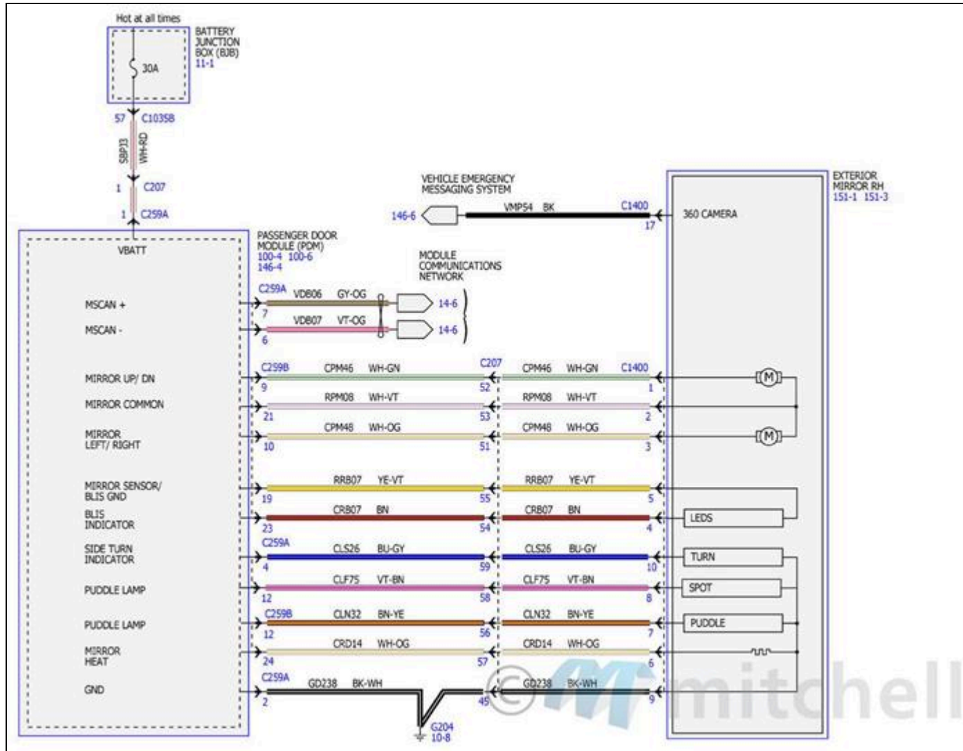
Fig. 166: Power Mirrors Wiring Diagrams (3 Of 4)
