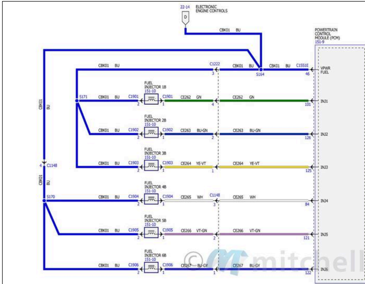
Fig. 63: Electronic Engine Controls Wiring Diagrams - 2.7L (4 Of 18)
