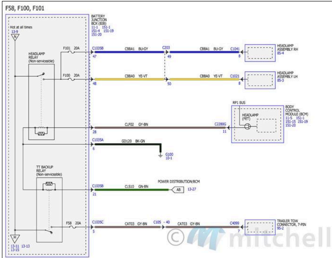
Fig. 143: Power Distribution/BCM Wiring Diagrams (14 Of 34)
