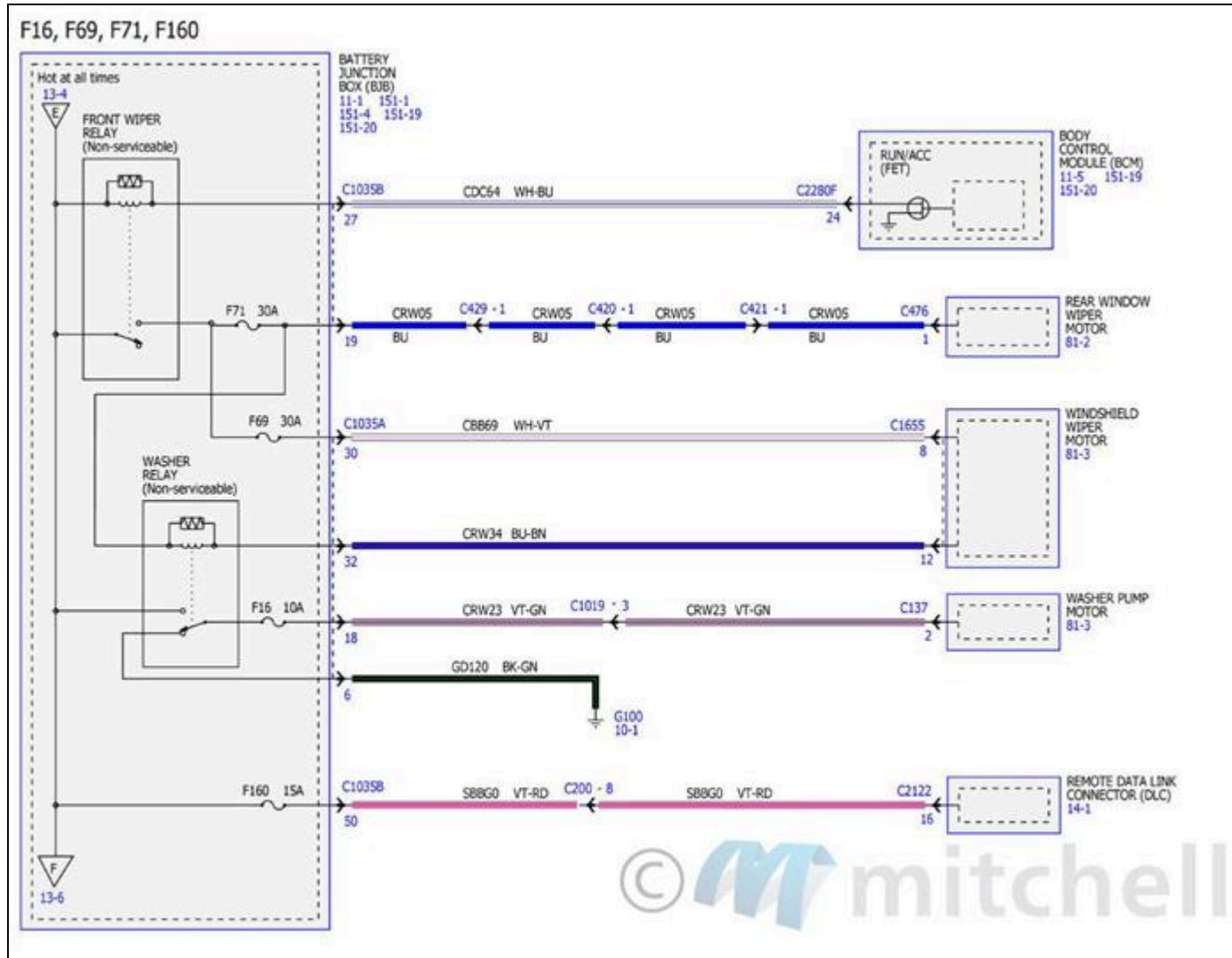
Fig. 134: Power Distribution/BCM Wiring Diagrams (5 Of 34)
