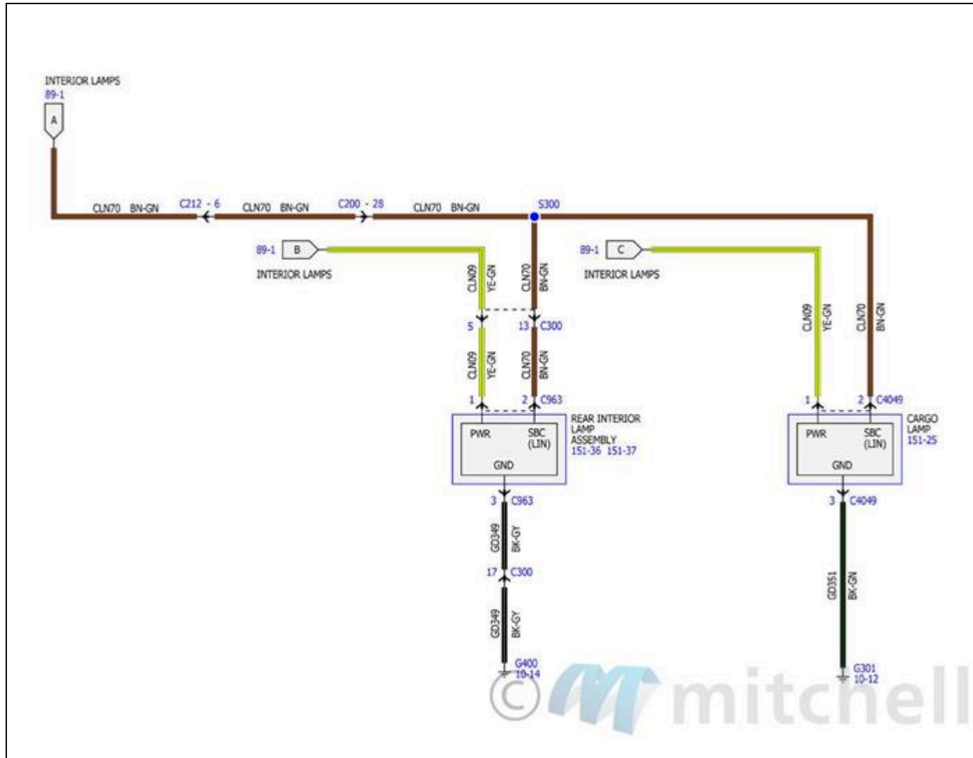
Fig. 99: Interior Lamps Wiring Diagrams (2 Of 4)
