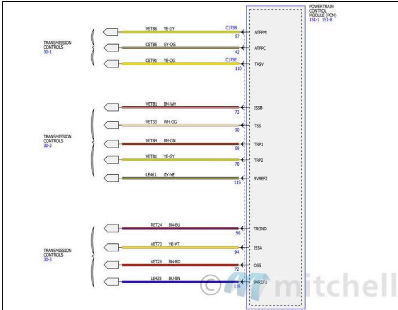
Fig. 59: Electronic Engine Controls Wiring Diagrams - 2.3L (17 Of 17)
