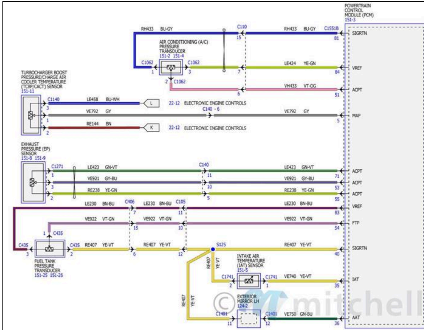
Fig. 68: Electronic Engine Controls Wiring Diagrams - 2.7L (9 Of 18)
