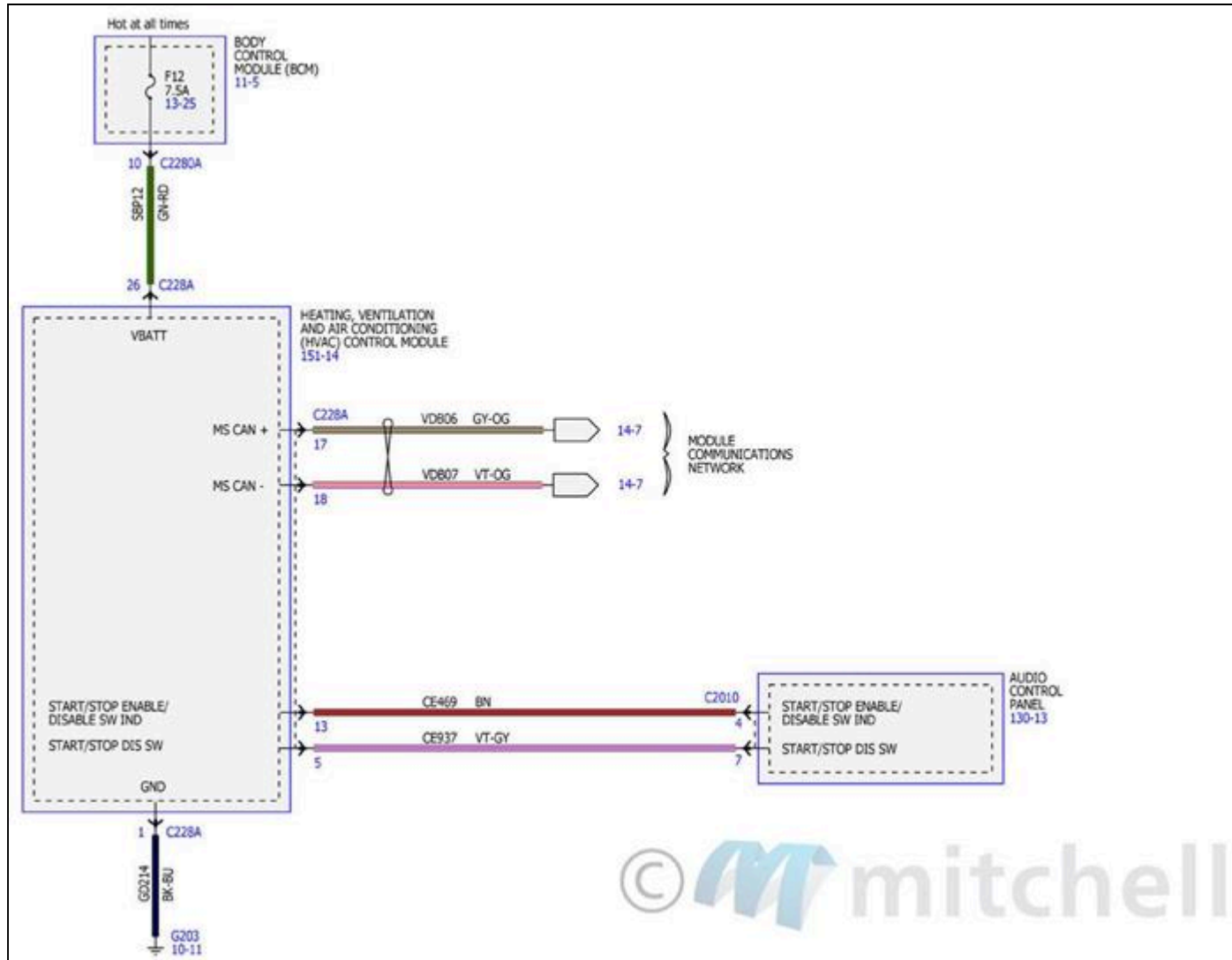
Fig. 102: Manual Climate Control System Wiring Diagrams (1 Of 5)
