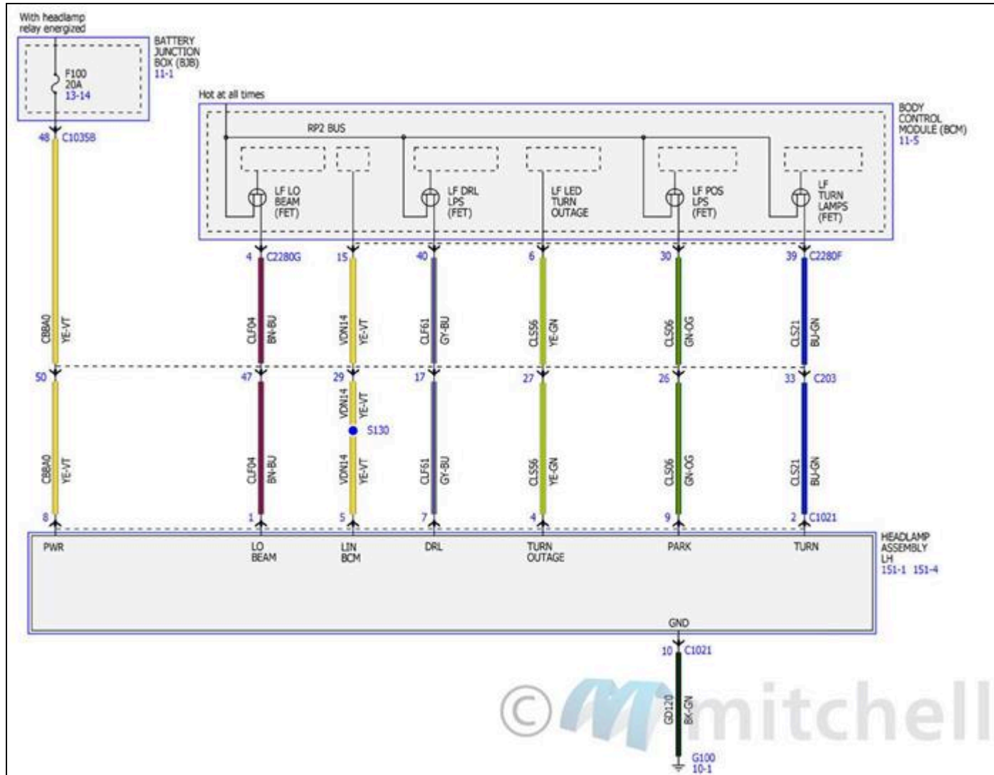
Fig. 86: Headlamps/Autolamps Wiring Diagrams (3 Of 4)
