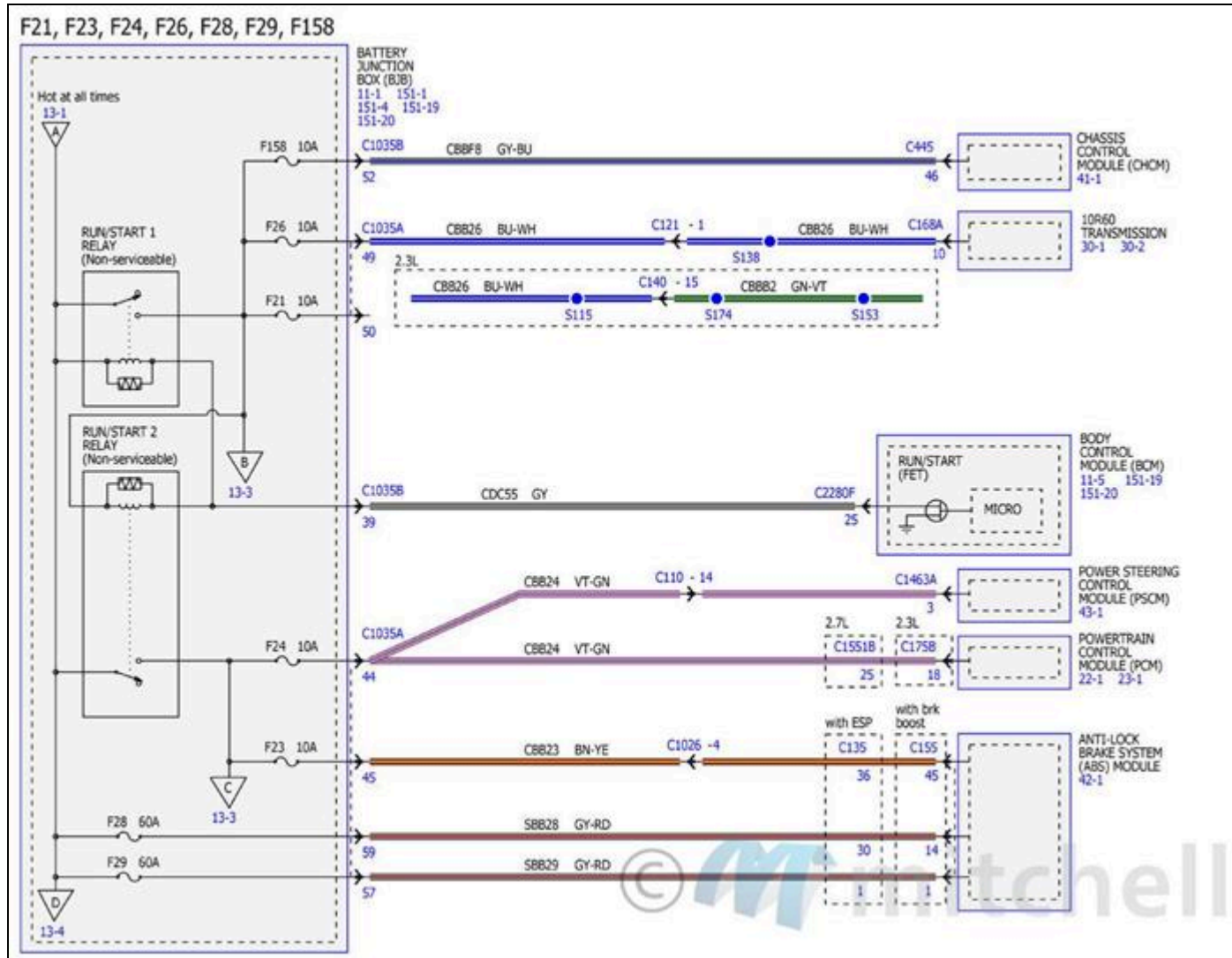
Fig. 131: Power Distribution/BCM Wiring Diagrams (2 Of 34)
