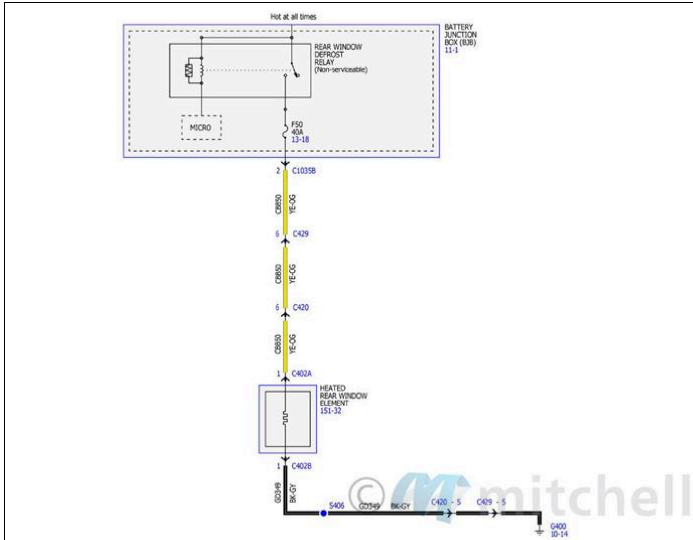
Fig. 88: Heated Window Wiring Diagram
