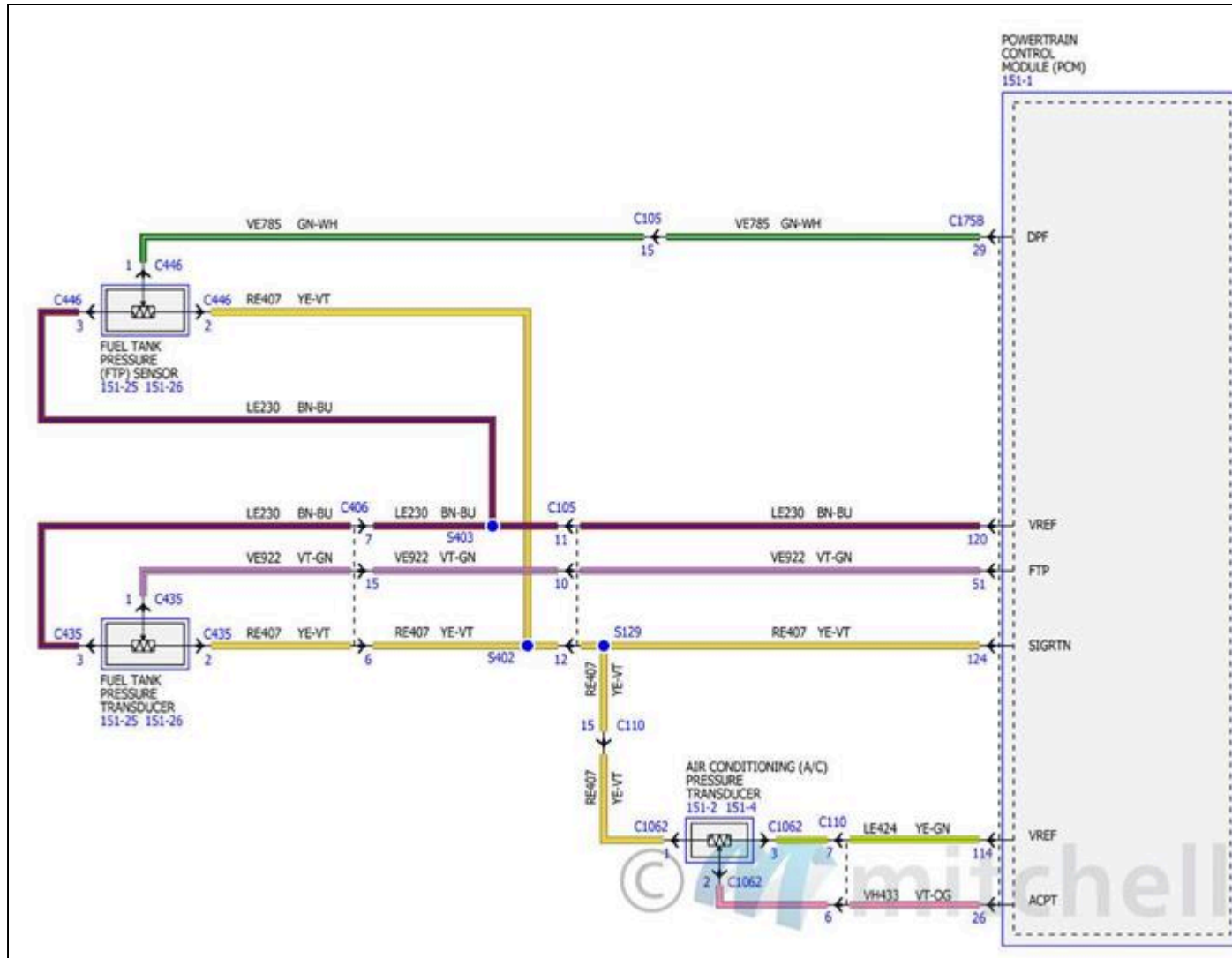
Fig. 53: Electronic Engine Controls Wiring Diagrams - 2.3L (11 Of 17)
