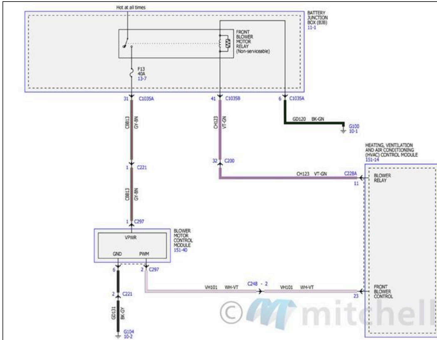
Fig. 103: Manual Climate Control System Wiring Diagrams (2 Of 5)
