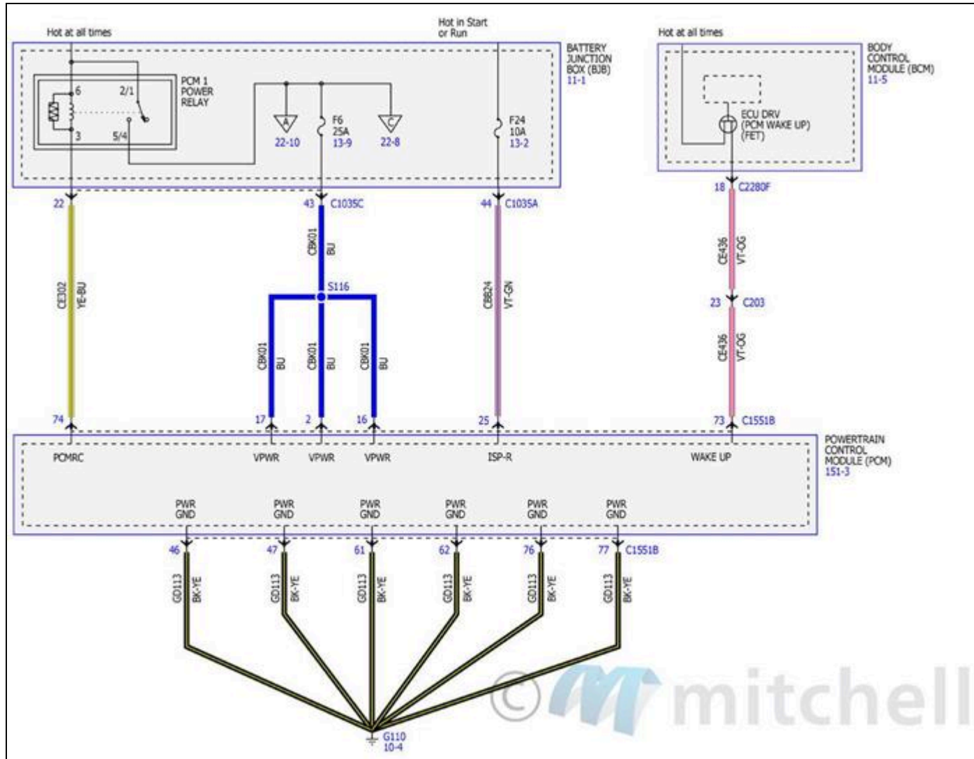
Fig. 60: Electronic Engine Controls Wiring Diagrams - 2.7L (1 Of 18)
