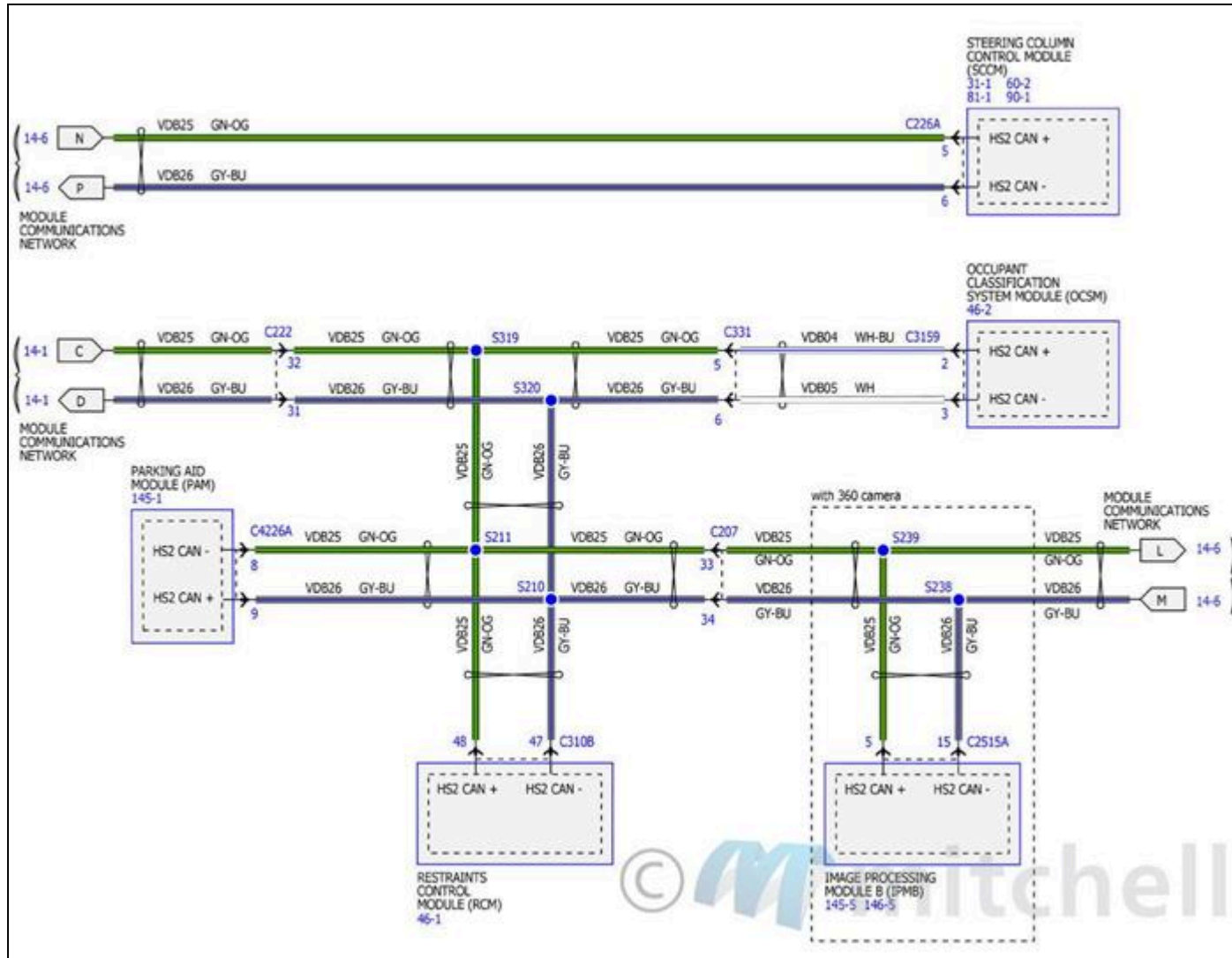
Fig. 111: Module Communications Network Wiring Diagrams (5 Of 8)
