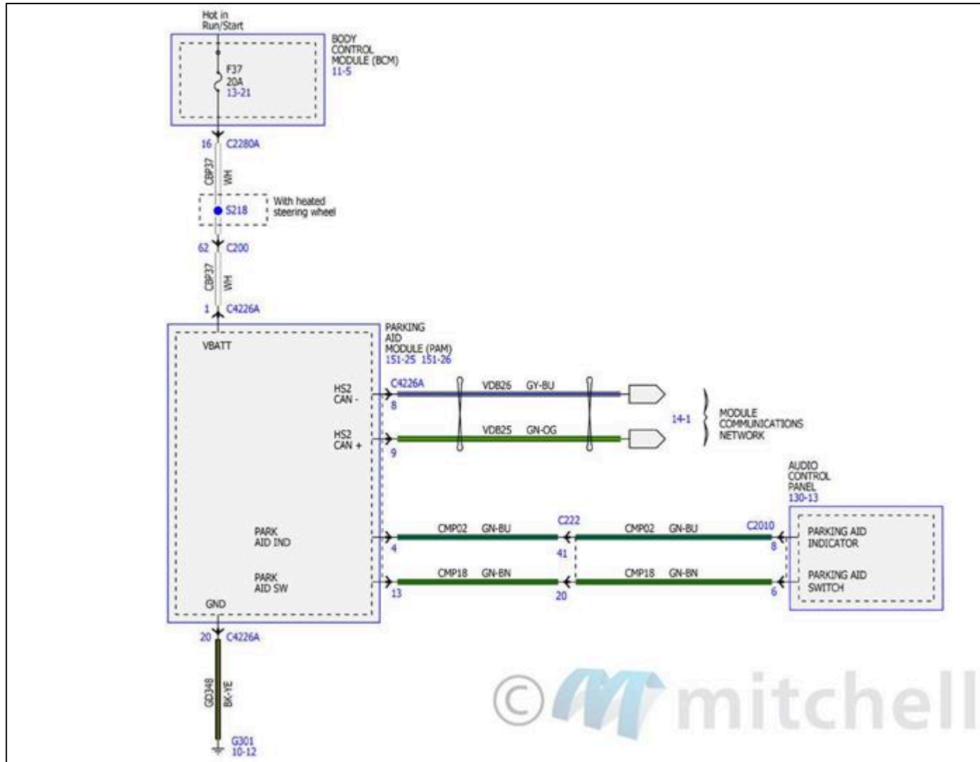
Fig. 115: Parking Aid Wiring Diagrams (1 Of 6)
