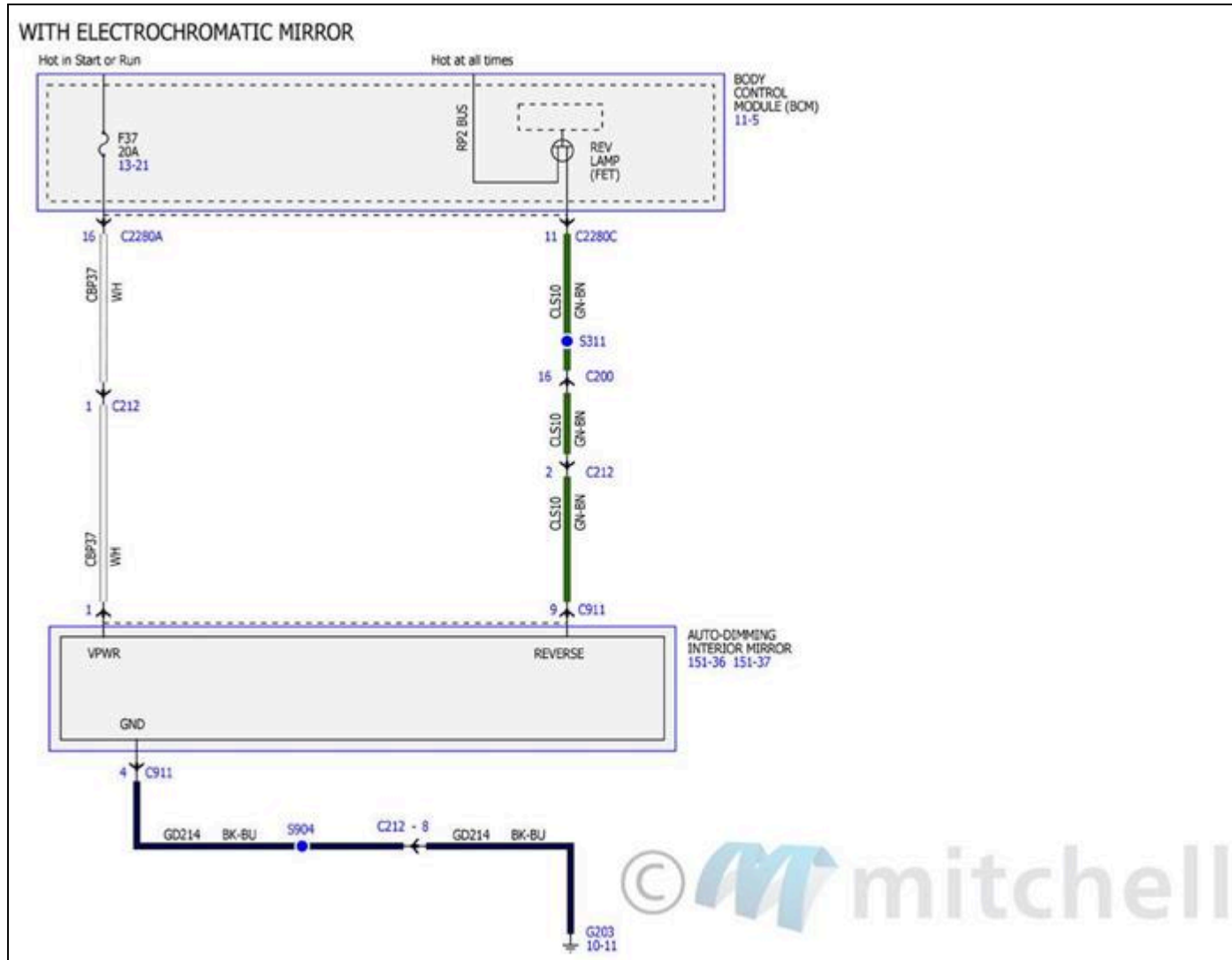
Fig. 167: Power Mirrors Wiring Diagrams (4 Of 4)
