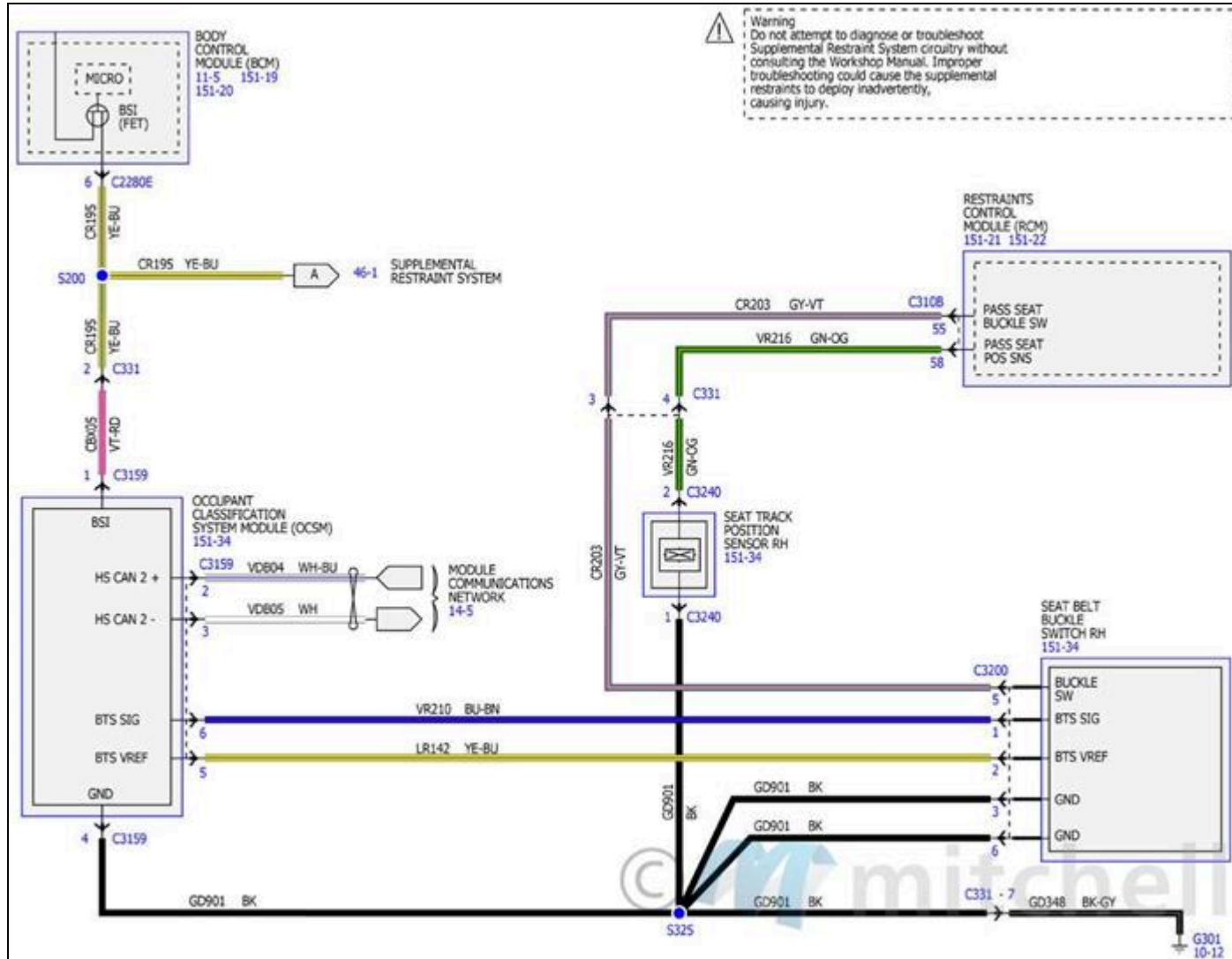
Fig. 190: Supplemental Restraint System Wiring Diagrams (2 Of 8)
