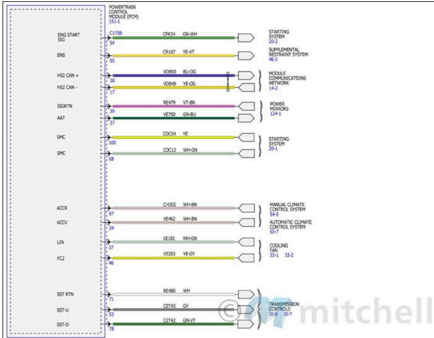
Fig. 58: Electronic Engine Controls Wiring Diagrams - 2.3L (16 Of 17)
