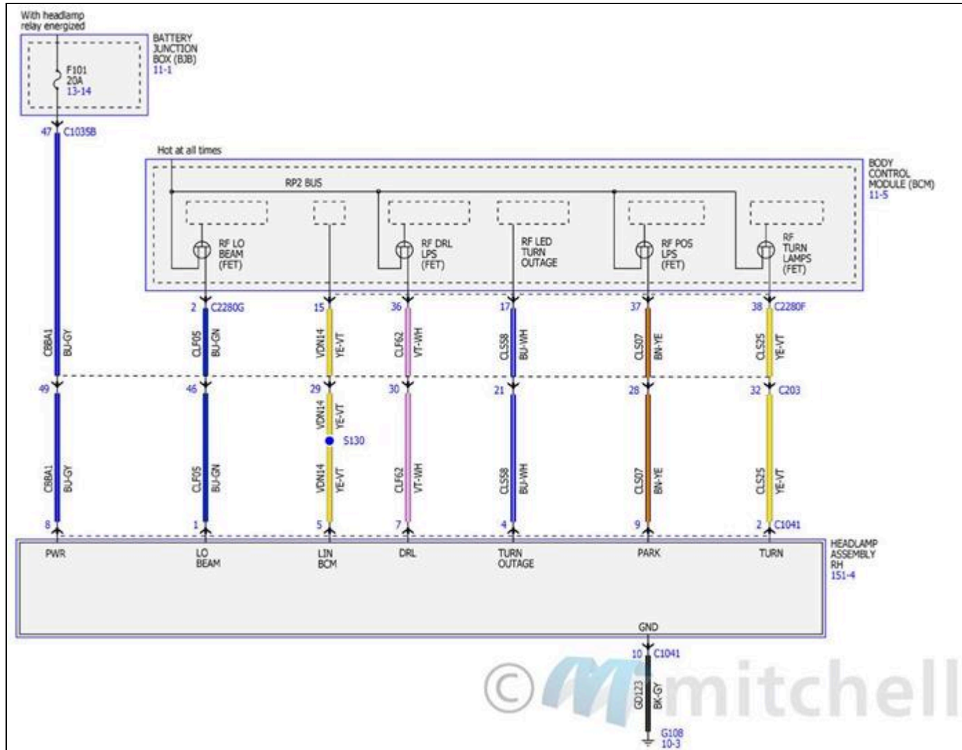
Fig. 87: Headlamps/Autolamps Wiring Diagrams (4 Of 4)
