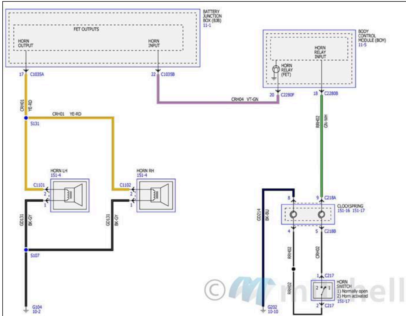
Fig. 89: Horn/Cigar Lighter Wiring Diagrams (1 Of 5)
