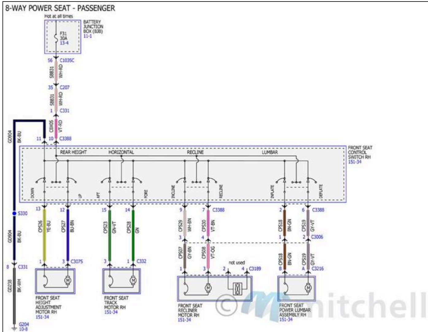
Fig. 169: Power Seats Wiring Diagrams (2 Of 2)
