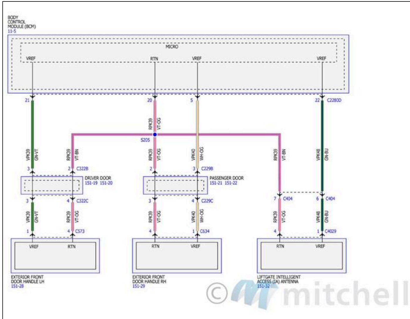
Fig. 129: Passive Anti-Theft System Wiring Diagrams (3 Of 3)
