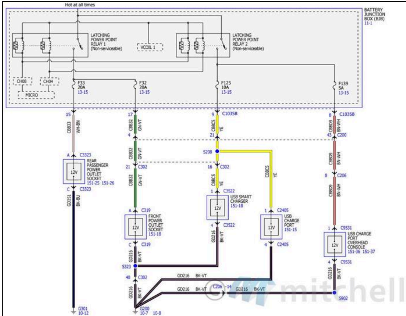
Fig. 90: Horn/Cigar Lighter Wiring Diagrams (2 Of 5)
