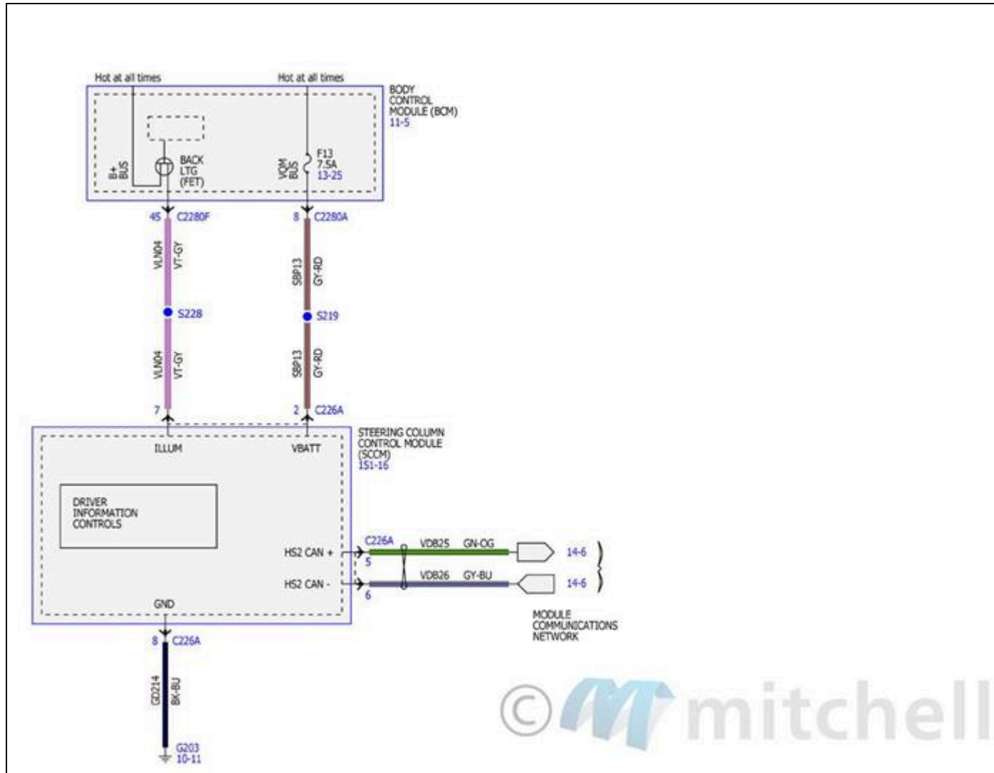
Fig. 95: Instrument Cluster Wiring Diagrams (2 Of 4)
