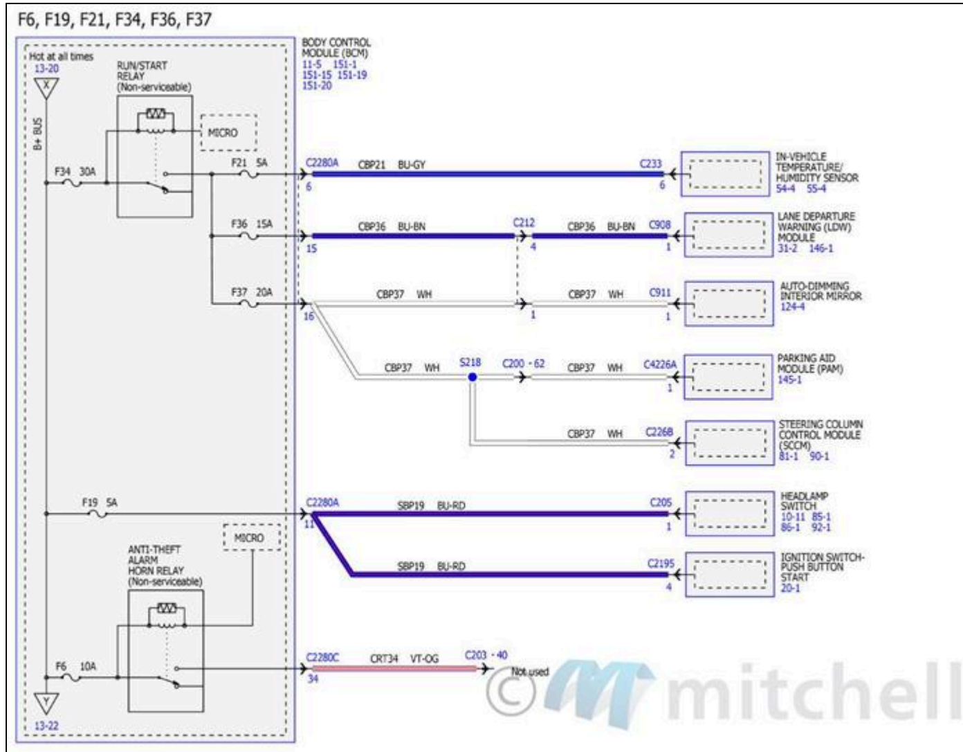
Fig. 150: Power Distribution/BCM Wiring Diagrams (21 Of 34)
