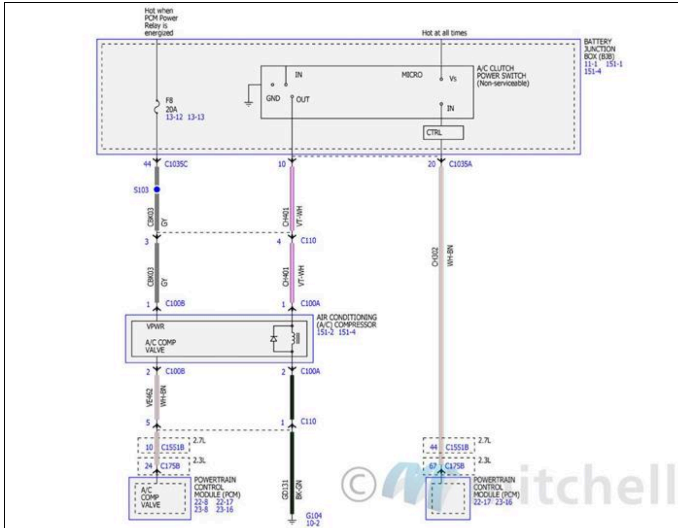
Fig. 106: Manual Climate Control System Wiring Diagrams (5 Of 5)
