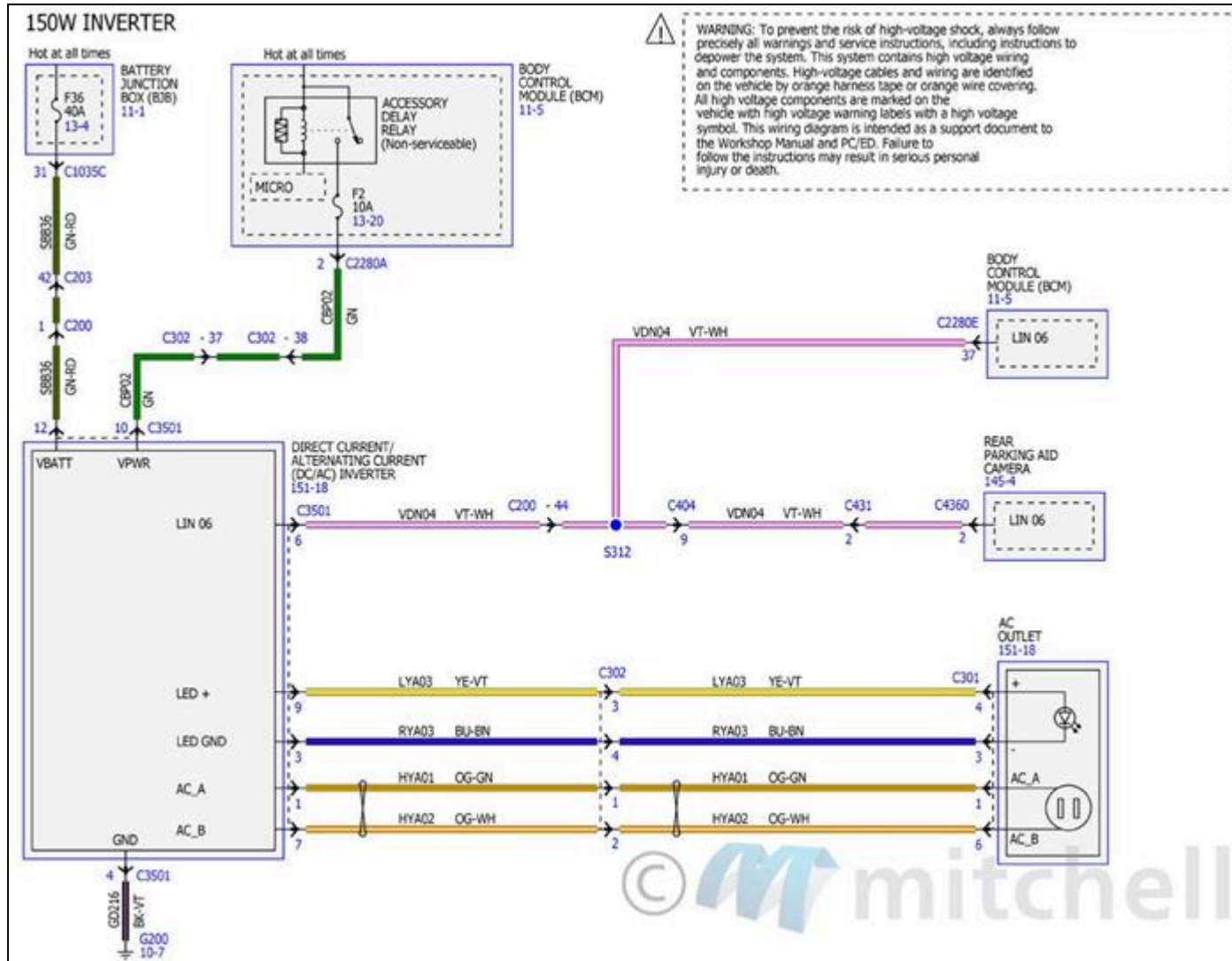
Fig. 91: Horn/Cigar Lighter Wiring Diagrams (3 Of 5)
