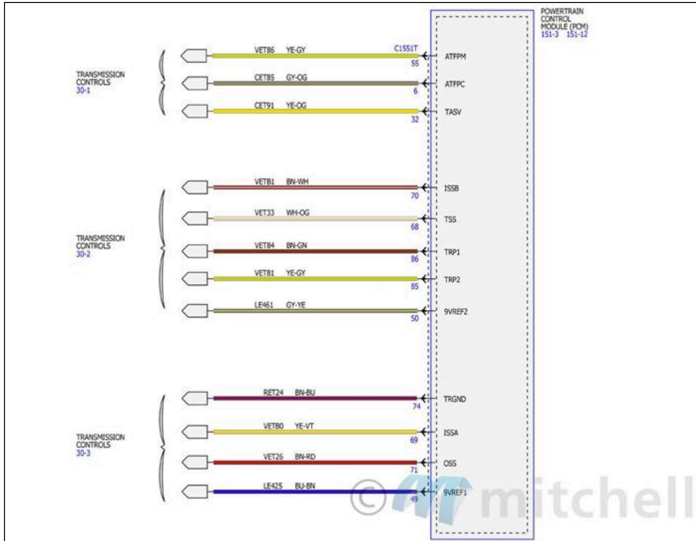
Fig. 76: Electronic Engine Controls Wiring Diagrams - 2.7L (17 Of 18)
