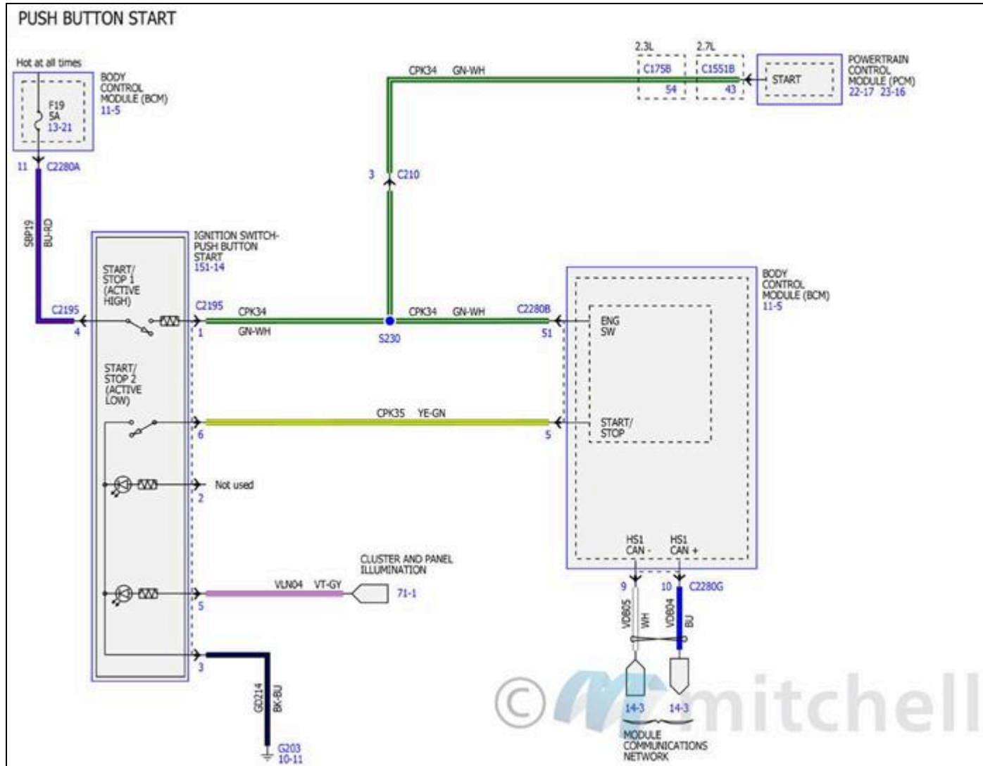
Fig. 187: Starting System Wiring Diagrams (1 Of 2)
