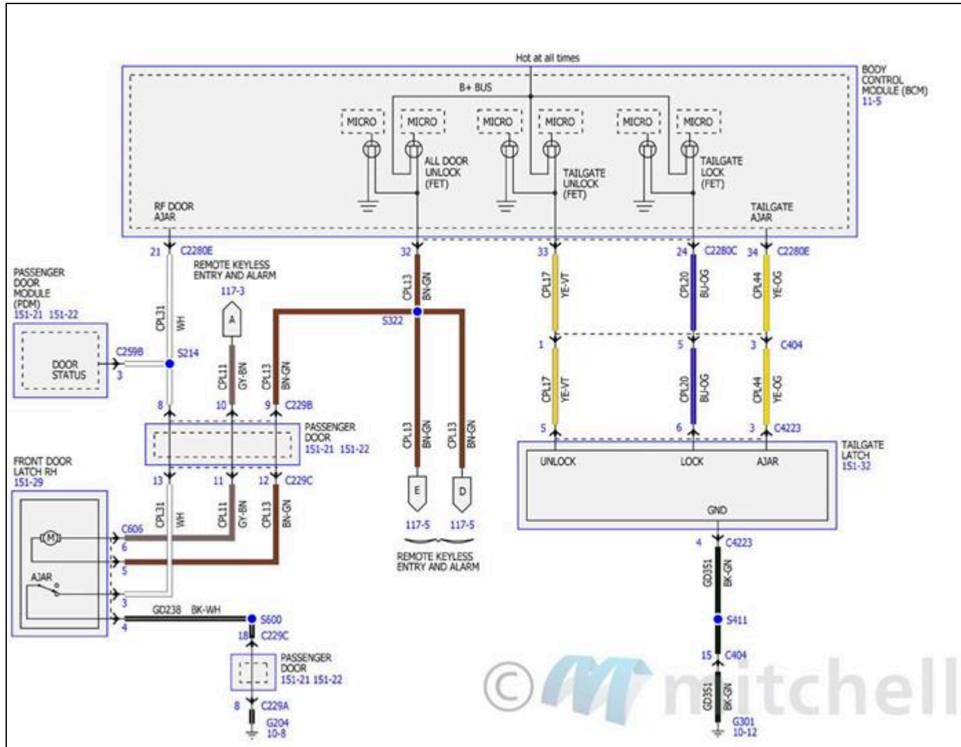
Fig. 180: Remote Keyless Entry and Alarm Wiring Diagrams (4 Of 8)
