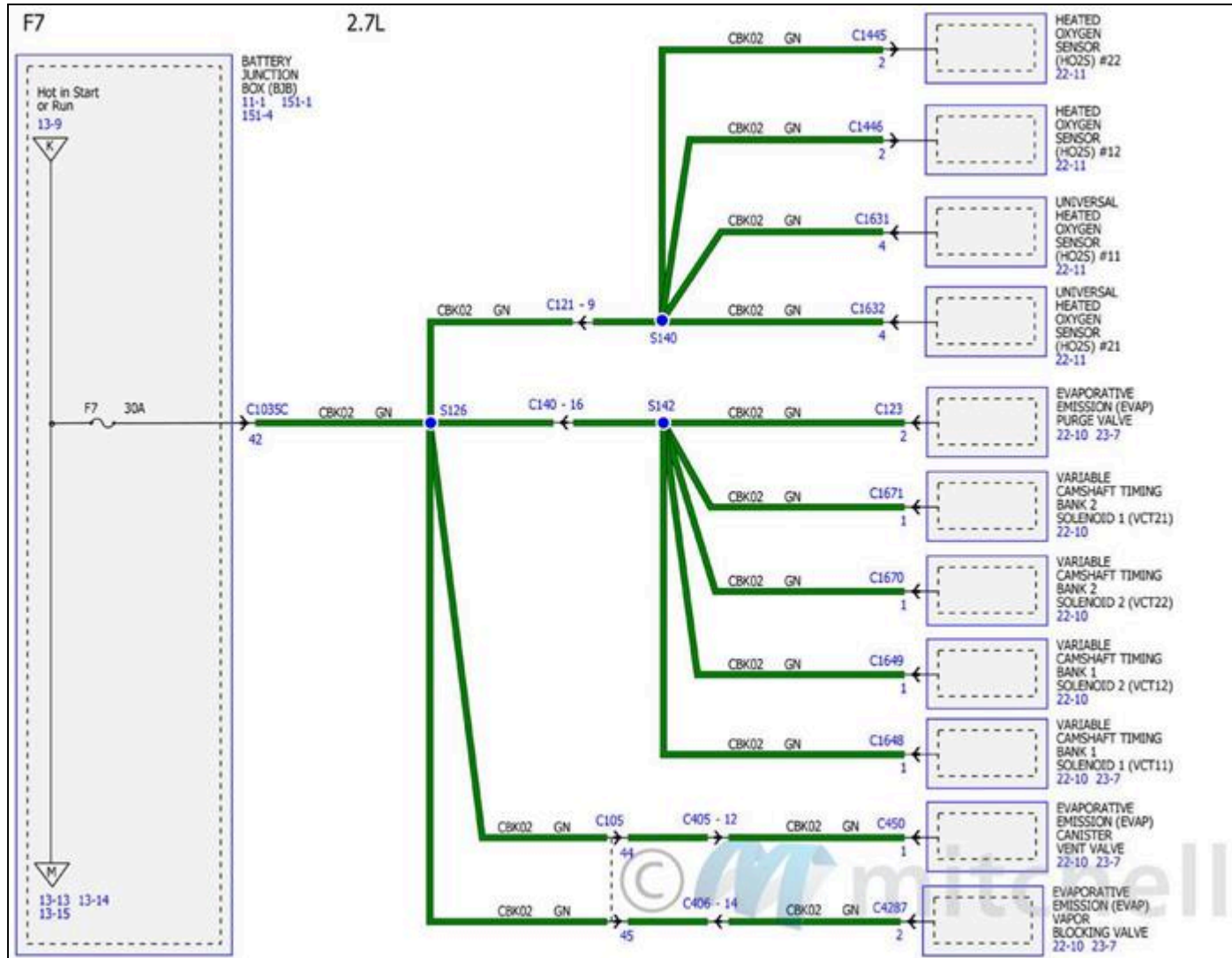
Fig. 140: Power Distribution/BCM Wiring Diagrams (11 Of 34)
