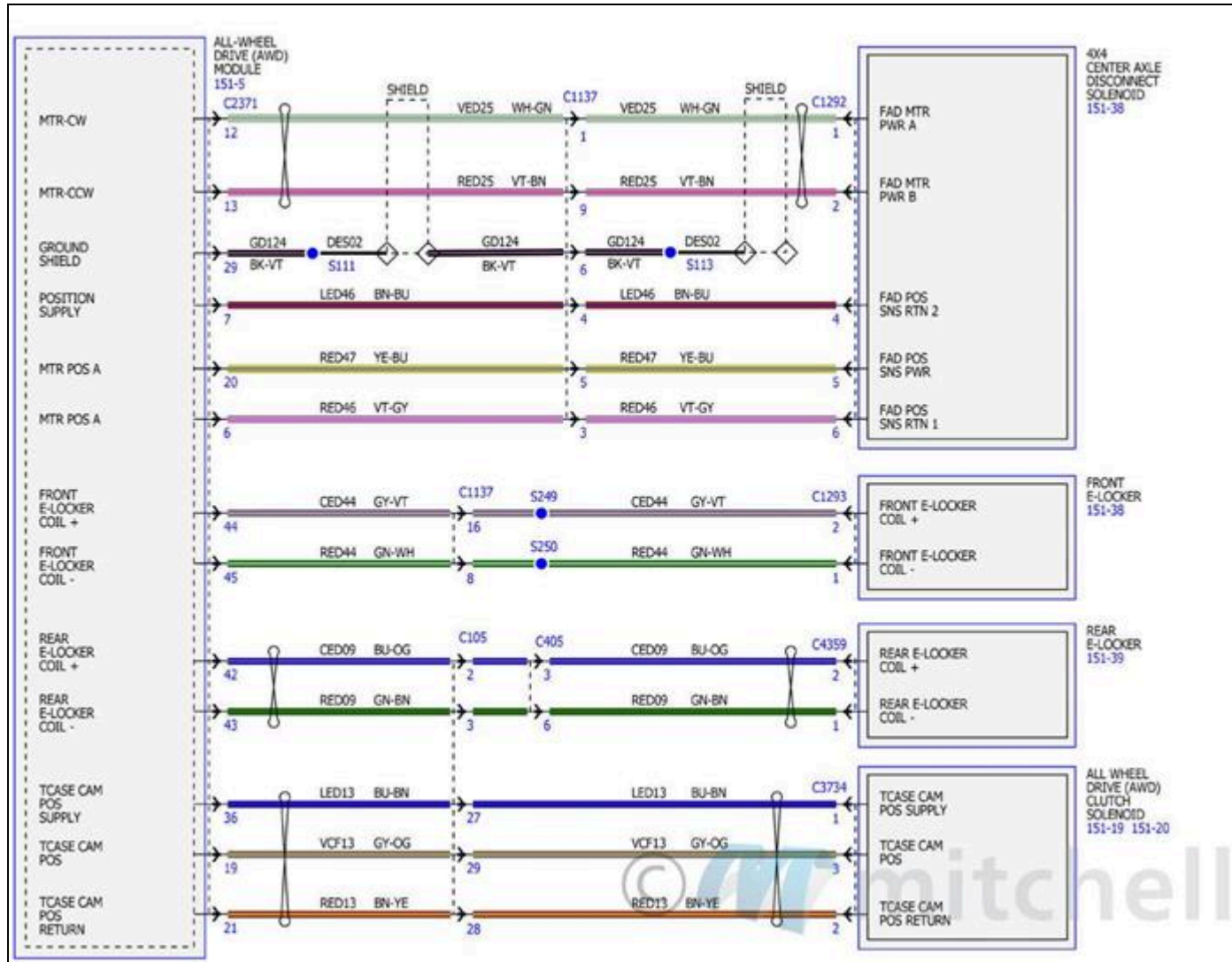
Fig. 83: Four Wheel Drive Systems Wiring Diagrams (4 Of 4)
