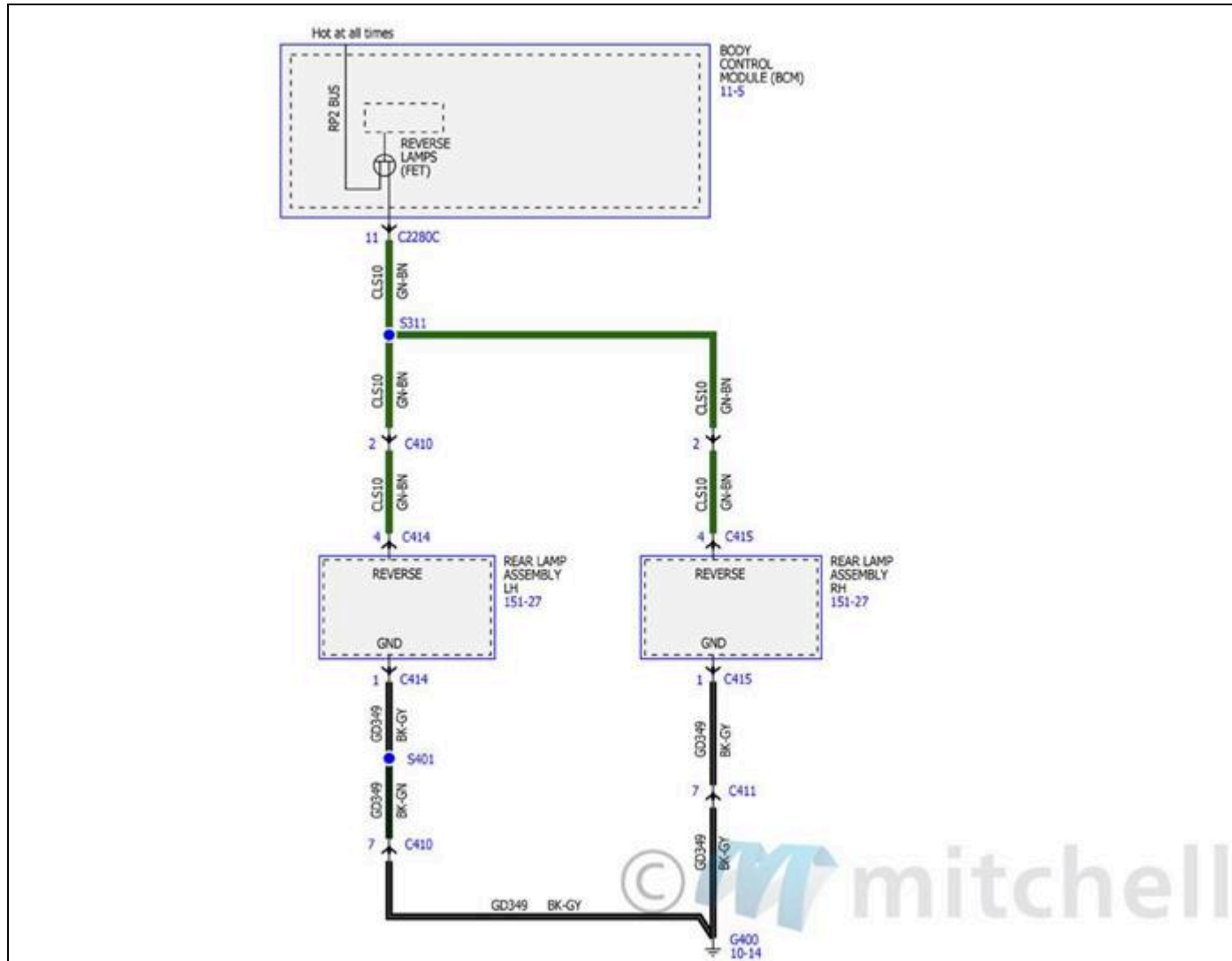
Fig. 185: Reversing Lamps Wiring Diagram
