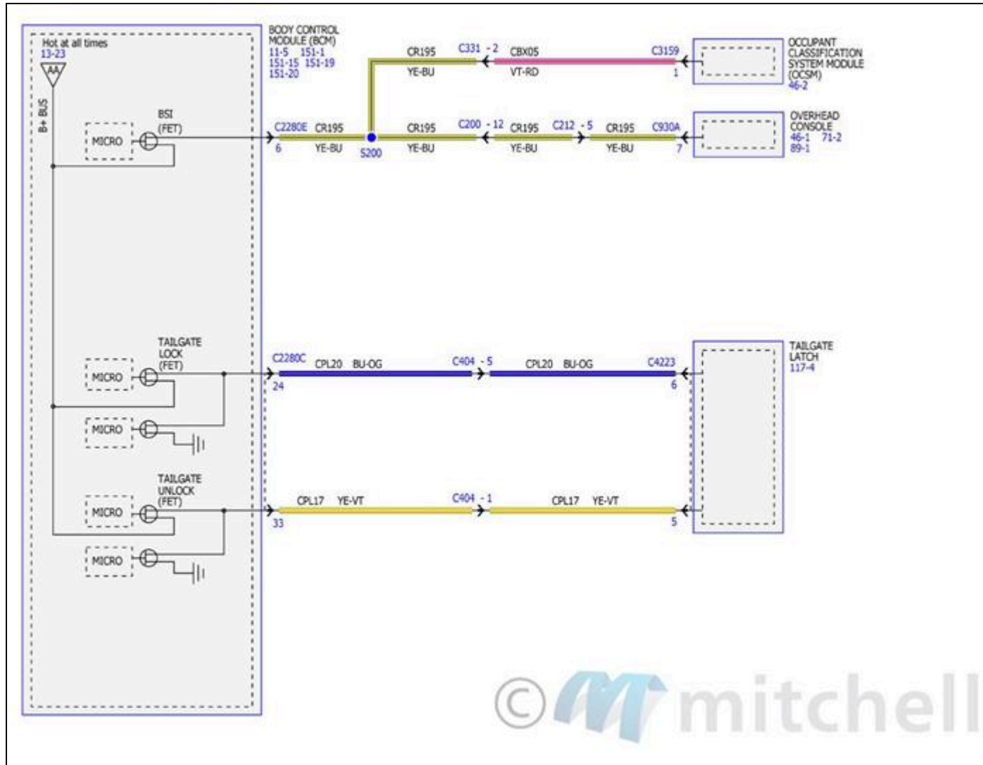
Fig. 153: Power Distribution/BCM Wiring Diagrams (24 Of 34)
