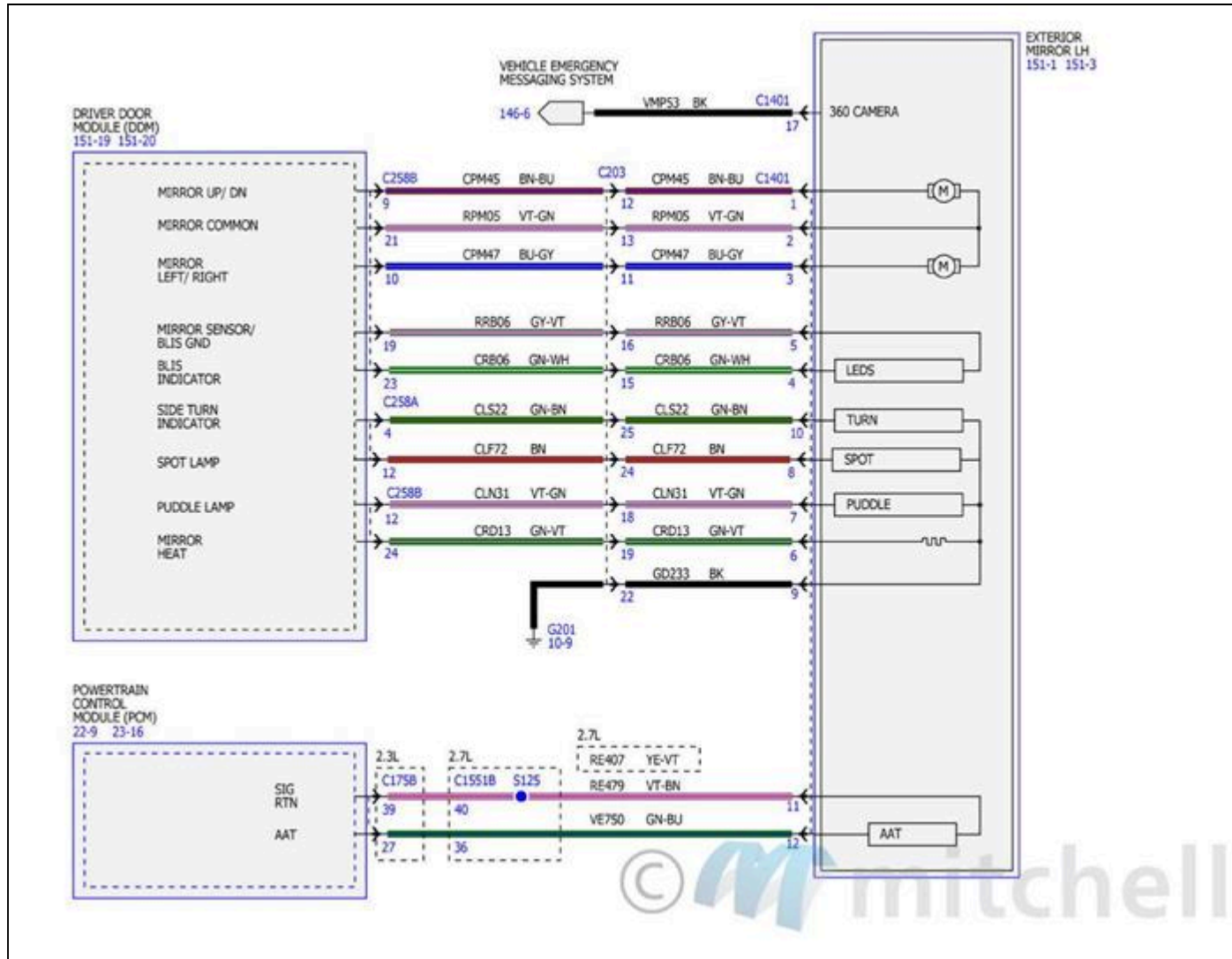
Fig. 165: Power Mirrors Wiring Diagrams (2 Of 4)
