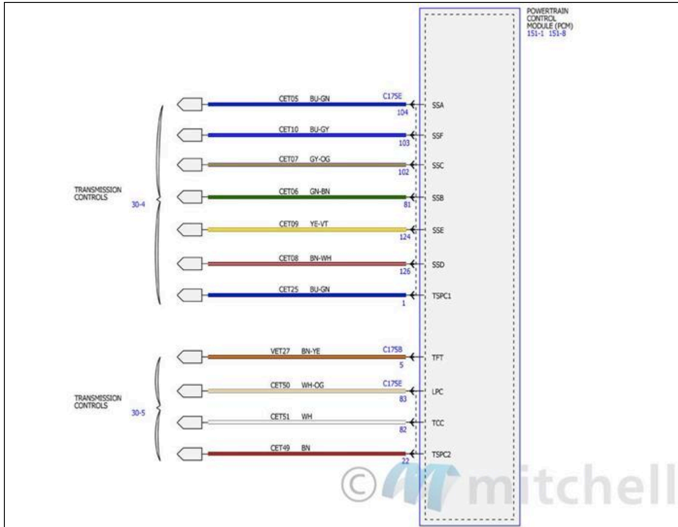
Fig. 57: Electronic Engine Controls Wiring Diagrams - 2.3L (15 Of 17)
