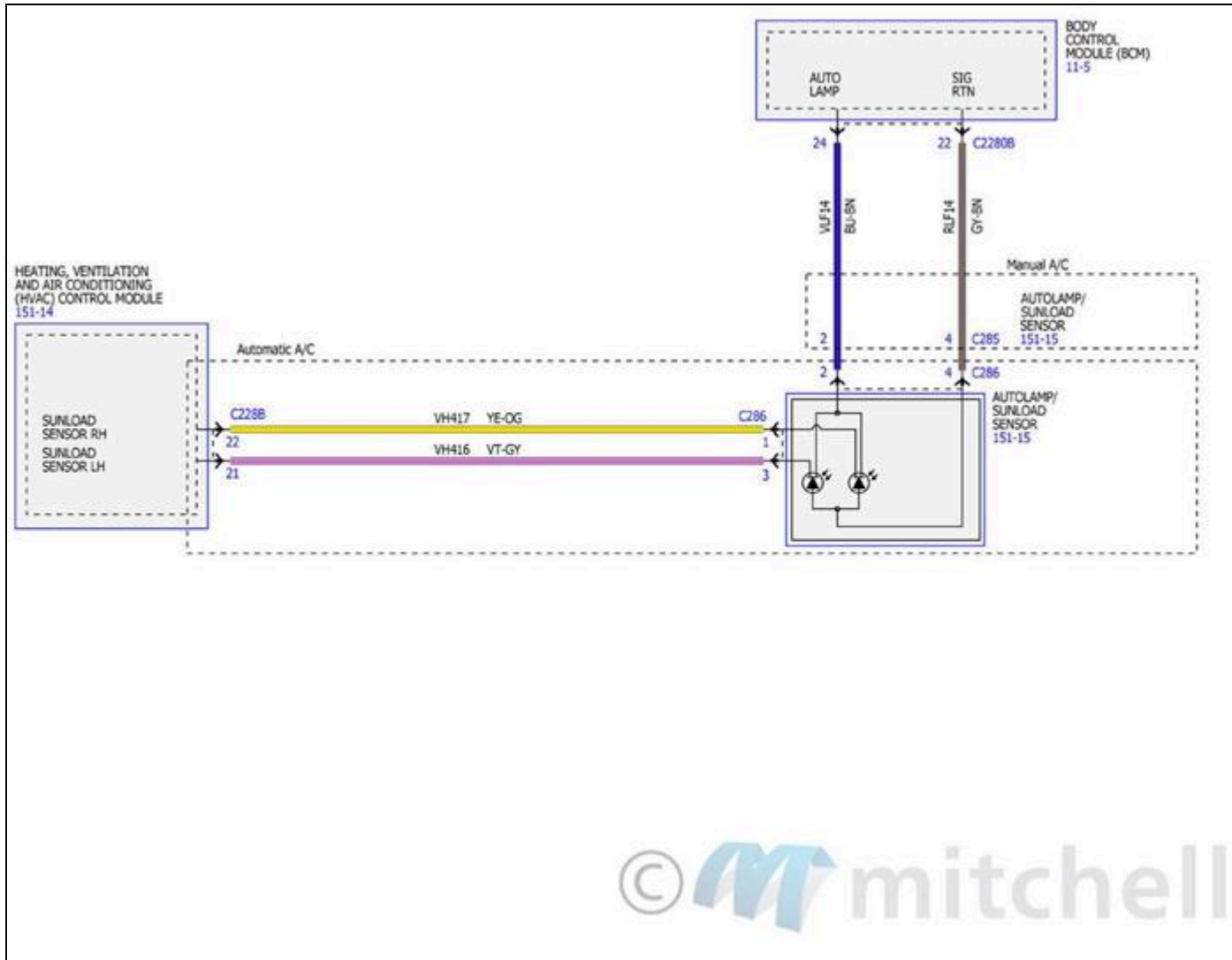
Fig. 85: Headlamps/Autolamps Wiring Diagrams (2 Of 4)
