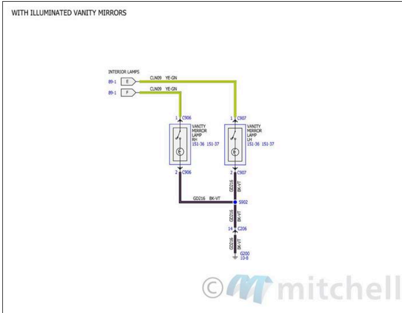
Fig. 101: Interior Lamps Wiring Diagrams (4 Of 4)
