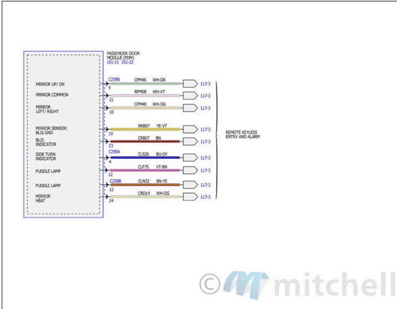
Fig. 176: Power Windows Wiring Diagrams (6 Of 6)
