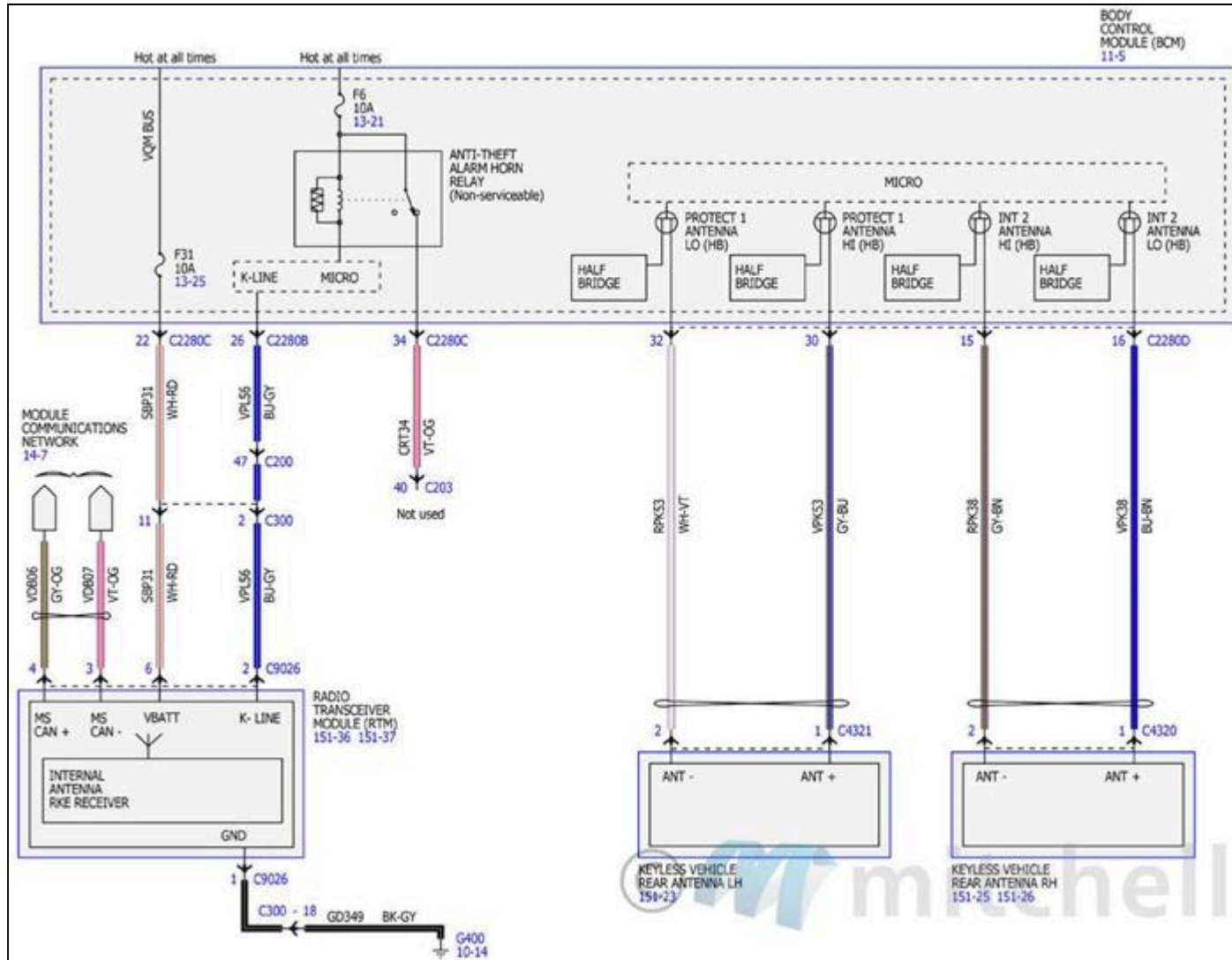
Fig. 183: Remote Keyless Entry and Alarm Wiring Diagrams (7 Of 8)
