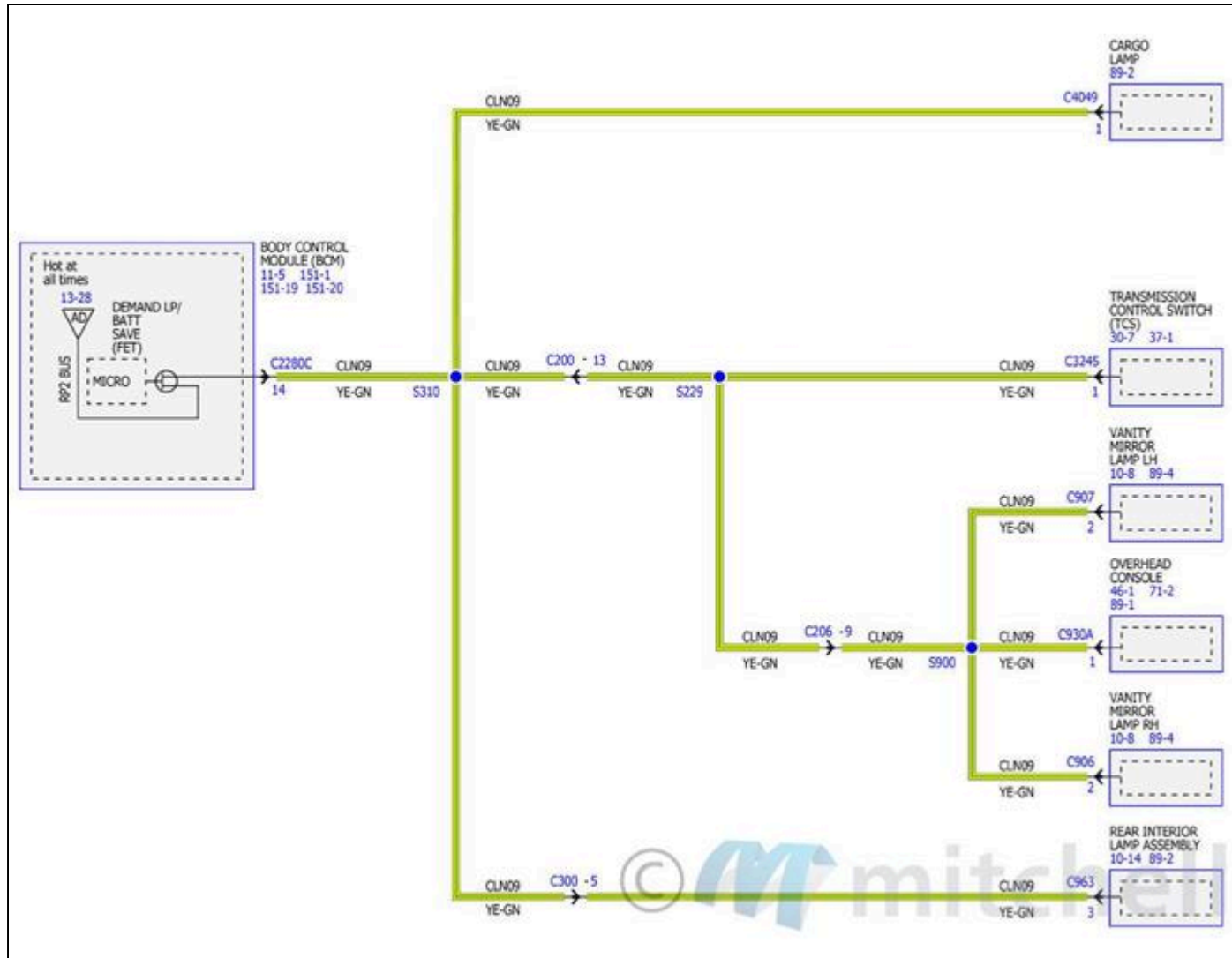
Fig. 158: Power Distribution/BCM Wiring Diagrams (29 Of 34)
