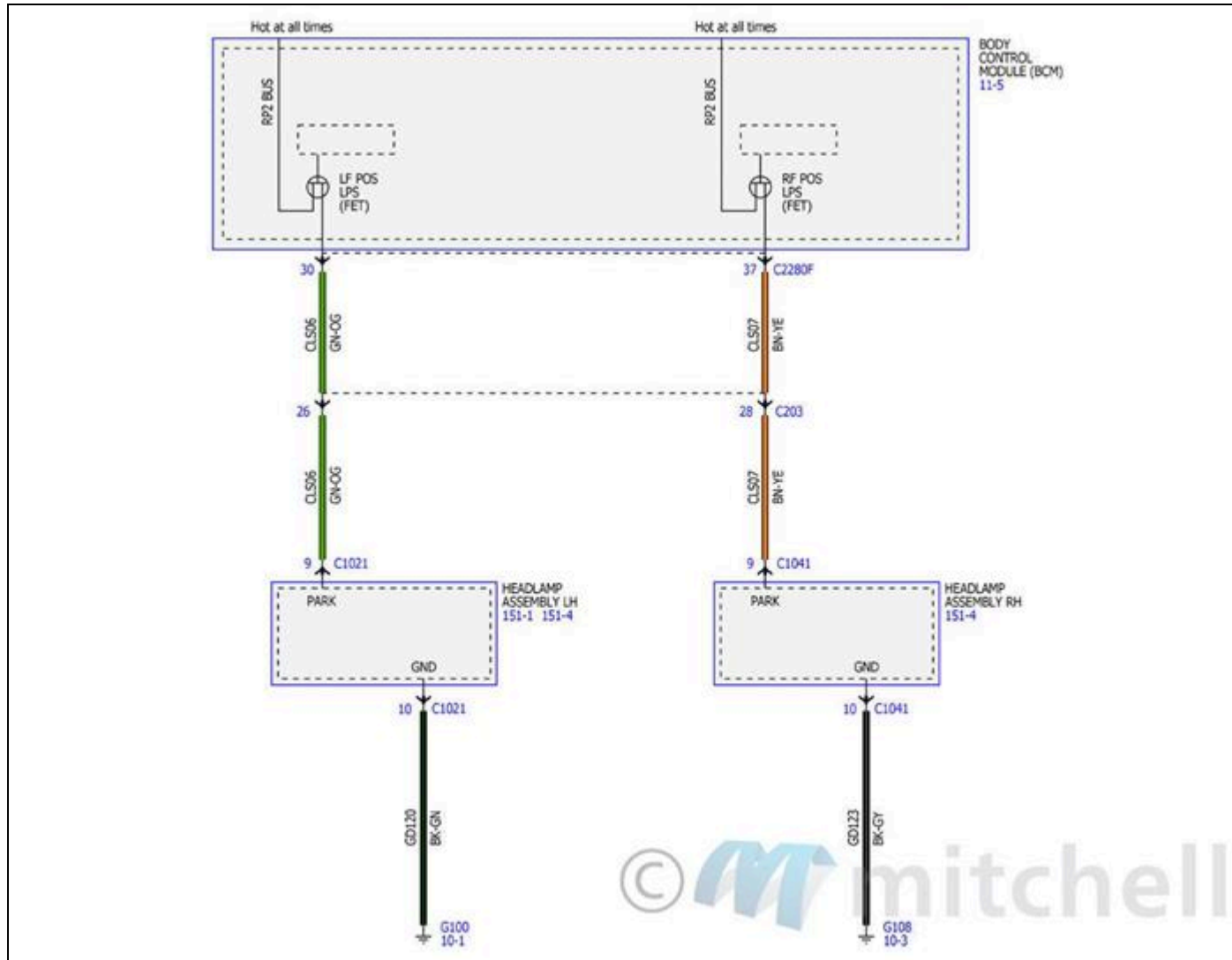
Fig. 122: Parking, Rear and License Lamps Wiring Diagrams (2 Of 6)
