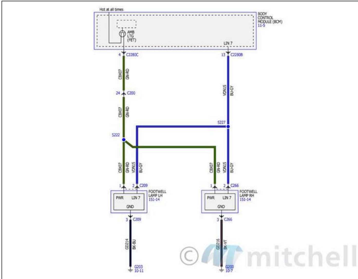
Fig. 100: Interior Lamps Wiring Diagrams (3 Of 4)
