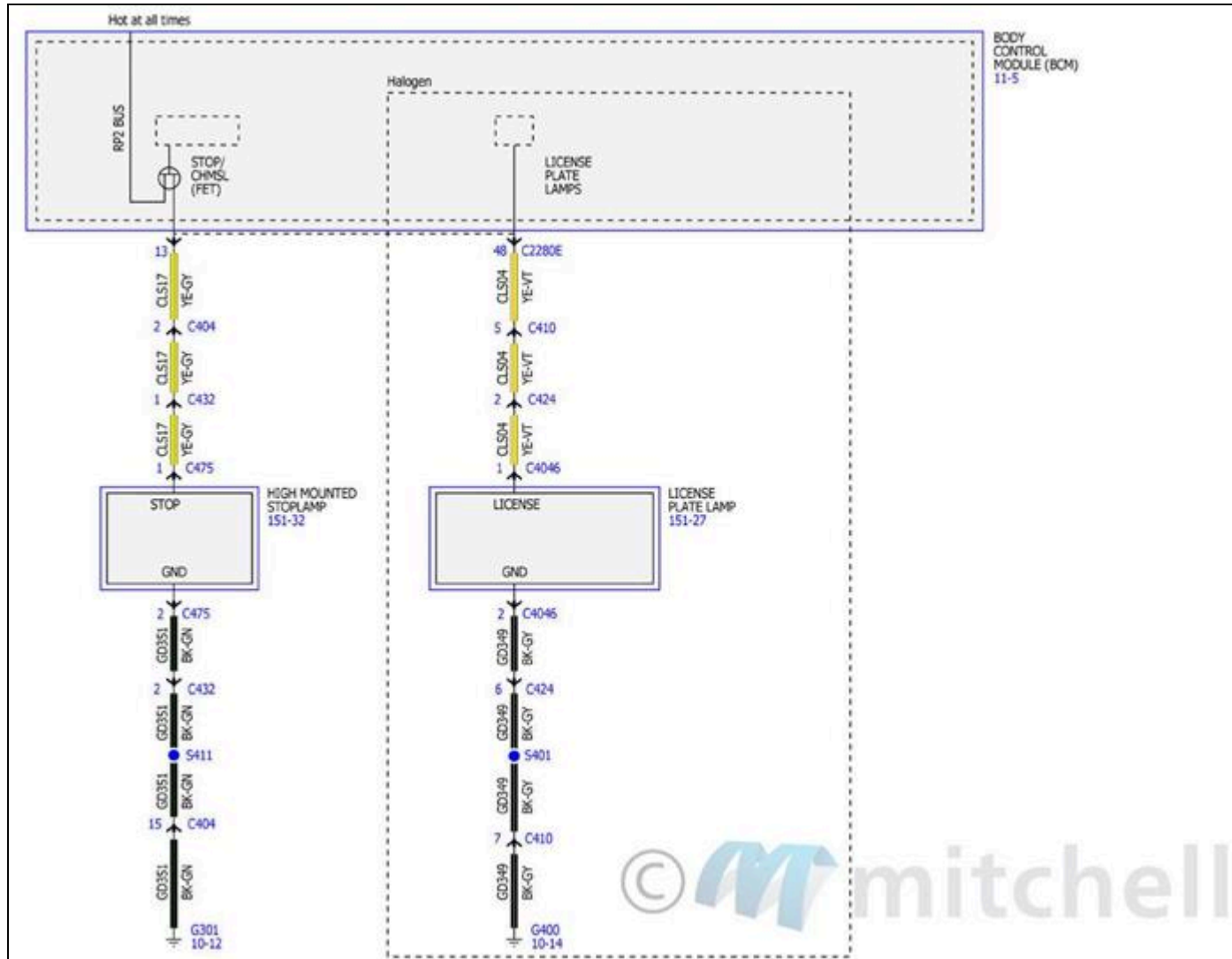
Fig. 126: Parking, Rear and License Lamps Wiring Diagrams (6 Of 6)
