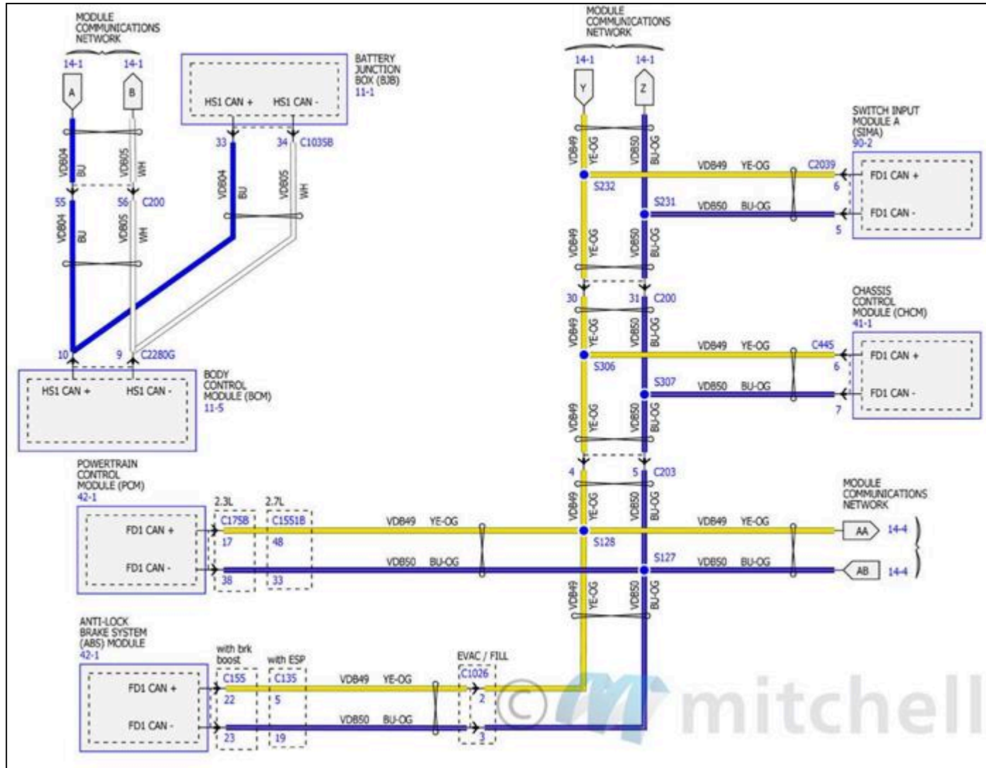
Fig. 109: Module Communications Network Wiring Diagrams (3 Of 8)
