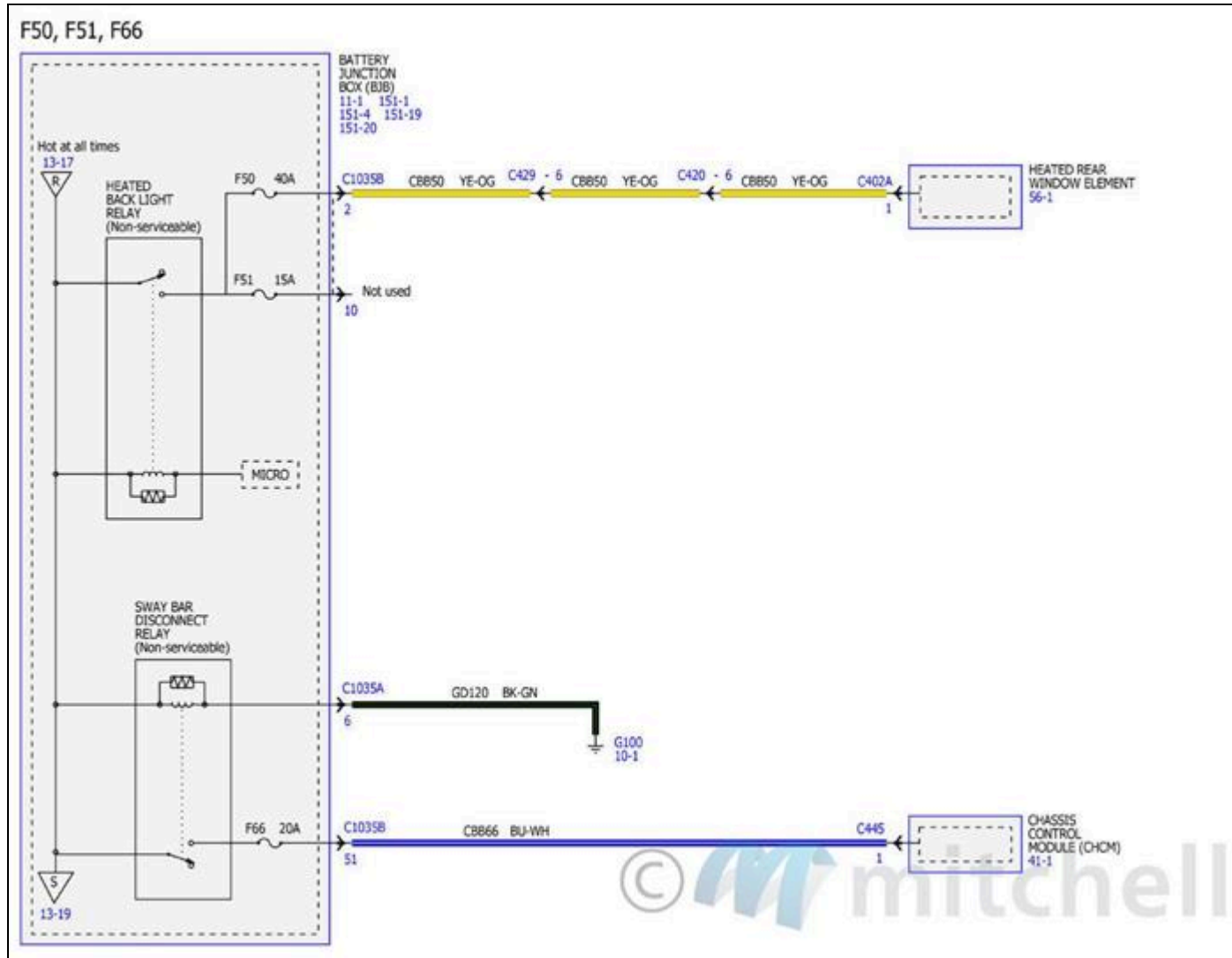
Fig. 147: Power Distribution/BCM Wiring Diagrams (18 Of 34)
