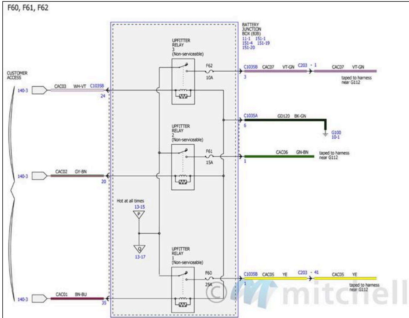
Fig. 145: Power Distribution/BCM Wiring Diagrams (16 Of 34)
