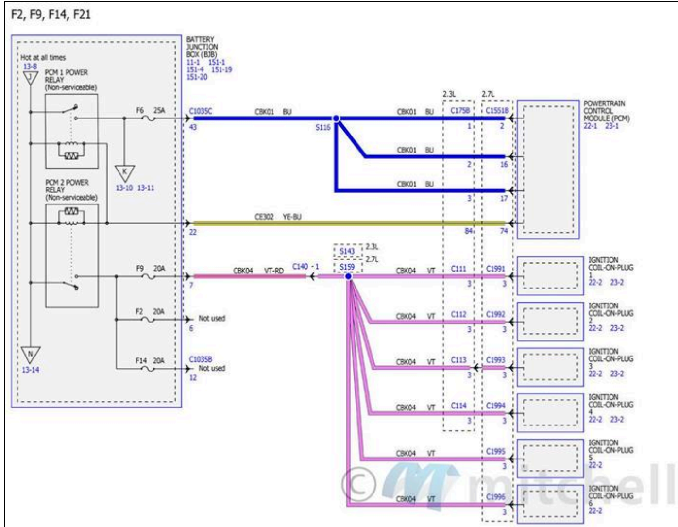
Fig. 138: Power Distribution/BCM Wiring Diagrams (9 Of 34)
