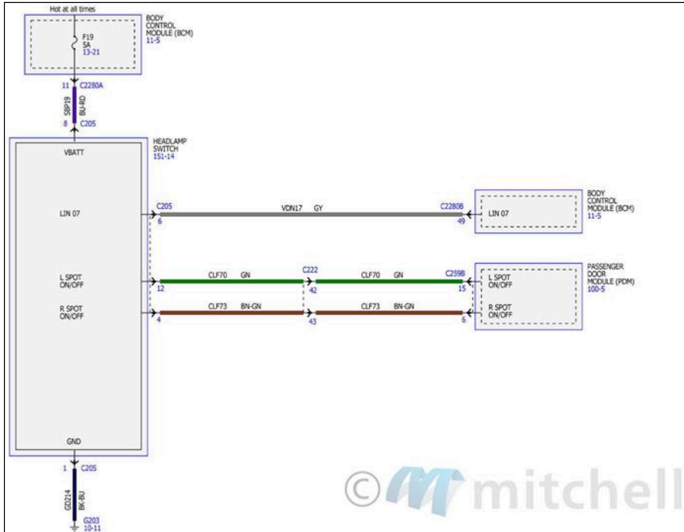
Fig. 121: Parking, Rear and License Lamps Wiring Diagrams (1 Of 6)
