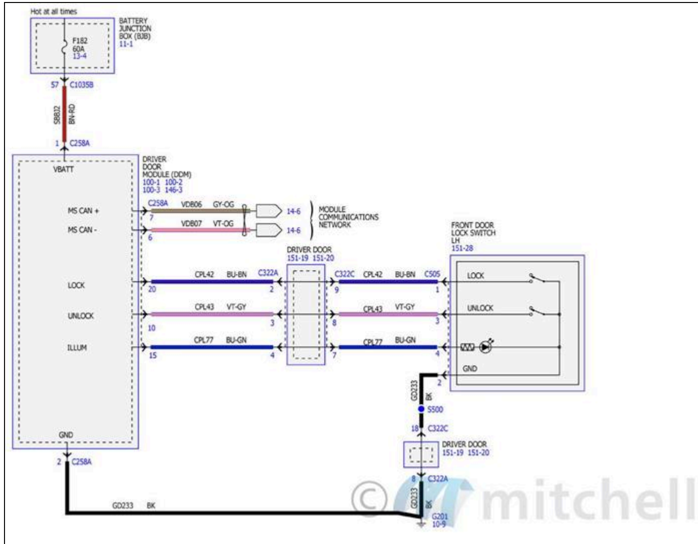
Fig. 177: Remote Keyless Entry and Alarm Wiring Diagrams (1 Of 8)
