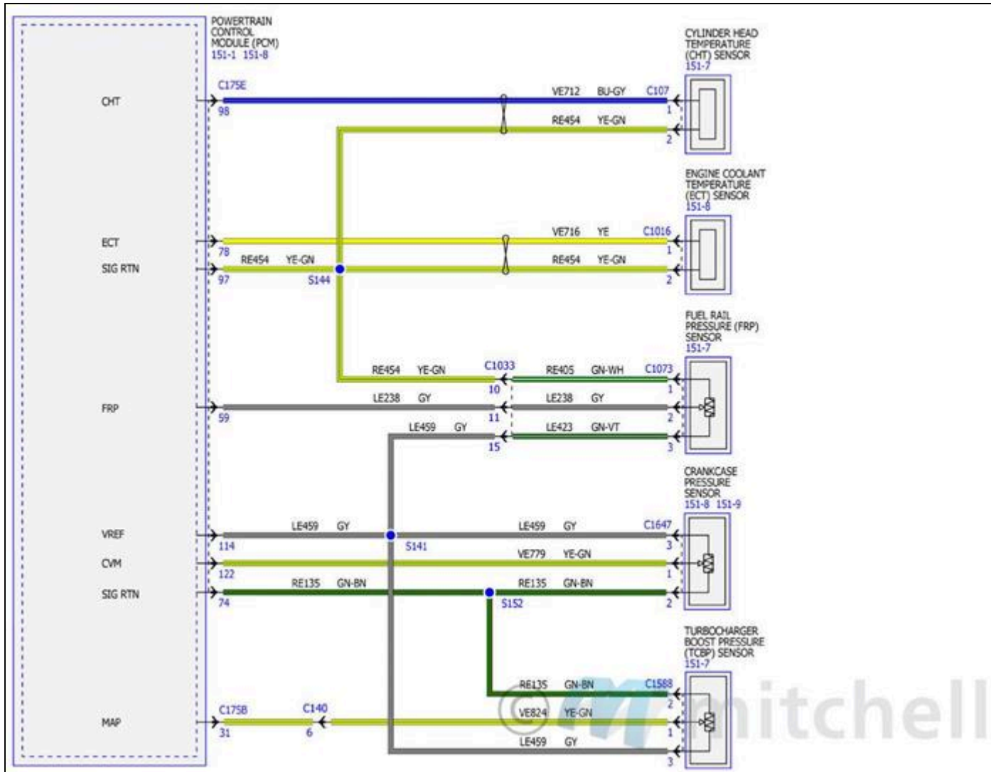
Fig. 51: Electronic Engine Controls Wiring Diagrams - 2.3L (9 Of 17)
