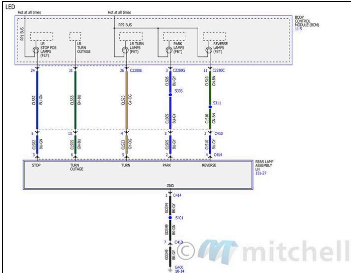
Fig. 124: Parking, Rear and License Lamps Wiring Diagrams (4 Of 6)
