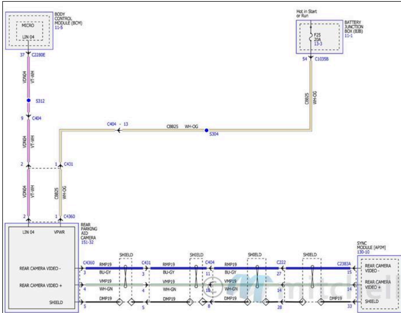
Fig. 118: Parking Aid Wiring Diagrams (4 Of 6)
