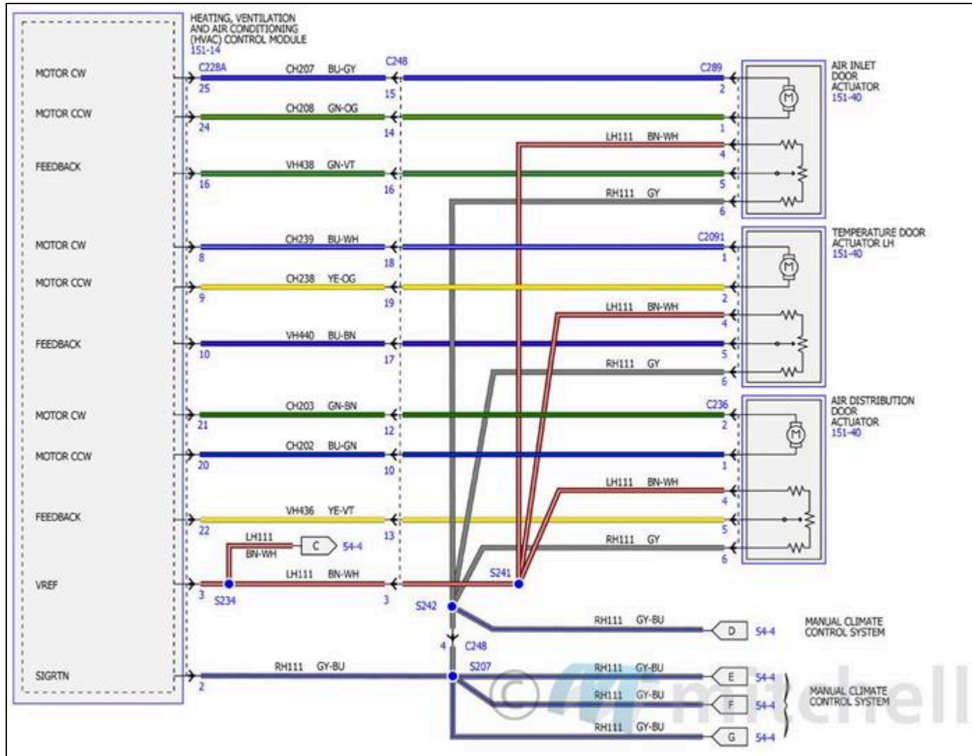
Fig. 104: Manual Climate Control System Wiring Diagrams (3 Of 5)
