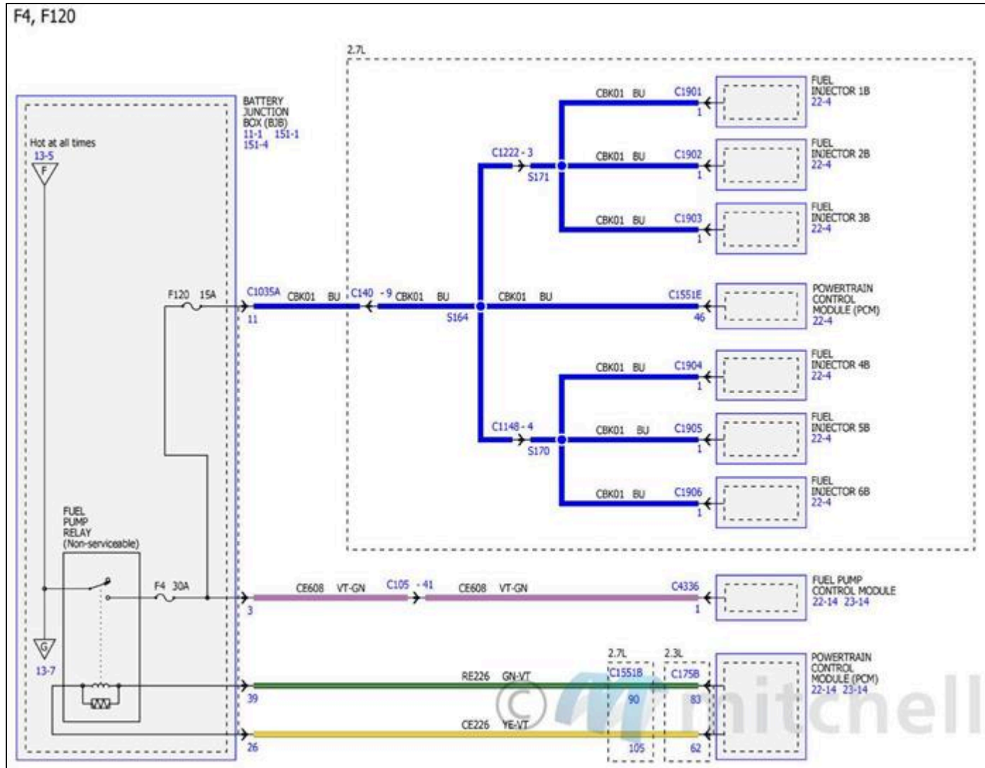
Fig. 135: Power Distribution/BCM Wiring Diagrams (6 Of 34)
