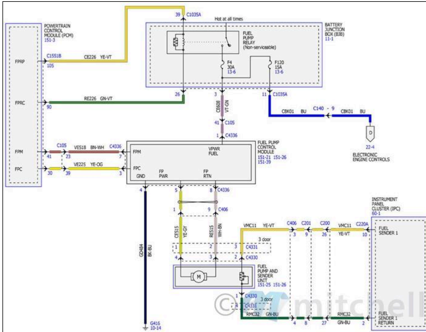
Fig. 73: Electronic Engine Controls Wiring Diagrams - 2.7L (14 Of 18)
