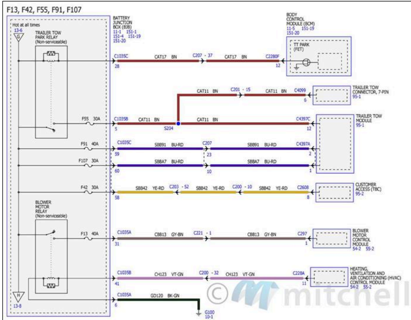
Fig. 136: Power Distribution/BCM Wiring Diagrams (7 Of 34)
