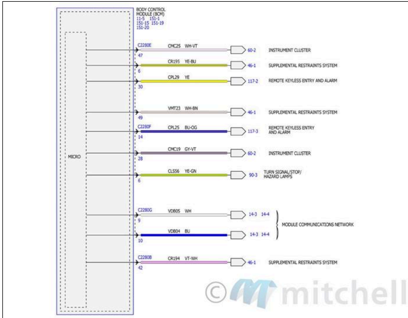
Fig. 163: Power Distribution/BCM Wiring Diagrams (34 Of 34)
