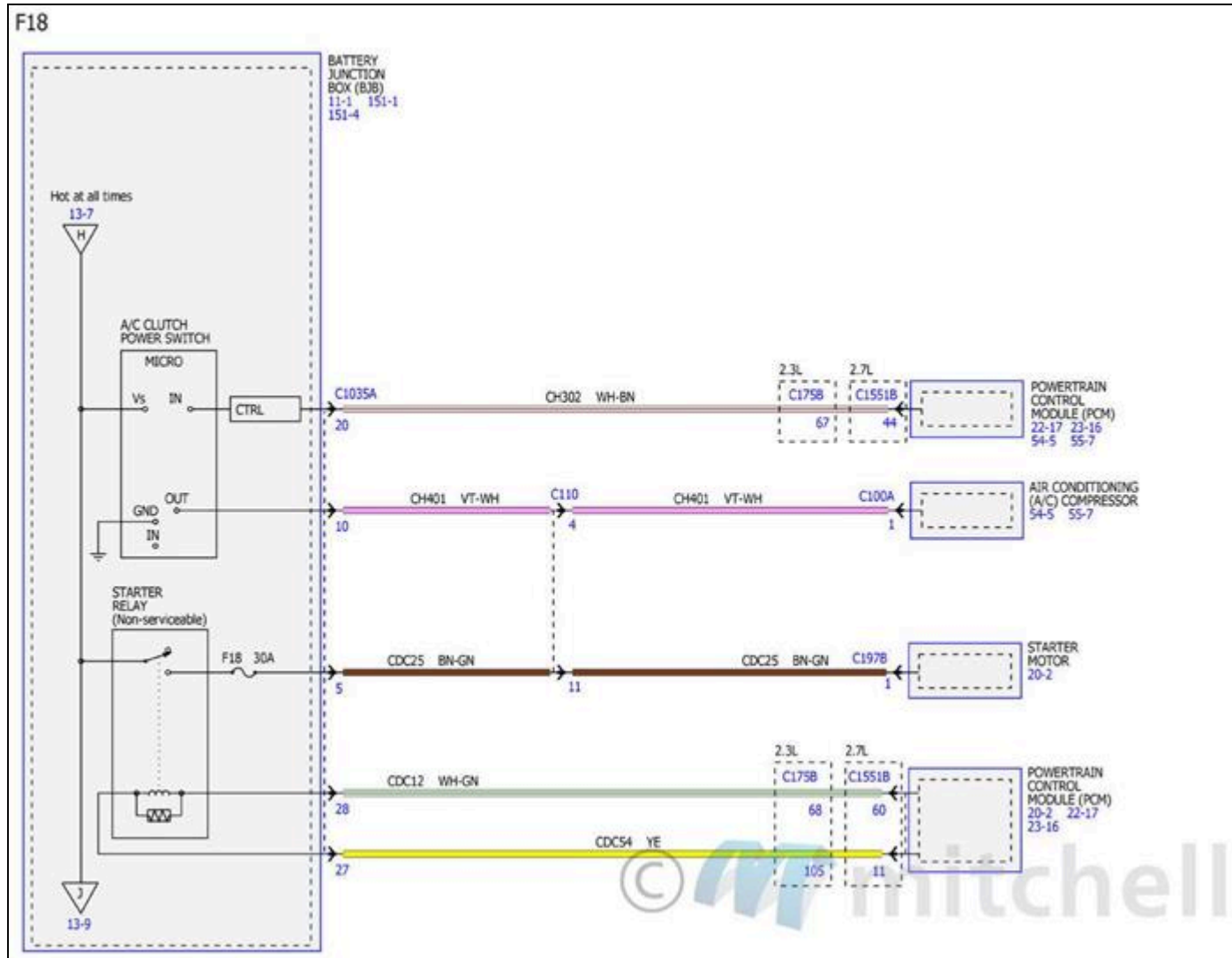
Fig. 137: Power Distribution/BCM Wiring Diagrams (8 Of 34)
