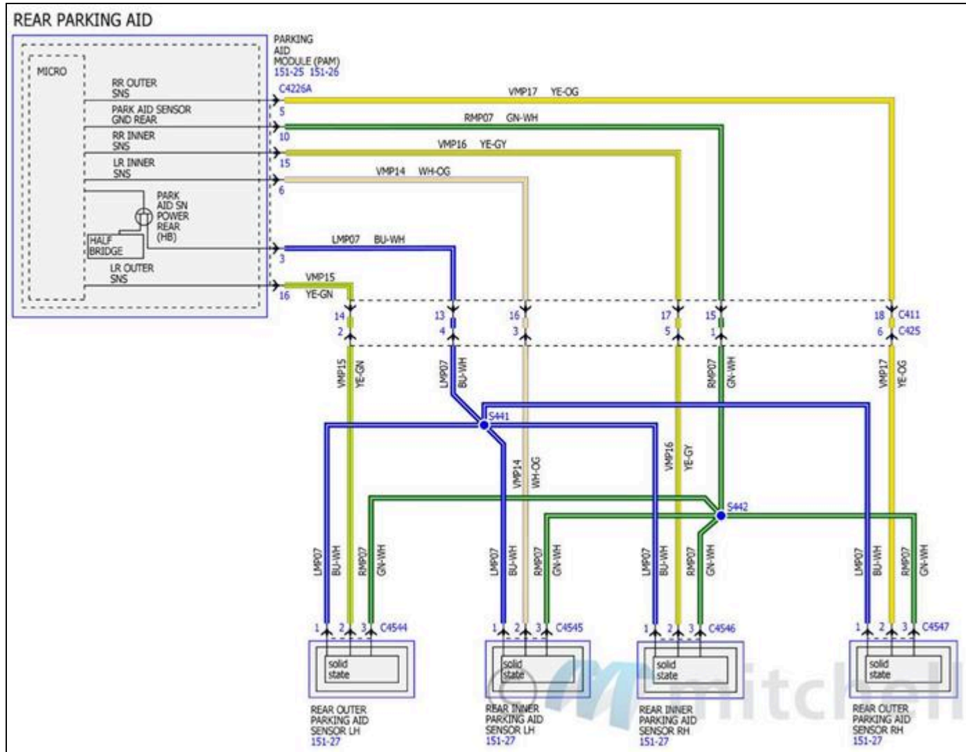
Fig. 117: Parking Aid Wiring Diagrams (3 Of 6)
