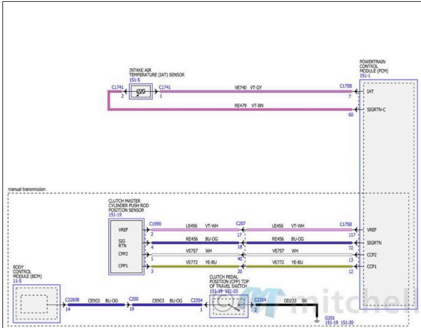
Fig. 52: Electronic Engine Controls Wiring Diagrams - 2.3L (10 Of 17)
