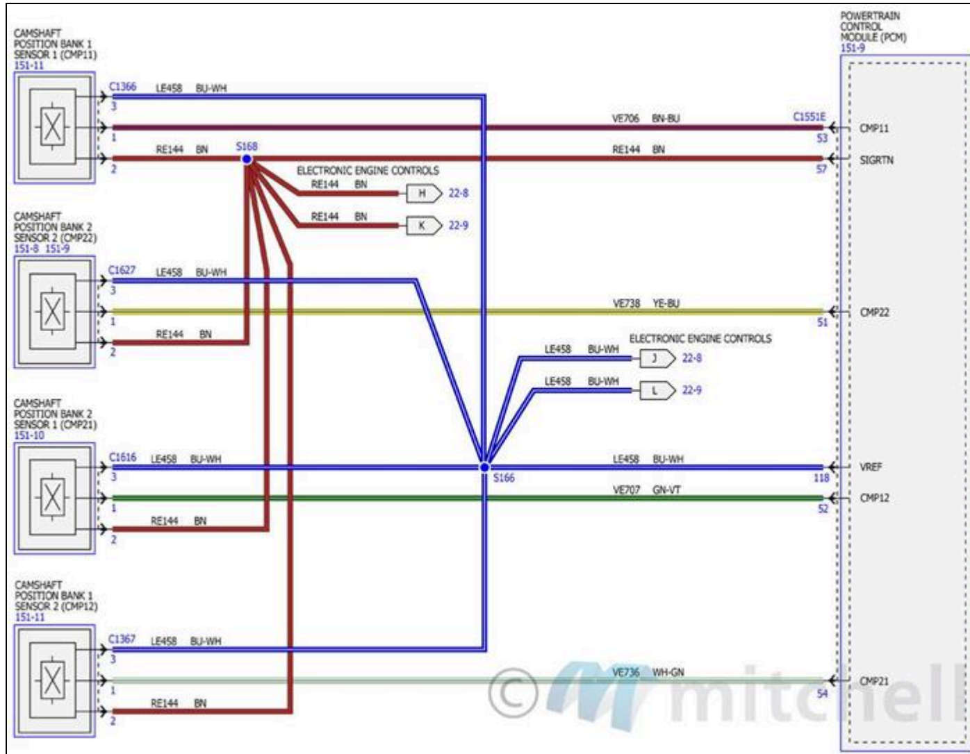
Fig. 71: Electronic Engine Controls Wiring Diagrams - 2.7L (12 Of 18)
