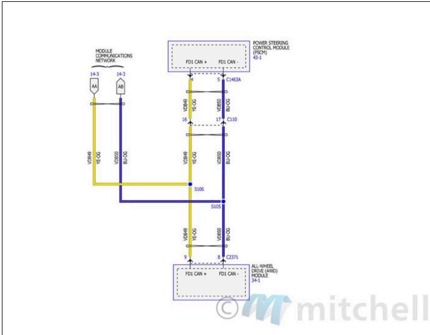
Fig. 110: Module Communications Network Wiring Diagrams (4 Of 8)
