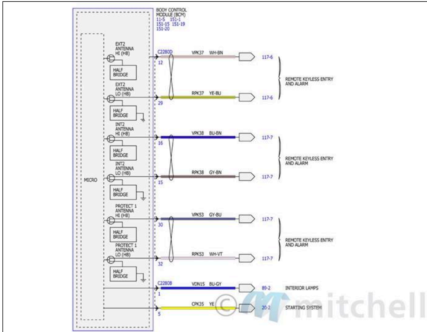
Fig. 160: Power Distribution/BCM Wiring Diagrams (31 Of 34)
