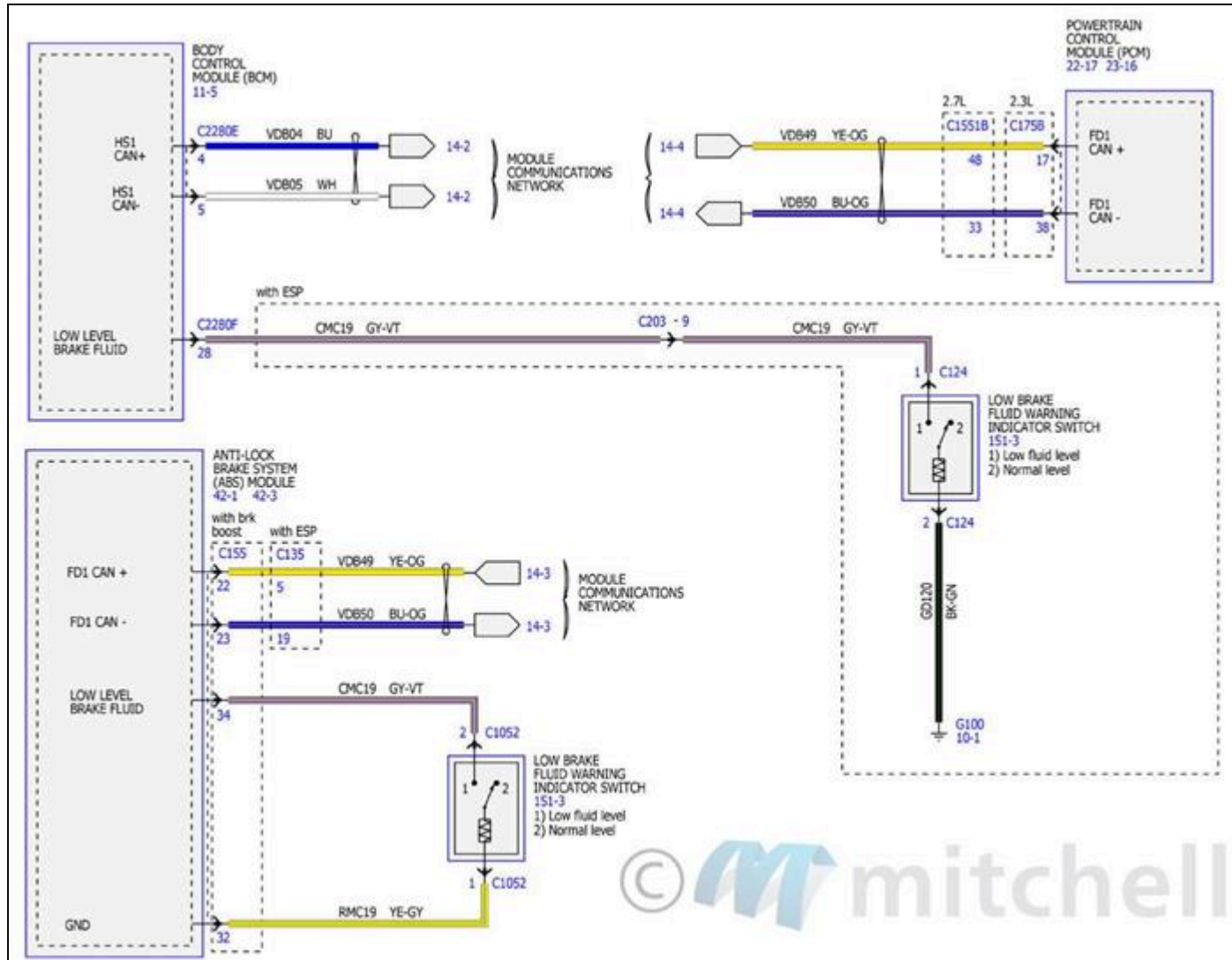
Fig. 96: Instrument Cluster Wiring Diagrams (3 Of 4)
