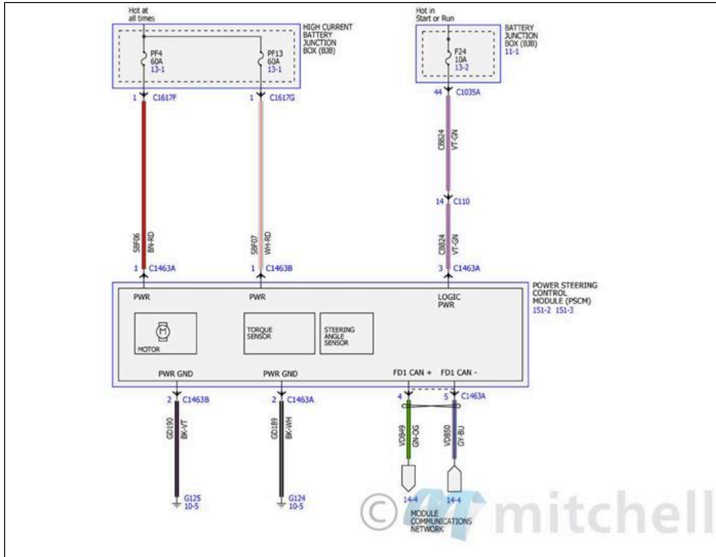
Fig. 170: Power Steering Controls Wiring Diagrams
