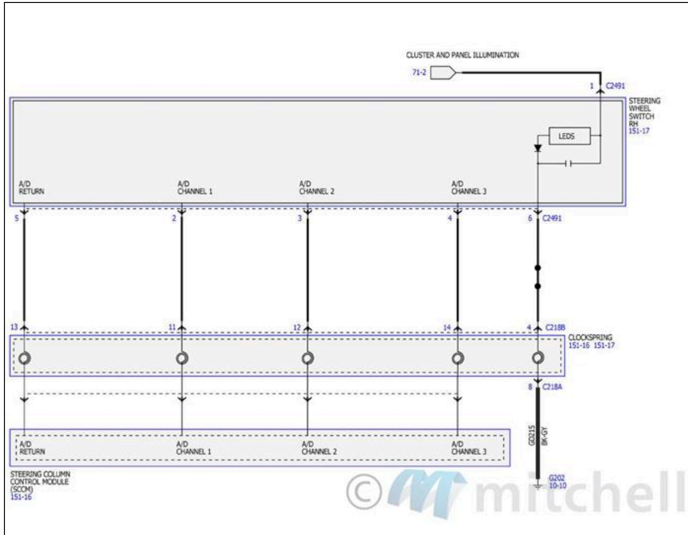
Fig. 97: Instrument Cluster Wiring Diagrams (4 Of 4)
