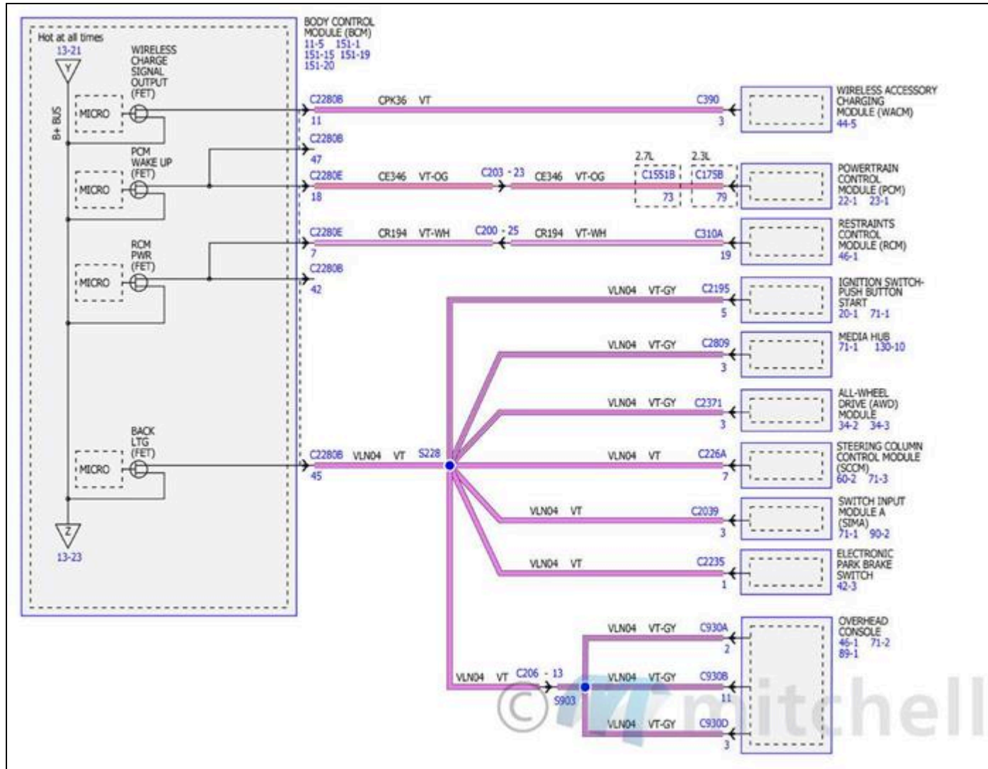
Fig. 151: Power Distribution/BCM Wiring Diagrams (22 Of 34)
