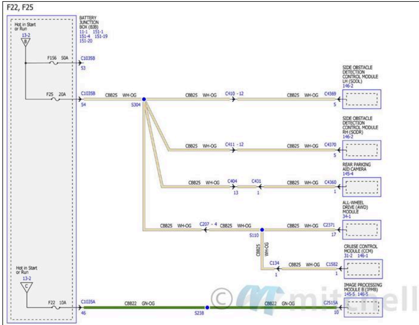
Fig. 132: Power Distribution/BCM Wiring Diagrams (3 Of 34)
