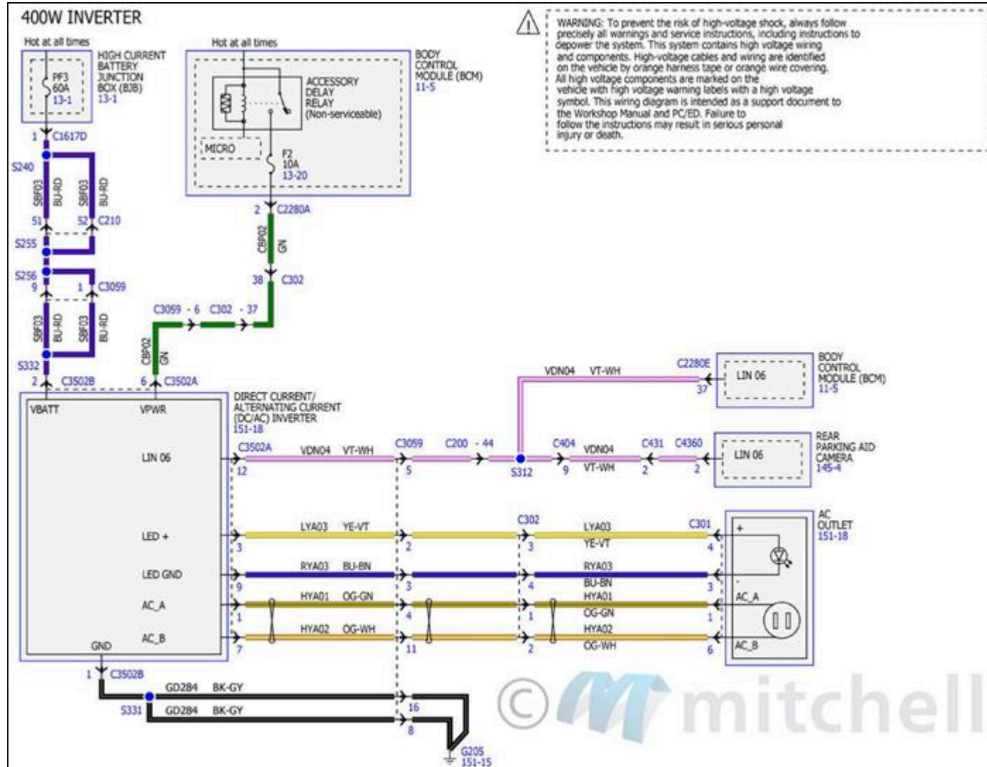
Fig. 92: Horn/Cigar Lighter Wiring Diagrams (4 Of 5)
