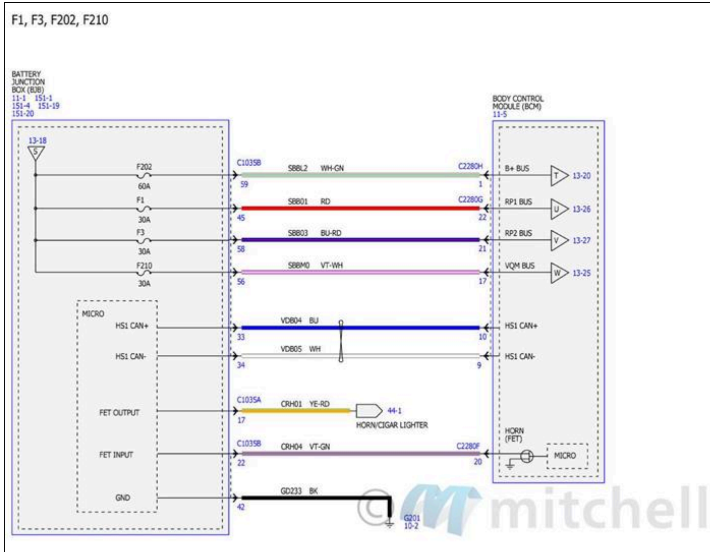
Fig. 148: Power Distribution/BCM Wiring Diagrams (19 Of 34)
