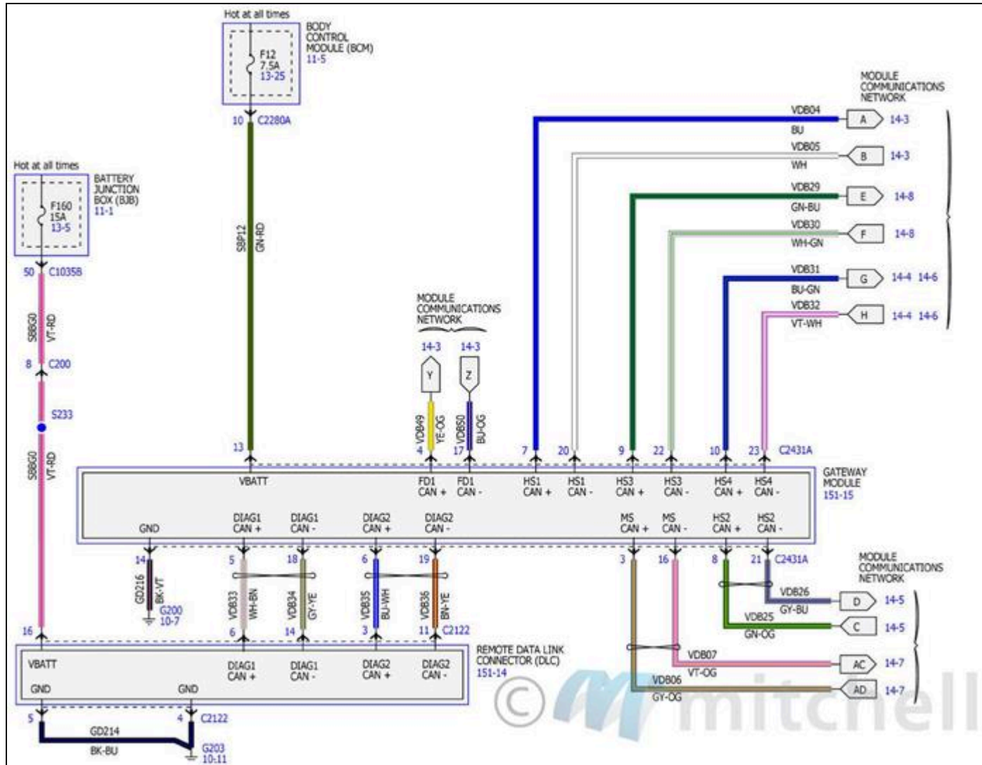
Fig. 107: Module Communications Network Wiring Diagrams (1 Of 8)
