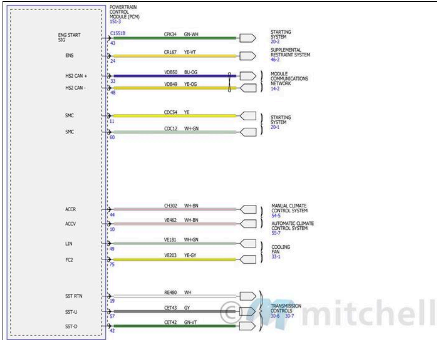
Fig. 75: Electronic Engine Controls Wiring Diagrams - 2.7L (16 Of 18)
