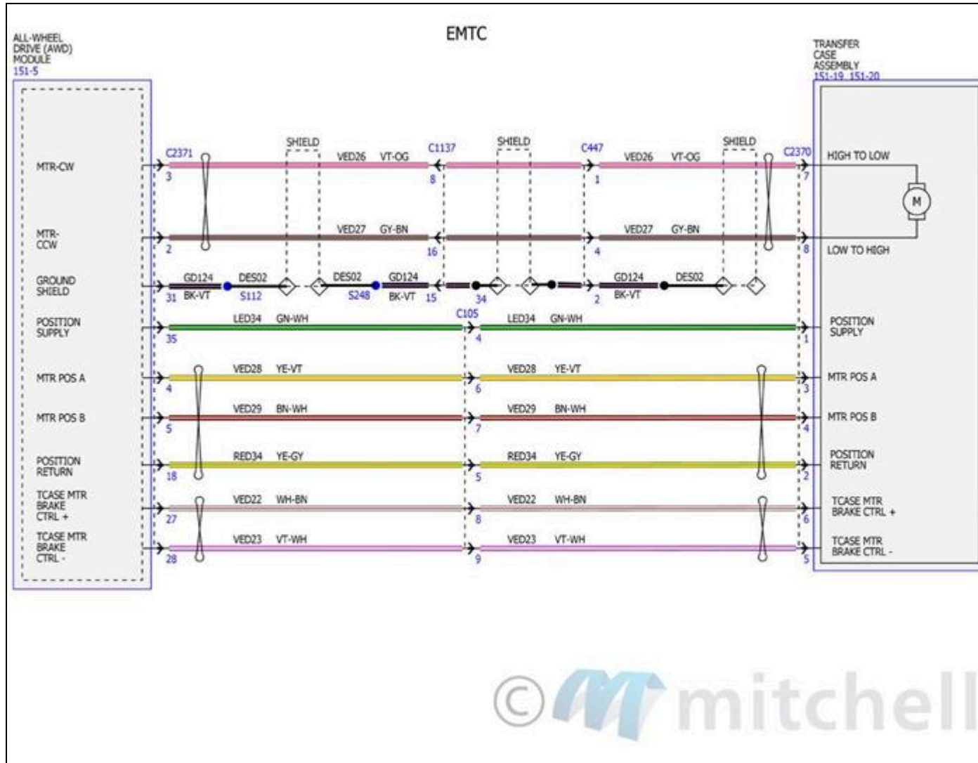
Fig. 82: Four Wheel Drive Systems Wiring Diagrams (3 Of 4)
