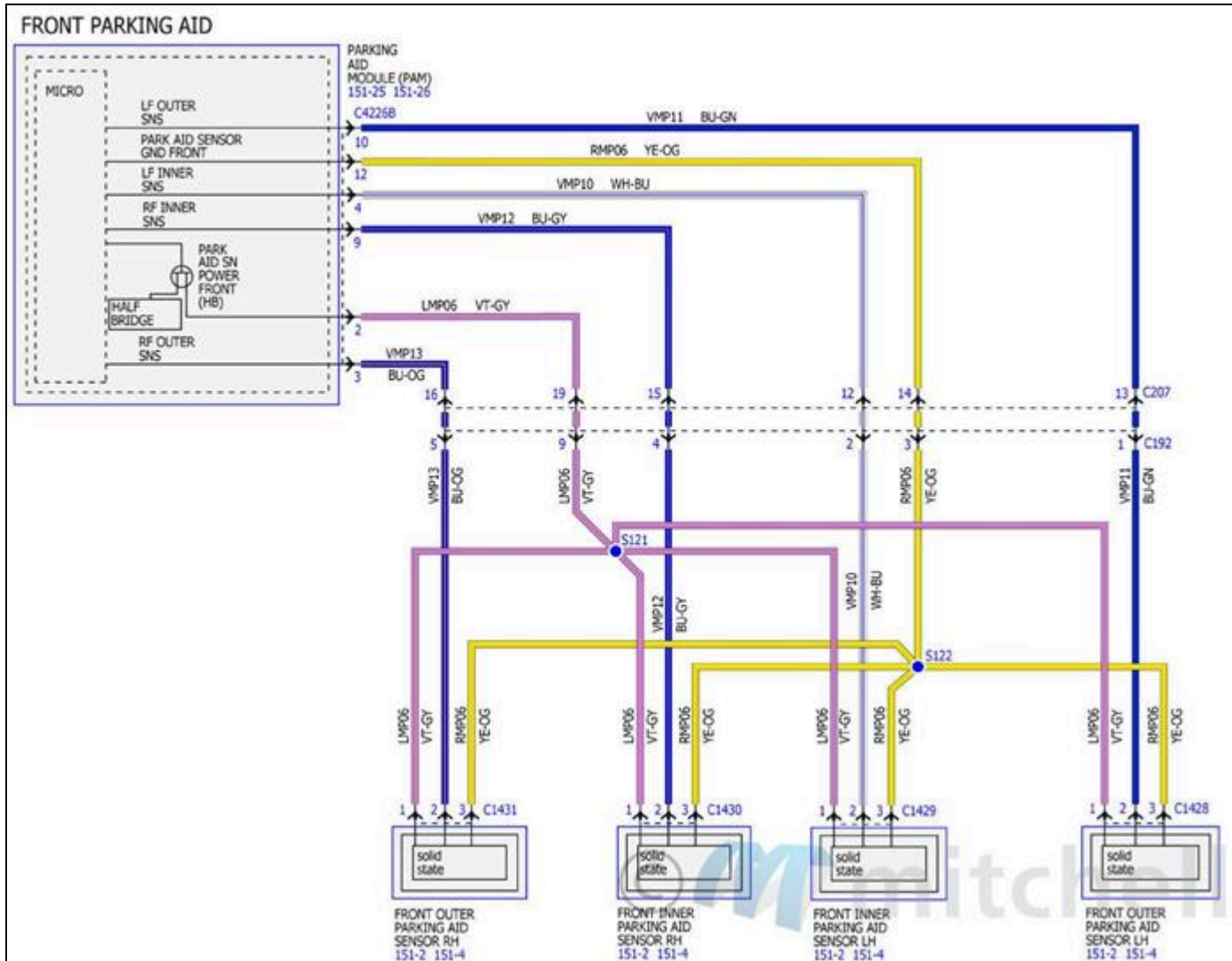
Fig. 116: Parking Aid Wiring Diagrams (2 Of 6)
