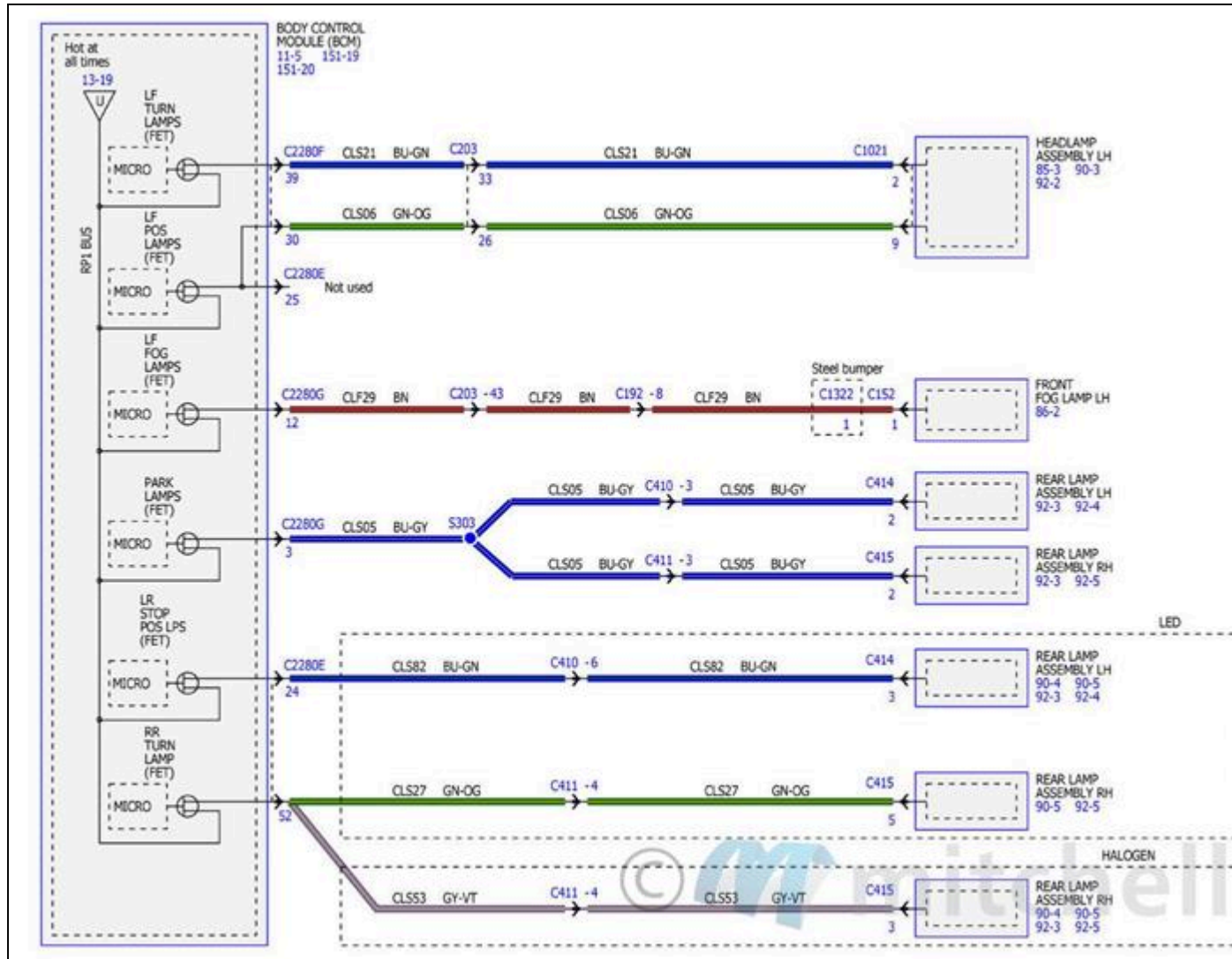
Fig. 155: Power Distribution/BCM Wiring Diagrams (26 Of 34)
