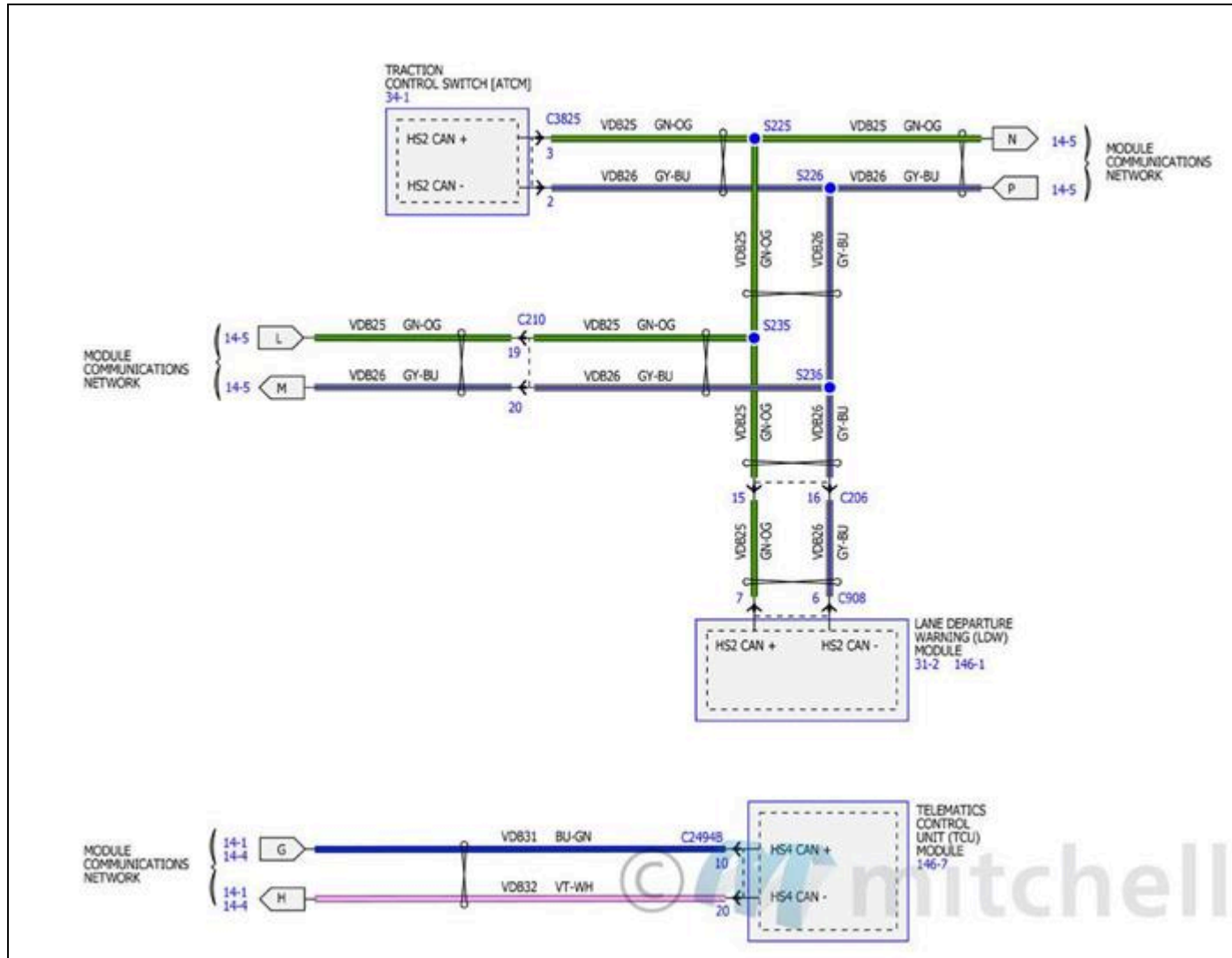
Fig. 112: Module Communications Network Wiring Diagrams (6 Of 8)
