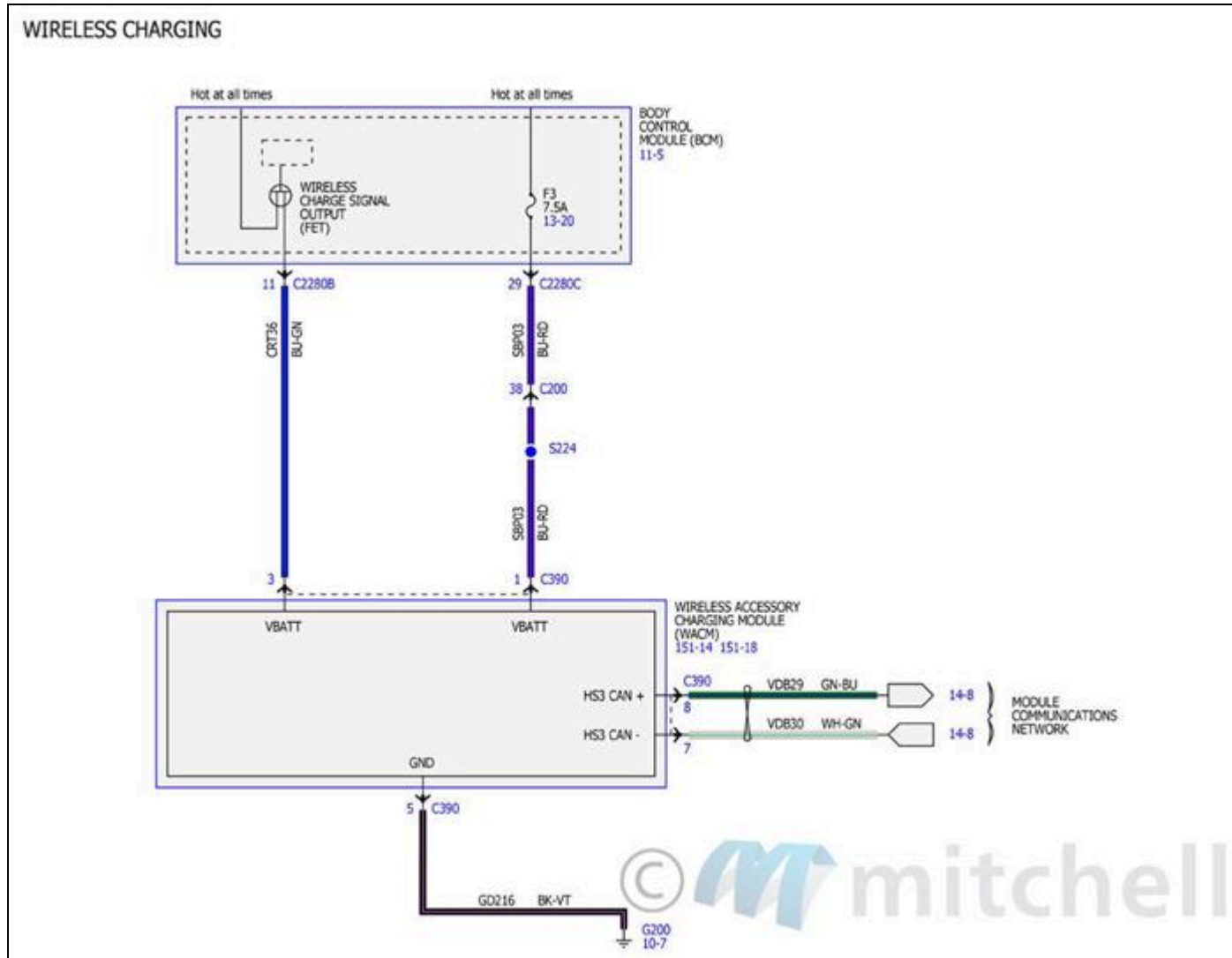
Fig. 93: Horn/Cigar Lighter Wiring Diagrams (5 Of 5)
