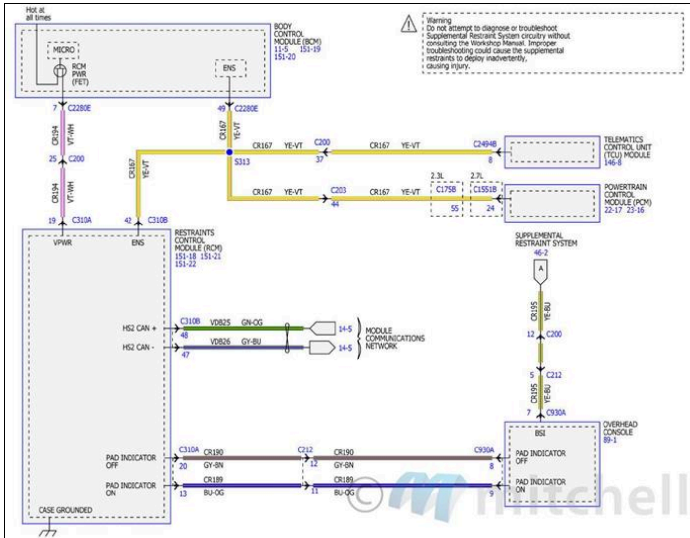
Fig. 189: Supplemental Restraint System Wiring Diagrams (1 Of 8)
