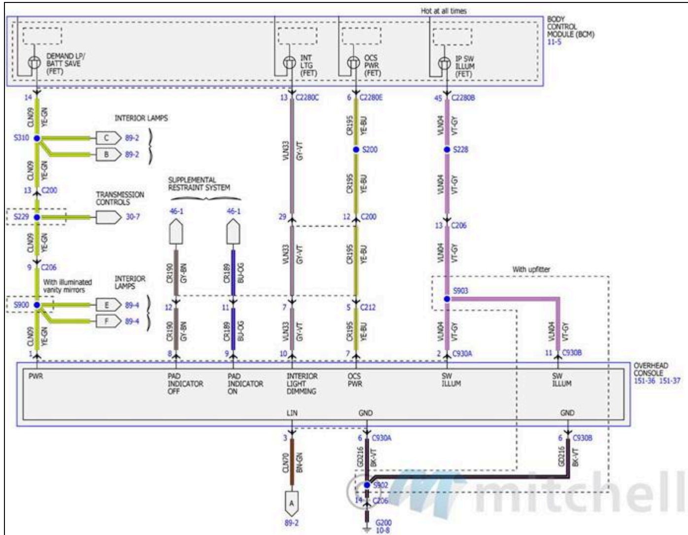
Fig. 98: Interior Lamps Wiring Diagrams (1 Of 4)
