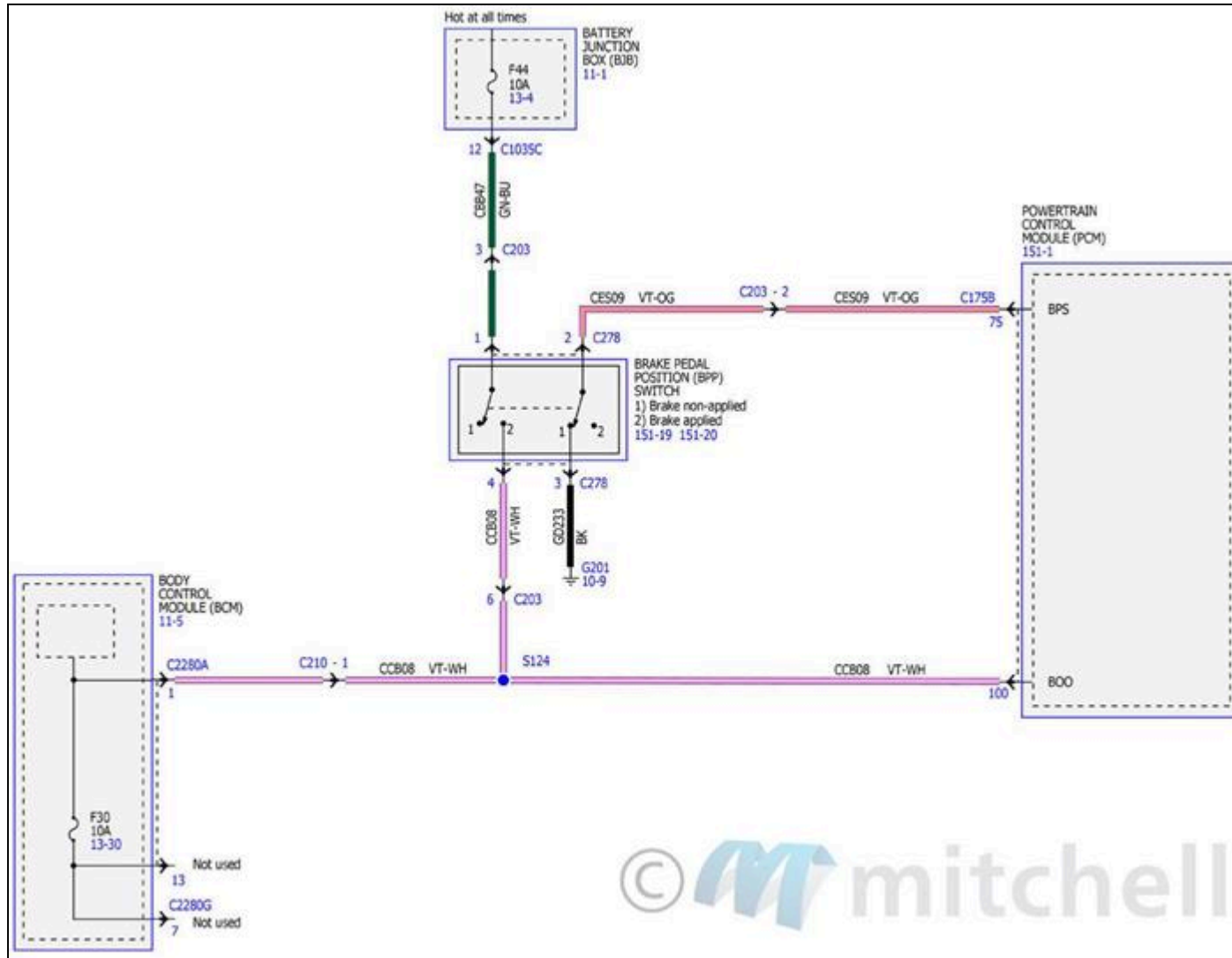
Fig. 54: Electronic Engine Controls Wiring Diagrams - 2.3L (12 Of 17)
