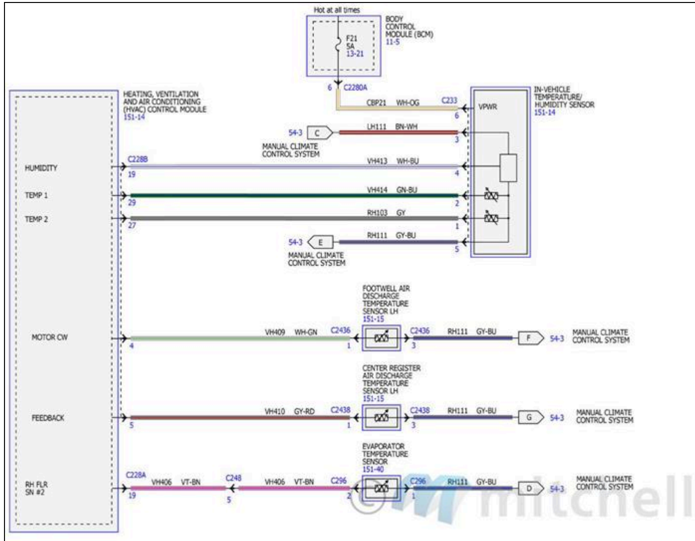
Fig. 105: Manual Climate Control System Wiring Diagrams (4 Of 5)
