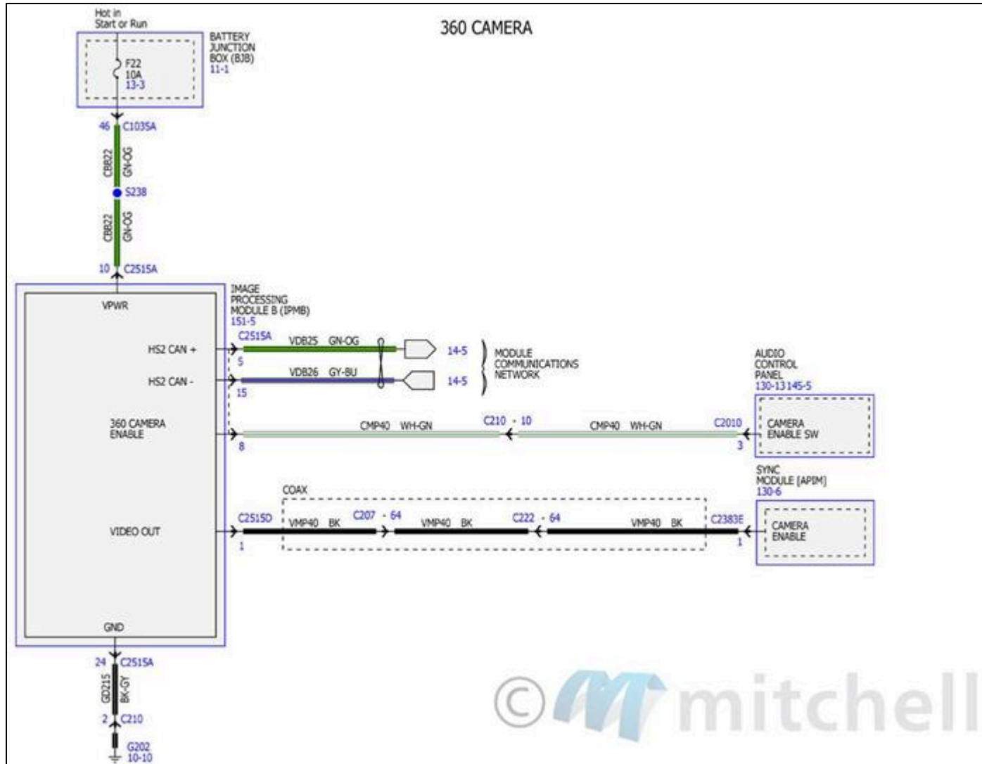
Fig. 119: Parking Aid Wiring Diagrams (5 Of 6)
