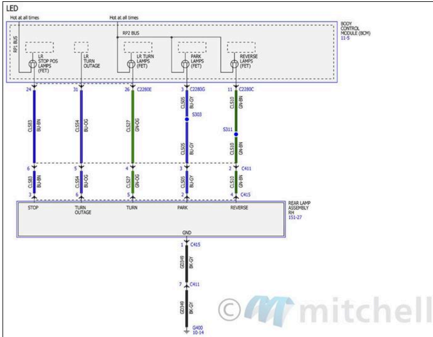
Fig. 125: Parking, Rear and License Lamps Wiring Diagrams (5 Of 6)
