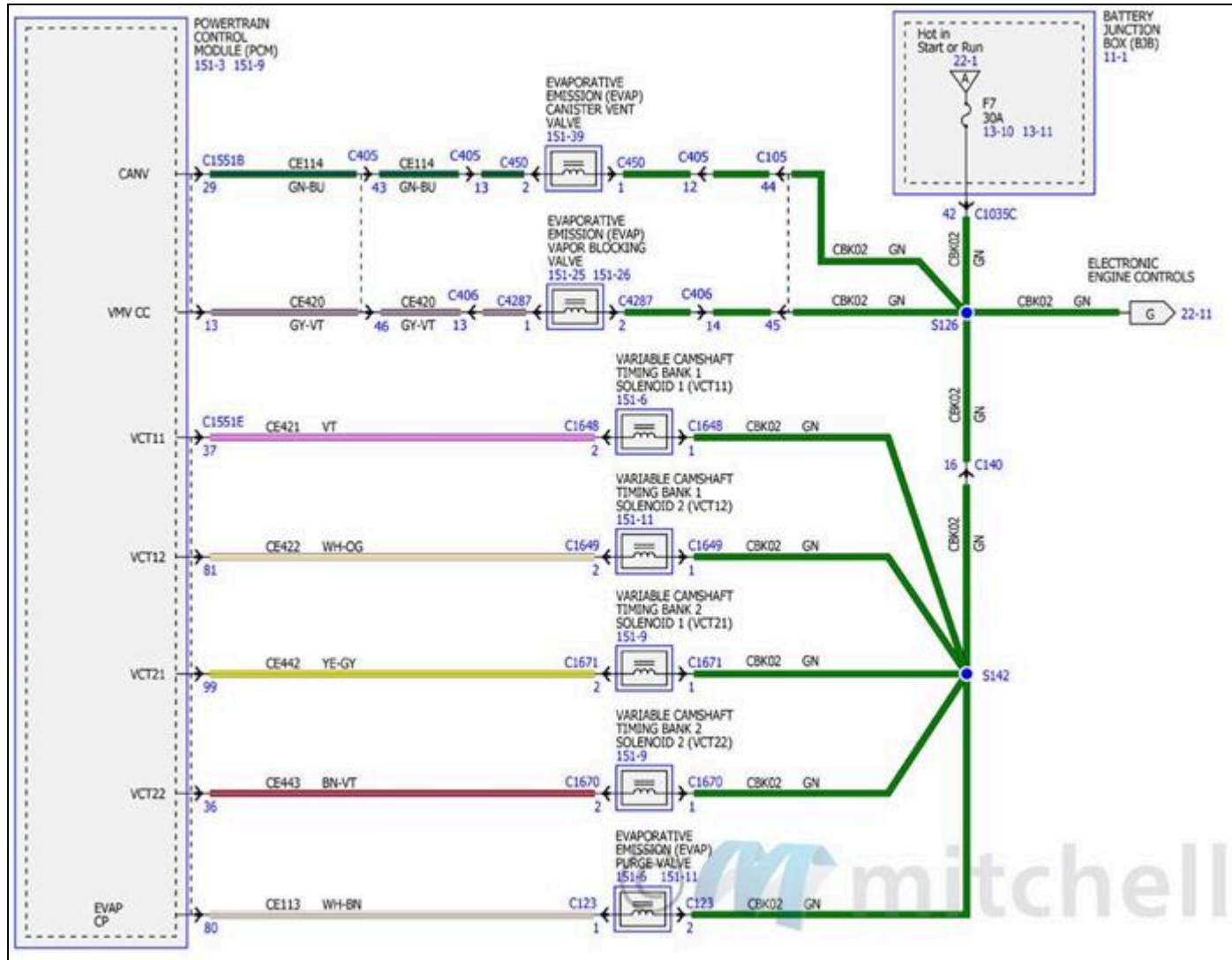
Fig. 69: Electronic Engine Controls Wiring Diagrams - 2.7L (10 Of 18)
