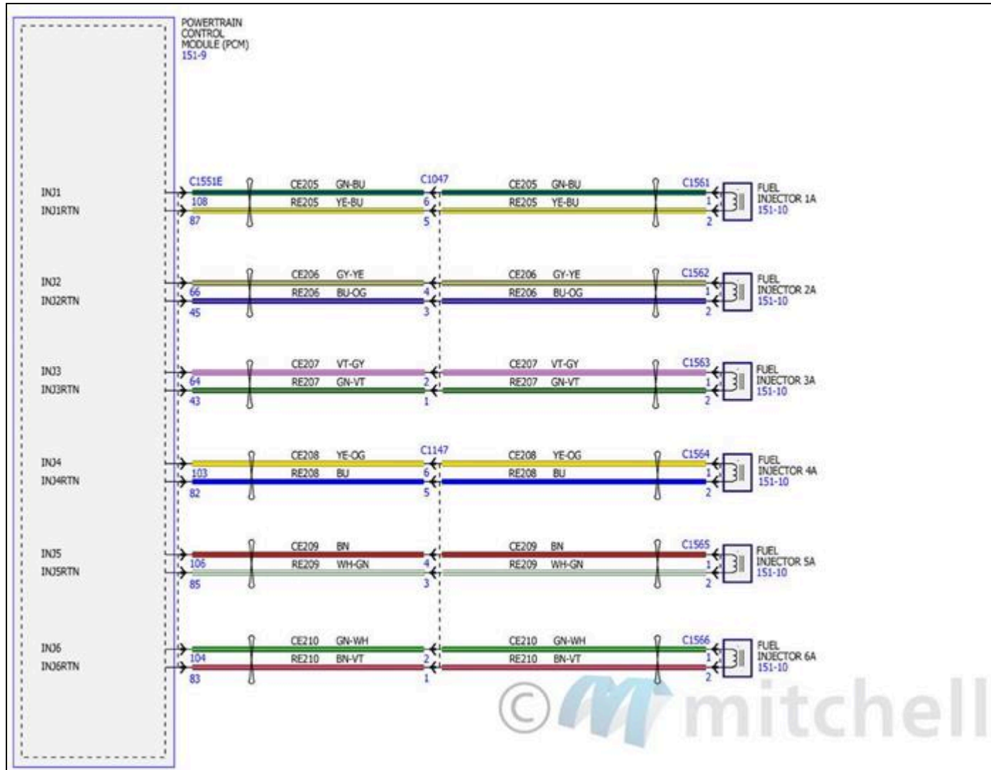
Fig. 62: Electronic Engine Controls Wiring Diagrams - 2.7L (3 Of 18)
