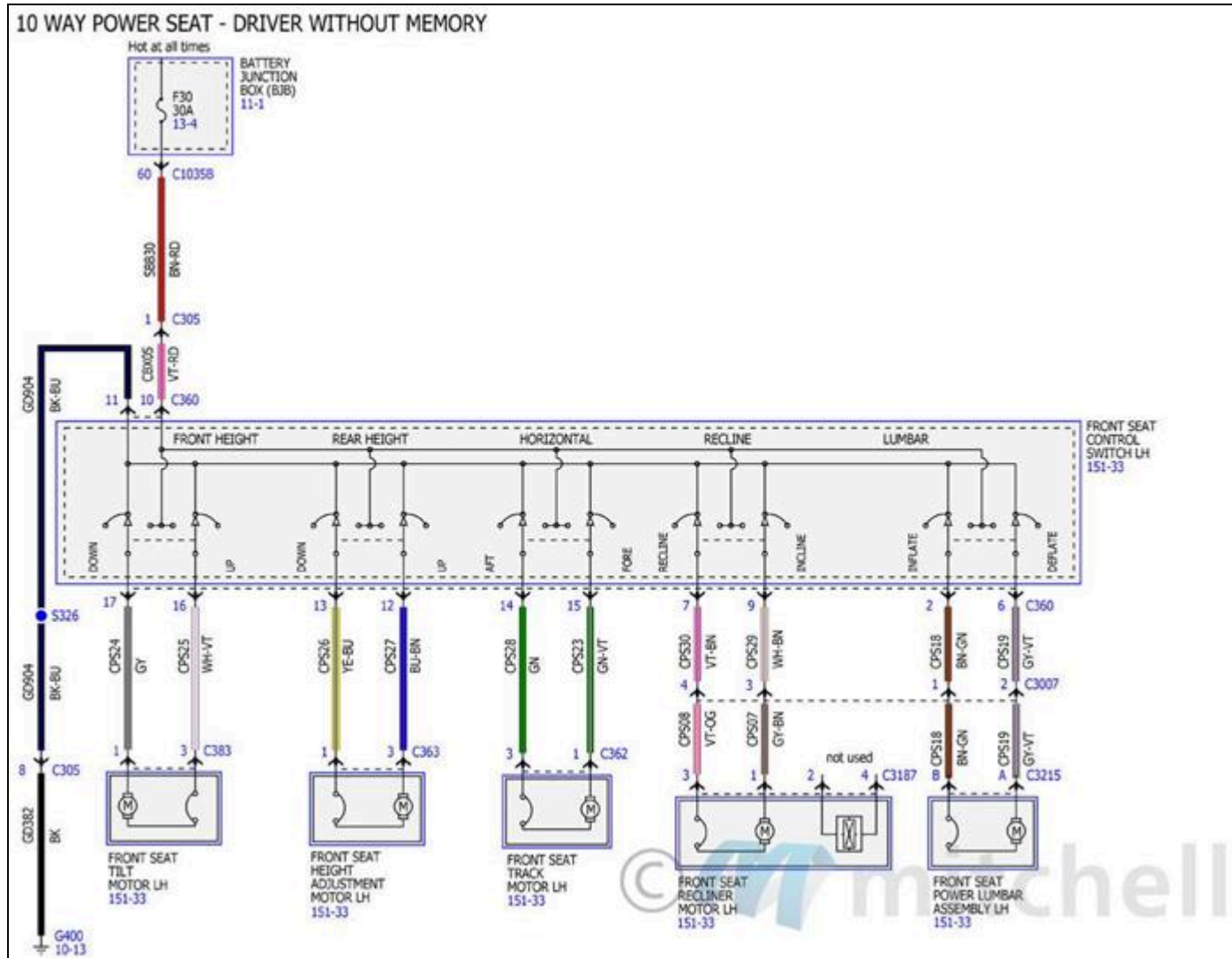
Fig. 168: Power Seats Wiring Diagrams (1 Of 2)
