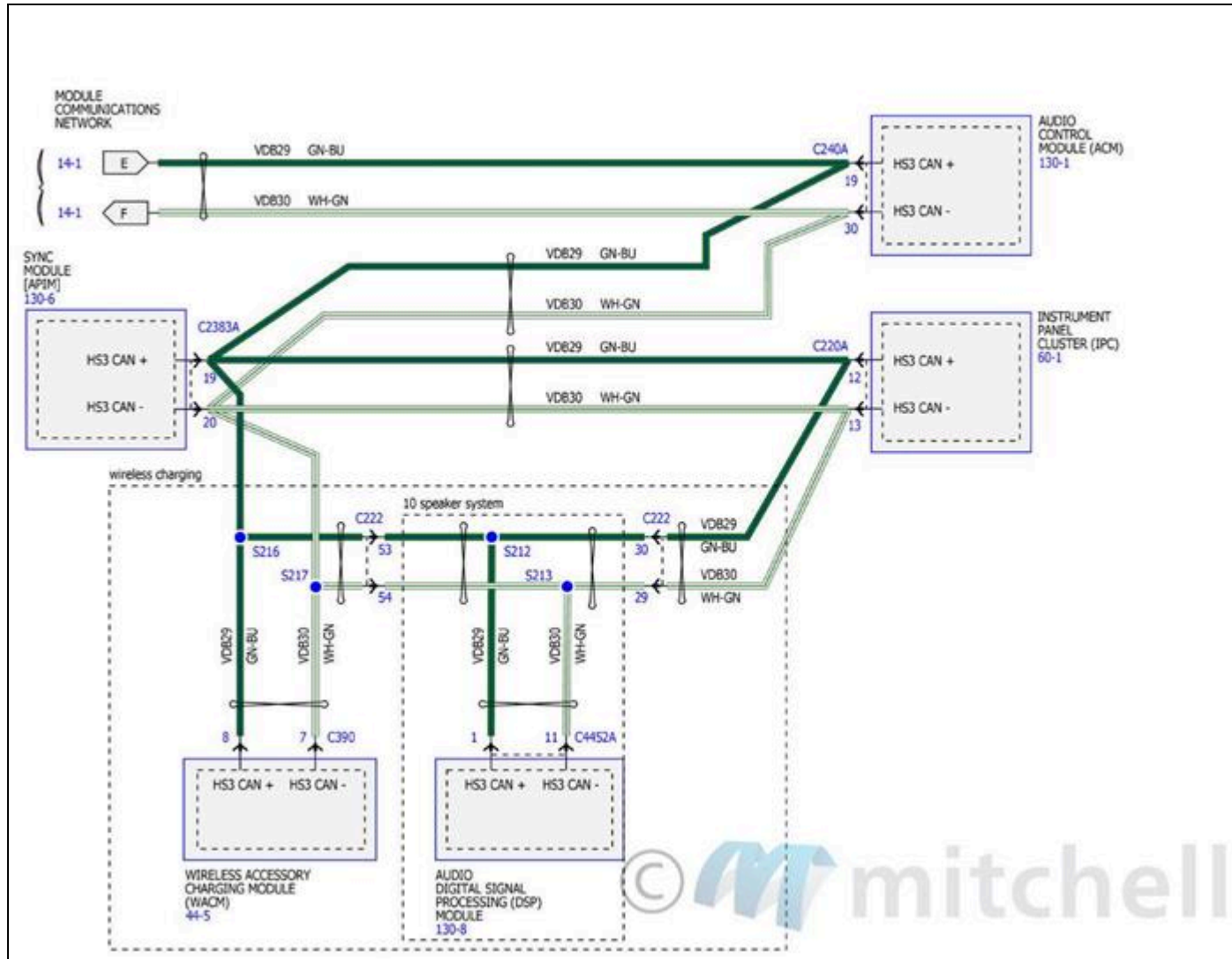
Fig. 114: Module Communications Network Wiring Diagrams (8 Of 8)
