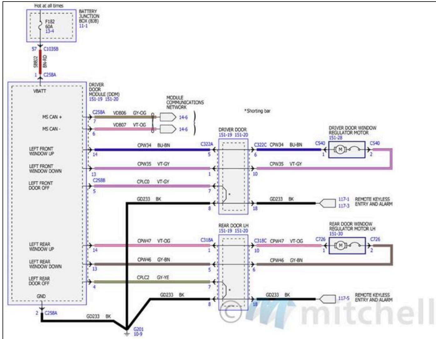
Fig. 171: Power Windows Wiring Diagrams (1 Of 6)
