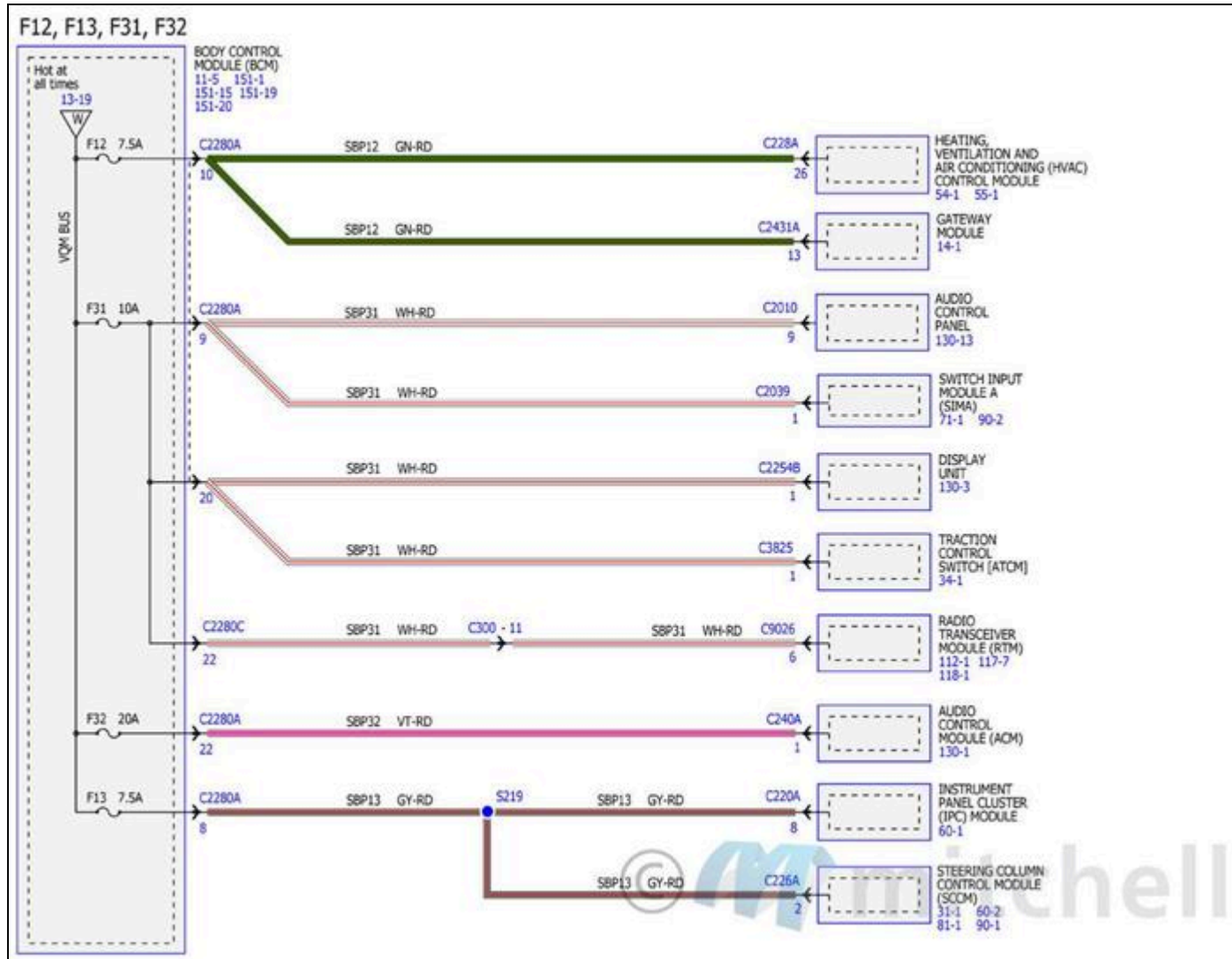
Fig. 154: Power Distribution/BCM Wiring Diagrams (25 Of 34)
