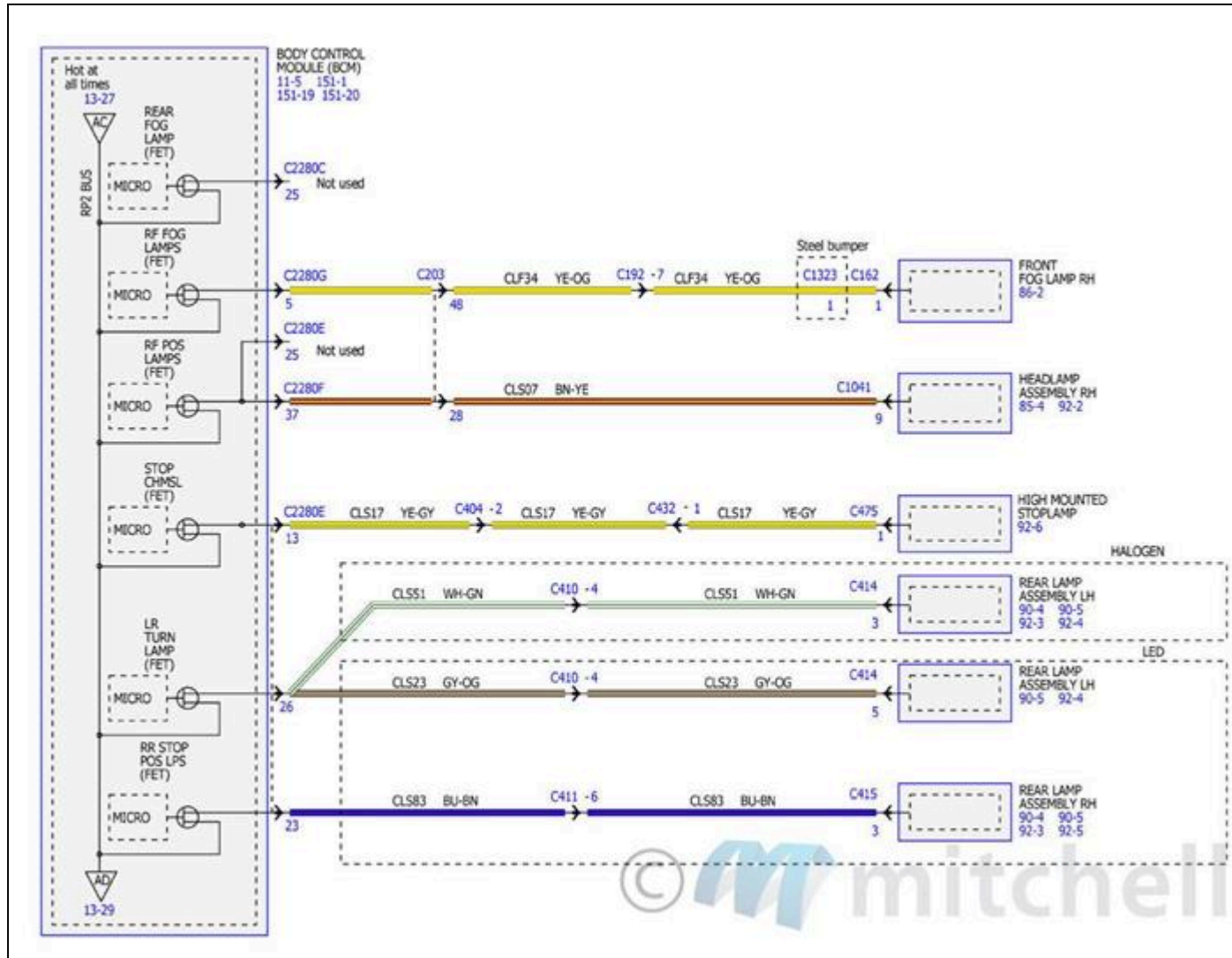
Fig. 157: Power Distribution/BCM Wiring Diagrams (28 Of 34)
