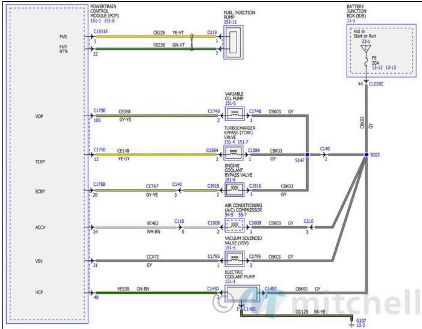
Fig. 50: Electronic Engine Controls Wiring Diagrams - 2.3L (8 Of 17)
