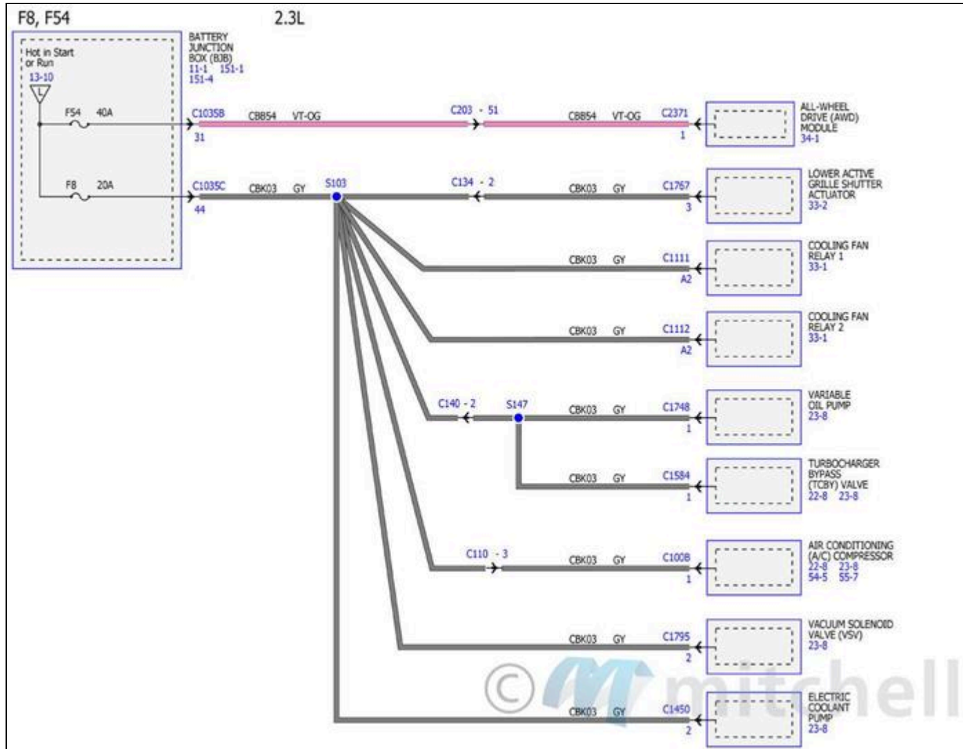
Fig. 141: Power Distribution/BCM Wiring Diagrams (12 Of 34)
