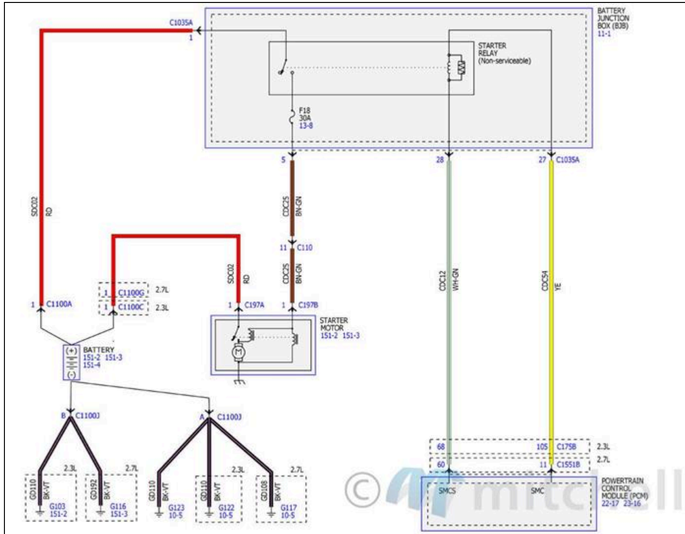
Fig. 188: Starting System Wiring Diagrams (2 Of 2)
