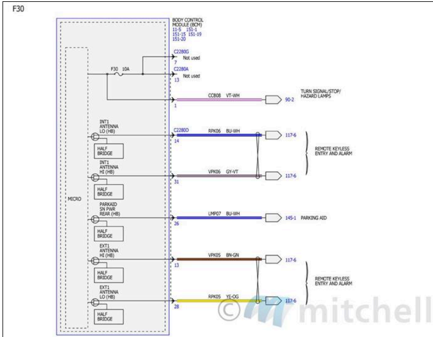
Fig. 159: Power Distribution/BCM Wiring Diagrams (30 Of 34)
