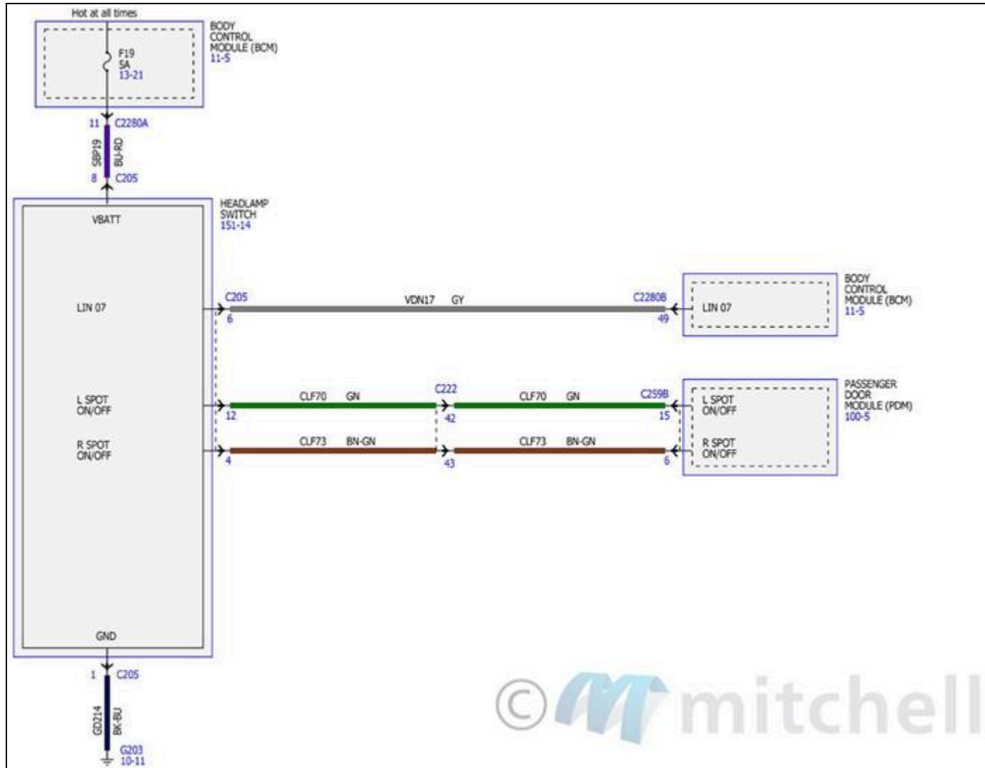
Fig. 78: Fog Lamps Wiring Diagrams (1 Of 2)
