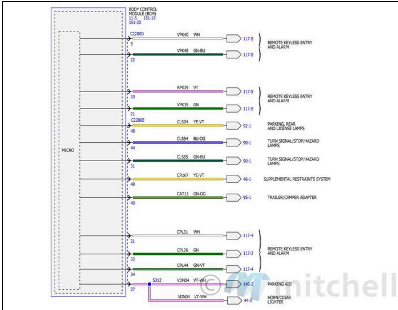
Fig. 162: Power Distribution/BCM Wiring Diagrams (33 Of 34)
