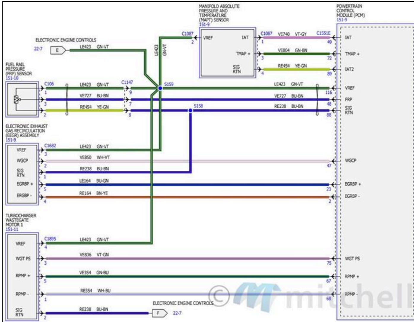
Fig. 65: Electronic Engine Controls Wiring Diagrams - 2.7L (6 Of 18)
