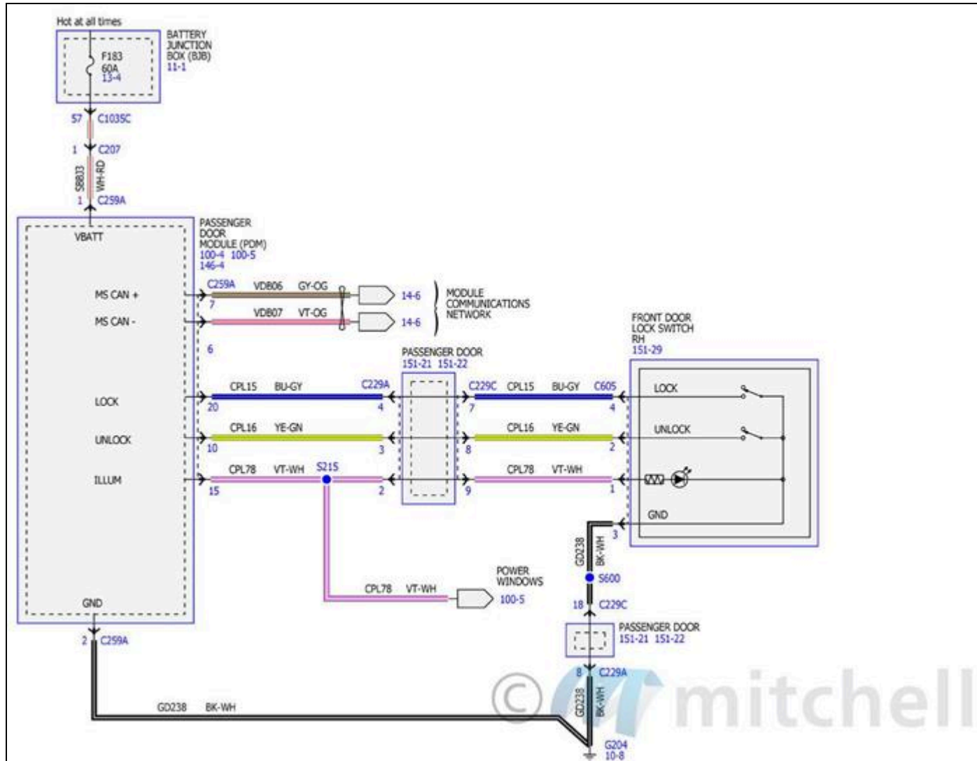
Fig. 178: Remote Keyless Entry and Alarm Wiring Diagrams (2 Of 8)
