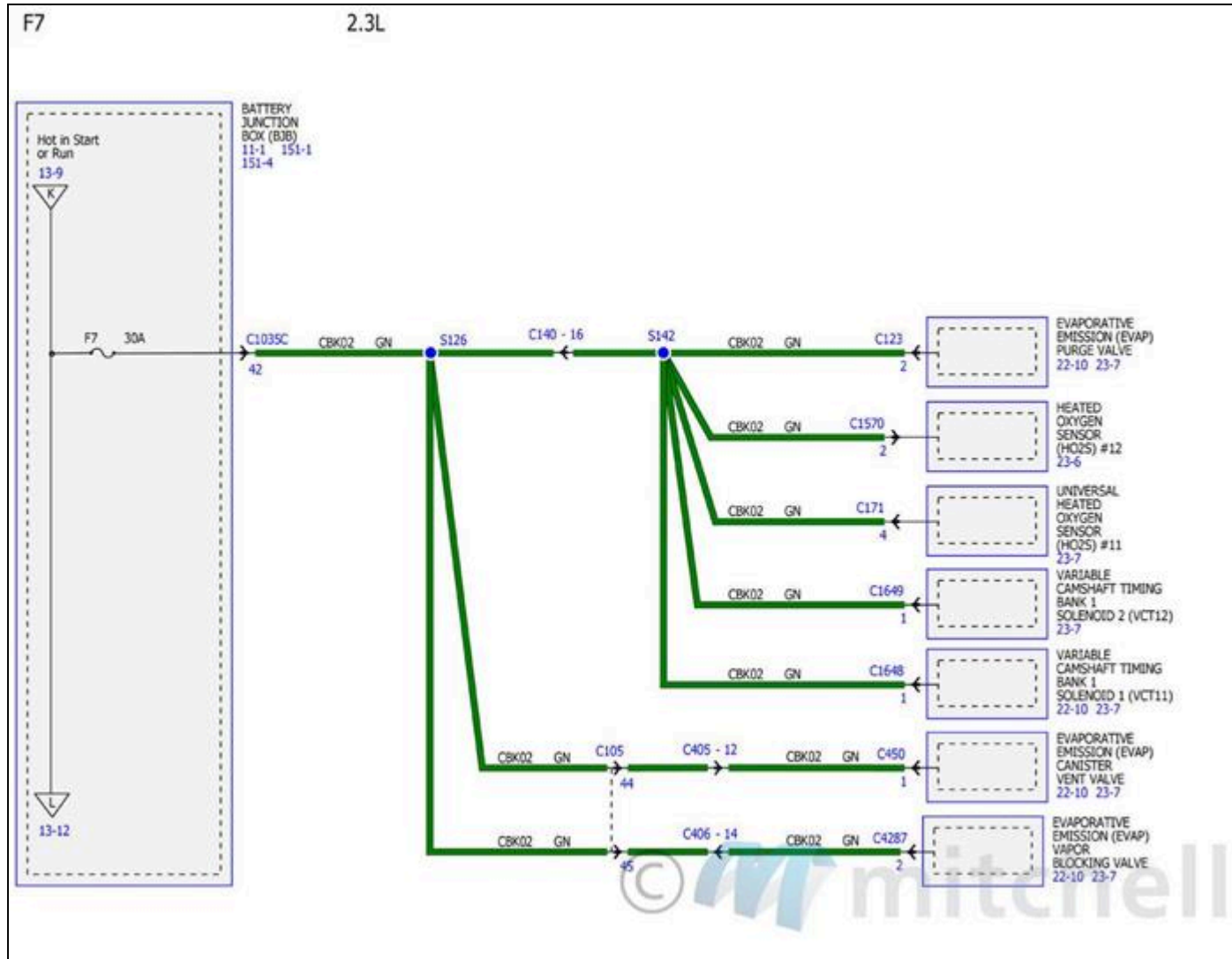
Fig. 139: Power Distribution/BCM Wiring Diagrams (10 Of 34)
