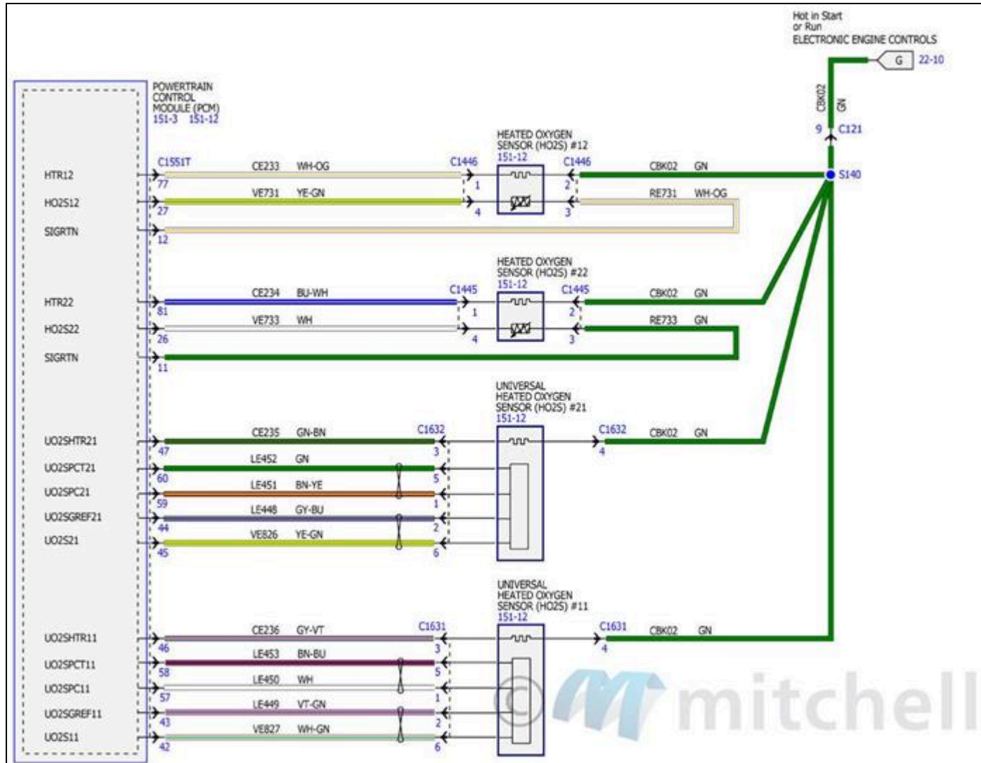
Fig. 70: Electronic Engine Controls Wiring Diagrams - 2.7L (11 Of 18)
