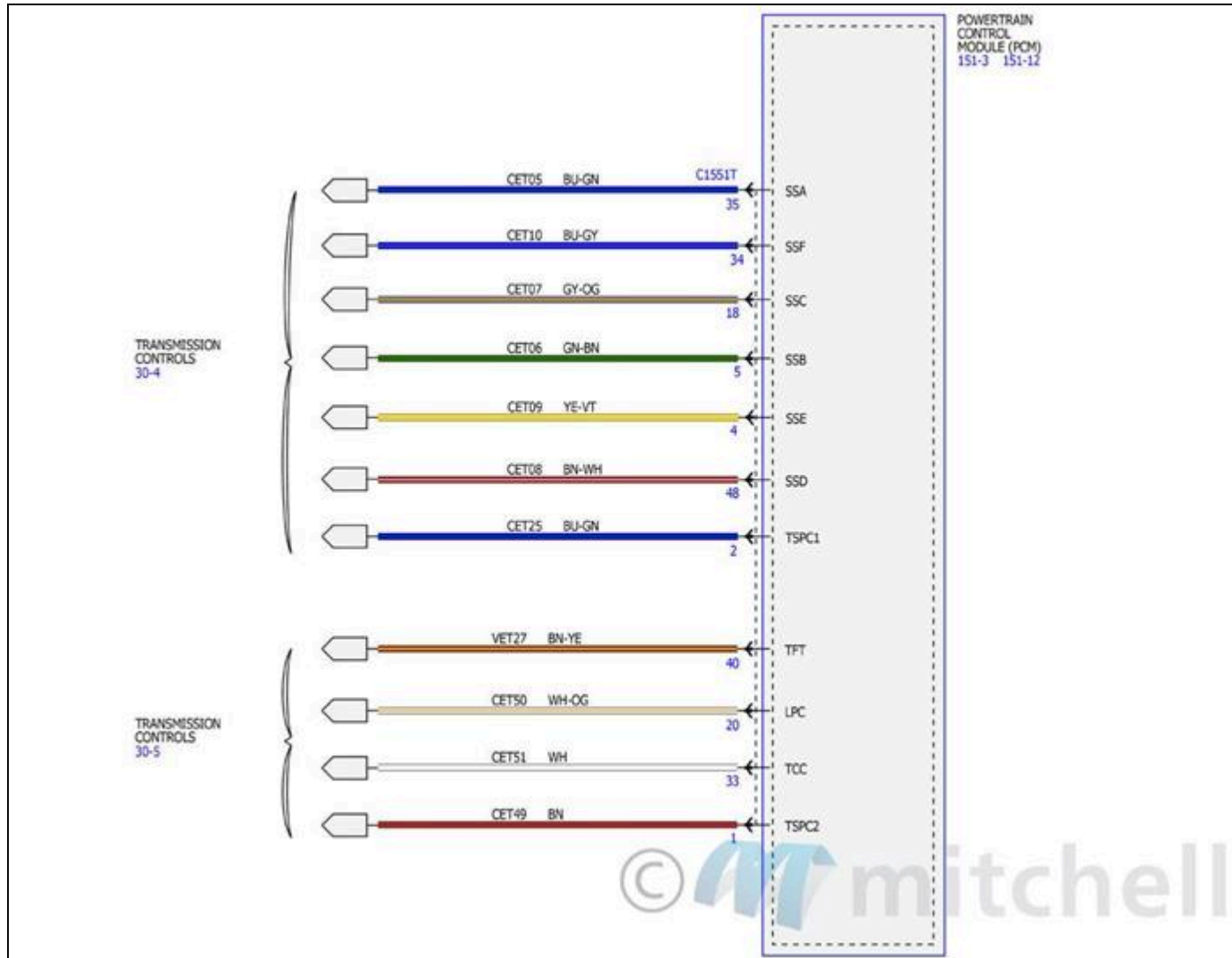
Fig. 77: Electronic Engine Controls Wiring Diagrams - 2.7L (18 Of 18)
