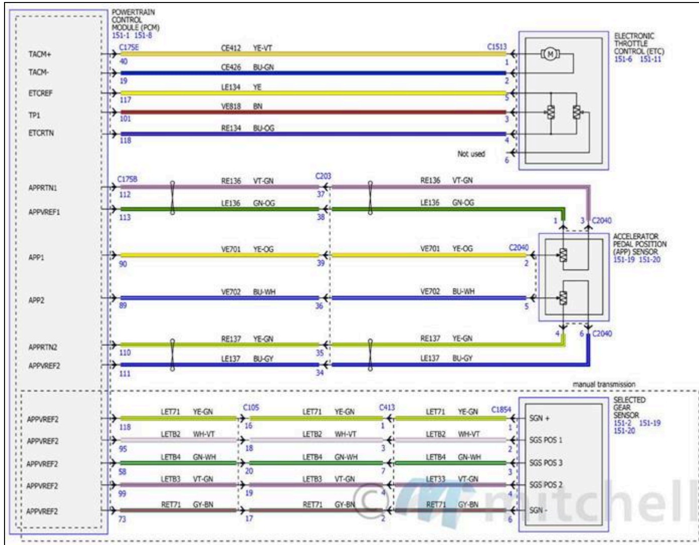
Fig. 55: Electronic Engine Controls Wiring Diagrams - 2.3L (13 Of 17)
