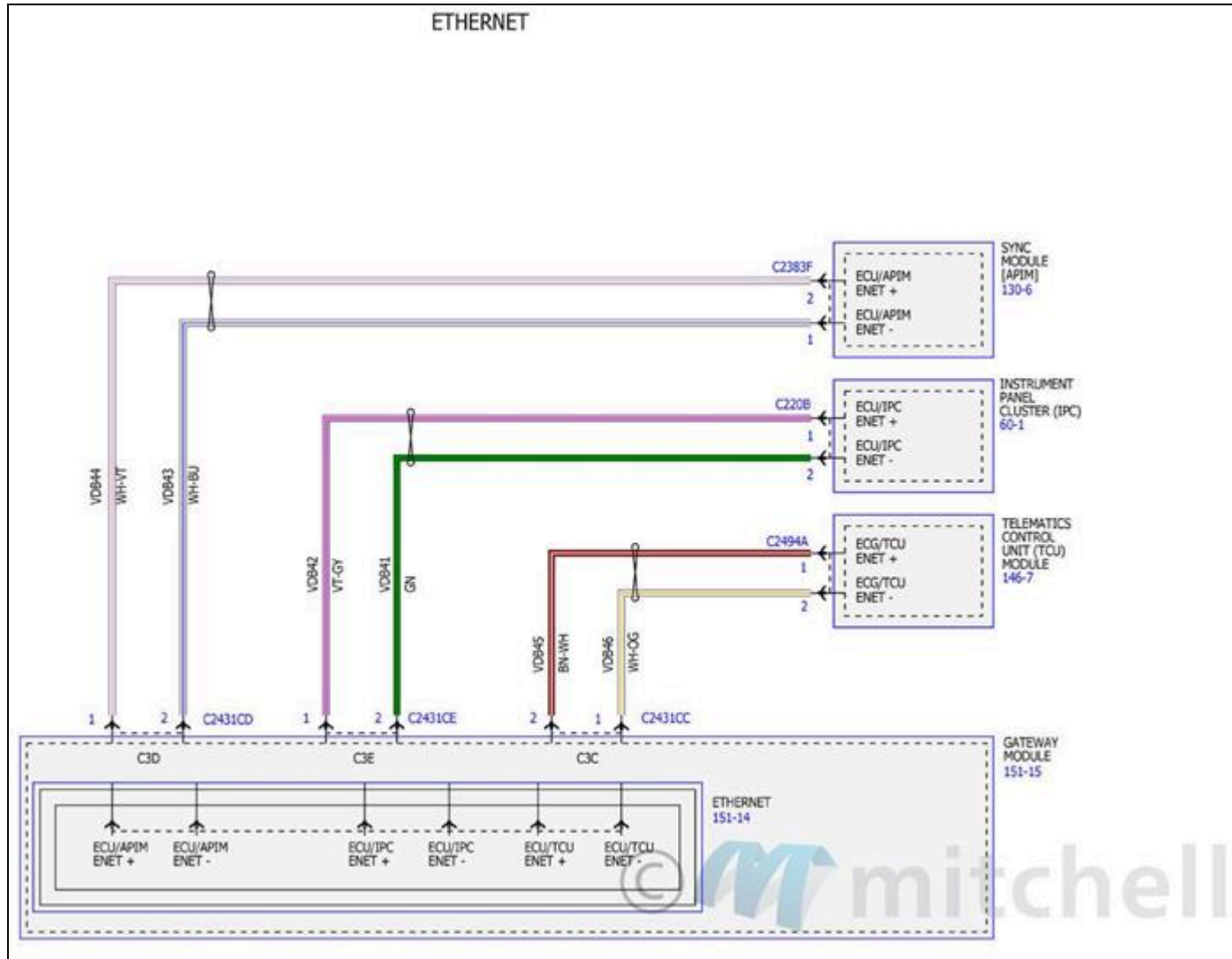
Fig. 108: Module Communications Network Wiring Diagrams (2 Of 8)
