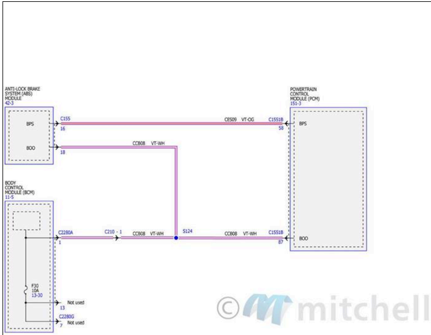
Fig. 74: Electronic Engine Controls Wiring Diagrams - 2.7L (15 Of 18)
