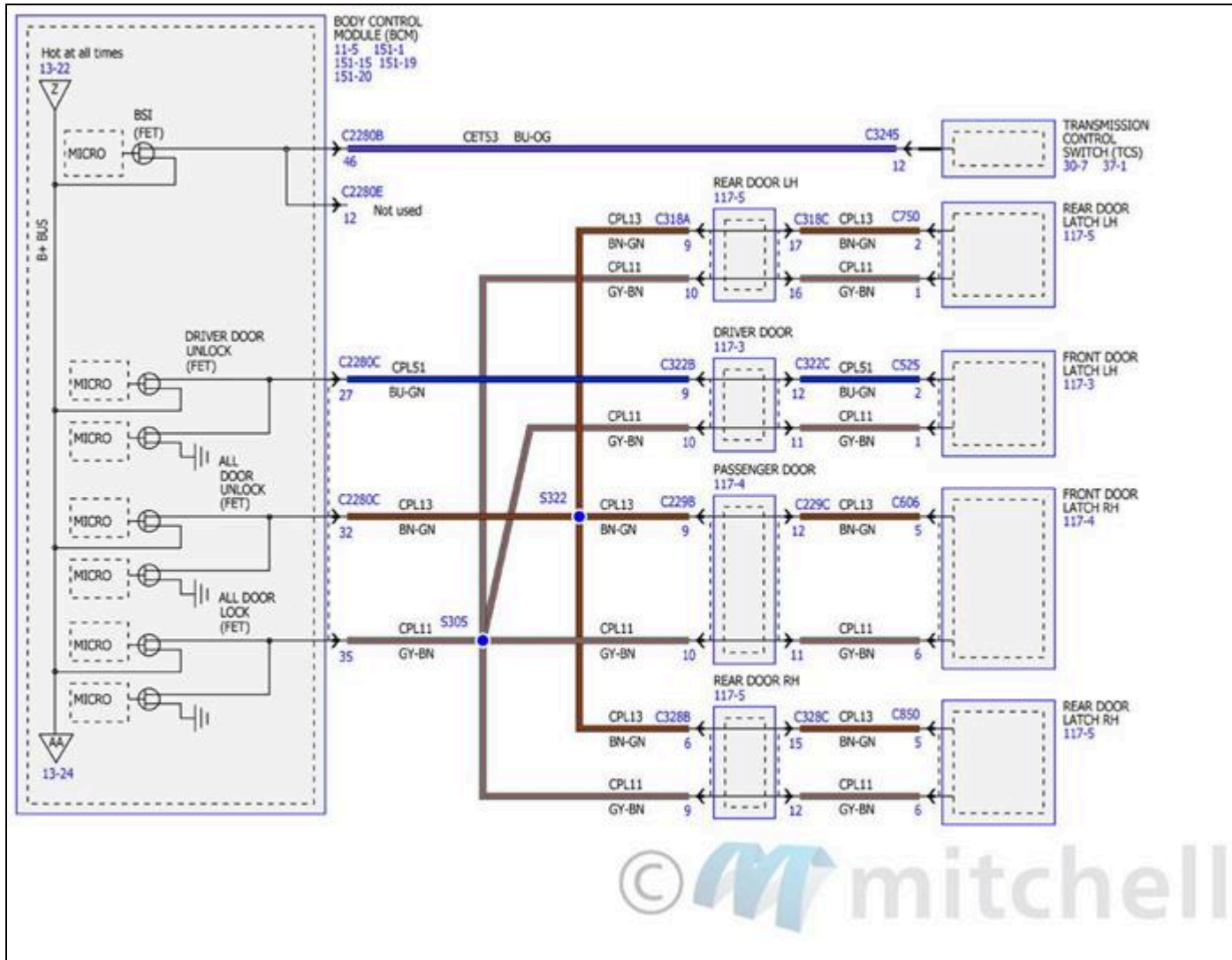
Fig. 152: Power Distribution/BCM Wiring Diagrams (23 Of 34)
