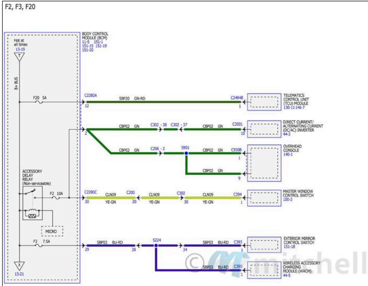
Fig. 149: Power Distribution/BCM Wiring Diagrams (20 Of 34)
