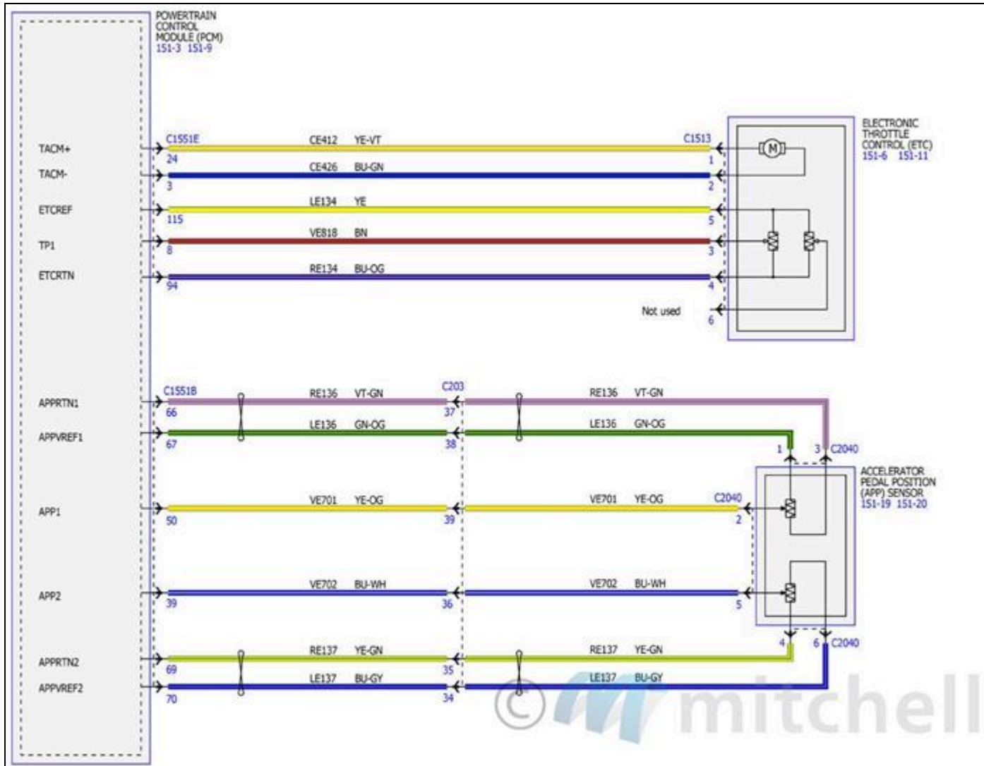
Fig. 72: Electronic Engine Controls Wiring Diagrams - 2.7L (13 Of 18)
