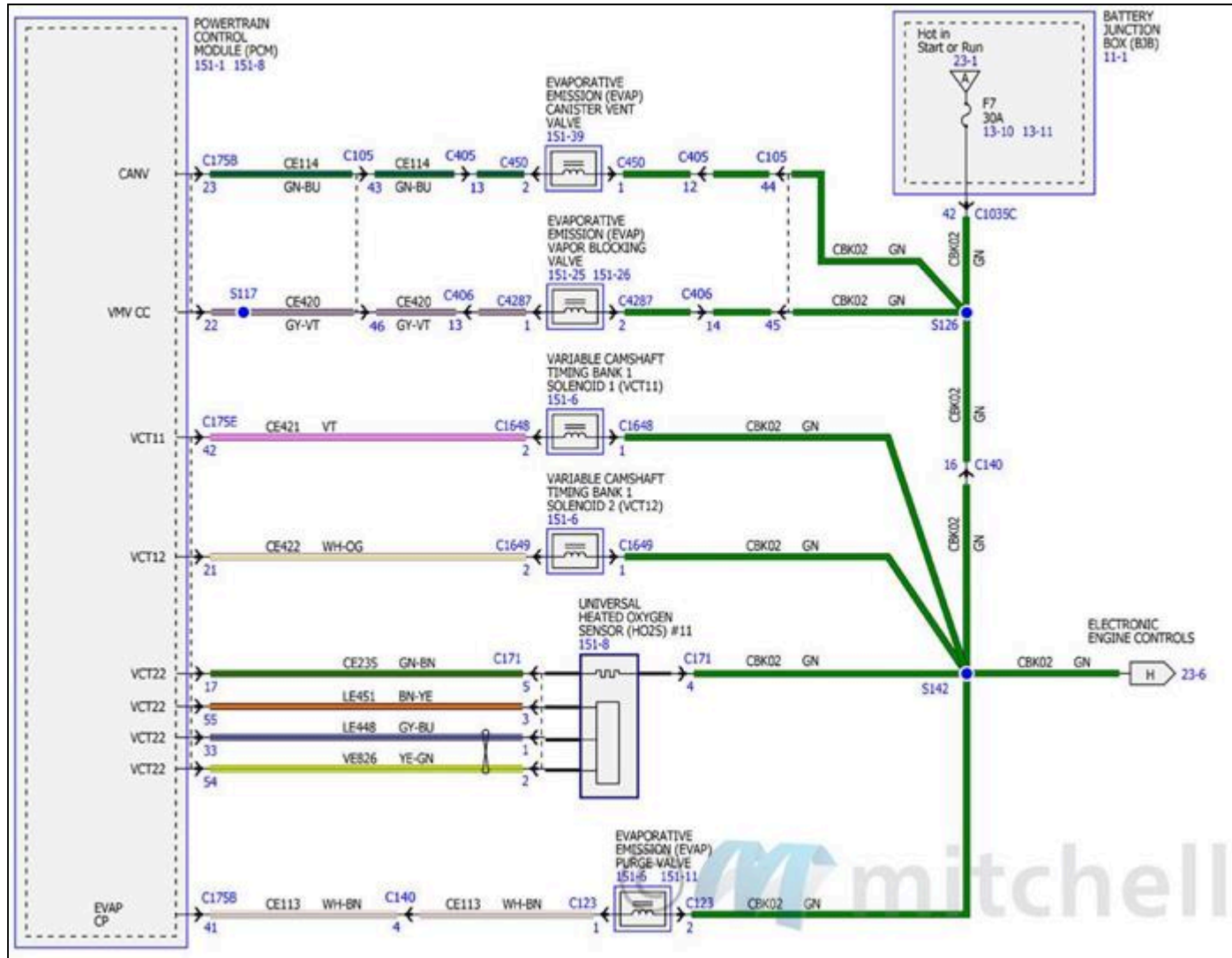
Fig. 49: Electronic Engine Controls Wiring Diagrams - 2.3L (7 Of 17)
