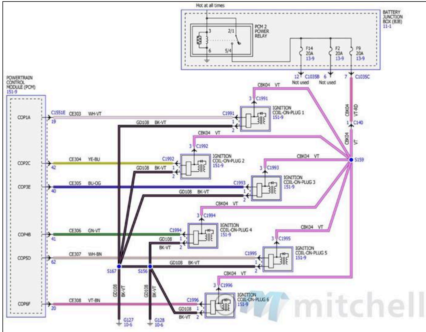
Fig. 61: Electronic Engine Controls Wiring Diagrams - 2.7L (2 Of 18)
