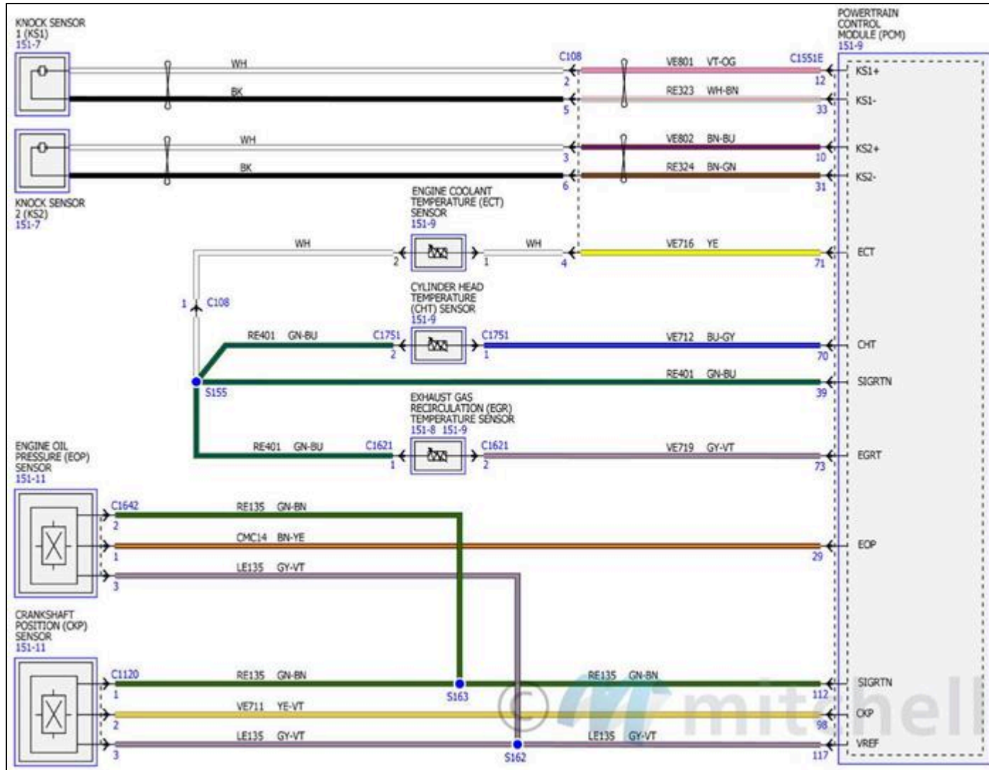
Fig. 64: Electronic Engine Controls Wiring Diagrams - 2.7L (5 Of 18)
