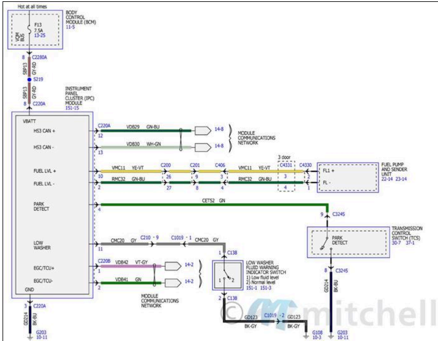
Fig. 94: Instrument Cluster Wiring Diagrams (1 Of 4)
