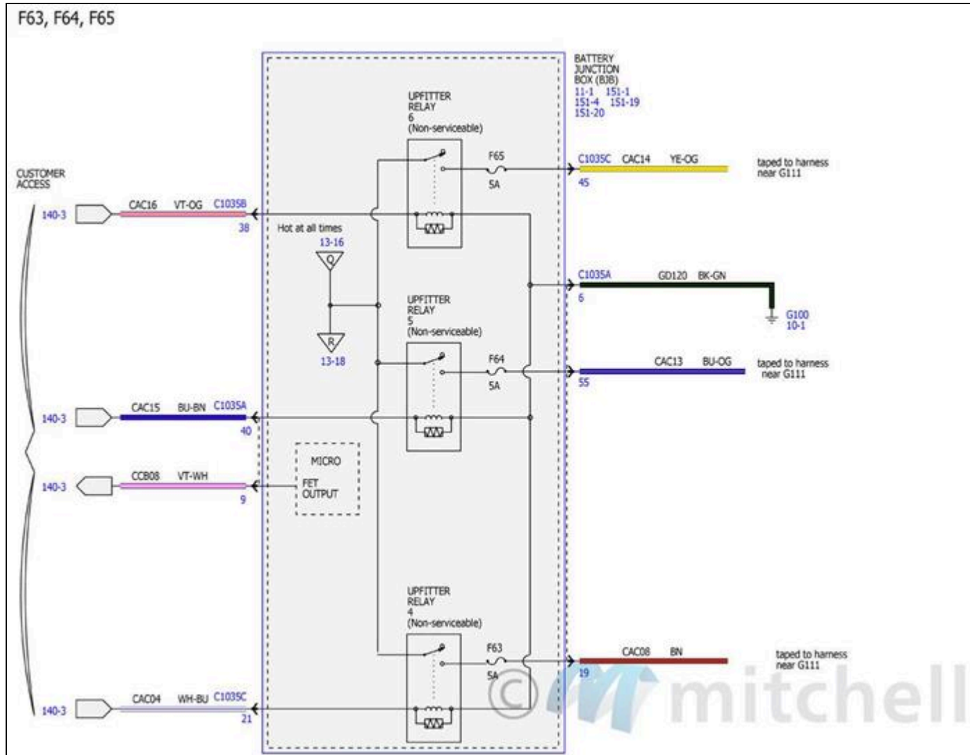
Fig. 146: Power Distribution/BCM Wiring Diagrams (17 Of 34)
