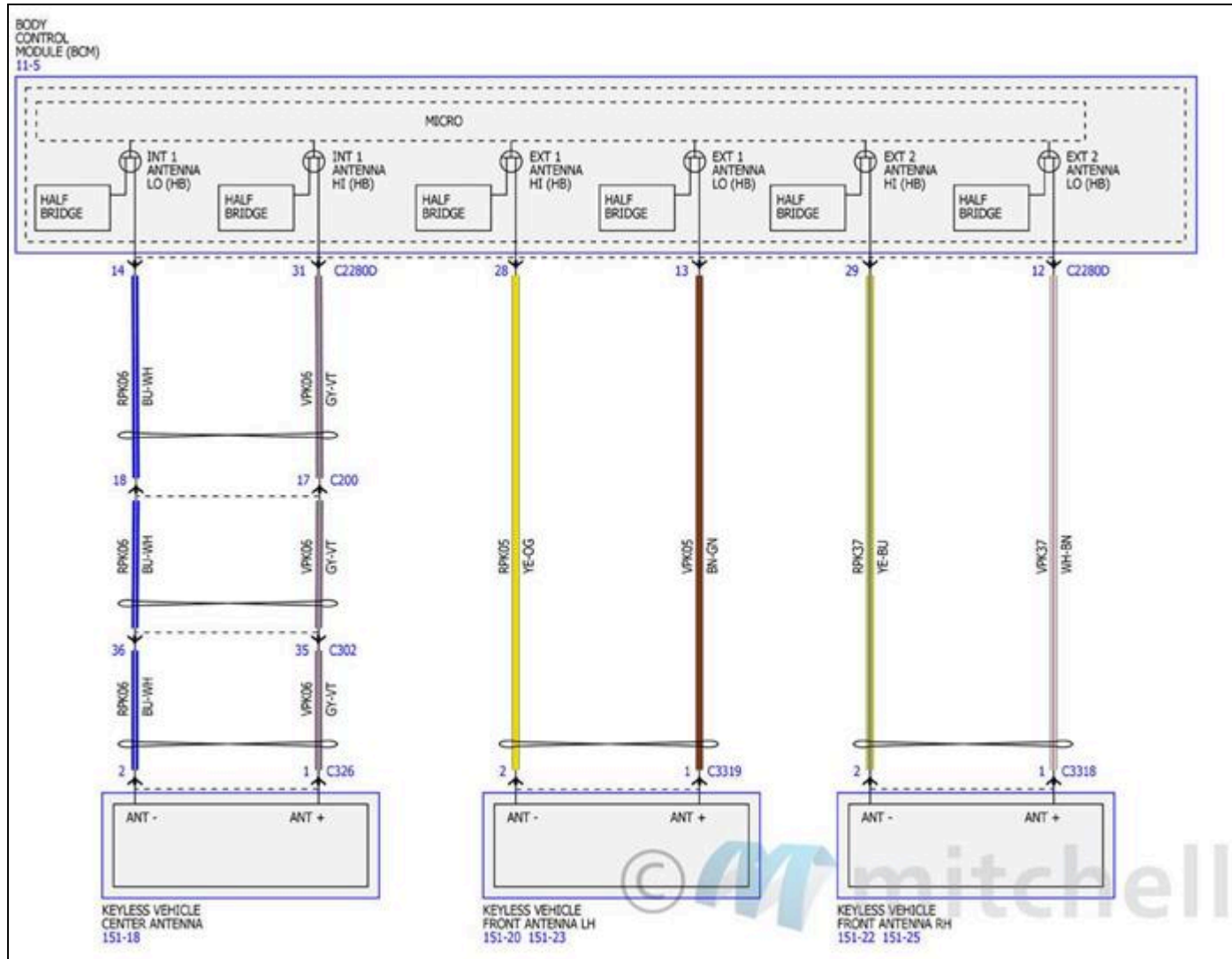
Fig. 128: Passive Anti-Theft System Wiring Diagrams (2 Of 3)
