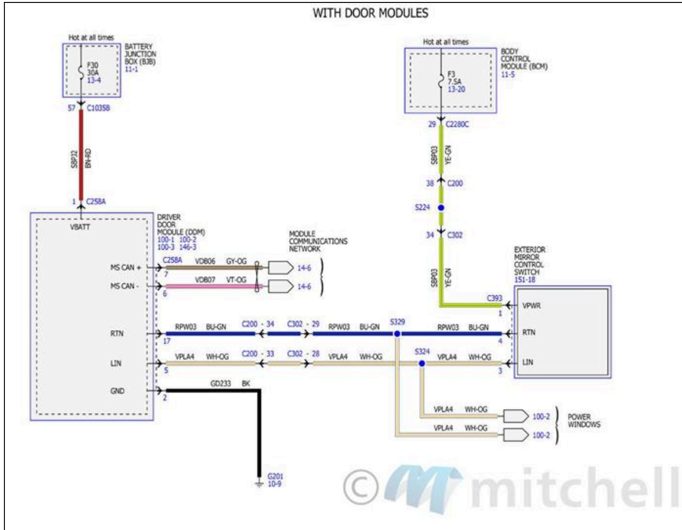
Fig. 164: Power Mirrors Wiring Diagrams (1 Of 4)
