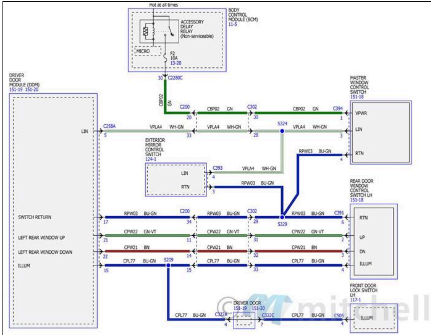
Fig. 172: Power Windows Wiring Diagrams (2 Of 6)
