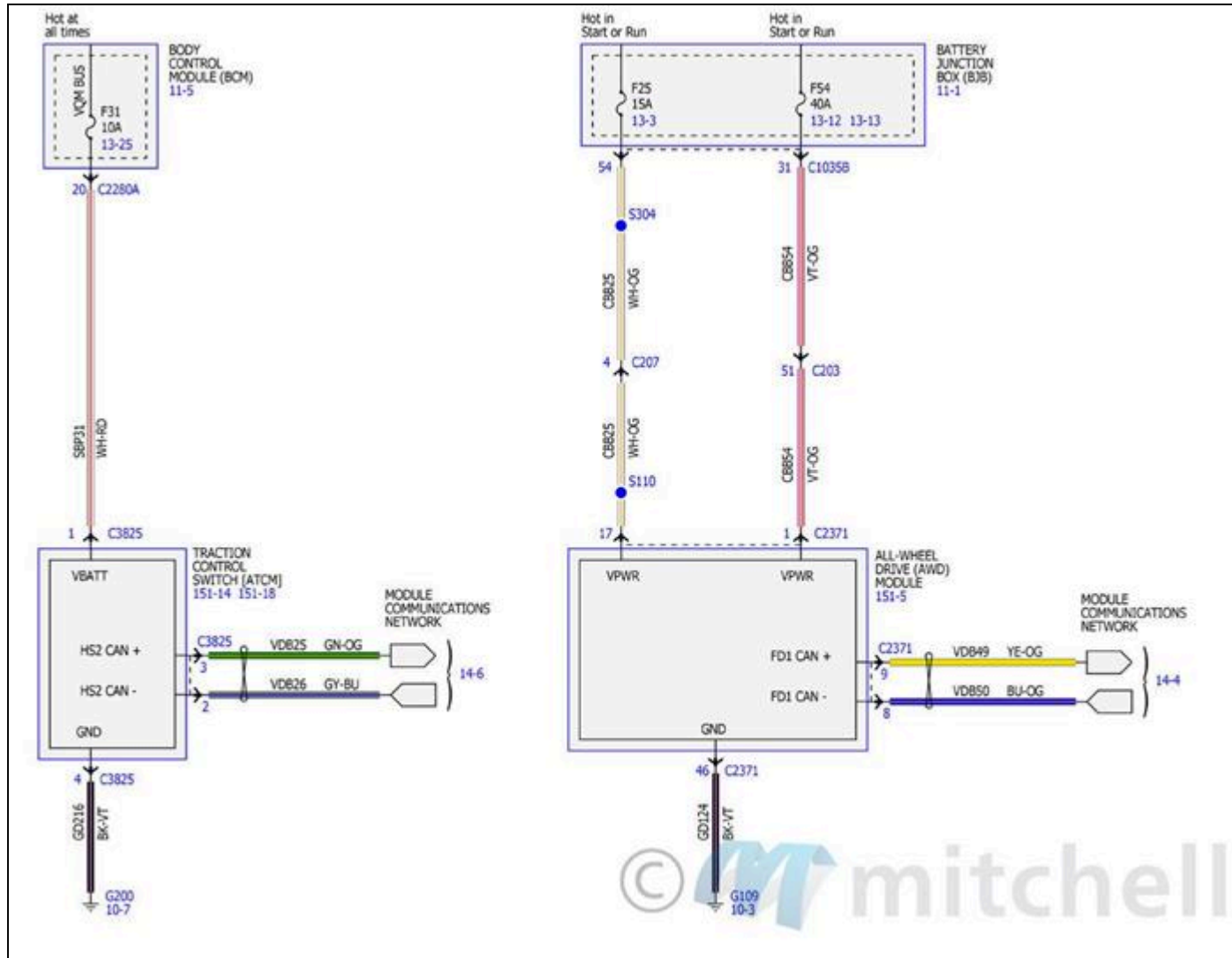
Fig. 80: Four Wheel Drive Systems Wiring Diagrams (1 Of 4)
