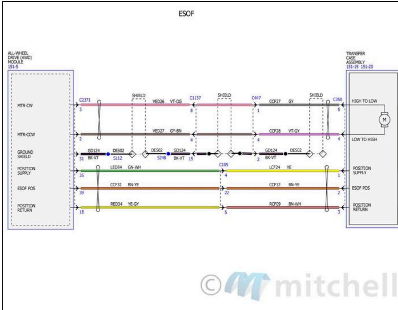
Fig. 81: Four Wheel Drive Systems Wiring Diagrams (2 Of 4)
