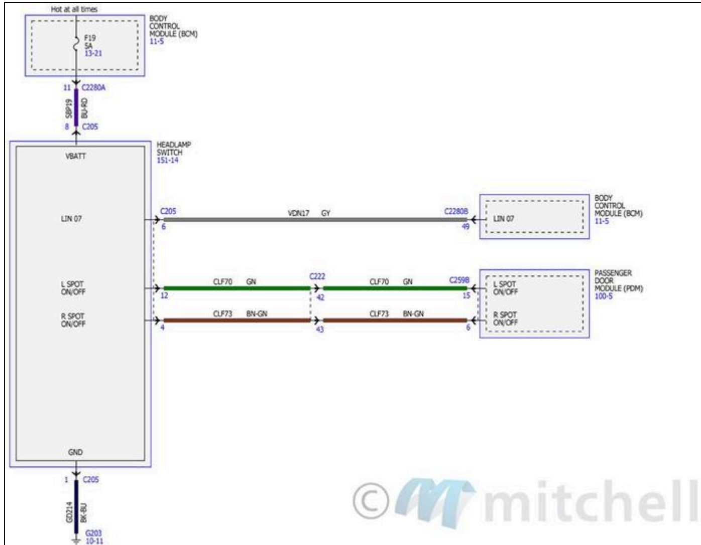
Fig. 84: Headlamps/Autolamps Wiring Diagrams (1 Of 4)
