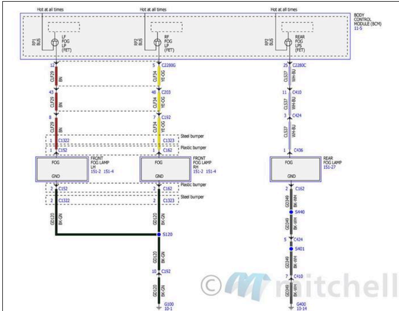
Fig. 79: Fog Lamps Wiring Diagrams (2 Of 2)
