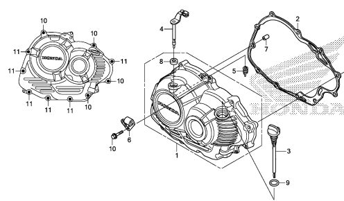
LEFT CRANKCASE COVER
