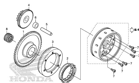
STARTING CLUTCH
