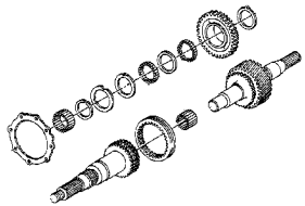
146-400 Gear Train
