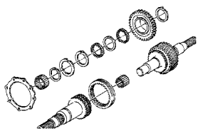
245-400 Gear Train
