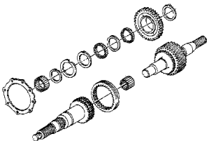
T355-400 Gear Train
