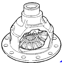
T355-800 Differential
