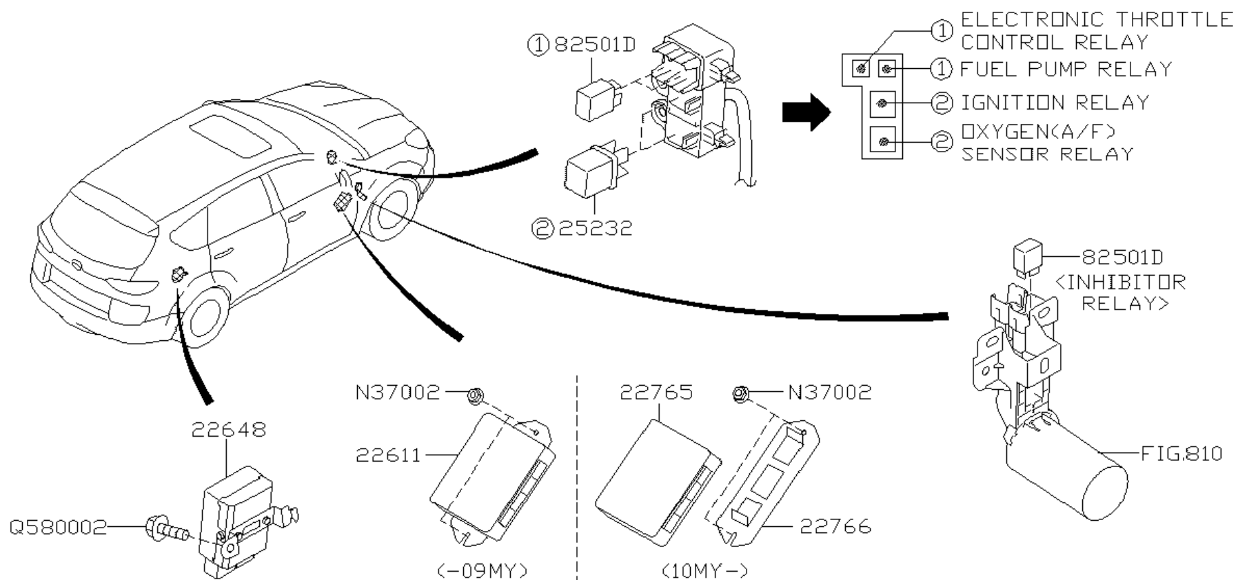
FUEL CONTROL
