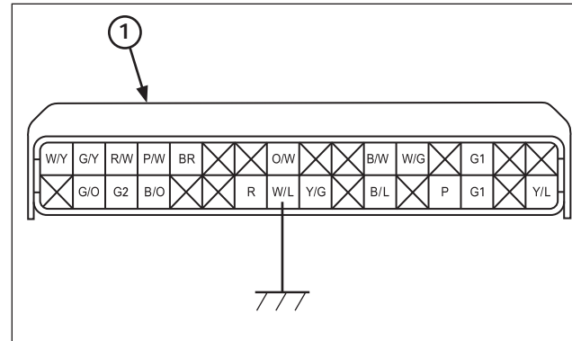
(1) CONECTOR 32P (NEGRO)(FRONTAL)
