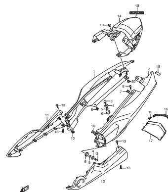
FIG.35 FRAME COVER
