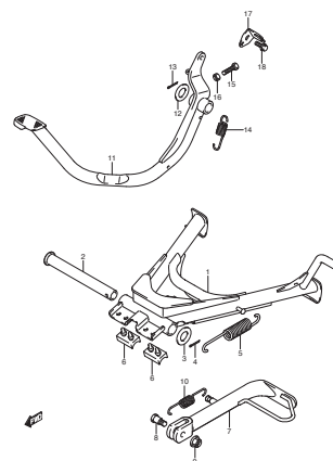
FIG.31 STAND-BRAKE PEDAL
