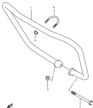
FIG.42 BUMPER
