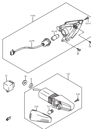
FIG.25 TURN SIGNAL LAMP
