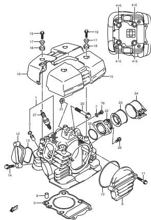
FIG.1 CYLINDER HEAD
