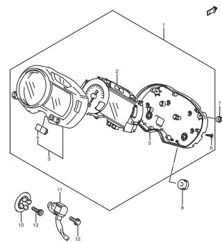
FIG.23 SPEEDOMETER
