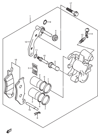
FIG.49 FRONT CALIPER
