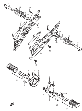
FIG.32 FOOTREST
