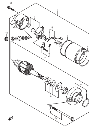
FIG.19 STARTING MOTOR
