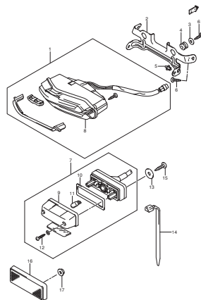
FIG.26 REAR COMBINATION LAMP
