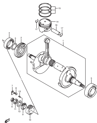
FIG.5 CRANKSHAFT
