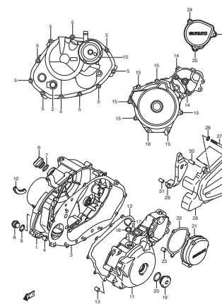
FIG.4 CRANKCASE COVER
