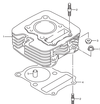
FIG.2 CYLINDER
