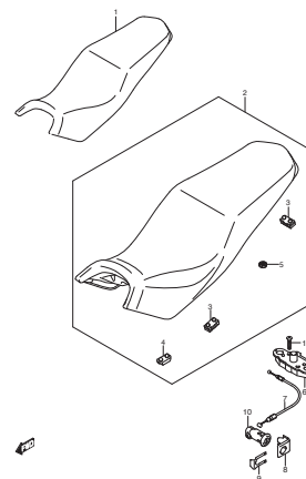
FIG.44 SEAT
