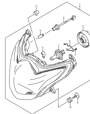
FIG.24 HEADLAMP
