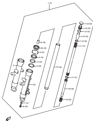
FIG.46 FRONT DAMPER
