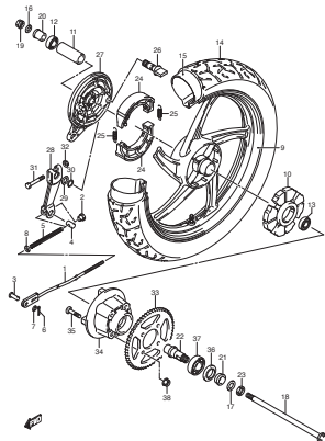
FIG.54 REAR WHEEL
