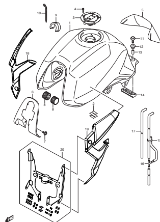
FIG.33 FUEL TANK
