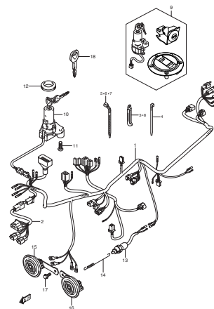
FIG.27 WIRING HARNESS
