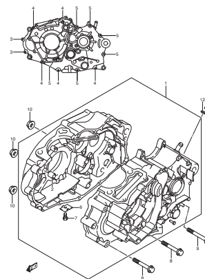
FIG.3 CRANKCASE
