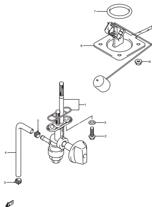
FIG.34 FUEL COCK
