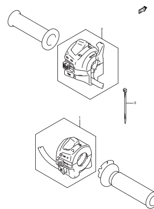
FIG.28 HANDLE SWITCH
