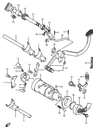
FIG.17 GEAR SHIFTING
