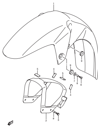
FIG.37 FRONT FENDER
