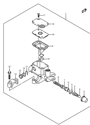
FIG.51 FRONT MASTER CYLINDER
