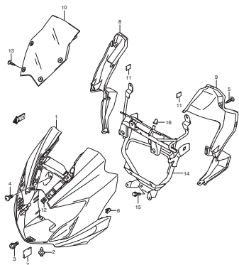
FIG.41 COWLING
