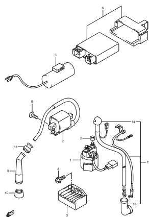
FIG.22 ELECTRICAL
