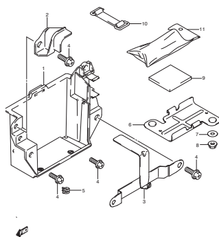
FIG.30 BATTERY HOLDER
