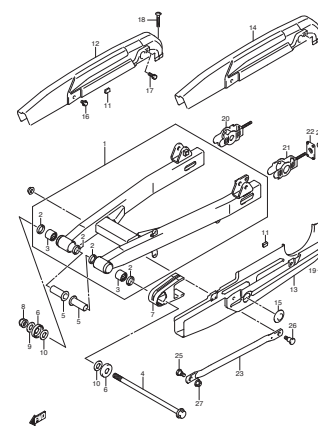
FIG.52 REAR SWINGARM
