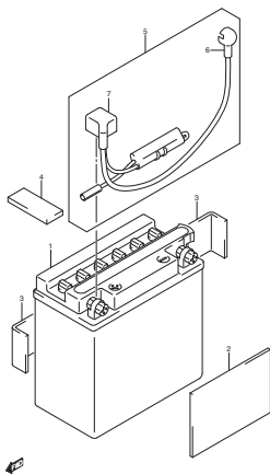
FIG.21 BATTERY
