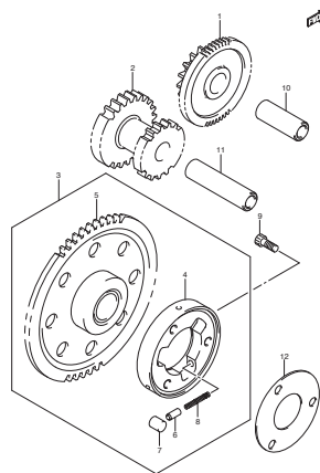
FIG.6 STARTER CLUTCH
