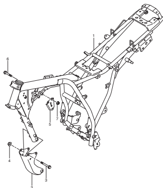
FIG.29 FRAME
