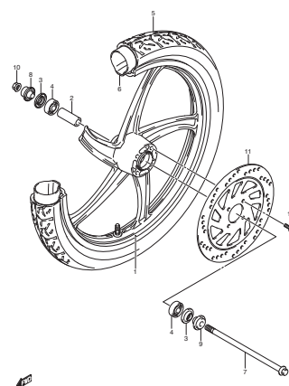
FIG.48 FRONT WHEEL
