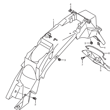
FIG.40 REAR FENDER
