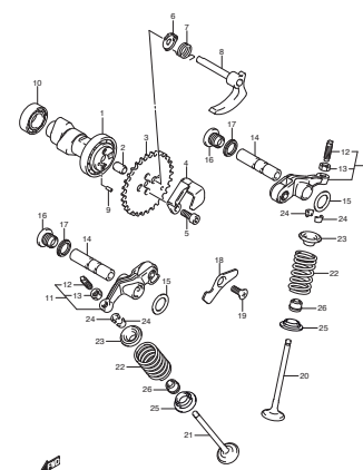
FIG.8 CAM SHAFT/VALVE
