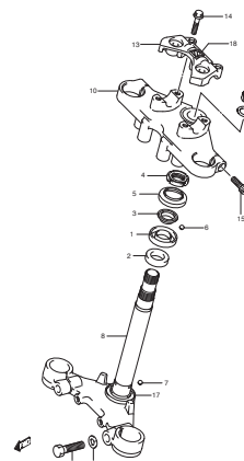
FIG.47 STEERING STEM
