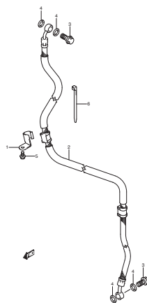
FIG.50 FRONT BRAKE HOSE
