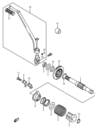
FIG.18 KICK STARTER
