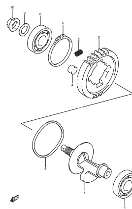
FIG.7 CRANK BALANCER
