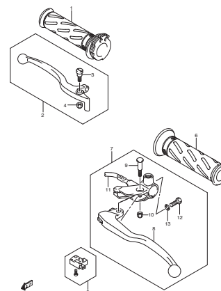
FIG.39 HANDLE LEVER
