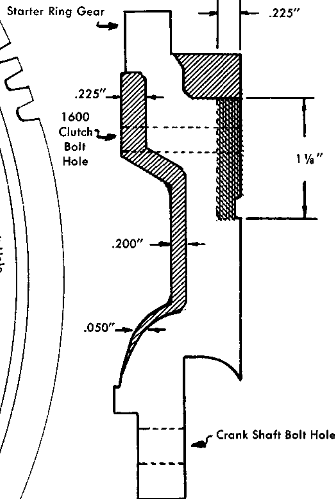
Figure 5 — Cross section of Datsun 1600 flywheel. Shaded area indicates metal removed to lighten unit to 13 lbs.
