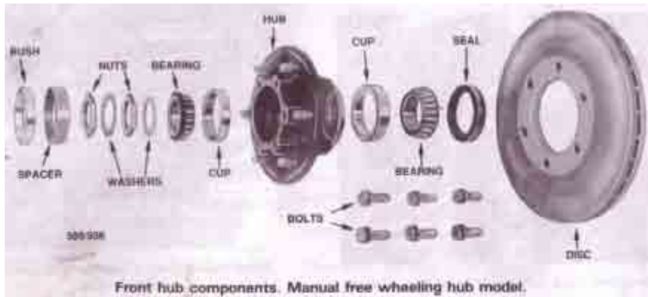
Front hub components. Manual free wheeling hub model.
