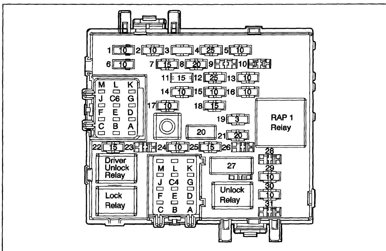
Fuse Block-Left I/P
