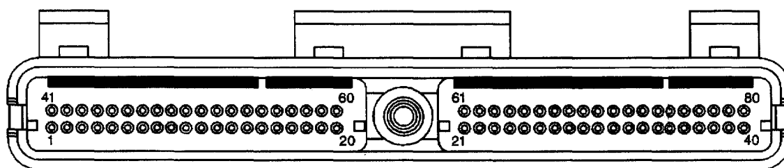
Powertrain Control Module (PCM) C2
