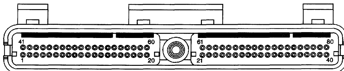
Powertrain Control Module (PCM) C1
