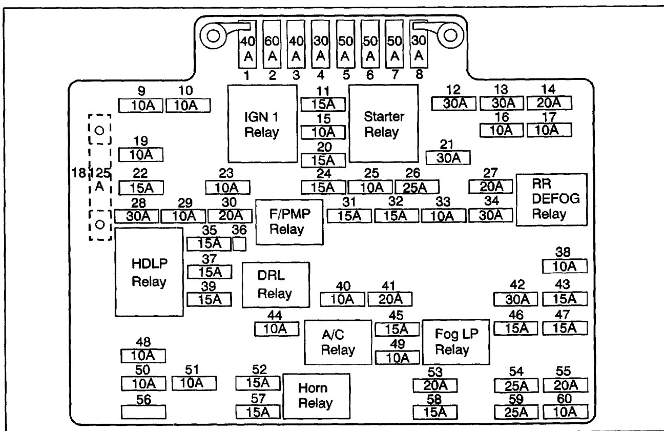
Fuse Block-Underhood
