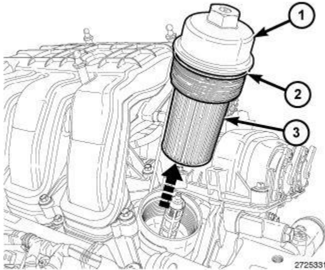
Fig. 487: Oil Filter Cap, O-Ring Seal & Oil Filter Courtesy of CHRYSLER GROUP, LLC
