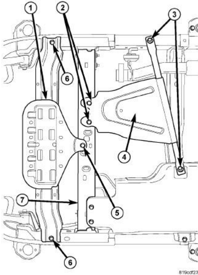
Fig. 452: Crossmember, Skid Plates & Fasteners Courtesy of CHRYSLER GROUP, LLC
