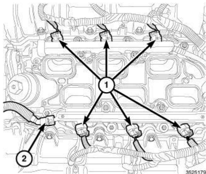
Fig. 597: Fuel Supply Line And Connectors Courtesy of CHRYSLER GROUP, LLC
