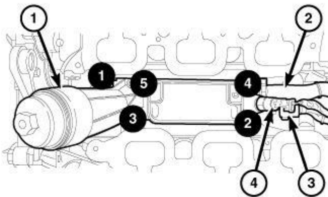
Fig. 553: Heater Hose, Electrical Connectors, Oil Filter Housing & Bolt Tightening Sequence Courtesy of CHRYSLER GROUP, LLC
