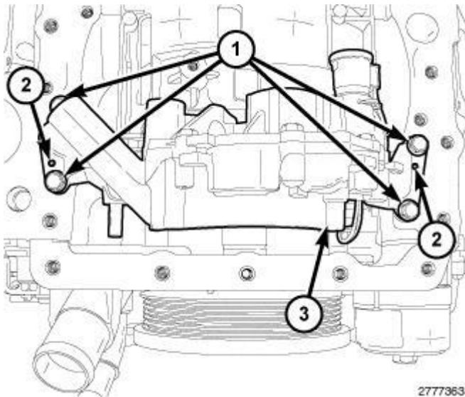
Fig. 534: Oil Pump, Locator Pins & Bolts Courtesy of CHRYSLER GROUP, LLC
