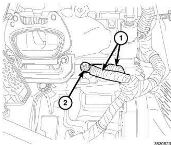
Fig. 50: Ground Straps & Nut
