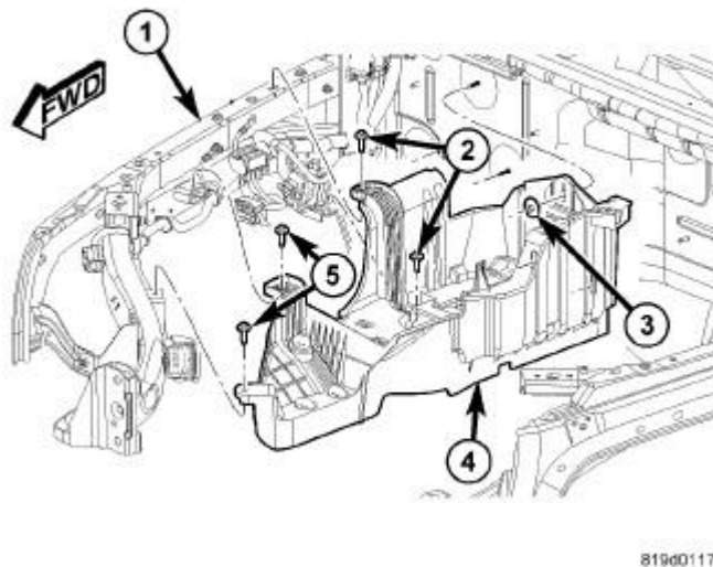
Fig. 72: Battery Tray Components Courtesy of CHRYSLER GROUP, LLC
