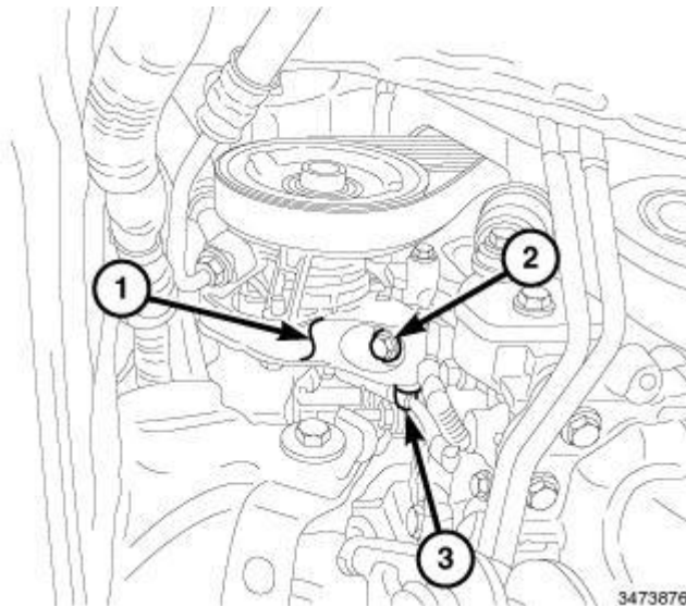
Fig. 19: Power Steering Pump Bracket, Bolt & Retainer Courtesy of CHRYSLER GROUP, LLC
