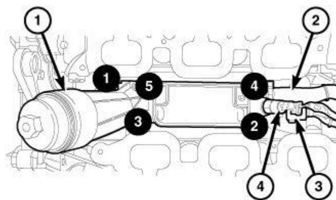
Fig. 480: Heater Hose, Electrical Connectors, Oil Filter Housing & Bolt Tightening Sequence Courtesy of CHRYSLER GROUP, LLC
