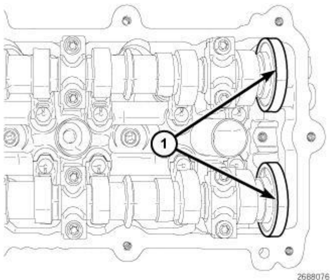
Fig. 210: Magnetic Timing Wheels
