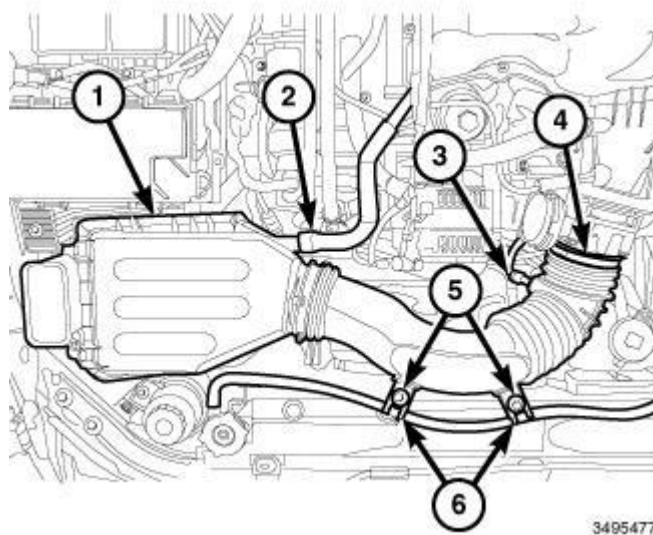
Fig. 646: Air Cleaner Body, Fresh Air Makeup Hose, Electrical Connector, Clamp, Bolts & Retainers
