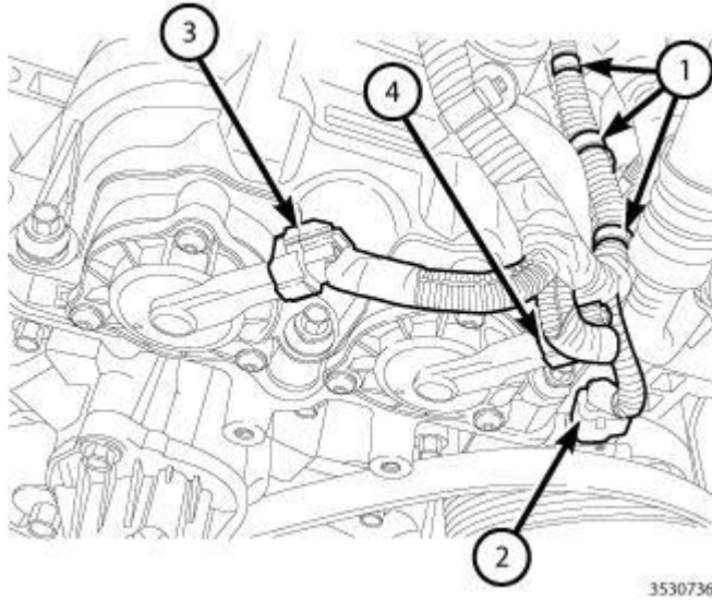
Fig. 24: Retainers, A/C Compressor Electrical Connector & Left Intake And Left Exhaust Variable Valve Timing Solenoid Electrical Connectors Courtesy of CHRYSLER GROUP, LLC
