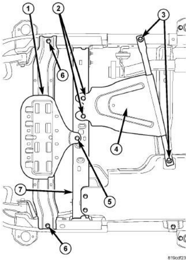
Fig. 445: Crossmember, Skid Plates & Fasteners Courtesy of CHRYSLER GROUP, LLC
