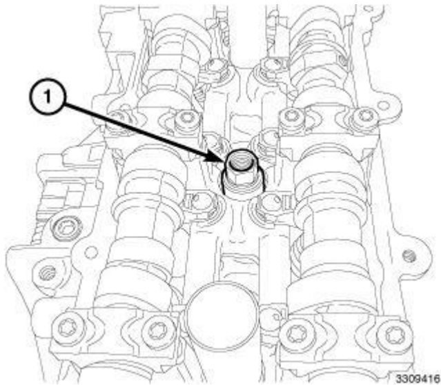
Fig. 316: Spark Plug Tube Installer Courtesy of CHRYSLER GROUP, LLC
