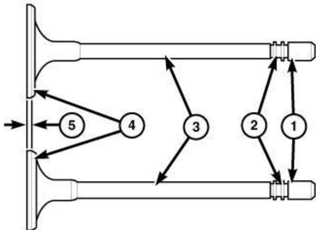
Fig. 332: Inspecting Valve Margin
