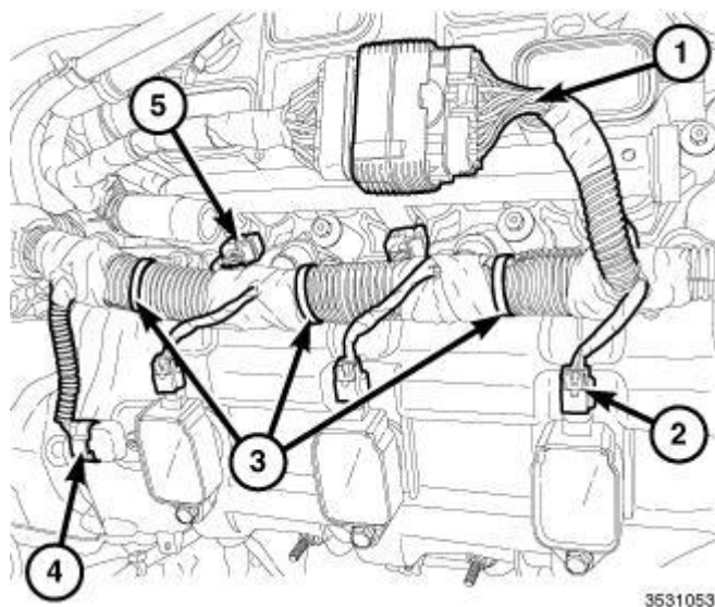
Fig. 22: Engine Injection/Ignition Harness, Ignition Coil Electrical Connectors, Retainers, Camshaft Position (CMP) Sensor Connector & Fuel Injector Electrical Connectors Courtesy of CHRYSLER GROUP, LLC
