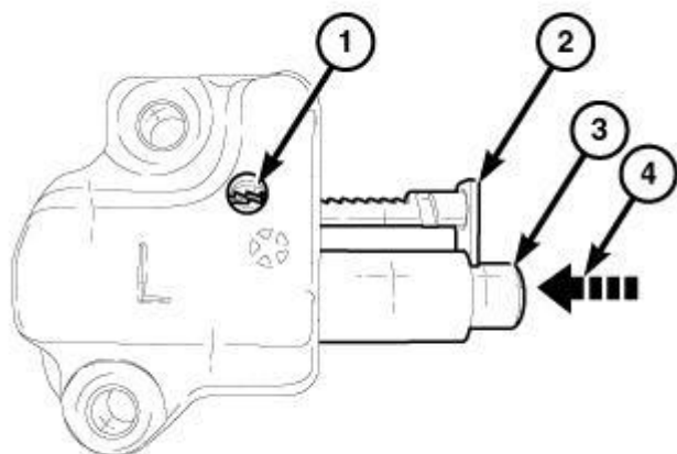
Fig. 603: Left Side Cam Chain Tensioner Ratchet Components Courtesy of CHRYSLER GROUP, LLC
