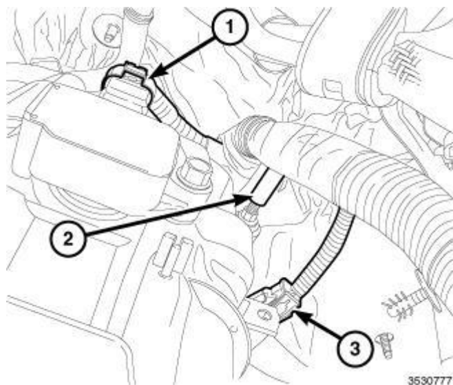
Fig. 54: Camshaft Position (CMP) Sensor, Retainer & Engine Coolant Temperature (ECT) Sensor Connector
