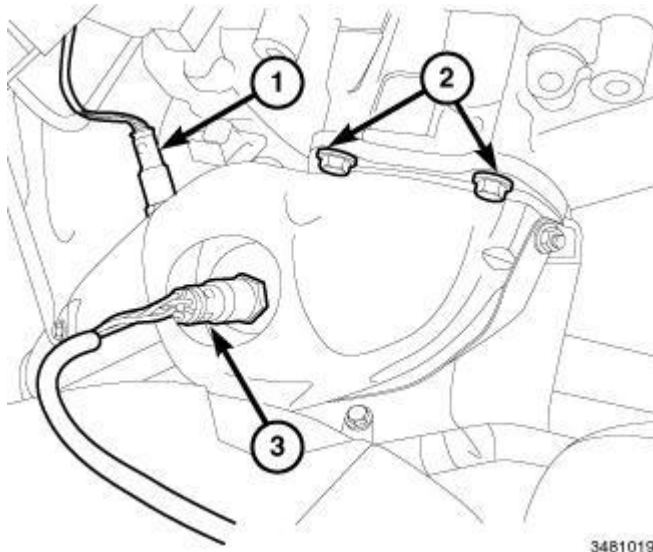
Fig. 110: Right And Left Upstream And Downstream Oxygen Sensor Connectors & Bolts Courtesy of CHRYSLER GROUP, LLC
