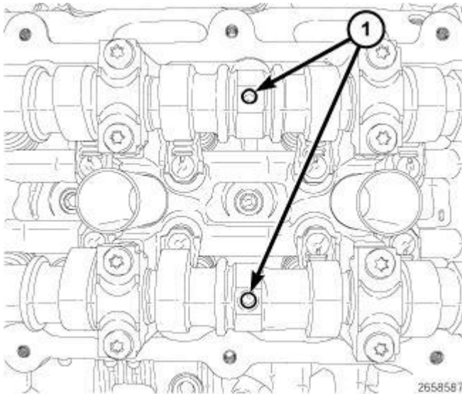
Fig. 631: Positioning Camshaft Alignment Holes Vertically Courtesy of CHRYSLER GROUP, LLC
