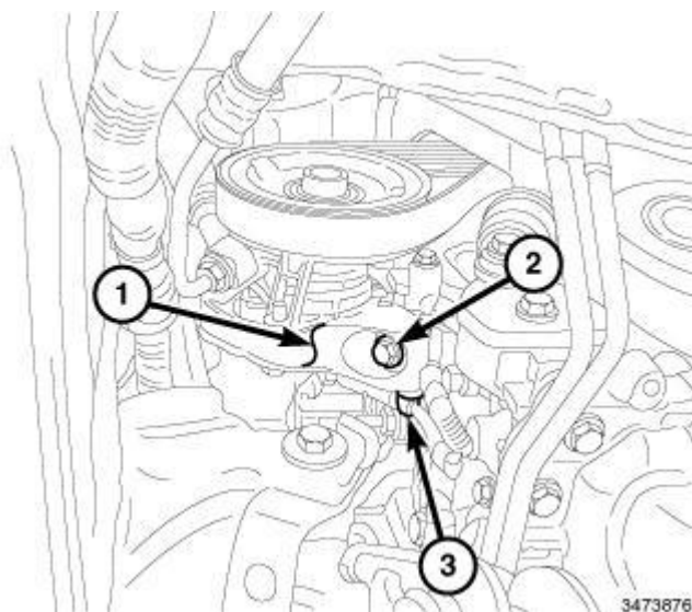
Fig. 156: Power Steering Pump Bracket, Bolt & Retainer Courtesy of CHRYSLER GROUP, LLC
