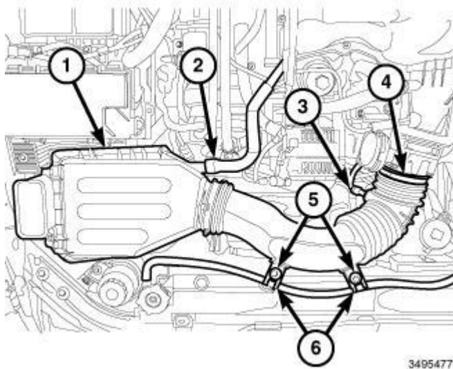
Fig. 558: Air Cleaner Body, Fresh Air Makeup Hose, Electrical Connector, Clamp, Bolts & Retainers
