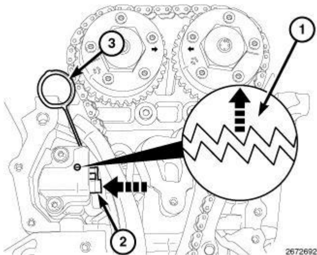
Fig. 618: Resetting Left Cam Chain Tensioner Courtesy of CHRYSLER GROUP, LLC
