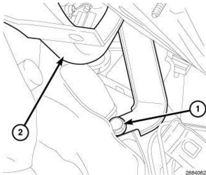
Fig. 263: Upper Transmission-To-Engine Bolt & Transmission Oil Level Indicator Tube Courtesy of CHRYSLER GROUP, LLC
