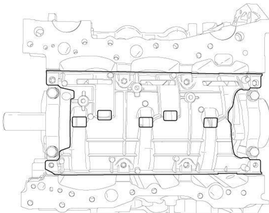
Fig. 494: Windage Tray
