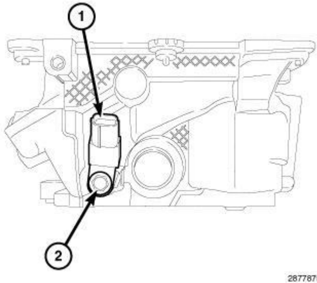
Fig. 123: Ignition Coil Capacitor & Bolt Courtesy of CHRYSLER GROUP, LLC
