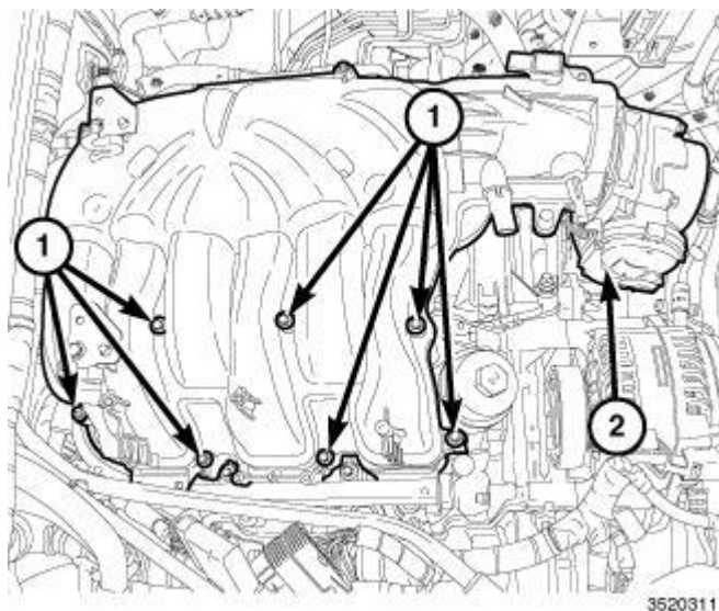
Fig. 211: Upper Intake Manifold & Fasteners
