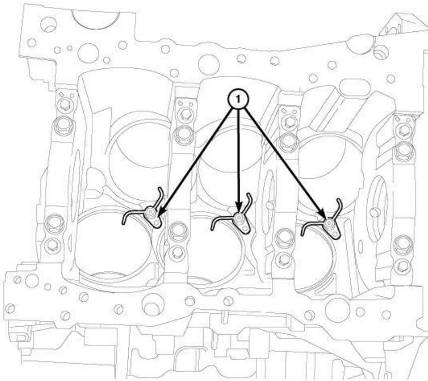
Fig. 481: Engine Blocked-Mounted Oil Jets Courtesy of CHRYSLER GROUP, LLC
