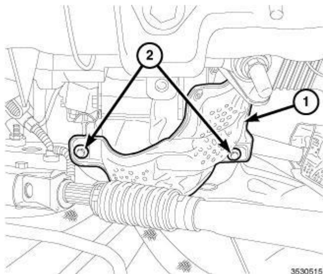
Fig. 33: Engine Mount Heatshield & Bolts Courtesy of CHRYSLER GROUP, LLC
