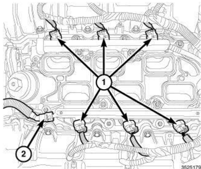
Fig. 572: Fuel Supply Line And Connectors
