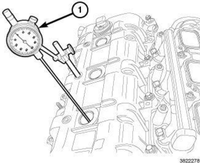
Fig. 183: Mount Dial Indicator Set To Stationary Point On Engine
