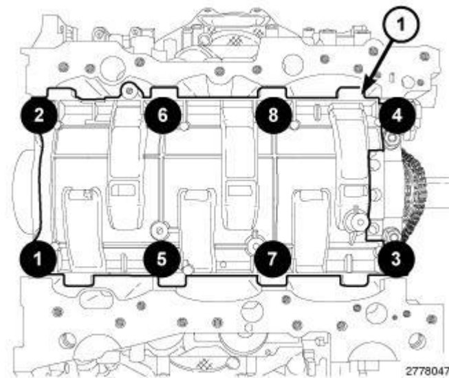
Fig. 360: Main Bearing Cap Bolts From Windage Tray Removal Sequence Courtesy of CHRYSLER GROUP, LLC
