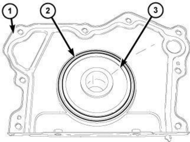
Fig. 429: Rear Crankshaft Oil Seal, Retainer & Seal Protector
