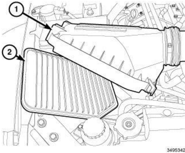
Fig. 79: Air Cleaner Housing Cover & Air Cleaner Element Courtesy of CHRYSLER GROUP, LLC
