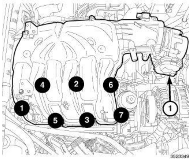
Fig. 267: Upper Intake Manifold Tightening Sequence Courtesy of CHRYSLER GROUP, LLC
