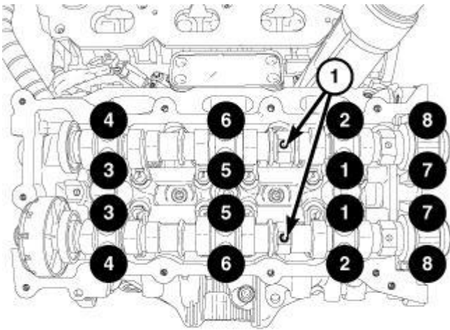
Fig. 208: Bearing Cap Retaining Bolts Tightening Sequence - Right Courtesy of CHRYSLER GROUP, LLC
