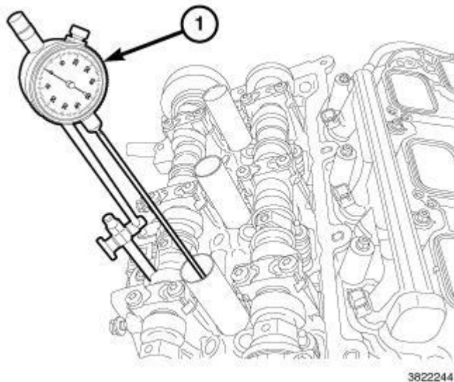
Fig. 610: Mount Dial Indicator Set To Stationary Point On Engine Courtesy of CHRYSLER GROUP, LLC
