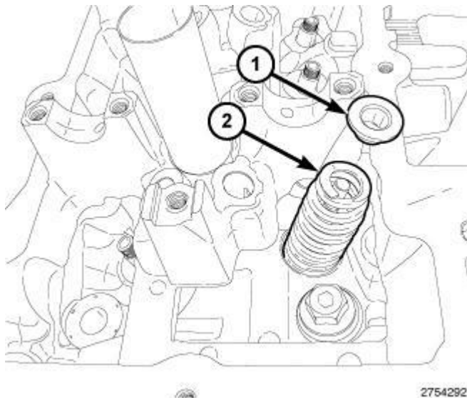
Fig. 299: Valve Spring & Valve Spring Retainer Courtesy of CHRYSLER GROUP, LLC
