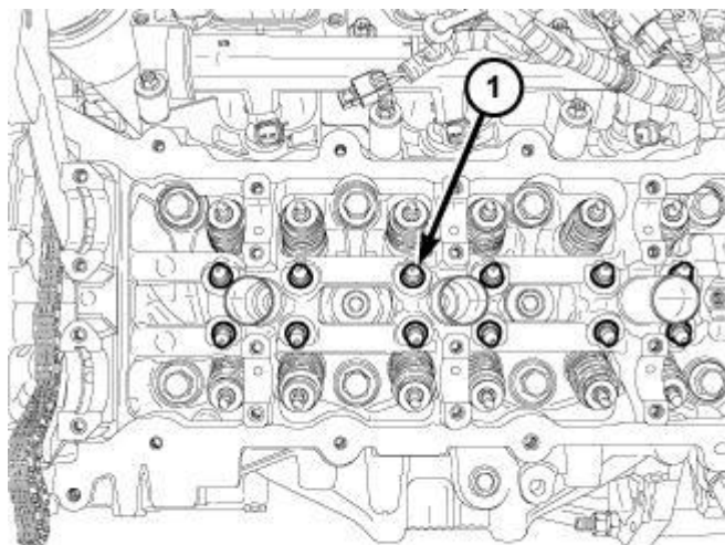
Fig. 268: Hydraulic Lifters
