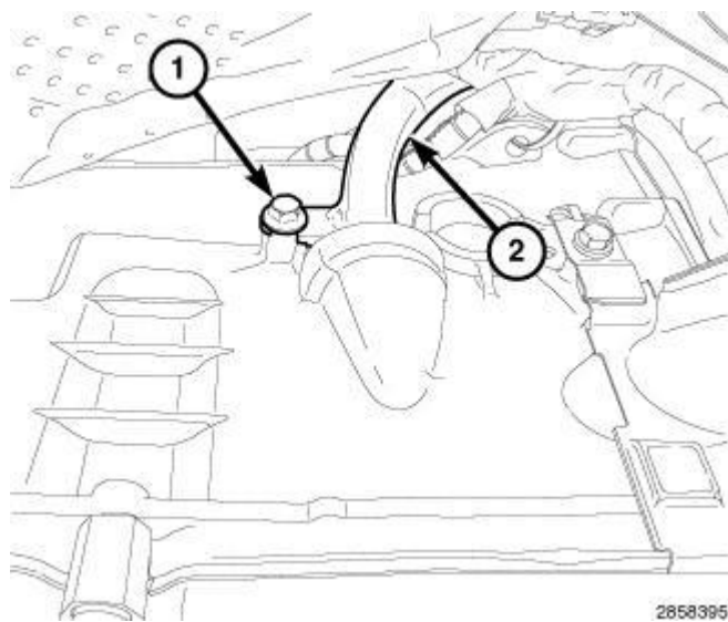
Fig. 264: Transmission Fluid Level Indicator Tube & Bolt Courtesy of CHRYSLER GROUP, LLC
