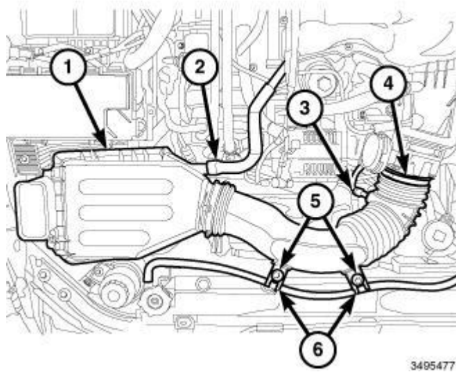
Fig. 591: Air Cleaner Body, Fresh Air Makeup Hose, Electrical Connector, Clamp, Bolts & Retainers
