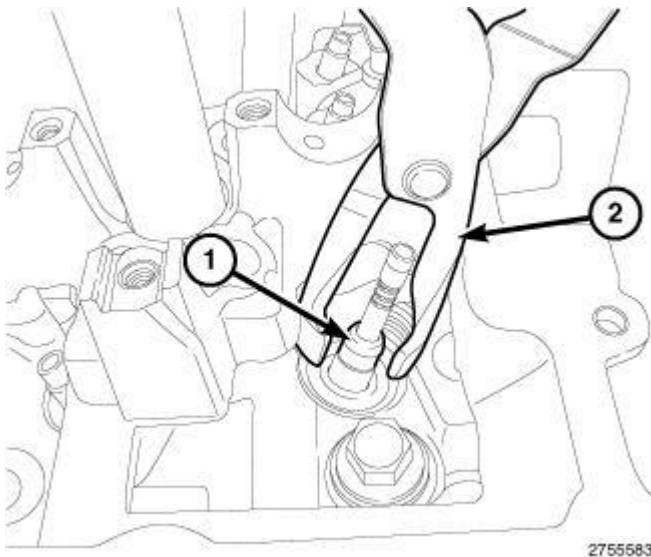
Fig. 276: Valve Guide Seal & Valve Seal Tool Courtesy of CHRYSLER GROUP, LLC
