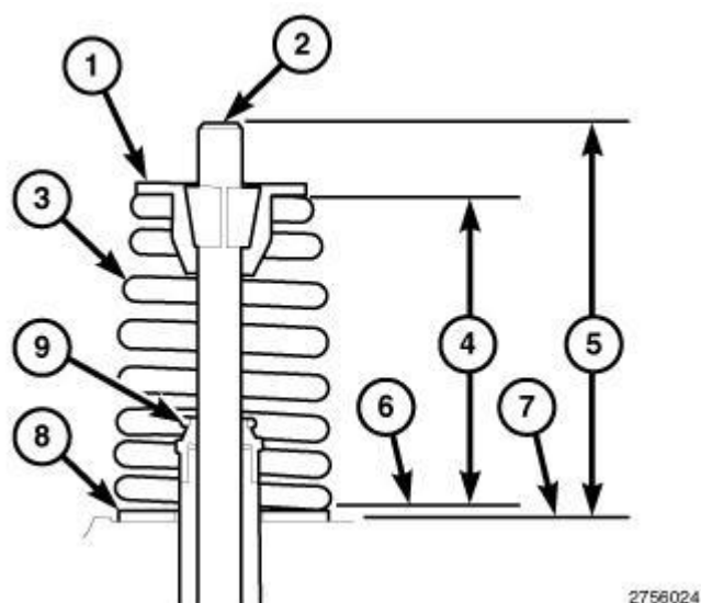
Fig. 297: Checking Valve Spring Installed Height
