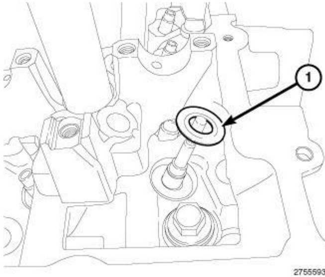
Fig. 277: Valve Spring Seat
