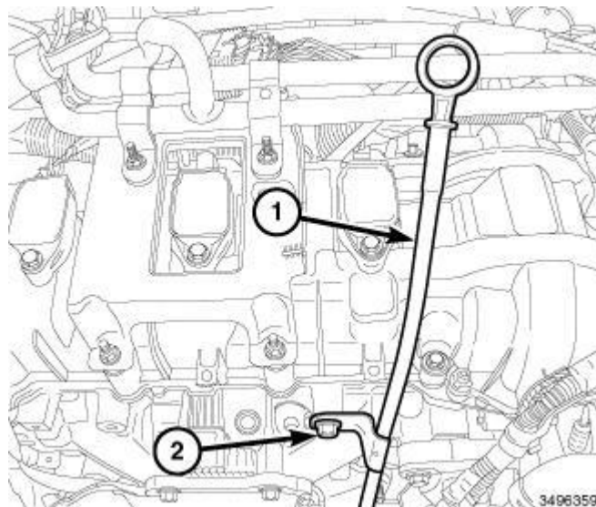
Fig. 262: Oil Level Indicator & Bolt
