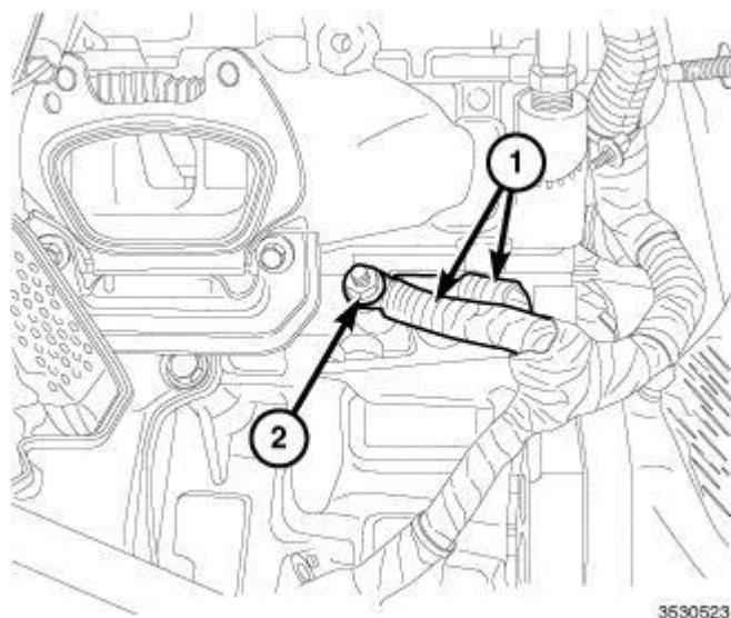
Fig. 27: Ground Straps & Nut Courtesy of CHRYSLER GROUP, LLC
