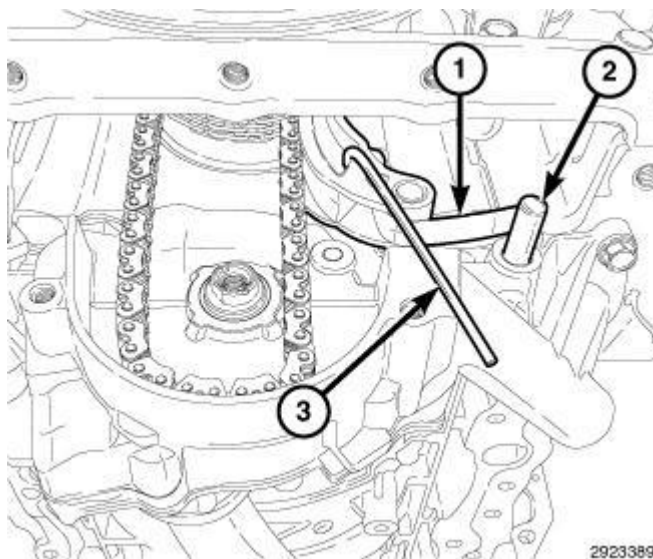
Fig. 535: Retaining Pin, Oil Pump Chain Tensioner Spring & Dowel Pin Courtesy of CHRYSLER GROUP, LLC
