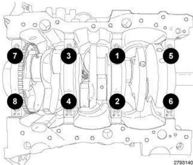
Fig. 385: Inner Main Bearing Cap Bolts Tightening Sequence
