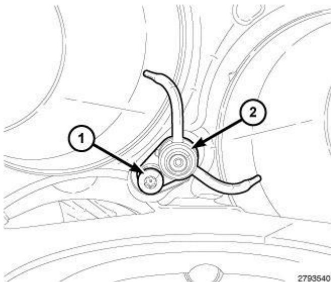
Fig. 482: Piston Oil Cooler Jet & Bolt Courtesy of CHRYSLER GROUP, LLC
