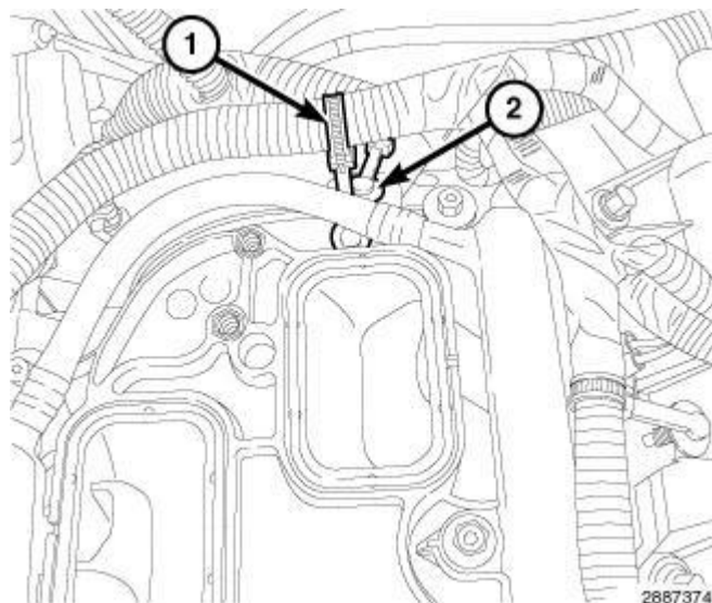
Fig. 596: Injection/Ignition Harness Retainer & Main Wire Harness Retainer Courtesy of CHRYSLER GROUP, LLC
