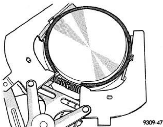
Fig. 404: Removing/Installing Upper & Intermediate Rings Courtesy of CHRYSLER GROUP, LLC
