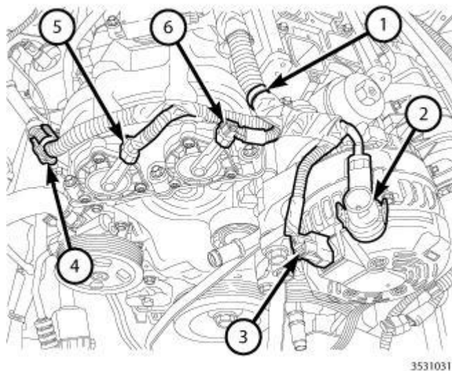
Fig. 258: Generator Stud, Connector, Retainers & Right Exhaust And Right Intake Variable Valve Timing Solenoid Electrical Connectors Courtesy of CHRYSLER GROUP, LLC
