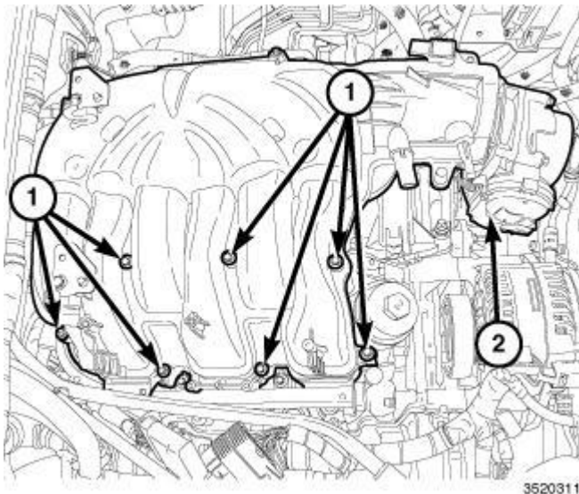
Fig. 287: Upper Intake Manifold & Fasteners Courtesy of CHRYSLER GROUP, LLC
