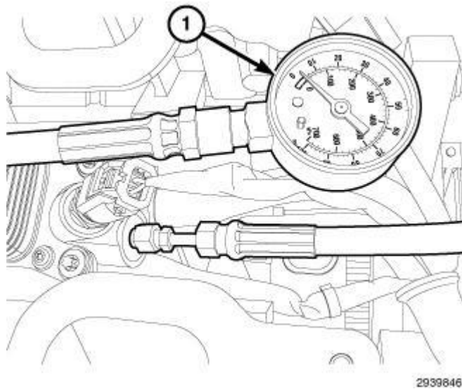
Fig. 456: Pressure Gauge Installed To Oil Pressure Port Courtesy of CHRYSLER GROUP, LLC
