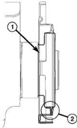
Fig. 431: Rear Seal Installed Courtesy of CHRYSLER GROUP, LLC
