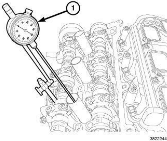
Fig. 190: Mount Dial Indicator Set To Stationary Point On Engine Courtesy of CHRYSLER GROUP, LLC
