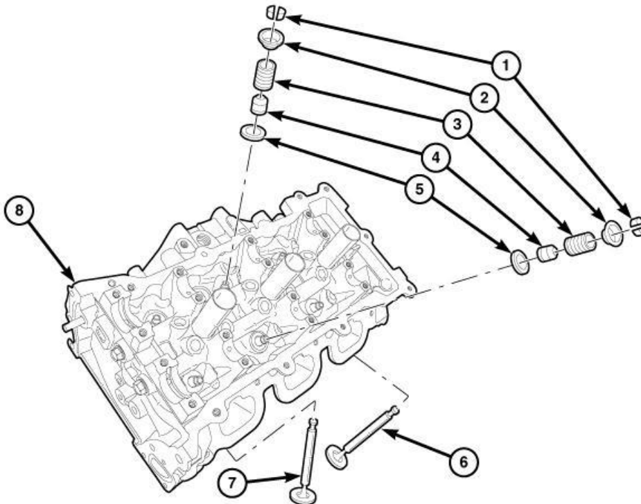
Fig. 320: Intake Valve & Exhaust Valve Component Configuration Courtesy of CHRYSLER GROUP, LLC
