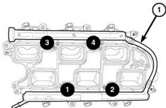
Fig. 594: Fuel Rail Bolt Tightening Sequence
