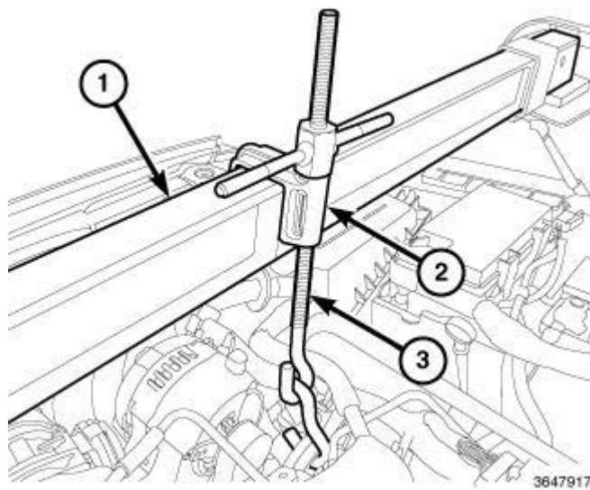
Fig. 357: Engine Support Fixture & Adapters Courtesy of CHRYSLER GROUP, LLC
