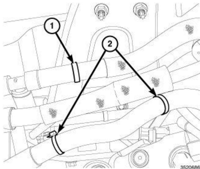
Fig. 562: Brake Booster Hose Retainer & Wire Harness Retainers Courtesy of CHRYSLER GROUP, LLC
