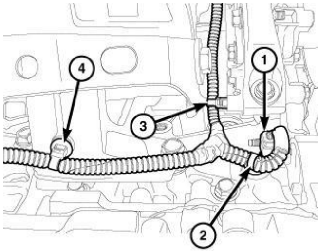
Fig. 442: Oil Pump Solenoid Electrical Connector & Wire Harness Retainers Courtesy of CHRYSLER GROUP, LLC
