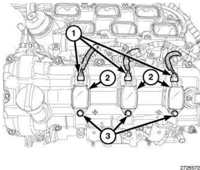
Fig. 229: Electrical Connector, Ignition Coils & Ignition Coil Retaining Bolts
