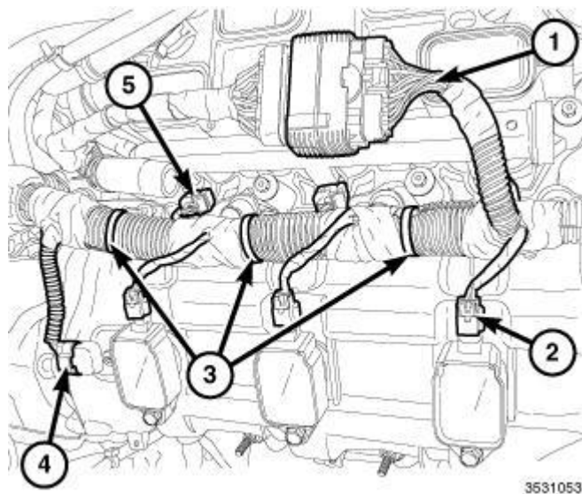
Fig. 260: Engine Injection/Ignition Harness, Ignition Coil Electrical Connectors, Retainers, Camshaft Position (CMP) Sensor Connector & Fuel Injector Electrical Connectors Courtesy of CHRYSLER GROUP, LLC
