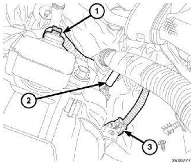
Fig. 214: Camshaft Position (CMP) Sensor, Retainer & Engine Coolant Temperature (ECT) Sensor Connector
