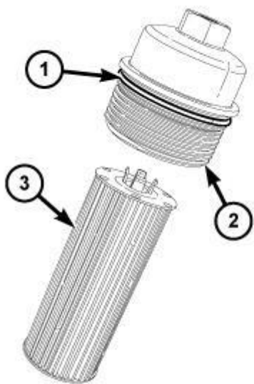
Fig. 467: O-Ring Seal, Oil Filter Cap & Oil Filter Courtesy of CHRYSLER GROUP, LLC
