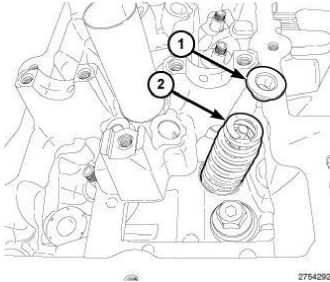
Fig. 280: Valve Spring & Valve Spring Retainer Courtesy of CHRYSLER GROUP, LLC
