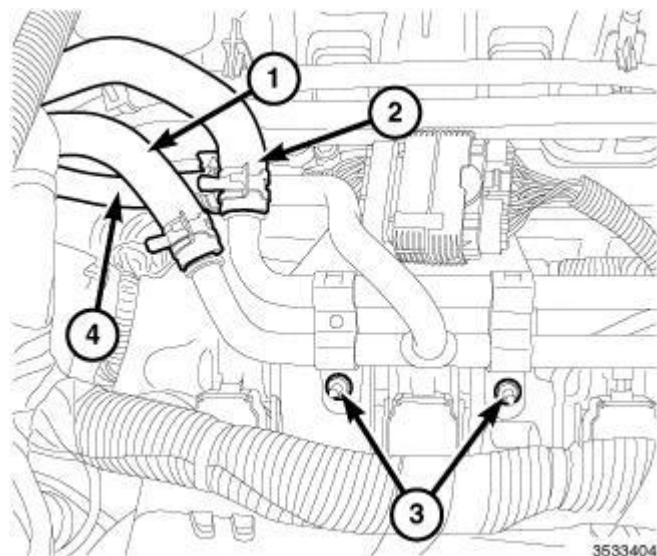
Fig. 649: Heater Core Return Hose, Heater Core Supply Hose, Nuts & Oil Cooler Return Hose Courtesy of CHRYSLER GROUP, LLC
