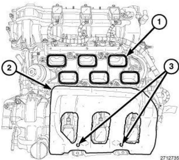
Fig. 249: Intake Ports, Insulator & Alignment Posts Courtesy of CHRYSLER GROUP, LLC
