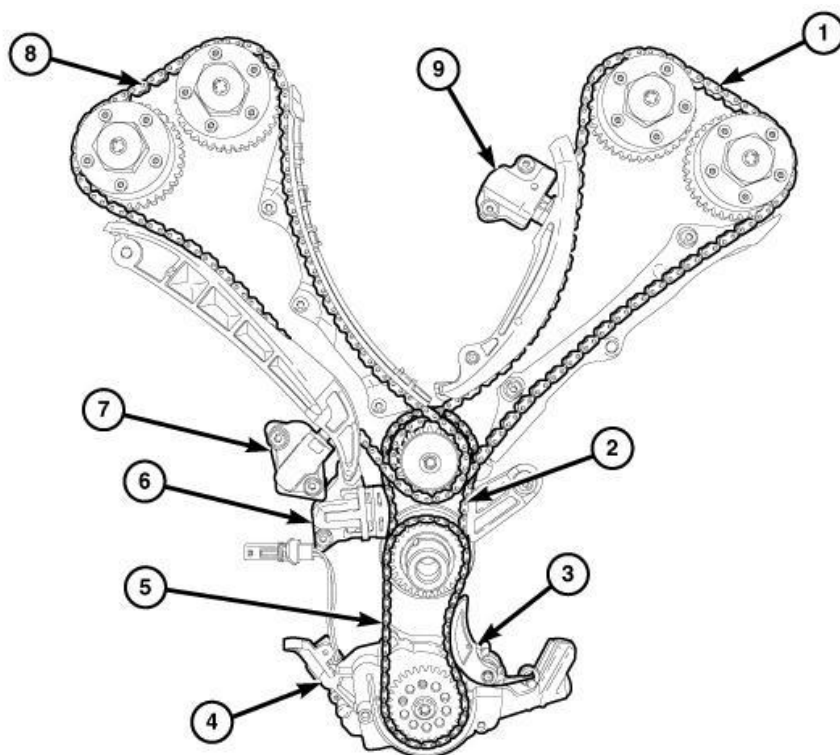
Fig. 600: Valve Timing System Components Courtesy of CHRYSLER GROUP, LLC
