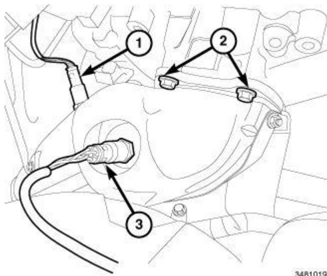
Fig. 52: Right And Left Upstream And Downstream Oxygen Sensor Connectors & Bolts Courtesy of CHRYSLER GROUP, LLC
