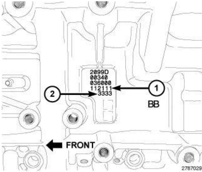
Fig. 407: Engine Block Cylinder Bore Diameter Grade Markings & Engine Block Main Bearing Journal Diameter Grade Markings
