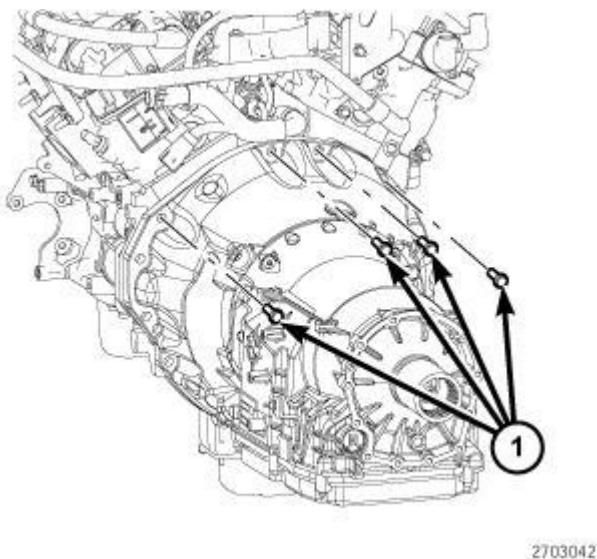
Fig. 45: Upper Transmission Engine Bolts Courtesy of CHRYSLER GROUP, LLC
