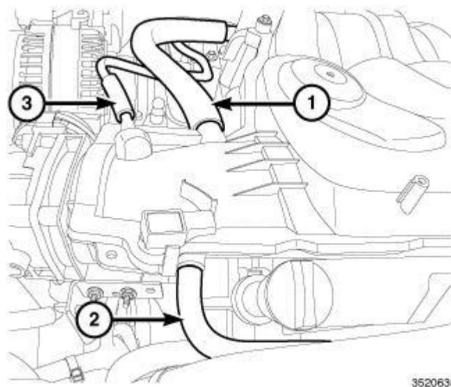
Fig. 589: Positive Crankcase Ventilation (PCV), Brake Booster & Vapor Purge Courtesy of CHRYSLER GROUP, LLC
