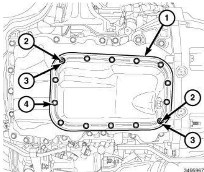
Fig. 516: Lower Oil Pan & Fasteners Courtesy of CHRYSLER GROUP, LLC
