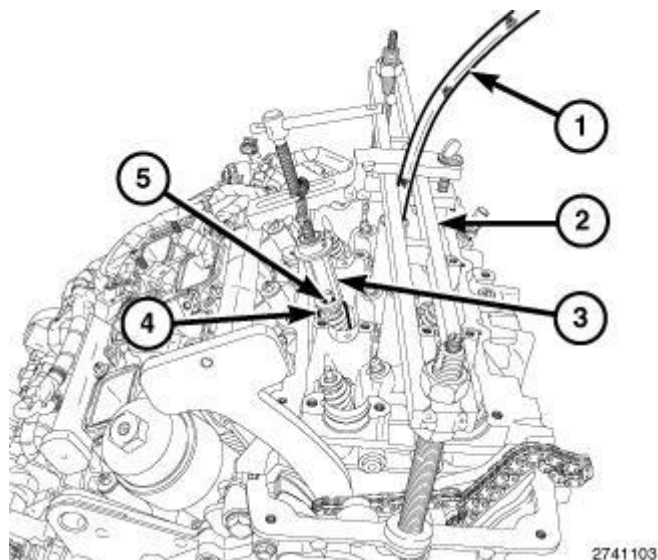
Fig. 291: Shop Air Supply & Valve Spring Compressor Courtesy of CHRYSLER GROUP, LLC
