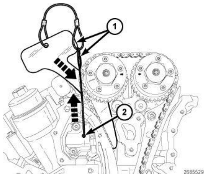
Fig. 172: Pin, Rack & Timing Chain Holder
