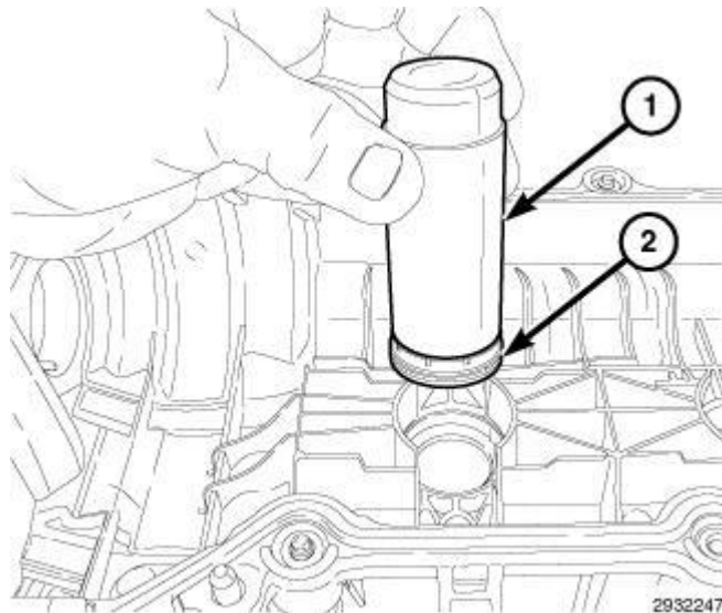
Fig. 240: Spark Plug Tube Seal & Installer Courtesy of CHRYSLER GROUP, LLC
