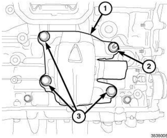
Fig. 359: Right Engine Mount Isolator & Fasteners Courtesy of CHRYSLER GROUP, LLC
