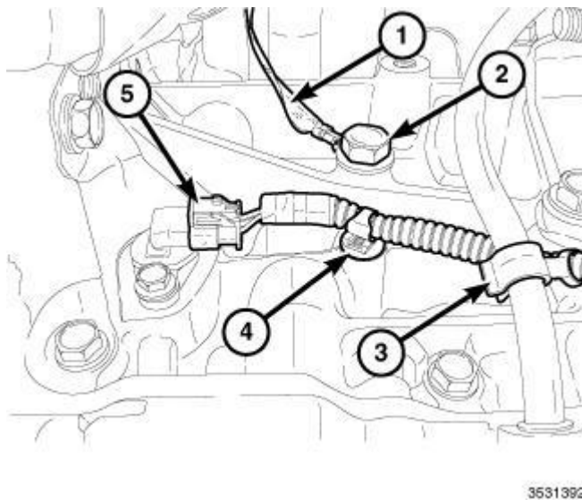
Fig. 9: Ground Strap, Bolt, Retainers & Crankshaft Position (CKP) Sensor Courtesy of CHRYSLER GROUP, LLC
