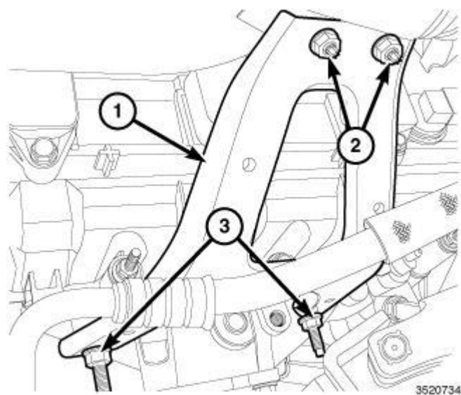
Fig. 563: Left Rear Upper Intake Manifold Support Bracket & Fasteners Courtesy of CHRYSLER GROUP, LLC
