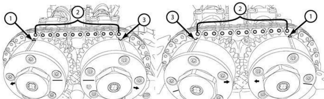
Fig. 616: Chain Pins, Exhaust Cam Phaser Triangle Marking & Circle Marking Courtesy of CHRYSLER GROUP, LLC
