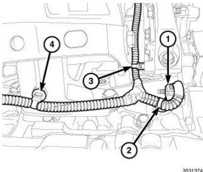
Fig. 437: Oil Pump Solenoid Electrical Connector & Wire Harness Retainers
