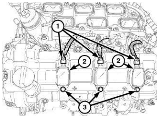
Fig. 243: Electrical Connector, Ignition Coils & Ignition Coil Retaining Bolts Courtesy of CHRYSLER GROUP, LLC
