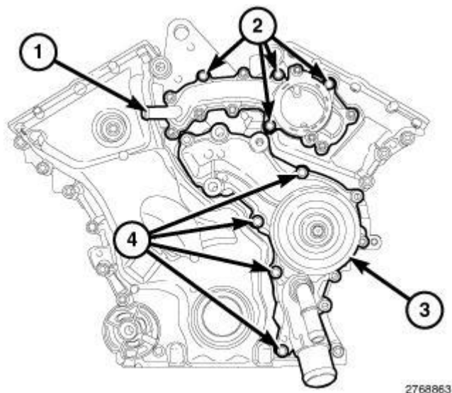
Fig. 656: Coolant Outlet Housing, Water Pump & Bolts Courtesy of CHRYSLER GROUP, LLC
