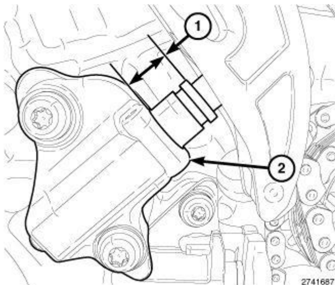
Fig. 626: Piston Extension & RH Cam Chain Tensioner Courtesy of CHRYSLER GROUP, LLC
