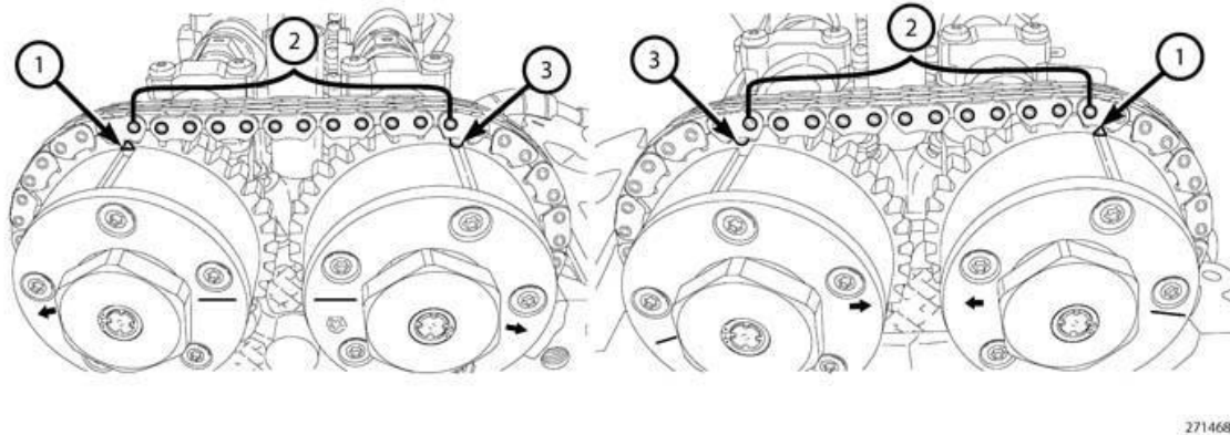
Fig. 644: Chain Pins, Exhaust Cam Phaser Triangle Marking & Circle Marking Courtesy of CHRYSLER GROUP, LLC
