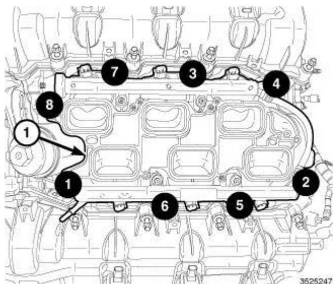
Fig. 595: Lower Intake Manifold Tightening Sequence
