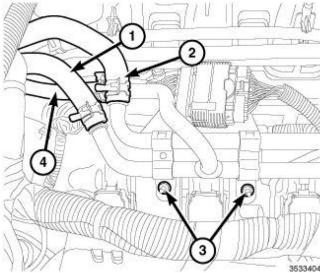
Fig. 286: Heater Core Return Hose, Heater Core Supply Hose, Nuts & Oil Cooler Return Hose Courtesy of CHRYSLER GROUP, LLC
