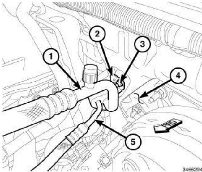
Fig. 288: A/C Suction & Liquid Line Assembly Courtesy of CHRYSLER GROUP, LLC
