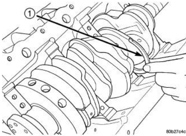
Fig. 382: Thrust Washer Installation Courtesy of CHRYSLER GROUP, LLC
