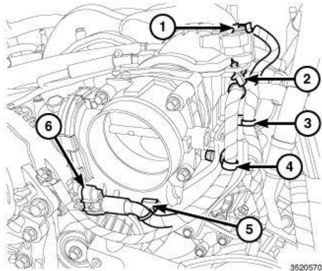
Fig. 559: Manifold Absolute Pressure (MAP) Sensor, Electronic Throttle Control (ETC), Clip & Retainers
