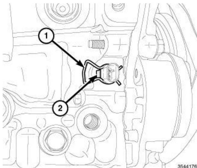
Fig. 527: Oil Pump Solenoid Electrical Connector Retaining Clip & Retention Lock Tab Courtesy of CHRYSLER GROUP, LLC
