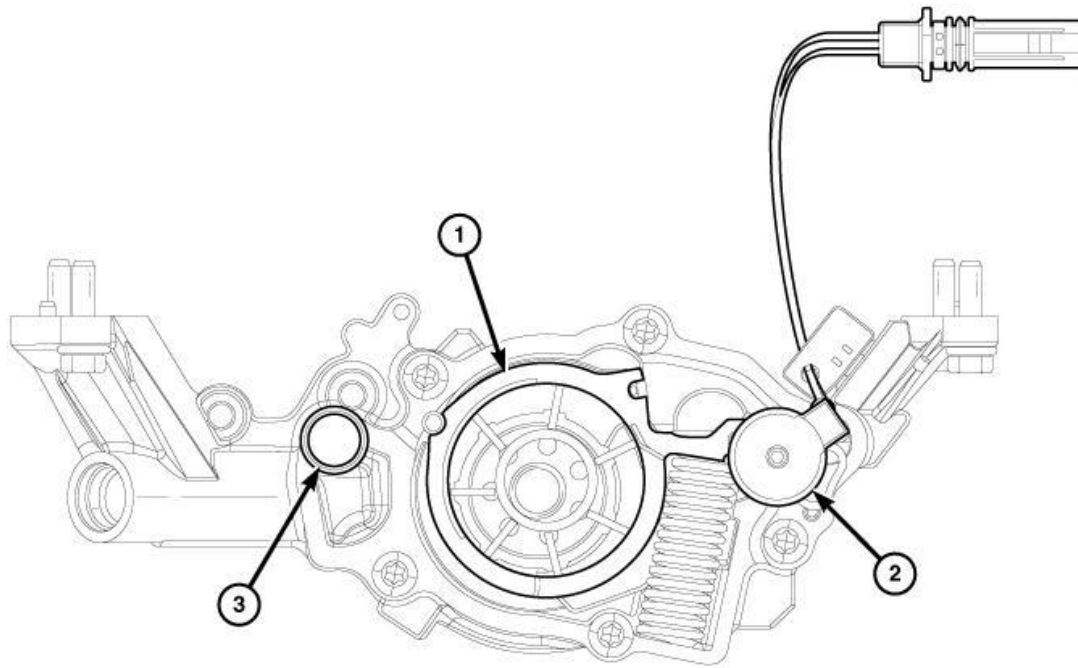
Fig. 523: Moving Element, On/Off Solenoid & Relief Valve Courtesy of CHRYSLER GROUP, LLC
