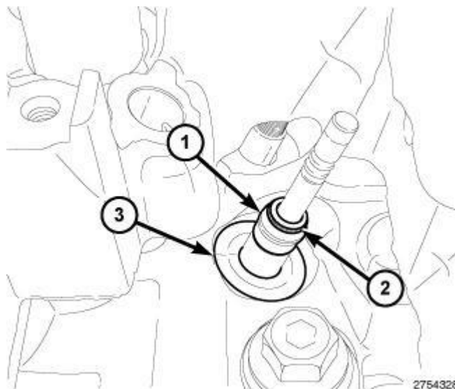
Fig. 331: Spring Seat, Valve Guide Seal & Garter Spring Courtesy of CHRYSLER GROUP, LLC
