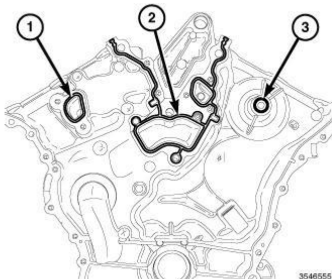
Fig. 655: Coolant Outlet Housing Gasket, Water Pump Gasket & O-Ring Courtesy of CHRYSLER GROUP, LLC
