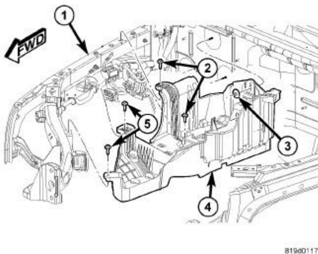
Fig. 285: Battery Tray Components
