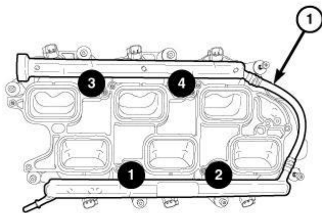
Fig. 580: Fuel Rail Bolt Tightening Sequence
