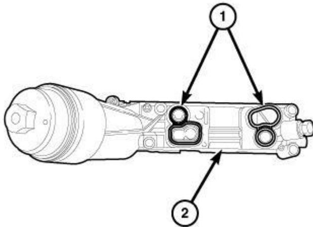
Fig. 474: Oil Cooler Seals & Oil Filter Housing
