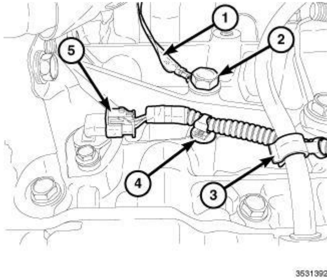
Fig. 230: Ground Strap, Bolt, Retainers & Crankshaft Position (CKP) Sensor Courtesy of CHRYSLER GROUP, LLC
