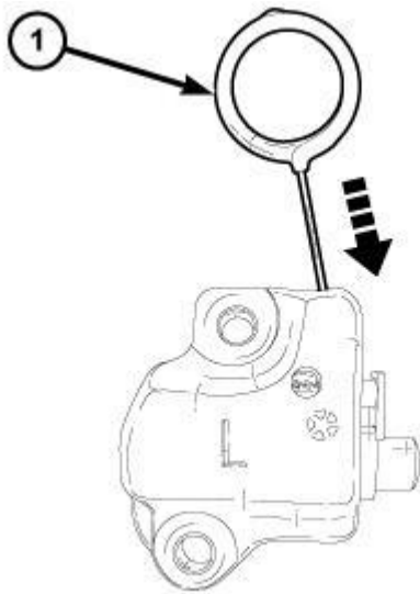
Fig. 605: Inserting Tensioner Pin To Hold Rack & Piston In Retracted Position Courtesy of CHRYSLER GROUP, LLC
