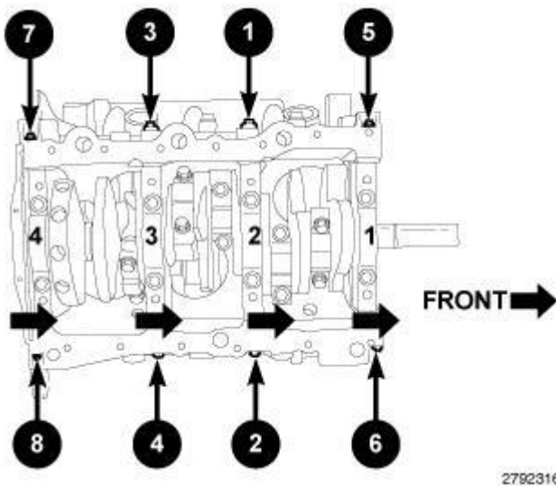
Fig. 388: Main Bearing Tie Bolts Installation Sequence
