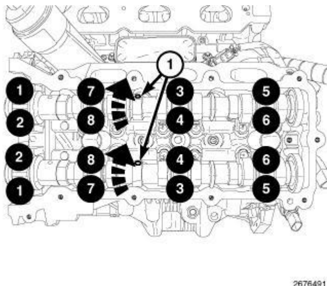
Fig. 200: Camshaft Bearing Cap Bolts Removal Sequence - Left
