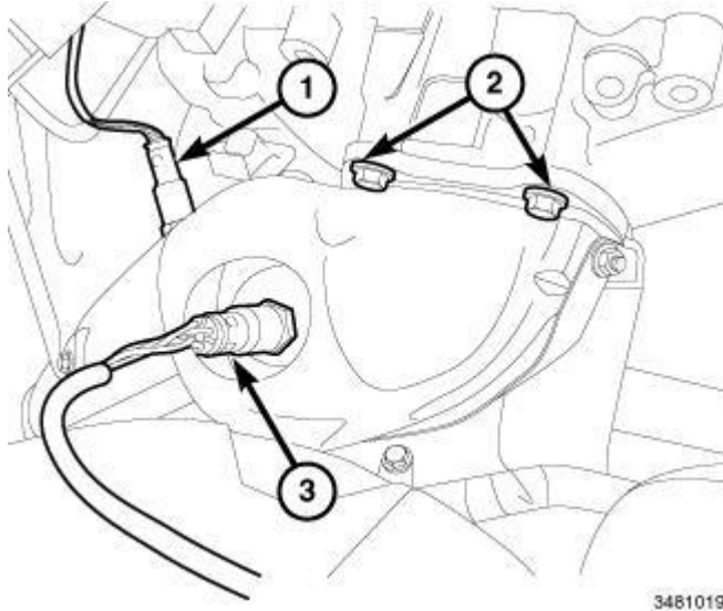
Fig. 158: Right And Left Upstream And Downstream Oxygen Sensor Connectors & Bolts Courtesy of CHRYSLER GROUP, LLC
