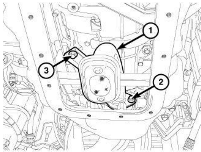
Fig. 521: Oil Pick-Up Tube & Bolts Courtesy of CHRYSLER GROUP, LLC
