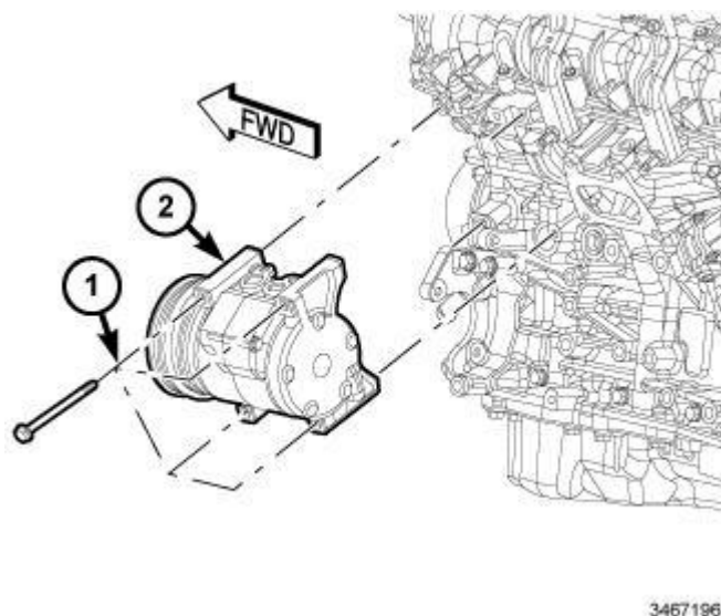
Fig. 51: A/C Compressor & Mounting Bolts
