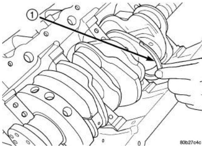
Fig. 363: Thrust Washer Installation Courtesy of CHRYSLER GROUP, LLC
