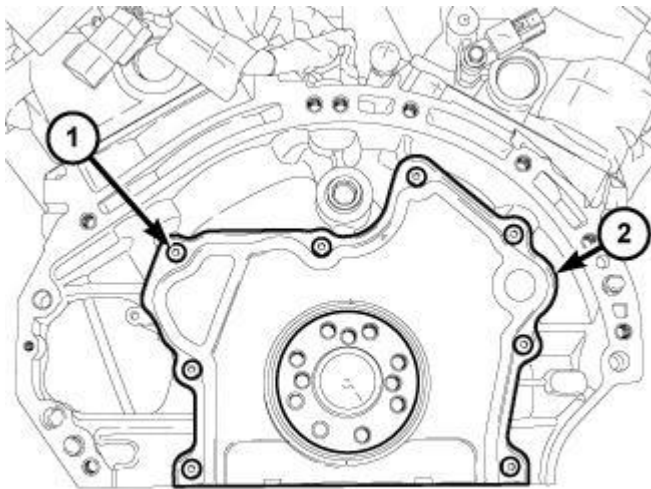
Fig. 432: Seal Retainer & Attaching Screws
