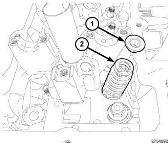
Fig. 336: Valve Spring & Valve Spring Retainer Courtesy of CHRYSLER GROUP, LLC
