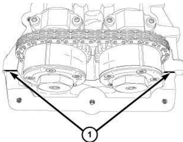
Fig. 221: RTV Sealant Locations Courtesy of CHRYSLER GROUP, LLC
