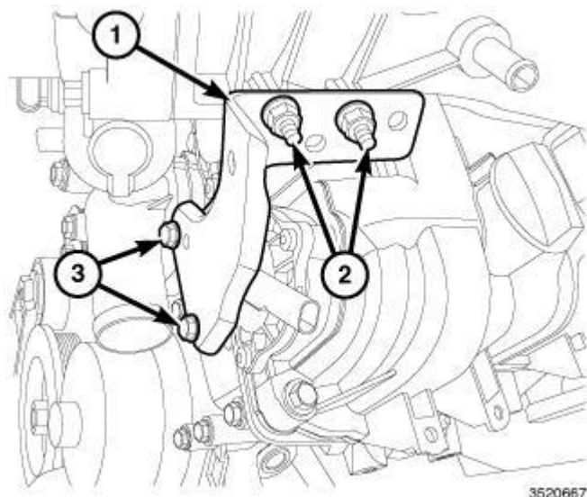
Fig. 588: Left Front Upper Intake Manifold Support Bracket & Fasteners Courtesy of CHRYSLER GROUP, LLC
