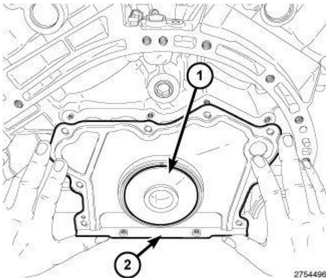
Fig. 430: Oil Seal Retainer Assembly & Seal Protector
