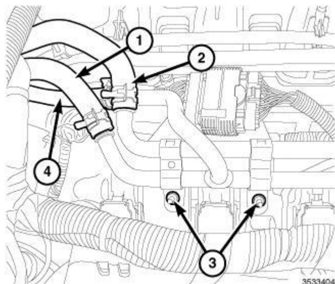
Fig. 661: Heater Core Return Hose, Heater Core Supply Hose, Nuts & Oil Cooler Return Hose
