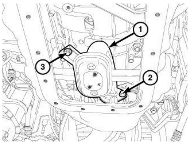
Fig. 518: Oil Pick-Up Tube & Bolts
