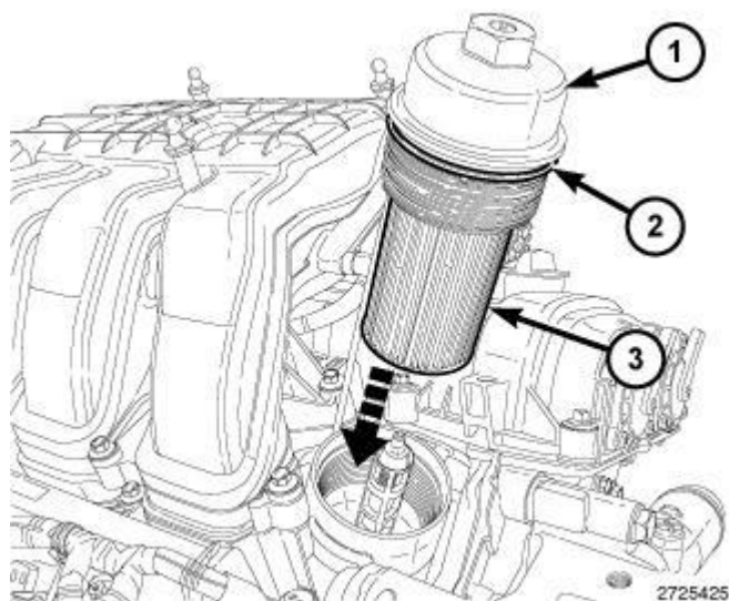
Fig. 490: Oil Filter Cap, O-Ring Seal & Oil Filter Courtesy of CHRYSLER GROUP, LLC
