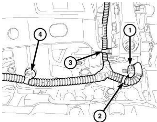
Fig. 526: Oil Pump Solenoid Electrical Connector & Wire Harness Retainers Courtesy of CHRYSLER GROUP, LLC
