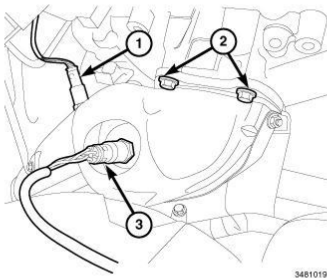
Fig. 11: Right And Left Upstream And Downstream Oxygen Sensor Connectors & Bolts Courtesy of CHRYSLER GROUP, LLC
