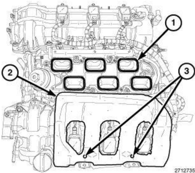
Fig. 224: Intake Ports, Insulator & Alignment Posts Courtesy of CHRYSLER GROUP, LLC
