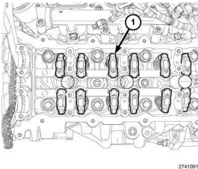
Fig. 273: Locating Rocker Arms
