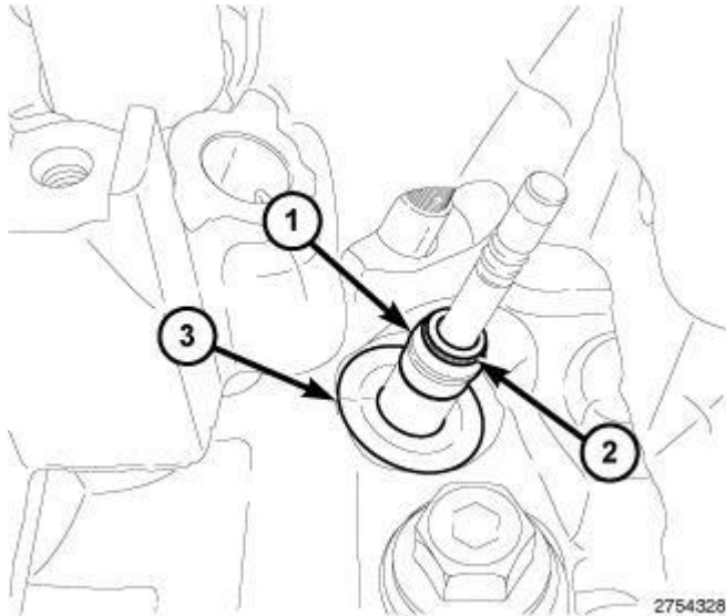
Fig. 325: Spring Seat, Valve Guide Seal & Garter Spring Courtesy of CHRYSLER GROUP, LLC
