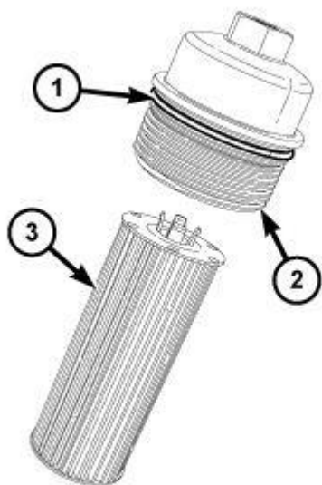
Fig. 466: O-Ring Seal, Oil Filter Cap & Oil Filter Courtesy of CHRYSLER GROUP, LLC
