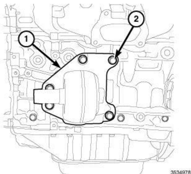
Fig. 368: Left Engine Mount Isolator & Fasteners Courtesy of CHRYSLER GROUP, LLC
