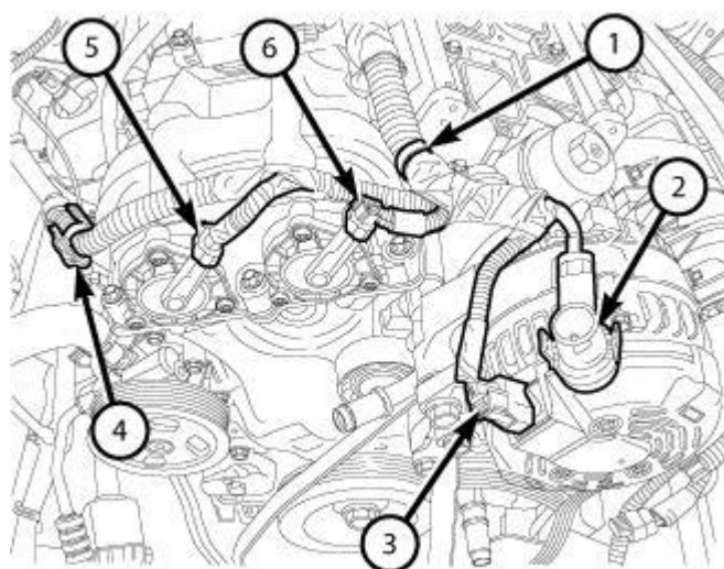
Fig. 56: Generator Stud, Connector, Retainers & Right Exhaust And Right Intake Variable Valve Timing Solenoid Electrical Connectors Courtesy of CHRYSLER GROUP, LLC
