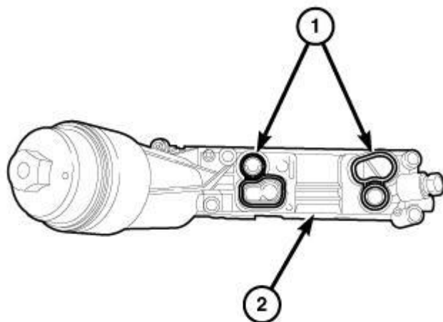
Fig. 477: Oil Cooler Seals & Oil Filter Housing Courtesy of CHRYSLER GROUP, LLC
