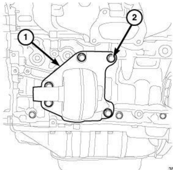
Fig. 435: Left Engine Mount Isolator & Fasteners Courtesy of CHRYSLER GROUP, LLC
