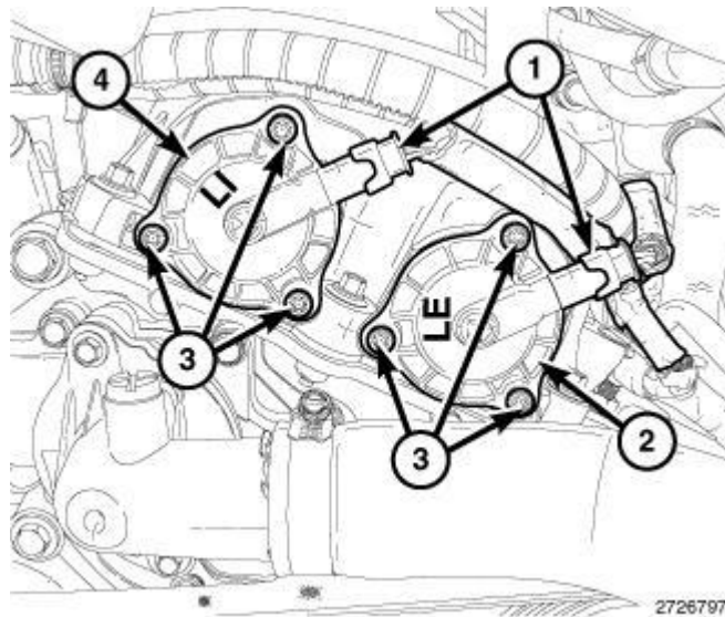
Fig. 245: Variable Valve Timing Solenoids, Connectors & Bolts Courtesy of CHRYSLER GROUP, LLC
