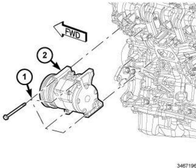
Fig. 26: A/C Compressor & Mounting Bolts
