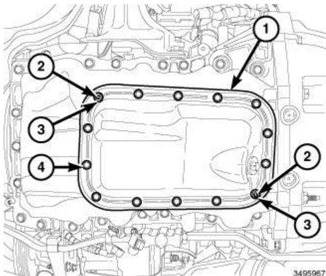
Fig. 495: Lower Oil Pan & Fasteners Courtesy of CHRYSLER GROUP, LLC
