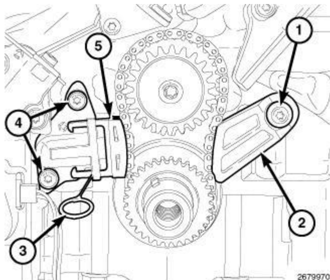
Fig. 622: Primary Chain Tensioner, Tensioner Pin, Primary Chain Guide & Bolts Courtesy of CHRYSLER GROUP, LLC
