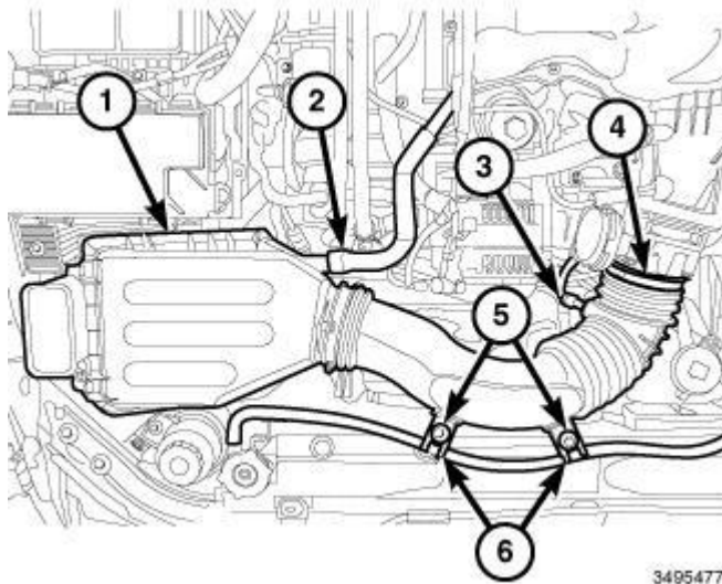
Fig. 284: Air Cleaner Body, Fresh Air Makeup Hose, Electrical Connector, Clamp, Bolts & Retainers
