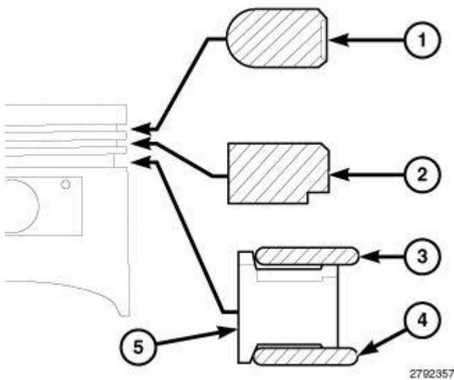
Fig. 398: Piston Ring Removal/Installation Sequence
