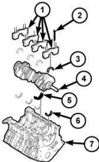
Fig. 381: Main Bearing Caps, Bolts, Crankshaft & Engine Block
