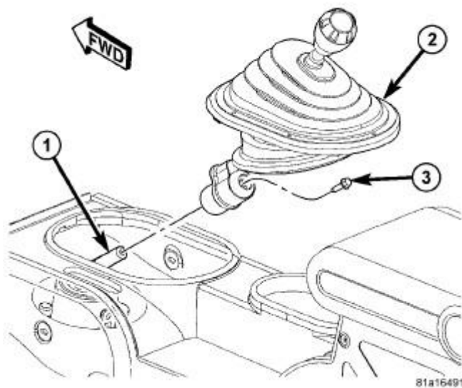
Fig. 7: Shifter Shaft, Boots & Bolt Courtesy of CHRYSLER GROUP, LLC
