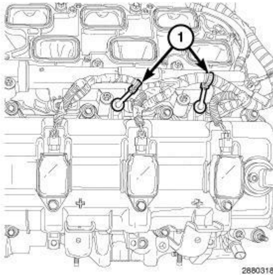
Fig. 244: Injection/Ignition Harness Retainers Courtesy of CHRYSLER GROUP, LLC
