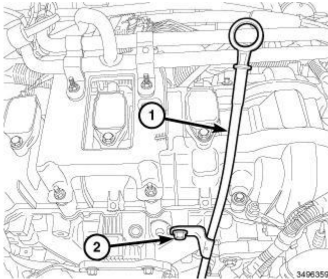
Fig. 18: Oil Level Indicator & Bolt Courtesy of CHRYSLER GROUP, LLC
