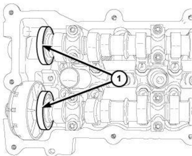
Fig. 251: Magnetic Timing Wheels
