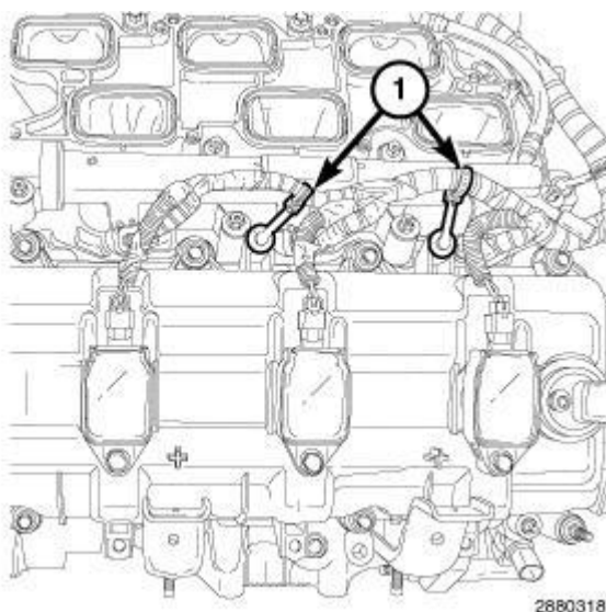
Fig. 217: Injection/Ignition Harness Retainers Courtesy of CHRYSLER GROUP, LLC
