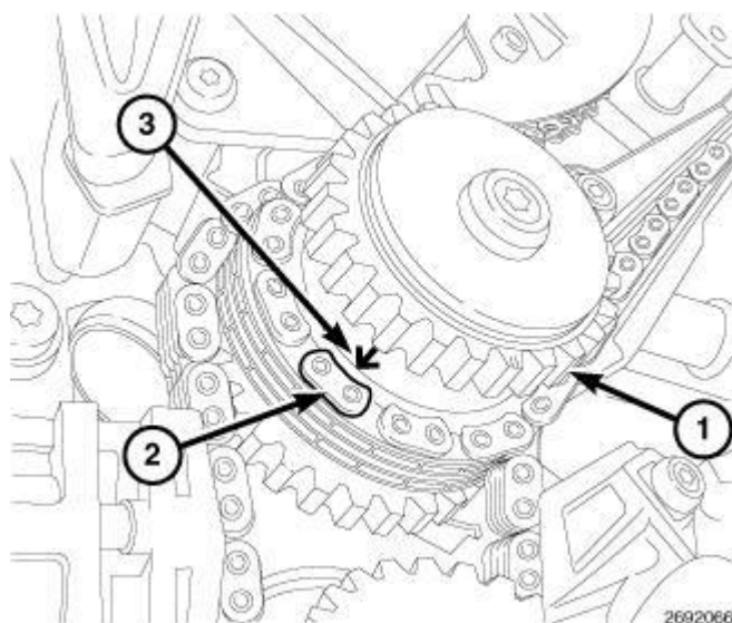
Fig. 132: Idler Sprocket, Plated Link & Arrow Courtesy of CHRYSLER GROUP, LLC
