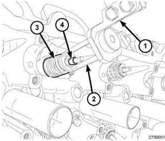
Fig. 327: Compressing Valve Spring & Locating Valve Retaining Locks Courtesy of CHRYSLER GROUP, LLC
