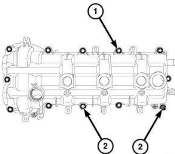
Fig. 219: Cylinder Head Cover Mounting Bolts & Studbolts Courtesy of CHRYSLER GROUP, LLC
