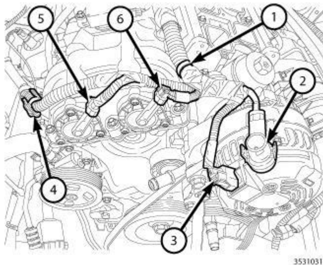
Fig. 225: Generator Stud, Connector, Retainers & Right Exhaust And Right Intake Variable Valve Timing Solenoid Electrical Connectors Courtesy of CHRYSLER GROUP, LLC
