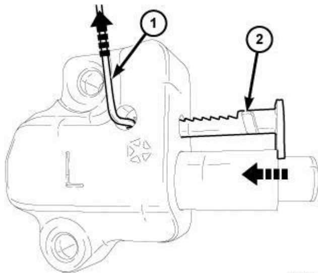
Fig. 604: Locating Slot In Rack & Allen Wrench Courtesy of CHRYSLER GROUP, LLC
