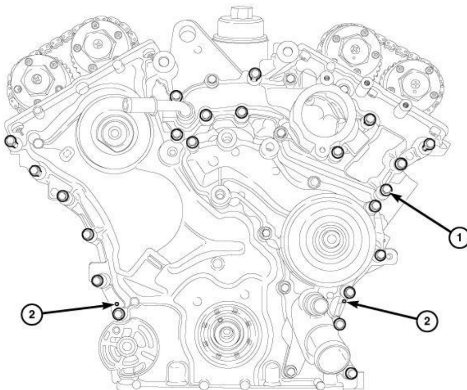
Fig. 659: Engine Timing Cover Bolts & Pins Courtesy of CHRYSLER GROUP, LLC
