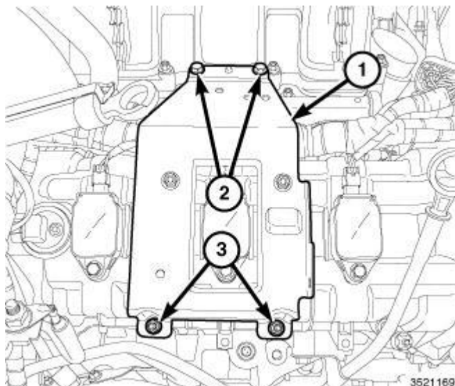
Fig. 565: Right Upper Intake Manifold Support Bracket & Fasteners Courtesy of CHRYSLER GROUP, LLC
