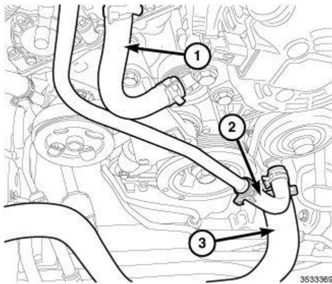
Fig. 648: Heater Core Supply Hose, Heater Core Return Hose & Lower Radiator Hose Courtesy of CHRYSLER GROUP, LLC
