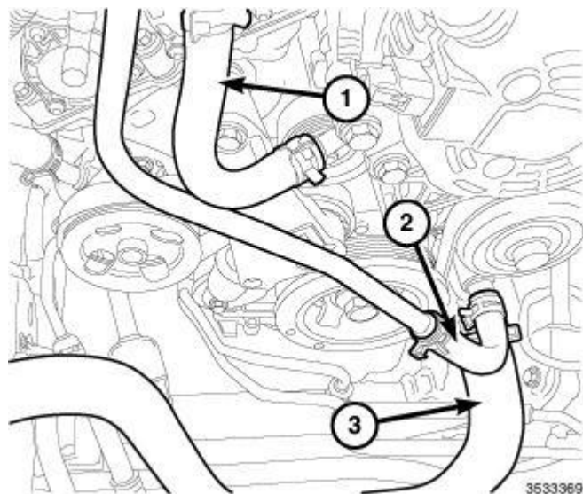
Fig. 662: Heater Core Supply Hose, Heater Core Return Hose & Lower Radiator Hose Courtesy of CHRYSLER GROUP, LLC
