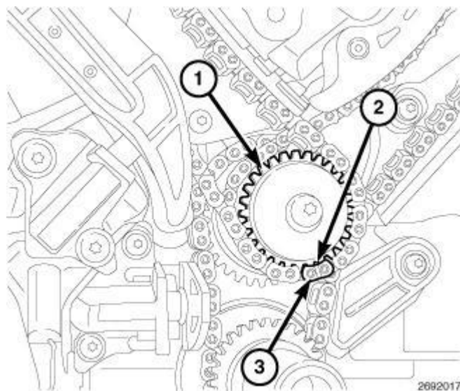
Fig. 640: Idler Sprocket, Dimple & Plated Link Courtesy of CHRYSLER GROUP, LLC
