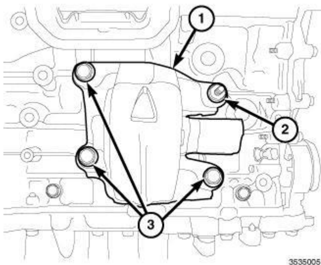
Fig. 440: Right Engine Mount Isolator & Fasteners Courtesy of CHRYSLER GROUP, LLC
