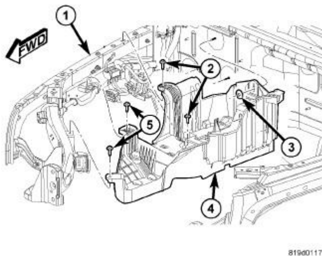
Fig. 160: Battery Tray Components Courtesy of CHRYSLER GROUP, LLC
