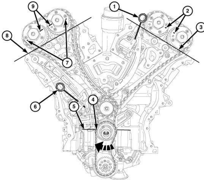
Fig. 643: Rotating Crankshaft Clockwise To Position No. 1 Piston At TDC On Exhaust Stroke Courtesy of CHRYSLER GROUP, LLC
