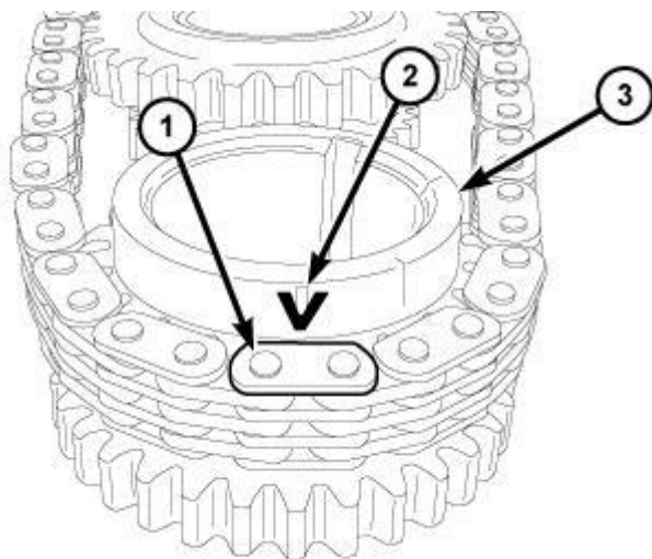
Fig. 632: Aligning Arrow With Plated Link On Primary Chain
