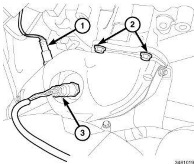
Fig. 92: Right And Left Upstream And Downstream Oxygen Sensor Connectors & Bolts
