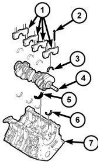
Fig. 365: Main Bearing Caps, Bolts, Crankshaft & Engine Block
