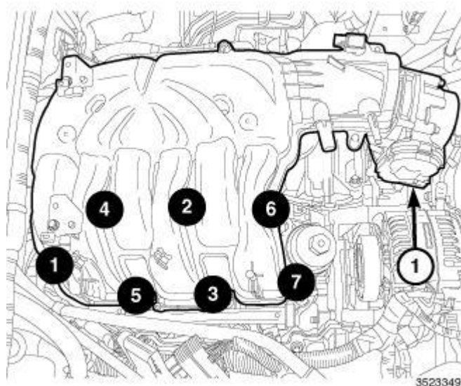
Fig. 250: Upper Intake Manifold Tightening Sequence
