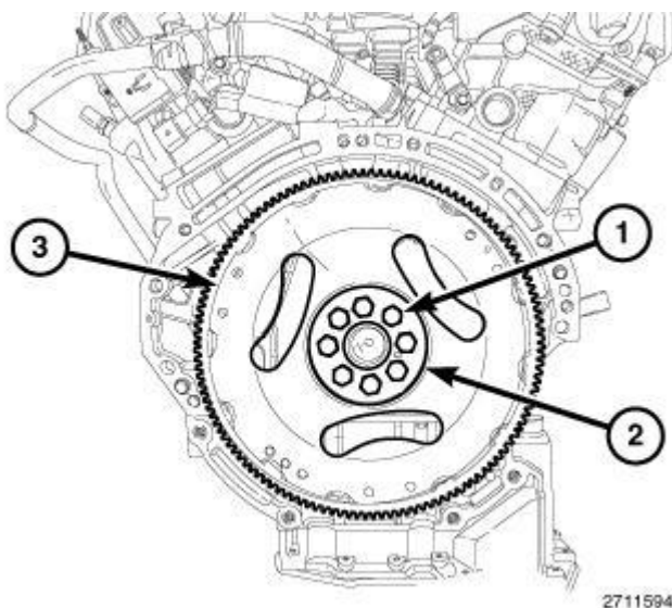
Fig. 394: Flexplate, Spacer Plate & Bolts Courtesy of CHRYSLER GROUP, LLC
