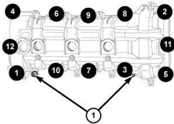
Fig. 255: Cylinder Head Cover Bolts & Double Ended Studs Tightening Sequence - Right Courtesy of CHRYSLER GROUP, LLC
