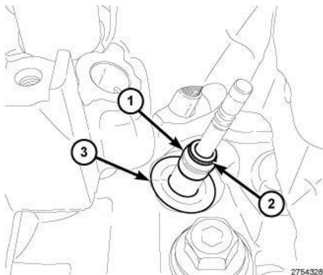
Fig. 335: Spring Seat, Valve Guide Seal & Garter Spring Courtesy of CHRYSLER GROUP, LLC
