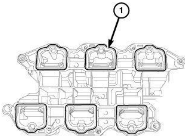
Fig. 593: Lower Intake Manifold To Cylinder Head Seals
