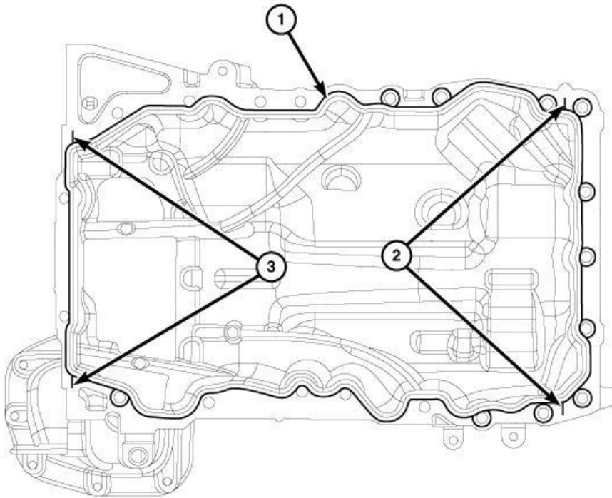
Fig. 505: Mopar® Threebond Engine RTV Sealant Locations Courtesy of CHRYSLER GROUP, LLC
