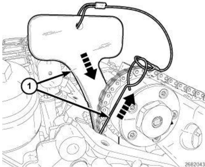
Fig. 607: Positioning Timing Chain Holder To Force Rack & Piston Back Into Tensioner Body Courtesy of CHRYSLER GROUP, LLC
