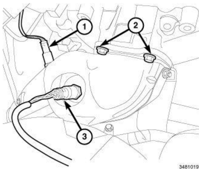
Fig. 139: Right And Left Upstream And Downstream Oxygen Sensor Connectors & Bolts Courtesy of CHRYSLER GROUP, LLC
