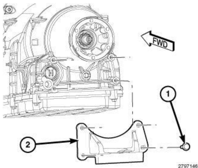
Fig. 447: Rear Engine Mount Bracket & Bolts (4x2) Courtesy of CHRYSLER GROUP, LLC
