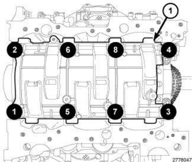
Fig. 373: Main Bearing Cap Bolts From Windage Tray Removal Sequence Courtesy of CHRYSLER GROUP, LLC
