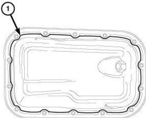
Fig. 506: Oil Pan RTV Sealant Courtesy of CHRYSLER GROUP, LLC
