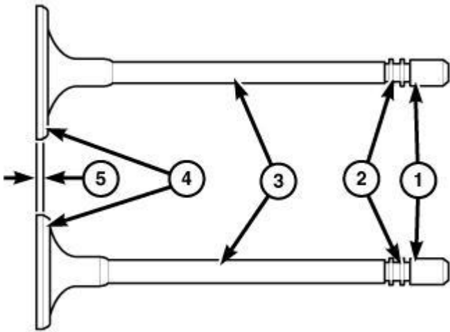
Fig. 322: Inspecting Valve Margin
