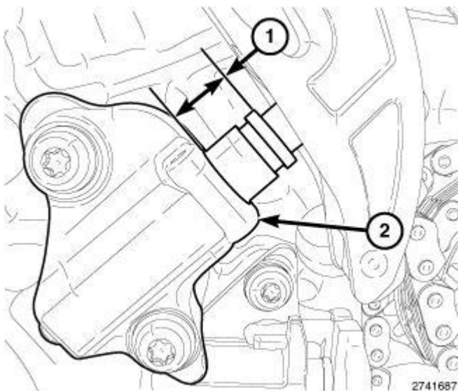
Fig. 608: Piston Extension & RH Cam Chain Tensioner Courtesy of CHRYSLER GROUP, LLC
