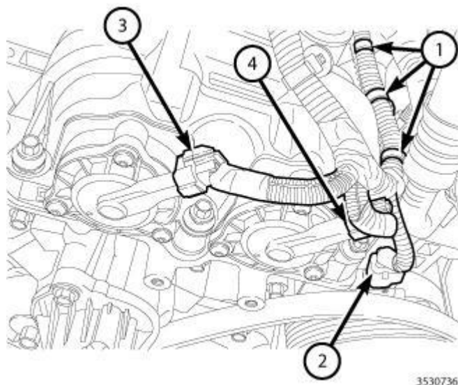
Fig. 246: Retainers, A/C Compressor Electrical Connector & Left Intake And Left Exhaust Variable Valve Timing Solenoid Electrical Connectors Courtesy of CHRYSLER GROUP, LLC
