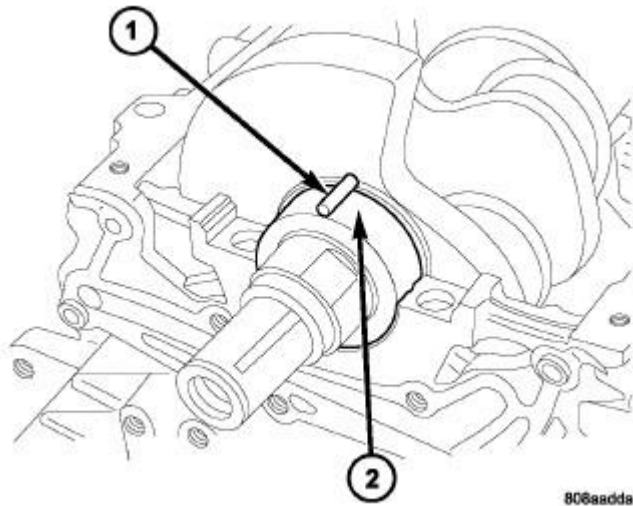
Fig. 338: Plastigage Placed In Lower Shell Courtesy of CHRYSLER GROUP, LLC
