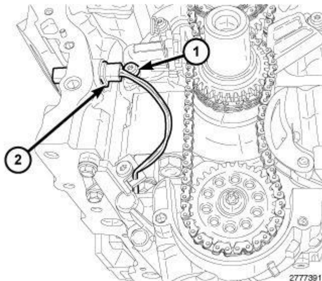
Fig. 537: Oil Pump Solenoid Electrical Connector & Primary Chain Tensioner Mounting Bolt Courtesy of CHRYSLER GROUP, LLC
