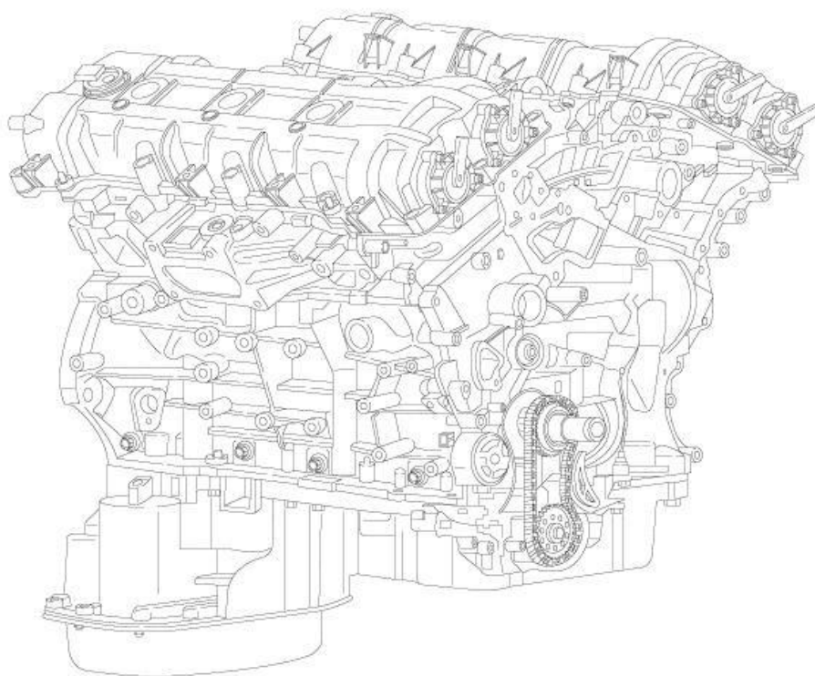
Fig. 453: 3.6L Engine
