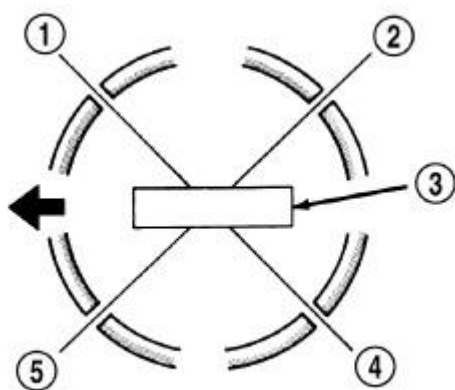
Fig. 405: Piston Ring End Gap Position Courtesy of CHRYSLER GROUP, LLC
