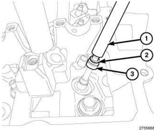
Fig. 279: Installing Valve Guide Seal Courtesy of CHRYSLER GROUP, LLC
