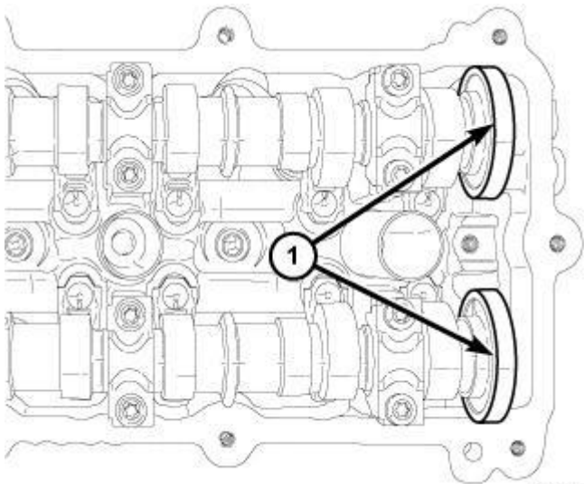
Fig. 204: Magnetic Timing Wheels
