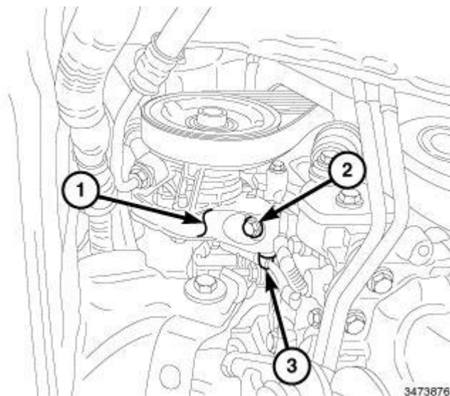
Fig. 61: Power Steering Pump Bracket, Bolt & Retainer Courtesy of CHRYSLER GROUP, LLC
