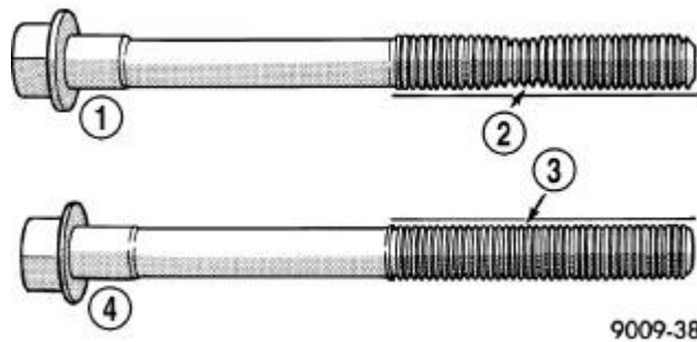
Fig. 364: Checking Cylinder Head Bolts For Stretching (Necking)
