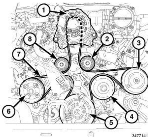
Fig. 138: Drive Belt Tensioners & Assembly With Drive Belt Routing Courtesy of CHRYSLER GROUP, LLC
