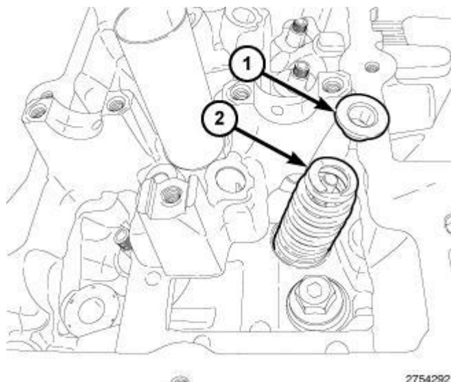
Fig. 292: Valve Spring & Valve Spring Retainer Courtesy of CHRYSLER GROUP, LLC
