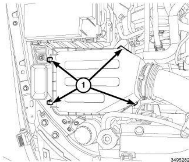
Fig. 80: Air Cleaner Housing Cover Latches Courtesy of CHRYSLER GROUP, LLC
