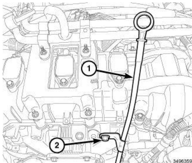
Fig. 517: Oil Level Indicator & Bolt Courtesy of CHRYSLER GROUP, LLC
