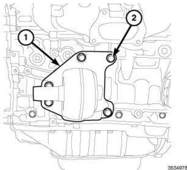
Fig. 358: Left Engine Mount Isolator & Fasteners Courtesy of CHRYSLER GROUP, LLC
