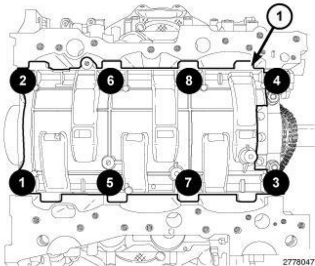
Fig. 412: Main Bearing Cap Bolts From Windage Tray Removal Sequence
