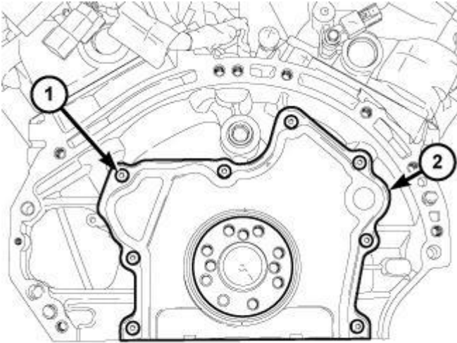
Fig. 428: Seal Retainer & Attaching Screws
