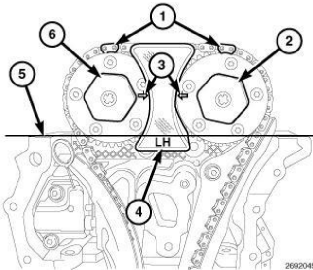
Fig. 638: Phaser Timing Marks, Oil Control Valves & LH Camshaft Phaser Lock Courtesy of CHRYSLER GROUP, LLC
