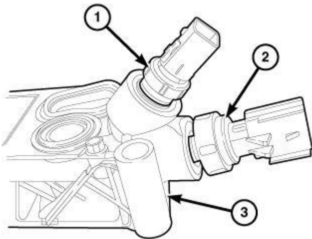
Fig. 455: Oil Temperature Sensor, Oil Pressure Sensor & Oil Filter Housing Courtesy of CHRYSLER GROUP, LLC
