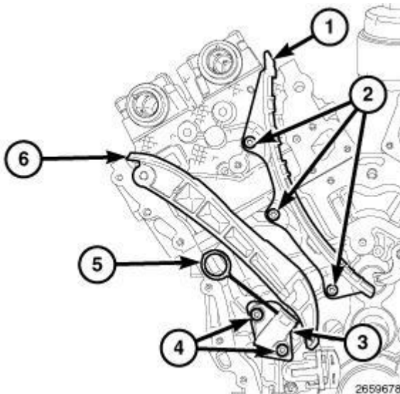
Fig. 625: Right Cam Chain Tensioner, Arm, Guide & Bolts Courtesy of CHRYSLER GROUP, LLC
