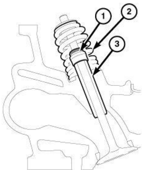
Fig. 274: Valve Stem Oil Seal, Valve Spring & Valve Guide Courtesy of CHRYSLER GROUP, LLC
