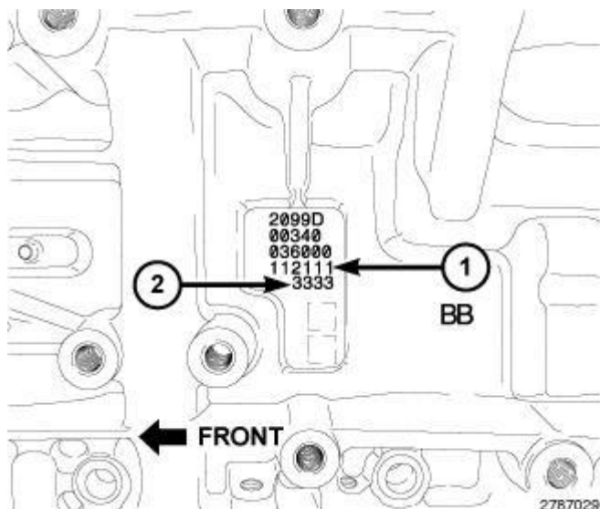
Fig. 353: Engine Block Cylinder Bore Diameter Grade Markings & Engine Block Main Bearing Journal Diameter Grade Markings
