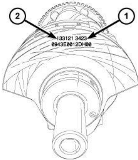
Fig. 352: Crankshaft Main Bearing Journal Diameter Grade Markings & Connecting Rod Bearing Journal Diameter Grade Markings Courtesy of CHRYSLER GROUP, LLC
