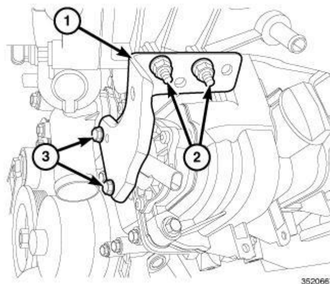
Fig. 561: Left Front Upper Intake Manifold Support Bracket & Fasteners Courtesy of CHRYSLER GROUP, LLC
