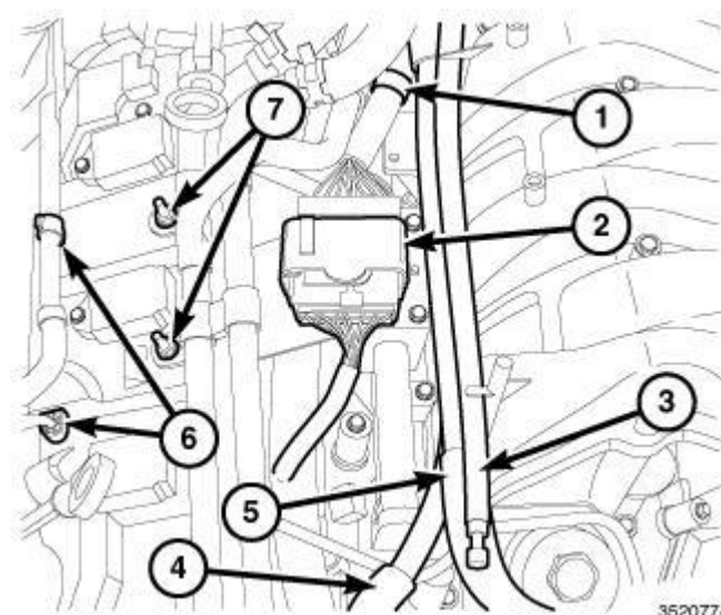
Fig. 564: Transfer Case Vent Hose, Fresh Air Makeup Hose, Positive Crankcase Ventilation (PCV) Hose, Retainers & Fasteners
