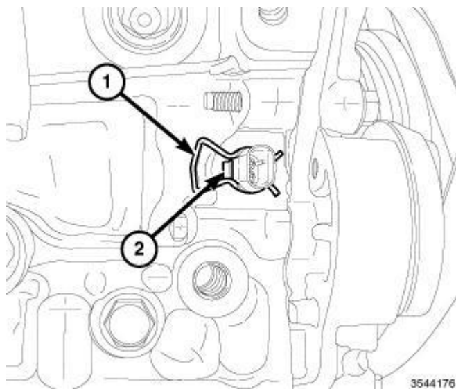
Fig. 538: Oil Pump Solenoid Electrical Connector Retaining Clip & Retention Lock Tab Courtesy of CHRYSLER GROUP, LLC
