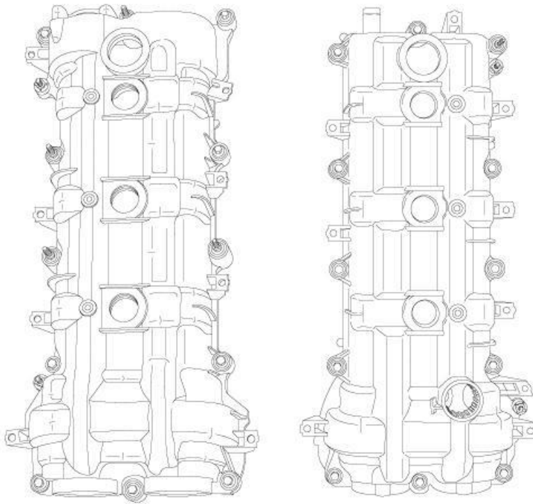
Fig. 209: Cylinder Head Covers
