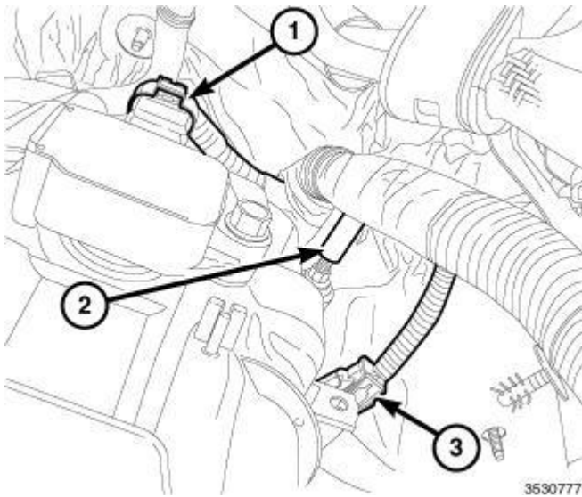
Fig. 248: Camshaft Position (CMP) Sensor, Retainer & Engine Coolant Temperature (ECT) Sensor Connector Courtesy of CHRYSLER GROUP, LLC
