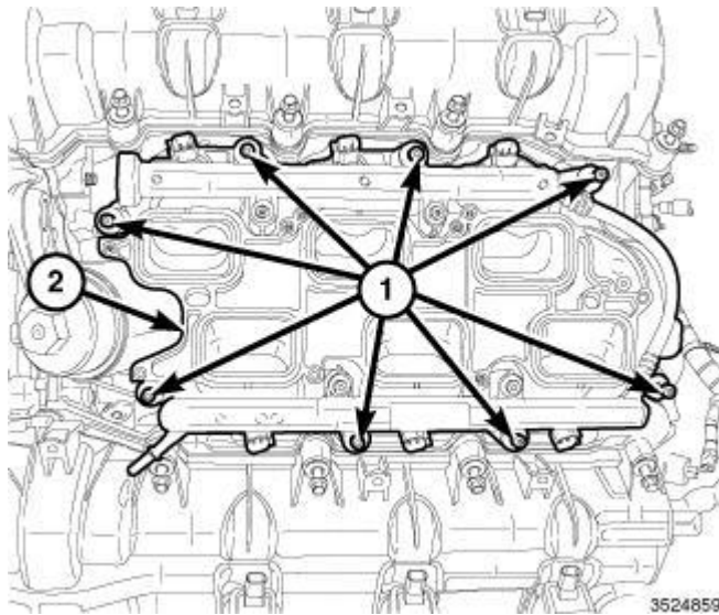
Fig. 574: Lower Intake Manifold & Bolts Courtesy of CHRYSLER GROUP, LLC
