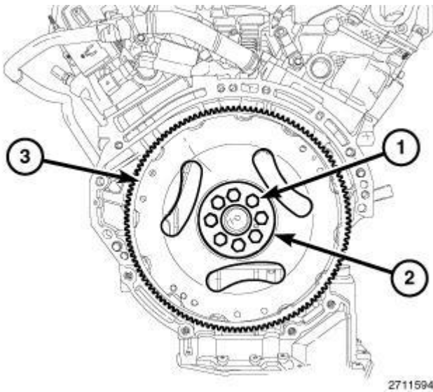
Fig. 395: Flexplate, Spacer Plate & Bolts Courtesy of CHRYSLER GROUP, LLC
