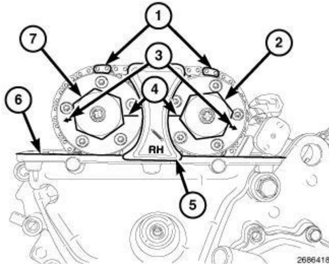
Fig. 290: Phaser Timing Marks, Oil Control Valves & RH Camshaft Phaser Lock Courtesy of CHRYSLER GROUP, LLC
