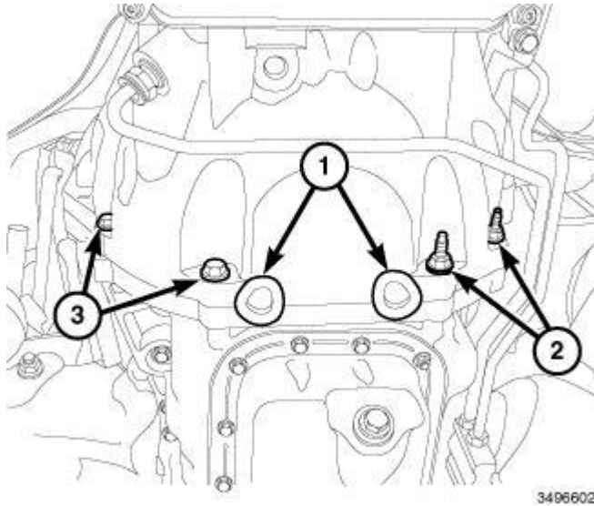
Fig. 514: Rubber Plugs & Transmission To Engine Oil Pan Bolts Courtesy of CHRYSLER GROUP, LLC
