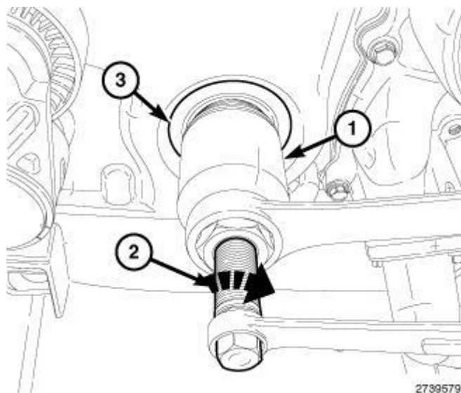
Fig. 426: Extractor Screw, Seal Remover & Front Crankshaft Oil Seal Courtesy of CHRYSLER GROUP, LLC
