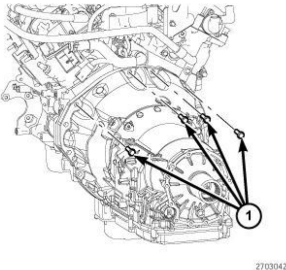
Fig. 32: Upper Transmission Engine Bolts Courtesy of CHRYSLER GROUP, LLC
