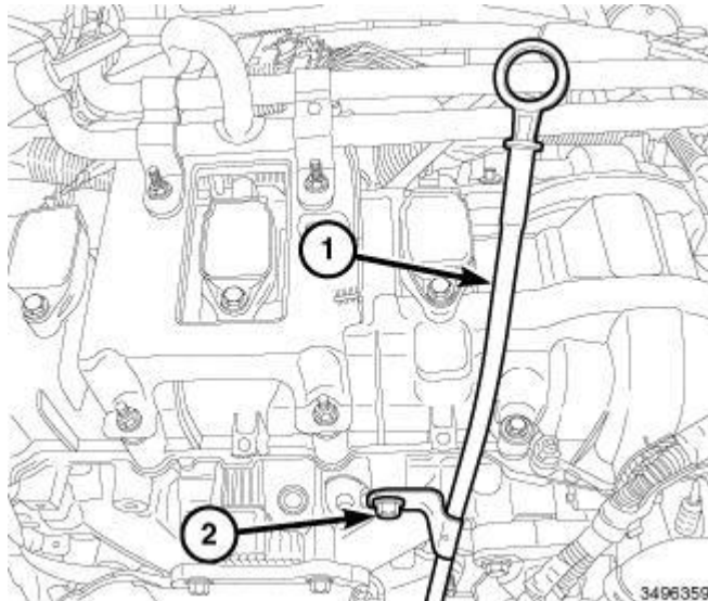
Fig. 233: Oil Level Indicator & Bolt Courtesy of CHRYSLER GROUP, LLC
