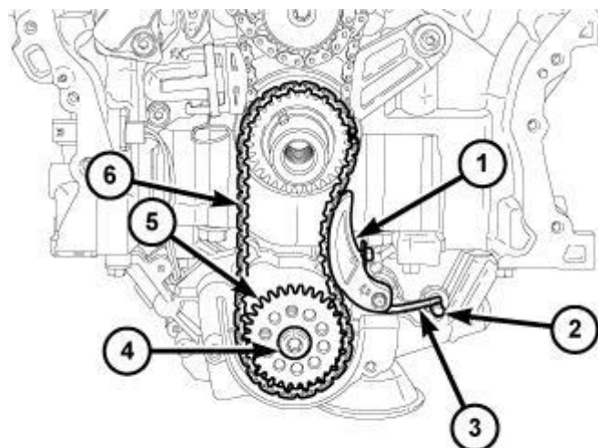
Fig. 619: Oil Pump Chain Tensioner, Spring, Retaining Bolt, Dowel Pin, Oil Pump Sprocket & Oil Pump Chain
