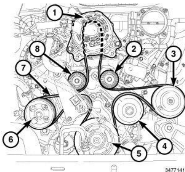
Fig. 650: Drive Belt Tensioners & Assembly With Drive Belt Routing Courtesy of CHRYSLER GROUP, LLC
