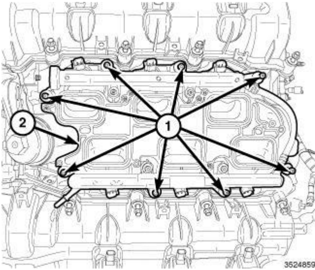
Fig. 549: Lower Intake Manifold & Bolts Courtesy of CHRYSLER GROUP, LLC
