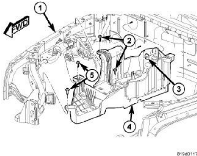
Fig. 109: Battery Tray Components
