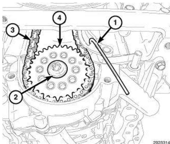
Fig. 530: Retaining Pin, Retaining Bolt, Oil Pump Chain & Sprocket Courtesy of CHRYSLER GROUP, LLC
