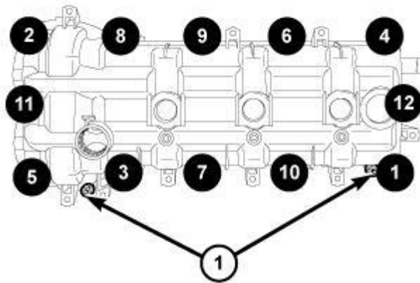
Fig. 242: Cylinder Head Cover Bolts & Double Ended Studs Tightening Sequence - Left Courtesy of CHRYSLER GROUP, LLC
