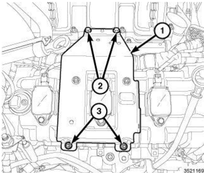
Fig. 584: Right Upper Intake Manifold Support Bracket & Fasteners Courtesy of CHRYSLER GROUP, LLC
