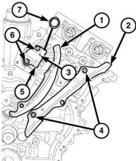
Fig. 629: Left Cam Chain Tensioner, Arm, Guide & Bolts Courtesy of CHRYSLER GROUP, LLC
