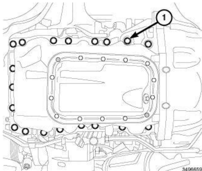
Fig. 512: Oil Pan Mounting Bolts Courtesy of CHRYSLER GROUP, LLC
