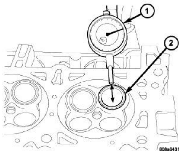
Fig. 333: Measuring Valve Guide Wear
