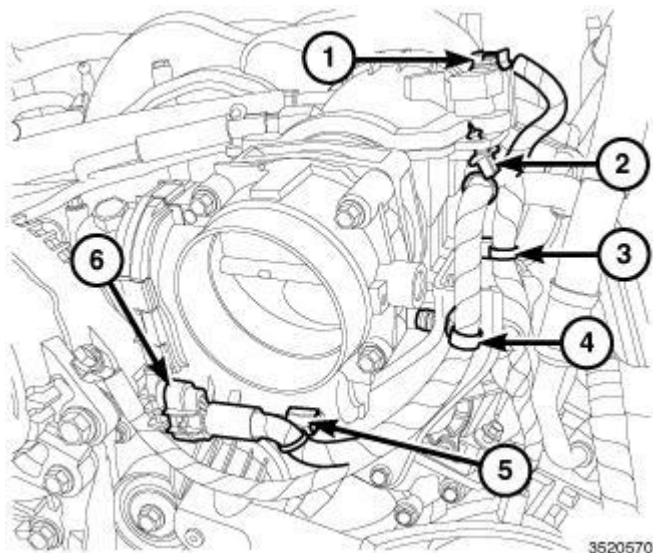
Fig. 590: Manifold Absolute Pressure (MAP) Sensor, Electronic Throttle Control (ETC), Clip & Retainers
