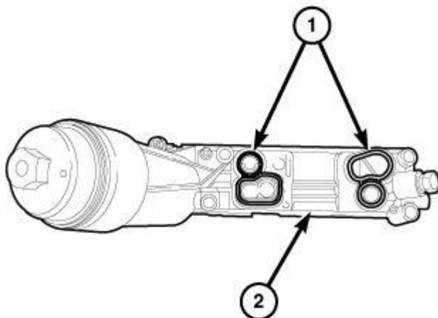
Fig. 462: Oil Cooler Seals & Oil Filter Housing
