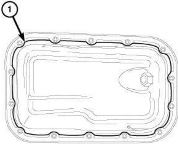
Fig. 507: Oil Pan RTV Sealant Courtesy of CHRYSLER GROUP, LLC
