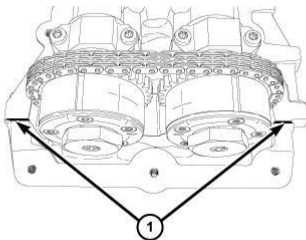
Fig. 237: RTV Sealant Locations
