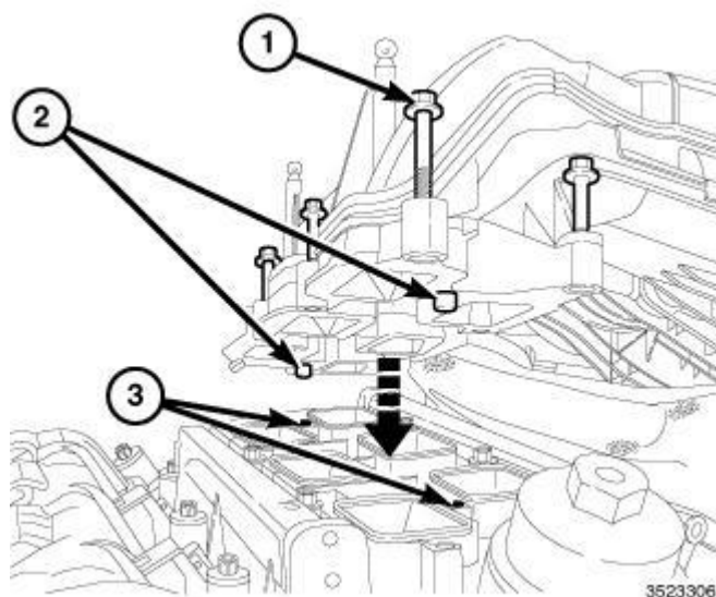
Fig. 582: Upper Intake Manifold & Bolts Courtesy of CHRYSLER GROUP, LLC
