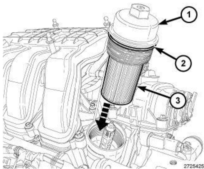
Fig. 468: Oil Filter Cap, O-Ring Seal & Oil Filter Courtesy of CHRYSLER GROUP, LLC
