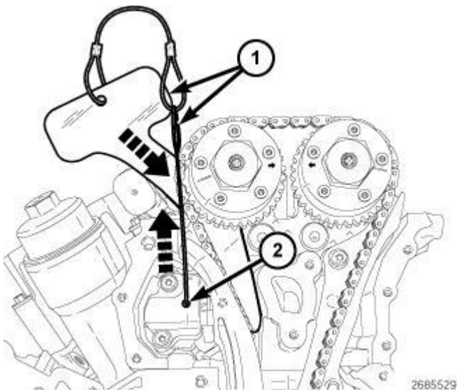
Fig. 606: Pin, Rack & Timing Chain Holder Courtesy of CHRYSLER GROUP, LLC
