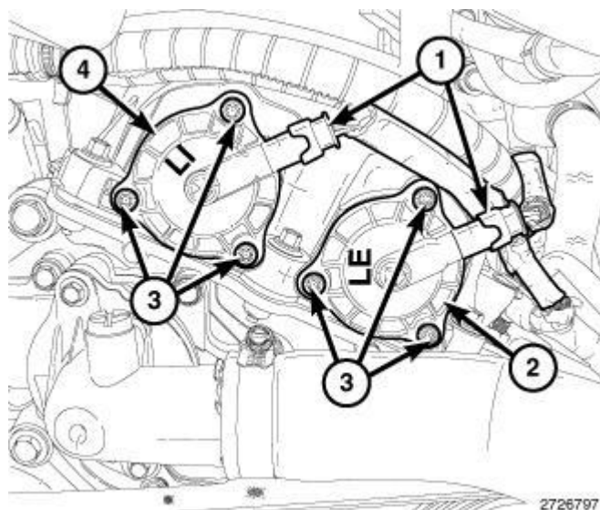
Fig. 215: Variable Valve Timing Solenoids, Connectors & Bolts
