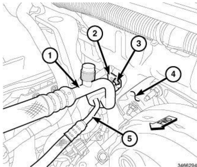
Fig. 302: A/C Suction & Liquid Line Assembly Courtesy of CHRYSLER GROUP, LLC
