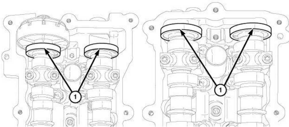
Fig. 282: Magnetic Timing Wheels Courtesy of CHRYSLER GROUP, LLC
