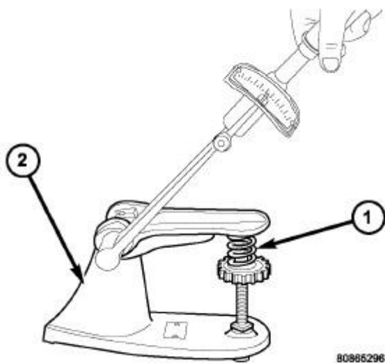
Fig. 296: Testing Valve Spring Courtesy of CHRYSLER GROUP, LLC
