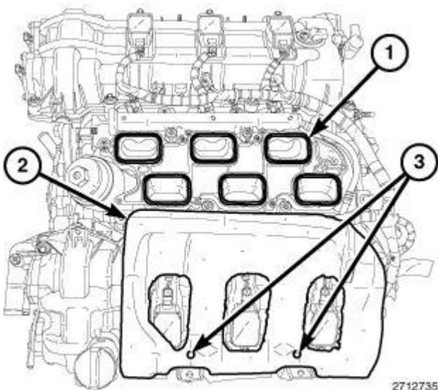
Fig. 266: Intake Ports, Insulator & Alignment Posts Courtesy of CHRYSLER GROUP, LLC
