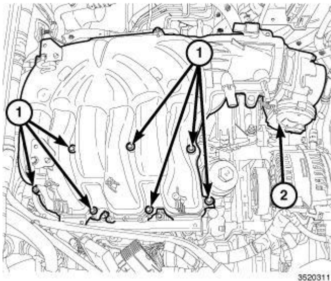
Fig. 223: Upper Intake Manifold & Fasteners Courtesy of CHRYSLER GROUP, LLC
