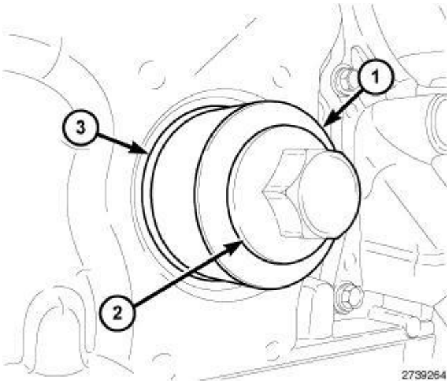
Fig. 427: Front Crankshaft Seal Installer & Oil Seal Courtesy of CHRYSLER GROUP, LLC
