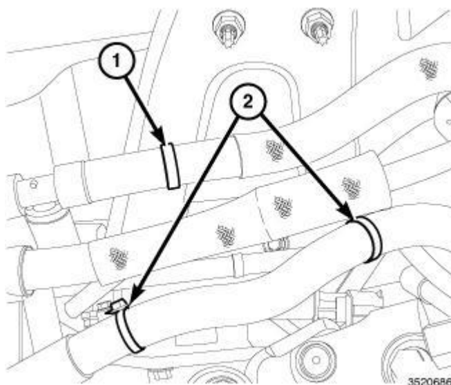
Fig. 587: Brake Booster Hose Retainer & Wire Harness Retainers Courtesy of CHRYSLER GROUP, LLC
