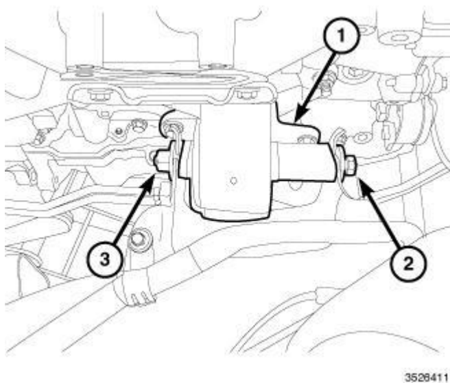
Fig. 441: Right Engine Mount & Fasteners Courtesy of CHRYSLER GROUP, LLC
