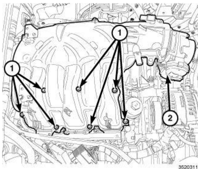
Fig. 566: Upper Intake Manifold & Fasteners Courtesy of CHRYSLER GROUP, LLC
