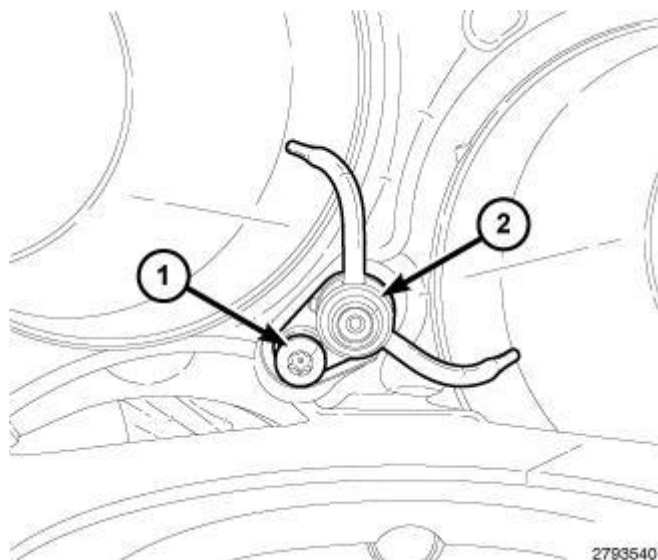
Fig. 485: Piston Oil Cooler Jet & Bolt Courtesy of CHRYSLER GROUP, LLC
