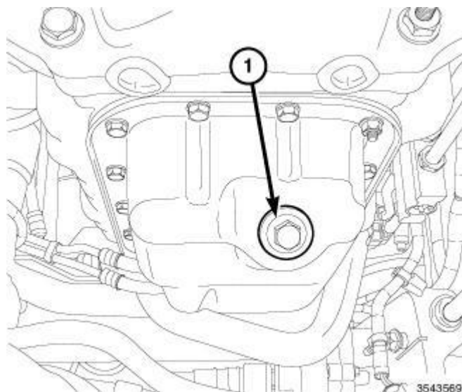
Fig. 488: Oil Pan Drain Plug
