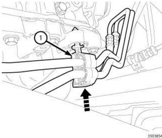
Fig. 515: Engaging Transmission Cooler Line Retainer Courtesy of CHRYSLER GROUP, LLC
