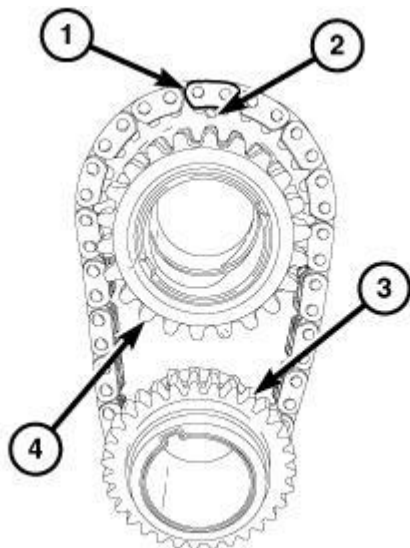
Fig. 633: Placing Idler Sprocket Into Timing Chain So That Dimple Is Aligned With Plated Link On Timing Chain
