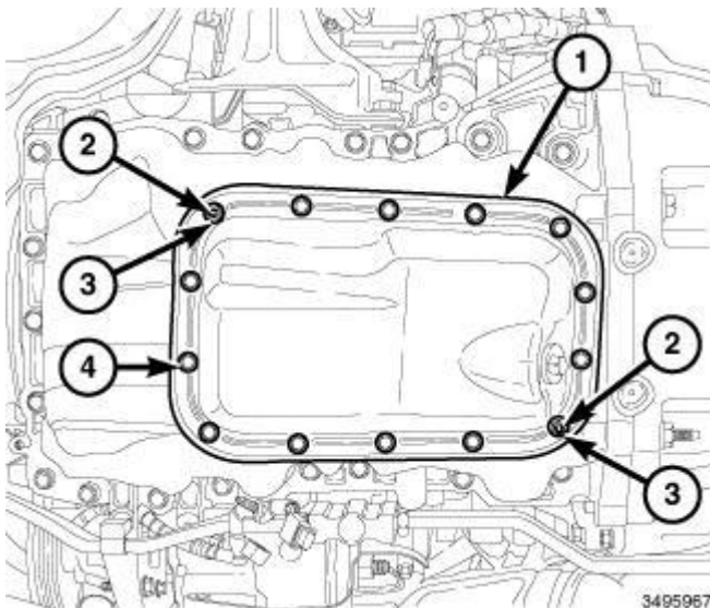
Fig. 498: Lower Oil Pan & Fasteners
