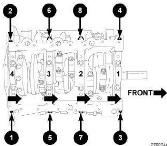
Fig. 376: Main Bearing Tie Bolts Removal Sequence
