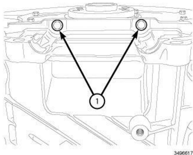
Fig. 513: Rear Oil Seal Retainer Flange Bolts Courtesy of CHRYSLER GROUP, LLC
