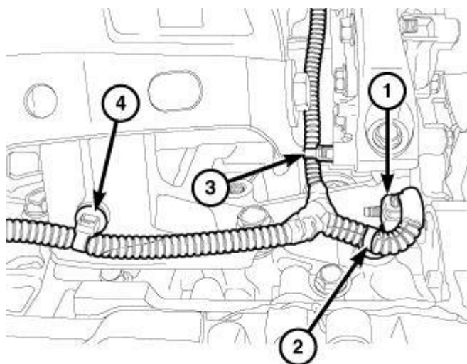
Fig. 10: Oil Pump Solenoid Electrical Connector & Wire Harness Retainers Courtesy of CHRYSLER GROUP, LLC
