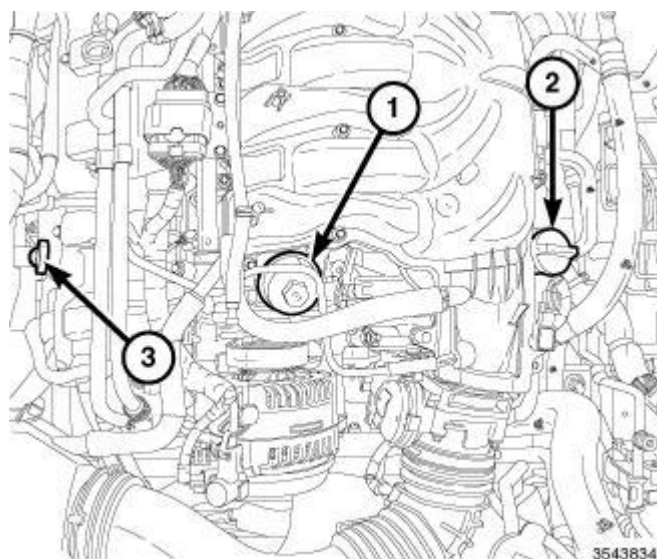
Fig. 491: Oil Filter Cap, Oil Fill Cap & Oil Level Dipstick Courtesy of CHRYSLER GROUP, LLC
