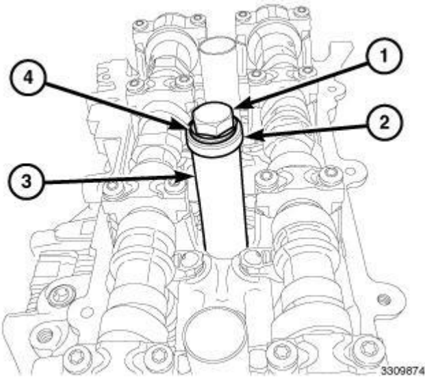
Fig. 318: Spark Plug Tube, Thrust Washers, Spark Plug Tube Installer & Bolt Courtesy of CHRYSLER GROUP, LLC
