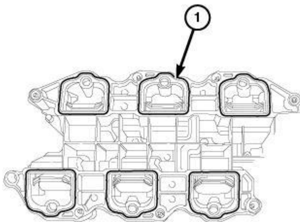
Fig. 575: Lower Intake Manifold To Cylinder Head Seals Courtesy of CHRYSLER GROUP, LLC
