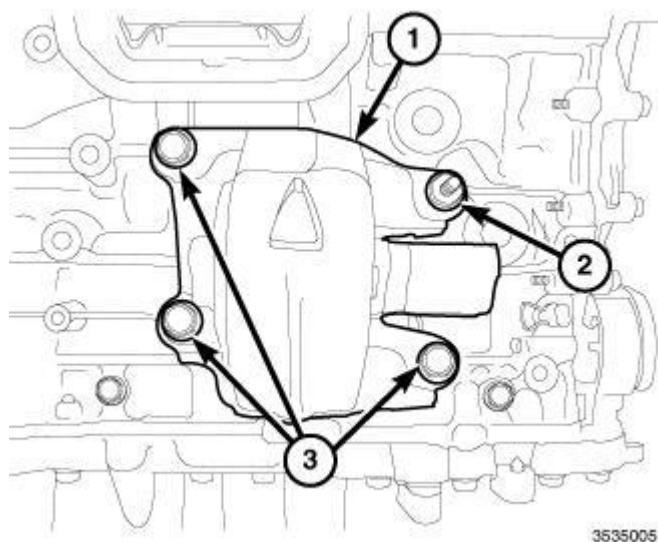
Fig. 369: Right Engine Mount Isolator & Fasteners Courtesy of CHRYSLER GROUP, LLC
