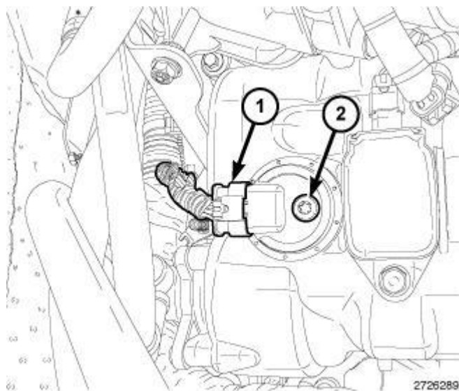
Fig. 247: CMP Sensor & Bolt Courtesy of CHRYSLER GROUP, LLC
