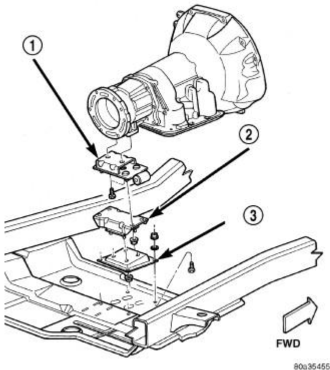
Fig. 451: Rear Engine Mount Isolator & Bracket (Automatic Transmission)
