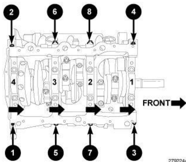
Fig. 361: Main Bearing Tie Bolts Removal Sequence Courtesy of CHRYSLER GROUP, LLC
