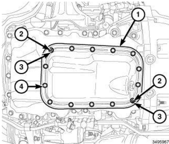
Fig. 508: Lower Oil Pan & Fasteners Courtesy of CHRYSLER GROUP, LLC
