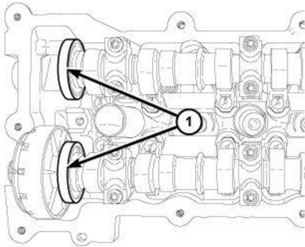
Fig. 222: Magnetic Timing Wheels Courtesy of CHRYSLER GROUP, LLC
