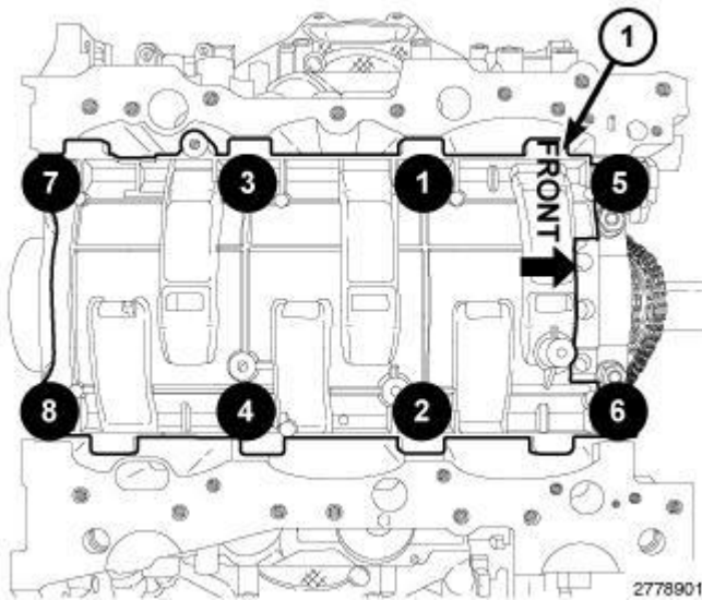
Fig. 387: Windage Tray With Main Bearing Cap Bolts Installation Sequence Courtesy of CHRYSLER GROUP, LLC
