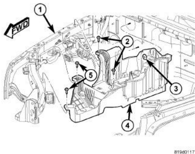
Fig. 305: Battery Tray Components Courtesy of CHRYSLER GROUP, LLC
