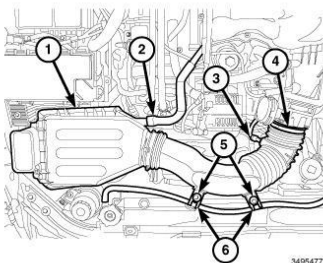
Fig. 664: Air Cleaner Body, Fresh Air Makeup Hose, Electrical Connector, Clamp, Bolts & Retainers
