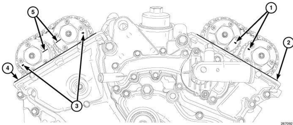
Fig. 611: Arrows, Scribe Lines & Cam Phasers Courtesy of CHRYSLER GROUP, LLC
