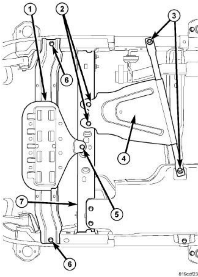
Fig. 443: Crossmember, Skid Plates & Fasteners Courtesy of CHRYSLER GROUP, LLC
