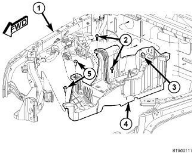
Fig. 8: Battery Tray Components Courtesy of CHRYSLER GROUP, LLC
