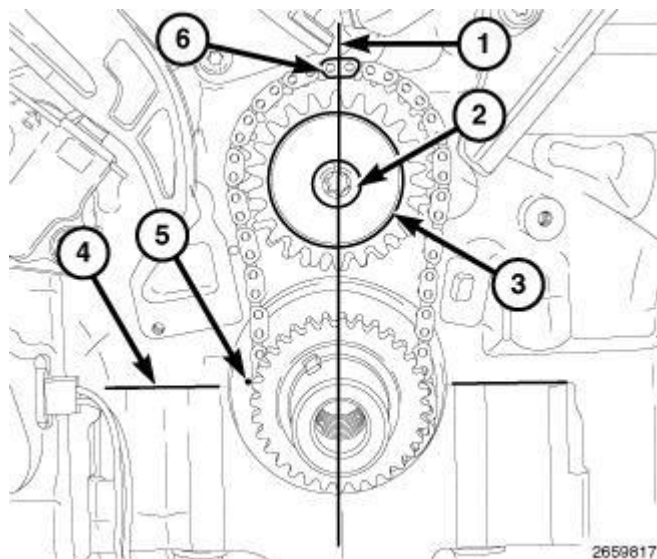
Fig. 623: Timing Chain Plated Link At 12 O'Clock, Washer, Retaining Bolt, Block/Bearing Cap Junction & Dimple Courtesy of CHRYSLER GROUP, LLC
