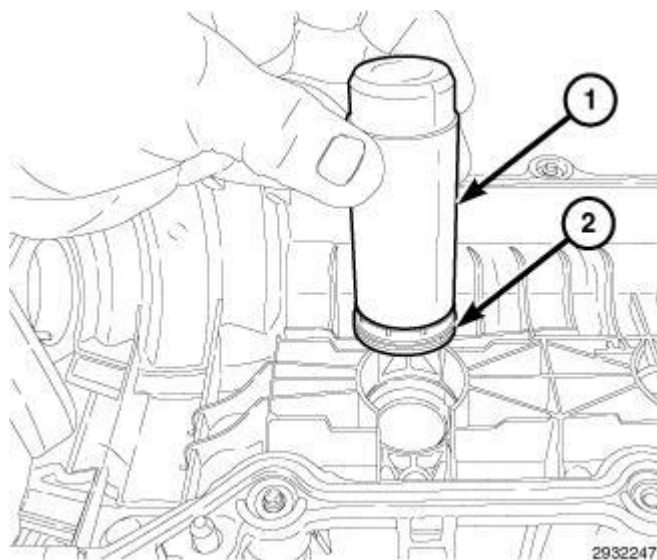
Fig. 253: Spark Plug Tube Seal & Installer
