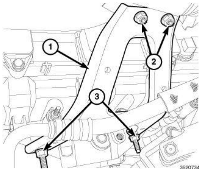
Fig. 586: Left Rear Upper Intake Manifold Support Bracket & Fasteners Courtesy of CHRYSLER GROUP, LLC
