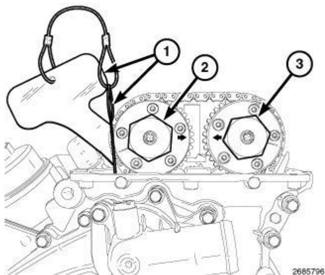
Fig. 173: Pin, Rack, Timing Chain Holder & Oil Control Valves
