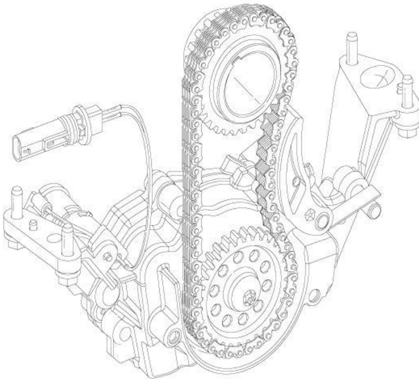
Fig. 522: Oil Pump Chain
