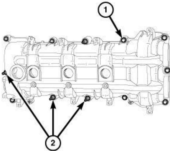
Fig. 235: Cylinder Head Cover Mounting Bolts & Studbolts
