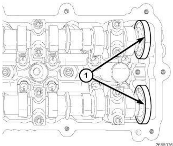
Fig. 199: Magnetic Timing Wheels
