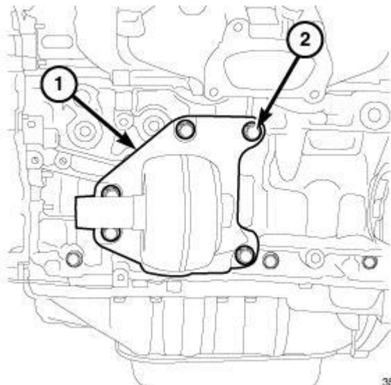
Fig. 434: Left Engine Mount Isolator & Fasteners Courtesy of CHRYSLER GROUP, LLC
