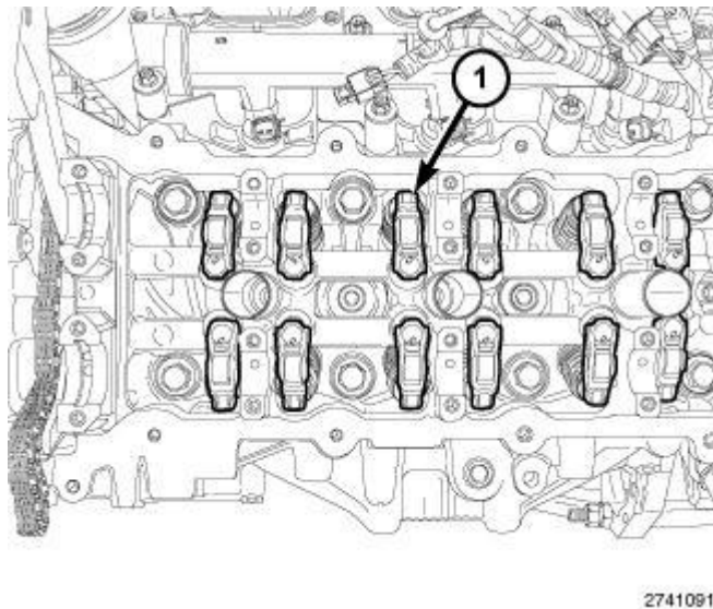
Fig. 289: Locating Rocker Arms Courtesy of CHRYSLER GROUP, LLC
