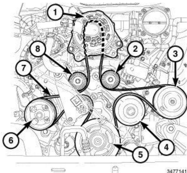
Fig. 660: Drive Belt Tensioners & Assembly With Drive Belt Routing Courtesy of CHRYSLER GROUP, LLC
