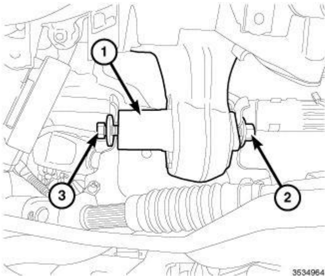
Fig. 433: Engine Mount & Fasteners Courtesy of CHRYSLER GROUP, LLC
