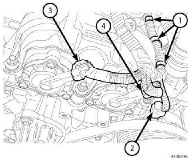
Fig. 213: Retainers, A/C Compressor Electrical Connector & Left Intake And Left Exhaust Variable Valve Timing Solenoid Electrical Connectors Courtesy of CHRYSLER GROUP, LLC
