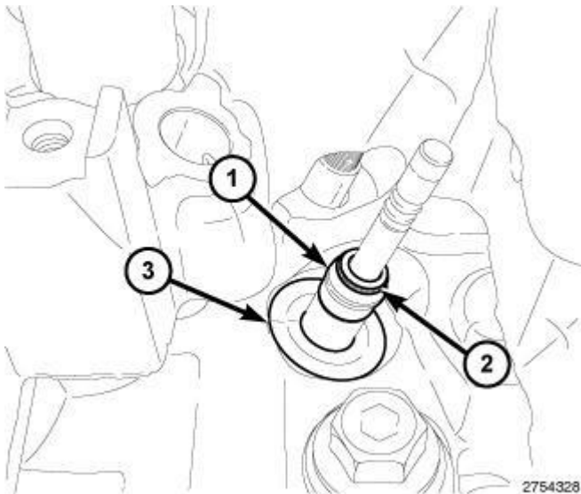
Fig. 308: Spring Seat, Valve Guide Seal & Garter Spring Courtesy of CHRYSLER GROUP, LLC
