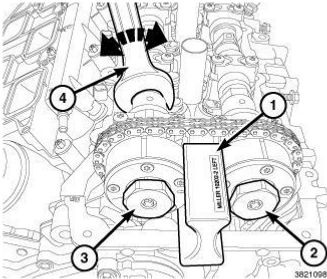
Fig. 621: Camshaft Phaser Lock, Oil Control Valves & Wrench Courtesy of CHRYSLER GROUP, LLC
