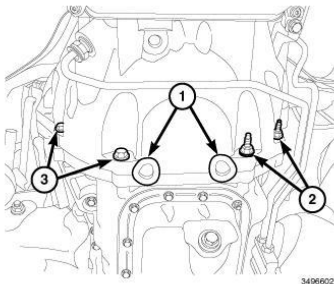
Fig. 511: Rubber Plugs & Transmission To Engine Oil Pan Bolts Courtesy of CHRYSLER GROUP, LLC
