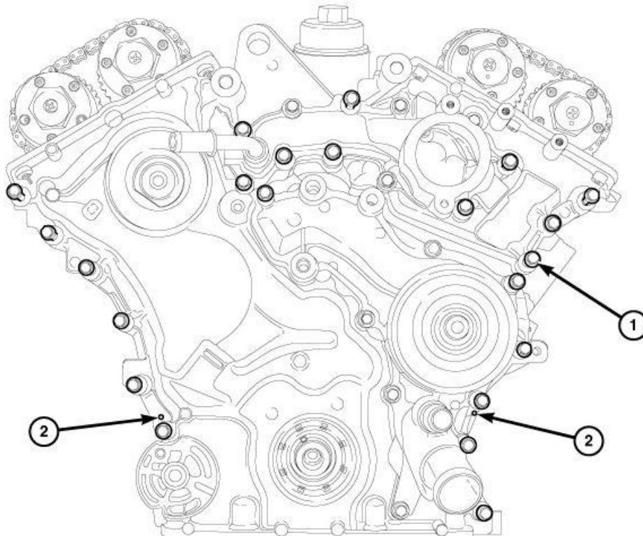
Fig. 651: Engine Timing Cover Bolts & Pins
