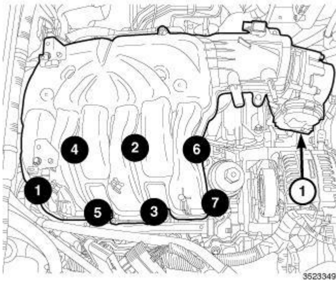
Fig. 583: Upper Intake Manifold Tightening Sequence Courtesy of CHRYSLER GROUP, LLC
