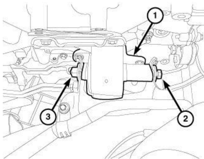
Fig. 438: Right Engine Mount & Fasteners Courtesy of CHRYSLER GROUP, LLC
