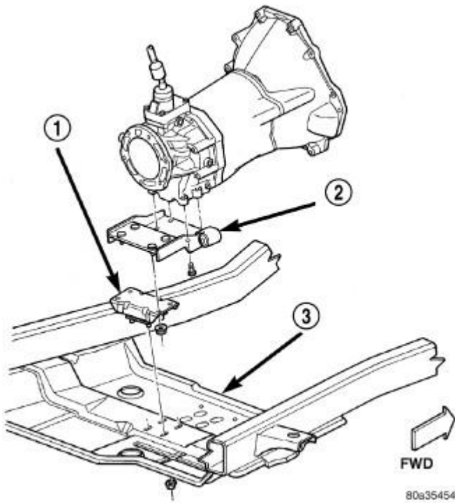
Fig. 448: Rear Engine Mount Isolator & Bracket (Manual Transmission)
