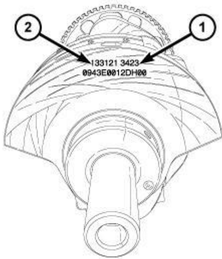
Fig. 344: Crankshaft Main Bearing Journal Diameter Grade Markings & Connecting Rod Bearing Journal Diameter Grade Markings Courtesy of CHRYSLER GROUP, LLC
