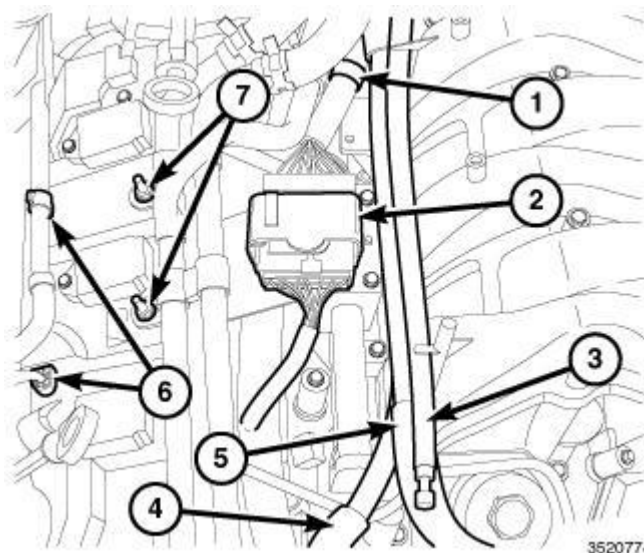
Fig. 585: Transfer Case Vent Hose, Fresh Air Makeup Hose, Positive Crankcase Ventilation (PCV) Hose, Retainers & Fasteners
