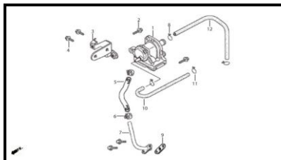
F-17-2 MOFLE 150
