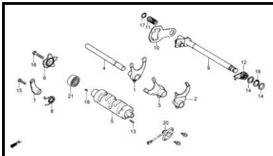
E-15-1 ARRANQUE 2007
