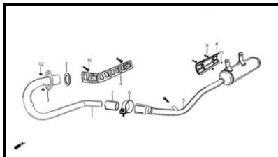
F-19 POSAPIES
